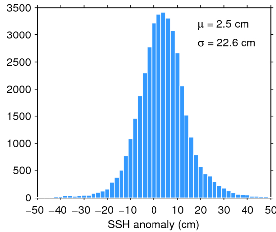
Figure 7. Histogram of flag-valid SSH anomaly over oceans and lakes for 06/05/2017. The mean ( \mu ) and standard deviation ( \sigma ) are also shown. Note that values outside [-50 50] cm are excluded from the histogram for the sake of readability but not from the computation of \mu and \sigma .
