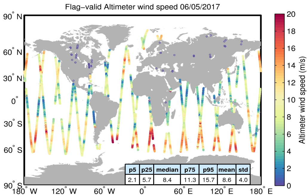
Figure 31. Geographical distribution of flag-valid wind data over oceans and lakes for 06/05/2017. The statistical values shown in the table refer to the wind in m/s and are calculated over all measurements shown in the figure.
