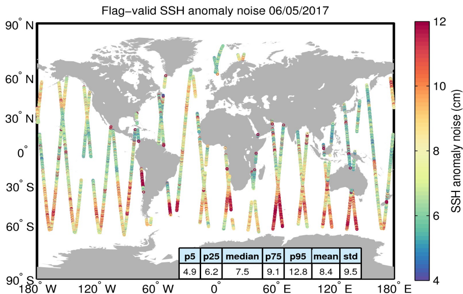
Figure 8. Geographical distribution of flag-valid 20-Hz SSH anomaly measurement noise over oceans and lakes for 06/05/2017. The statistical values shown in the table refer to the SSH anomaly noise and are calculated over all measurements shown in the figure.
