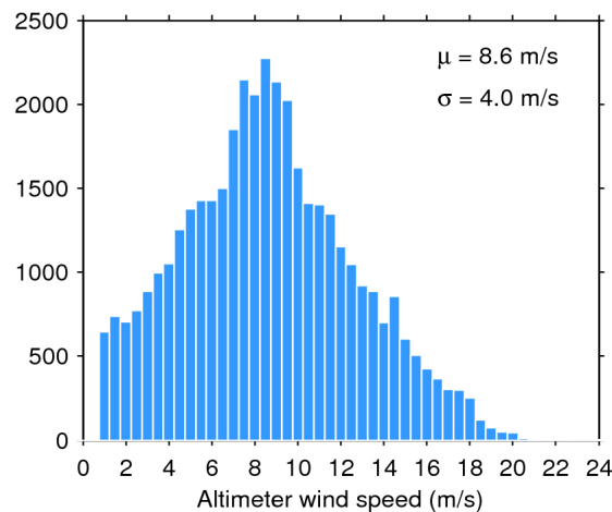
Figure 35. Histogram of science-valid wind over oceans and lakes for 06/05/2017. The mean ( \mu ) and standard deviation ( \sigma ) are also shown. Note that values larger than 24 m/s are excluded from the histogram for the sake of readability but not from the computation of \mu and \sigma .
