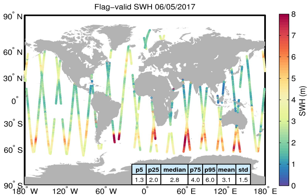
Figure 15. Geographical distribution of flag-valid SWH data over oceans and lakes for 06/05/2017. The statistical values shown in the table refer to the SWH in m and are calculated over all measurements shown in the figure.
