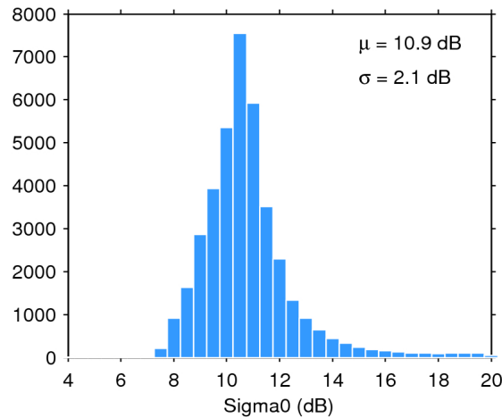
Figure 25. Histogram of flag-valid sigma0 over oceans and lakes for 06/05/2017. The mean ( \mu ) and standard deviation ( \sigma ) are also shown. Note that values outside [4 20] dB are excluded from the histogram for the sake of readability but not from the computation of \mu and \sigma .
