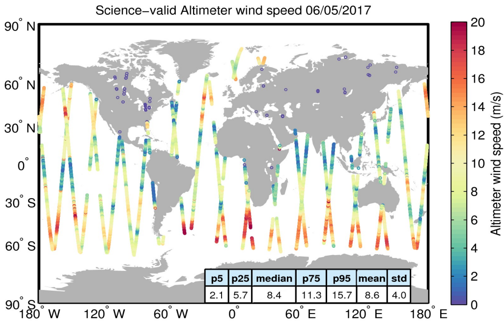
Figure 34. Geographical distribution of science-valid wind data over oceans and lakes for 06/05/2017. The statistical values shown in the table refer to the wind in m/s and are calculated over all measurements shown in the figure. Gray circles denote records that have been rejected based on the editing criteria described in Table 5.
