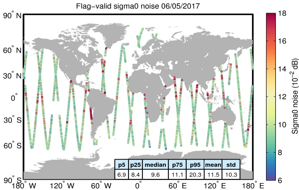
Figure 26. Geographical distribution of flag-valid 20-Hz sigma0 measurement noise over oceans and lakes for 06/05/2017. The statistical values shown in the table refer to the sigma0 noise and are calculated over all measurements shown in the figure.
