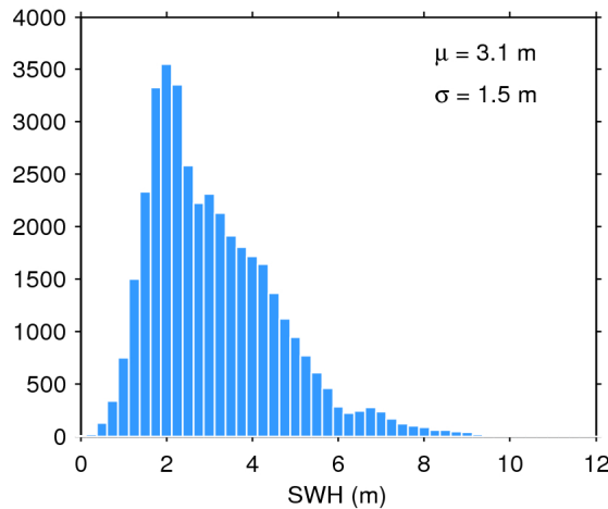
Figure 20. Histogram of science-valid SWH over oceans and lakes for 06/05/2017. The mean ( \mu ) and standard deviation ( \sigma ) are also shown. Note that values larger than 12 m are excluded from the histogram for the sake of readability but not from the computation of \mu and \sigma .
