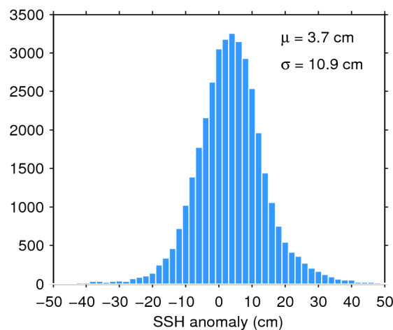
Figure 11. Histogram of science-valid SSH anomaly over oceans and lakes for 06/05/2017. The mean ( \mu ) and standard deviation ( \sigma ) are also shown. Note that values outside [-50 50] cm are excluded from the histogram for the sake of readability but not from the computation of \mu and \sigma .
