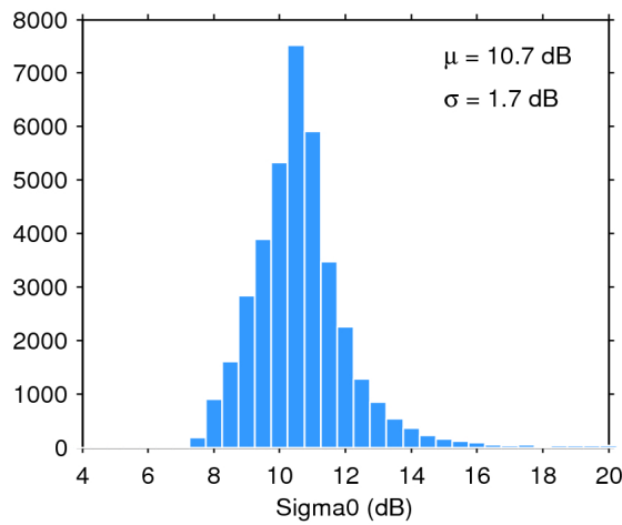
Figure 28. Histogram of science-valid sigma0 over oceans and lakes for 06/05/2017. The mean ( \mu ) and standard deviation ( \sigma ) are also shown. Note that values outside [4 20] dB are excluded from the histogram for the sake of readability but not from the computation of \mu and \sigma .
