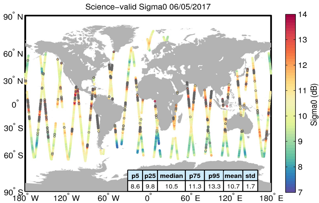
Figure 27. Geographical distribution of science-valid sigma0 data over oceans and lakes for 06/05/2017. The statistical values shown in the table refer to the sigma0 in dB and are calculated over all measurements shown in the figure. Gray circles denote records that have been rejected based on the editing criteria described in Table 4.
