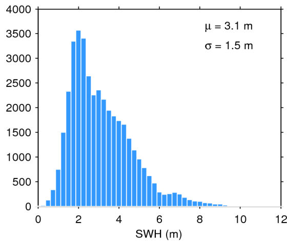
Figure 17. Histogram of flag-valid SWH over oceans and lakes for 06/05/2017. The mean ( \mu ) and standard deviation ( \sigma ) are also shown. Note that values larger than 12 m are excluded from the histogram for the sake of readability but not from the computation of \mu and \sigma .
