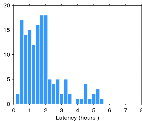
Figure 2. Histogram of the data latency for 06/05/2017. The y-axis denotes the number of files that are made available with a delay of x-hours with respect to the mean time of the records stored in the file.
