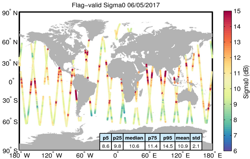
Figure 23. Geographical distribution of flag-valid sigma0 data over oceans and lakes for 06/05/2017. The statistical values shown in the table refer to the sigma0 in dB and are calculated over all measurements shown in the figure.
