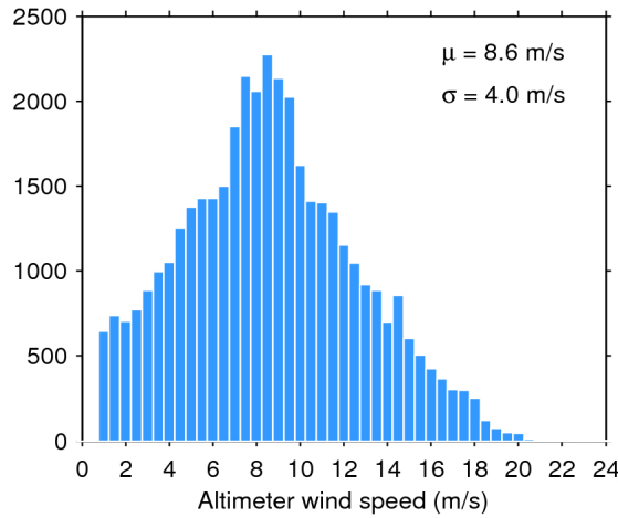
Figure 33. Histogram of flag-valid wind over oceans and lakes for 06/05/2017. The mean ( \mu ) and standard deviation ( \sigma ) are also shown. Note that values larger than 24 m/s are excluded from the histogram for the sake of readability but not from the computation of \mu and \sigma .
