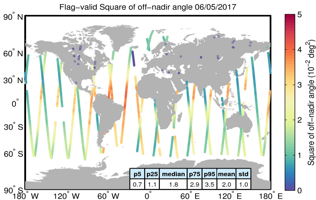
Figure 37. Geographical distribution of flag-valid mispointing data over oceans and lakes for 06/05/2017. The statistical values shown in the table refer to the mispointing in 10^{-2} deg 2 and are calculated over all measurements shown in the figure.
