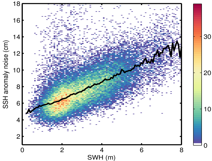
Figure 9. 2D histogram showing flag-valid SSH anomaly noise as a function of SWH for 06/05/2017. The black line denotes the median SSH anomaly noise as a function of SWH.
