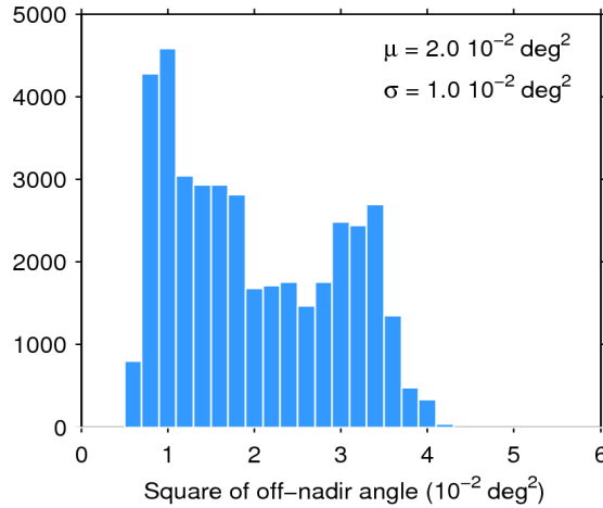
Figure 39. Histogram of flag-valid mispointing over oceans and lakes for 06/05/2017. The mean ( \mu ) and standard deviation ( \sigma ) are also shown. Note that values larger than 6 \cdot 10^{-2} \text{ deg}^2 are excluded from the histogram for the sake of readability but not from the computation of \mu and \sigma .
