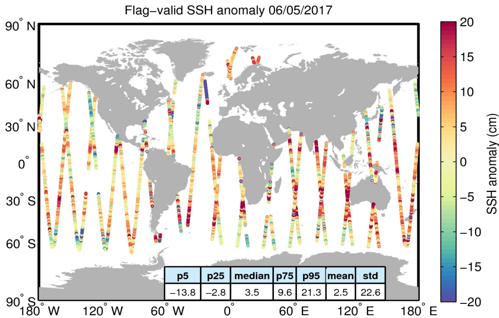
Figure 5. Geographical distribution of flag-valid 1-Hz SSH anomaly data over oceans and lakes for 06/05/2017. The statistical values shown in the table refer to the SSH anomaly in cm and are calculated over all measurements shown in the figure.
