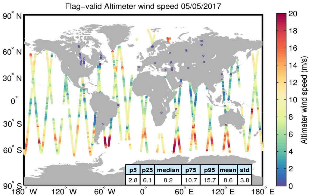
Figure 31. Geographical distribution of flag-valid wind data over oceans and lakes for 05/05/2017. The statistical values shown in the table refer to the wind in m/s and are calculated over all measurements shown in the figure.
