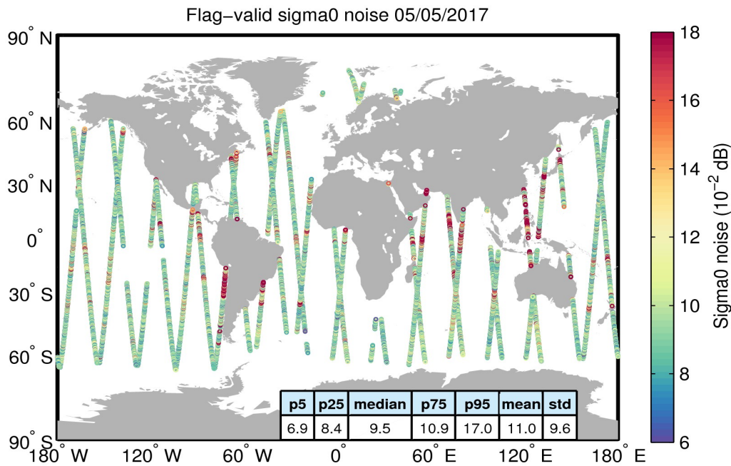
Figure 26. Geographical distribution of flag-valid 20-Hz sigma0 measurement noise over oceans and lakes for 05/05/2017. The statistical values shown in the table refer to the sigma0 noise and are calculated over all measurements shown in the figure.
