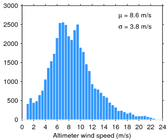
Figure 35. Histogram of science-valid wind over oceans and lakes for 05/05/2017. The mean ( \mu ) and standard deviation ( \sigma ) are also shown. Note that values larger than 24 m/s are excluded from the histogram for the sake of readability but not from the computation of \mu and \sigma .
