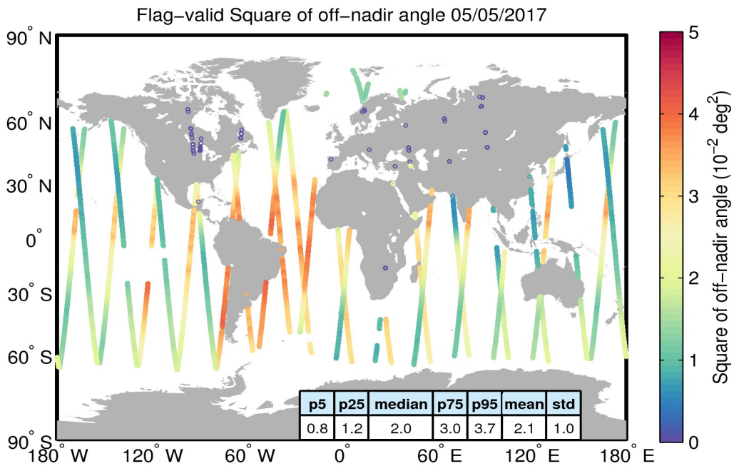
Figure 37. Geographical distribution of flag-valid mispointing data over oceans and lakes for 05/05/2017. The statistical values shown in the table refer to the mispointing in 10^{-2} deg 2 and are calculated over all measurements shown in the figure.
