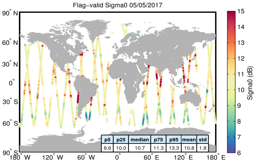
Figure 23. Geographical distribution of flag-valid sigma0 data over oceans and lakes for 05/05/2017. The statistical values shown in the table refer to the sigma0 in dB and are calculated over all measurements shown in the figure.
