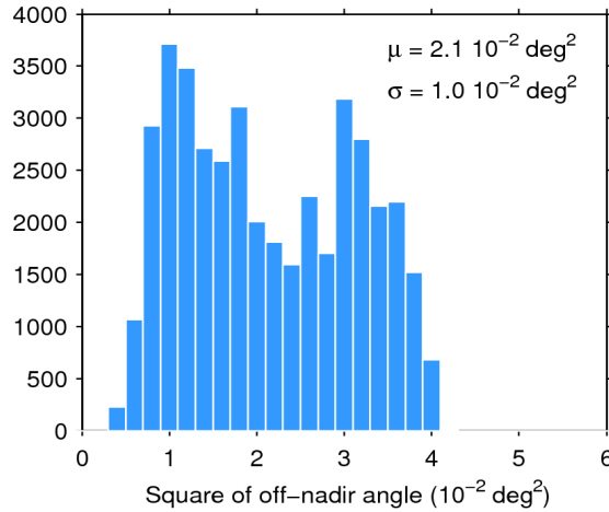
Figure 39. Histogram of flag-valid mispointing over oceans and lakes for 05/05/2017. The mean ( \mu ) and standard deviation ( \sigma ) are also shown. Note that values larger than 6 \cdot 10^{-2} \text{ deg}^2 are excluded from the histogram for the sake of readability but not from the computation of \mu and \sigma .
