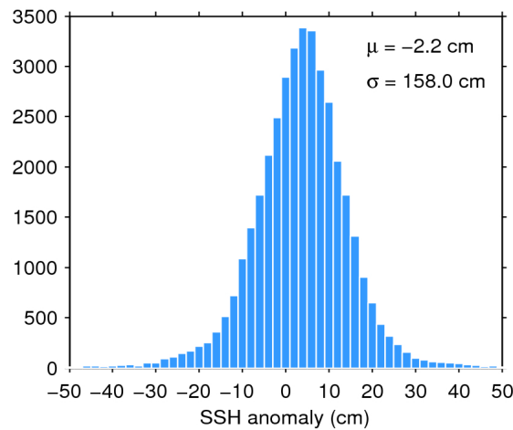
Figure 7. Histogram of flag-valid SSH anomaly over oceans and lakes for 05/05/2017. The mean ( \mu ) and standard deviation ( \sigma ) are also shown. Note that values outside [-50 50] cm are excluded from the histogram for the sake of readability but not from the computation of \mu and \sigma .
