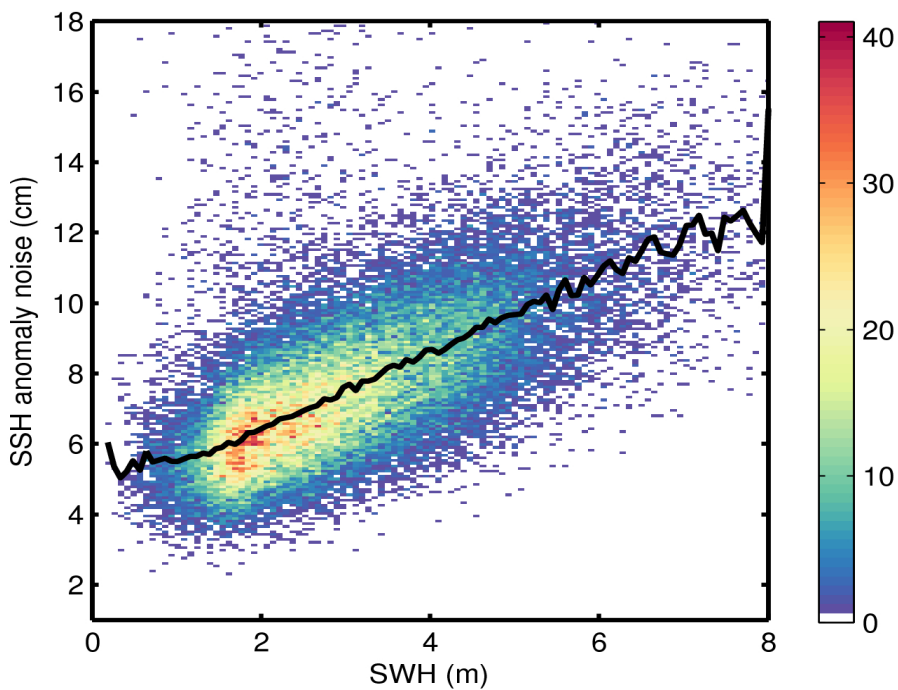
Figure 9. 2D histogram showing flag-valid SSH anomaly noise as a function of SWH for 05/05/2017. The black line denotes the median SSH anomaly noise as a function of SWH.
