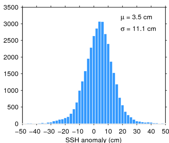
Figure 11. Histogram of science-valid SSH anomaly over oceans and lakes for 05/05/2017. The mean ( \mu ) and standard deviation ( \sigma ) are also shown. Note that values outside [-50 50] cm are excluded from the histogram for the sake of readability but not from the computation of \mu and \sigma .
