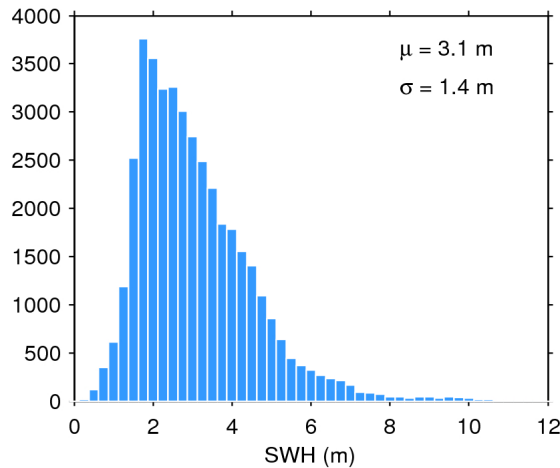
Figure 20. Histogram of science-valid SWH over oceans and lakes for 05/05/2017. The mean ( \mu ) and standard deviation ( \sigma ) are also shown. Note that values larger than 12 m are excluded from the histogram for the sake of readability but not from the computation of \mu and \sigma .
