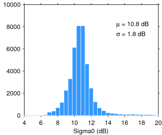
Figure 25. Histogram of flag-valid sigma0 over oceans and lakes for 05/05/2017. The mean ( \mu ) and standard deviation ( \sigma ) are also shown. Note that values outside [4 20] dB are excluded from the histogram for the sake of readability but not from the computation of \mu and \sigma .
