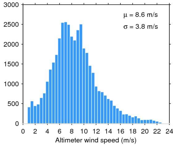
Figure 33. Histogram of flag-valid wind over oceans and lakes for 05/05/2017. The mean ( \mu ) and standard deviation ( \sigma ) are also shown. Note that values larger than 24 m/s are excluded from the histogram for the sake of readability but not from the computation of \mu and \sigma .
