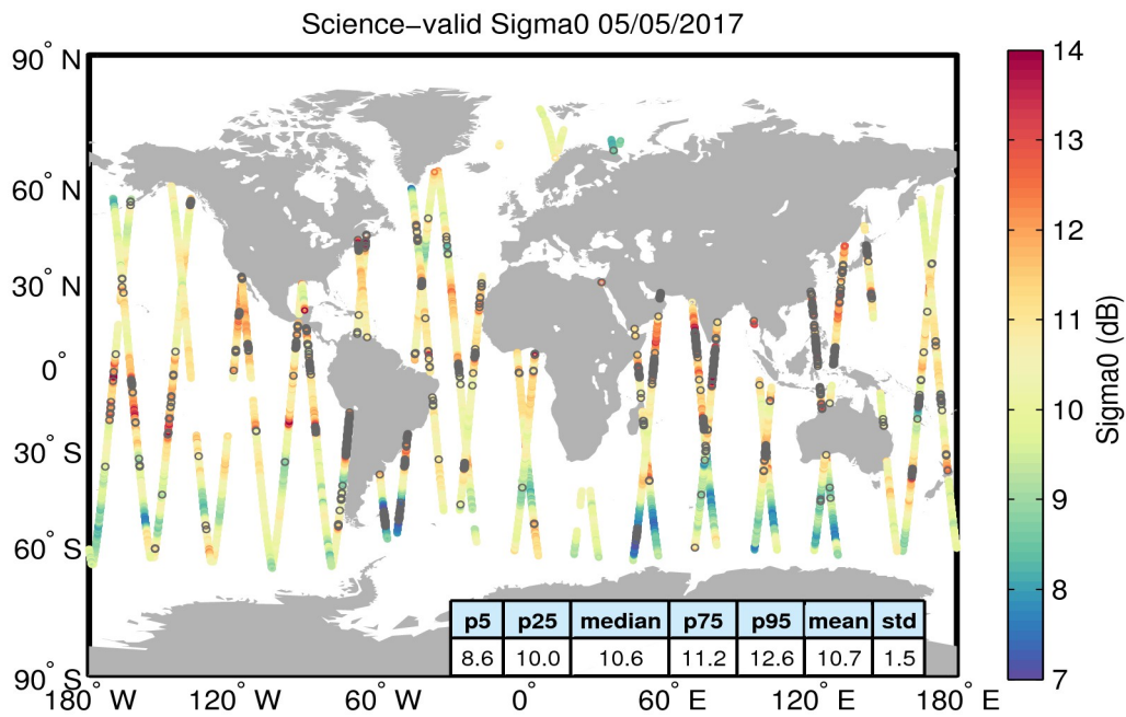
Figure 27. Geographical distribution of science-valid sigma0 data over oceans and lakes for 05/05/2017. The statistical values shown in the table refer to the sigma0 in dB and are calculated over all measurements shown in the figure. Gray circles denote records that have been rejected based on the editing criteria described in Table 4.
