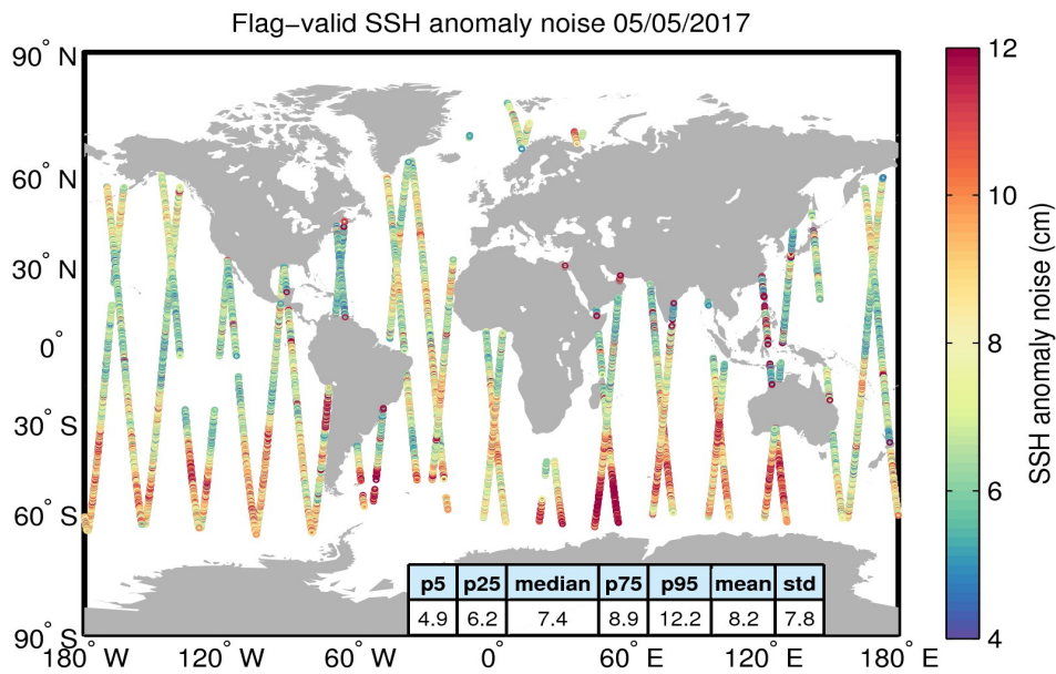
Figure 8. Geographical distribution of flag-valid 20-Hz SSH anomaly measurement noise over oceans and lakes for 05/05/2017. The statistical values shown in the table refer to the SSH anomaly noise and are calculated over all measurements shown in the figure.
