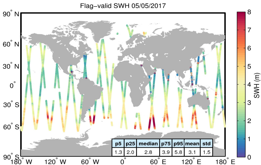
Figure 15. Geographical distribution of flag-valid SWH data over oceans and lakes for 05/05/2017. The statistical values shown in the table refer to the SWH in m and are calculated over all measurements shown in the figure.
