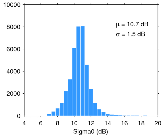
Figure 28. Histogram of science-valid sigma0 over oceans and lakes for 05/05/2017. The mean ( \mu ) and standard deviation ( \sigma ) are also shown. Note that values outside [4 20] dB are excluded from the histogram for the sake of readability but not from the computation of \mu and \sigma .
