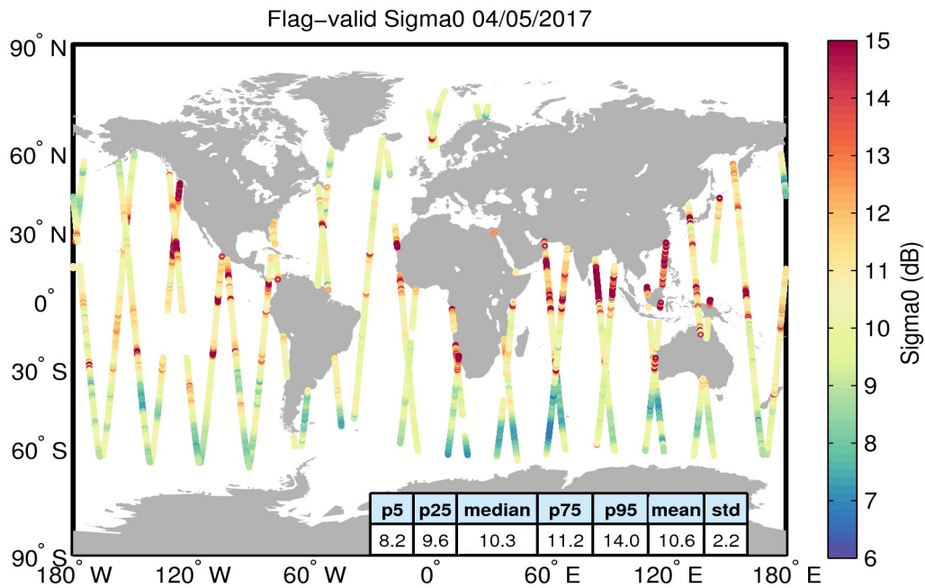
Figure 23. Geographical distribution of flag-valid sigma0 data over oceans and lakes for 04/05/2017. The statistical values shown in the table refer to the sigma0 in dB and are calculated over all measurements shown in the figure.
