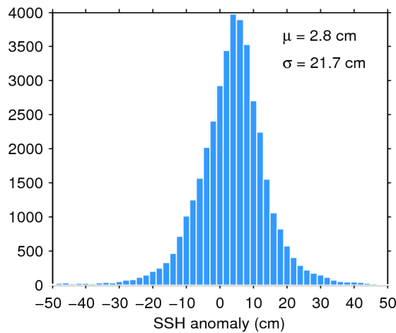
Figure 7. Histogram of flag-valid SSH anomaly over oceans and lakes for 04/05/2017. The mean ( \mu ) and standard deviation ( \sigma ) are also shown. Note that values outside [-50 50] cm are excluded from the histogram for the sake of readability but not from the computation of \mu and \sigma .
