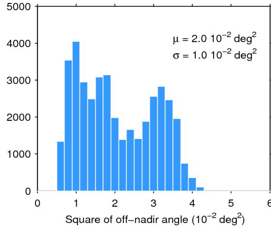
Figure 39. Histogram of flag-valid mispointing over oceans and lakes for 04/05/2017. The mean ( \mu ) and standard deviation ( \sigma ) are also shown. Note that values larger than 6 \cdot 10^{-2} \text{ deg}^2 are excluded from the histogram for the sake of readability but not from the computation of \mu and \sigma .
