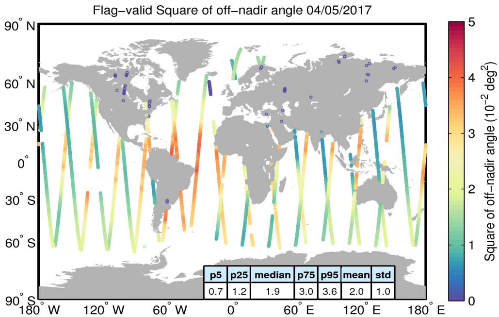
Figure 37. Geographical distribution of flag-valid mispointing data over oceans and lakes for 04/05/2017. The statistical values shown in the table refer to the mispointing in 10^{-2} deg 2 and are calculated over all measurements shown in the figure.
