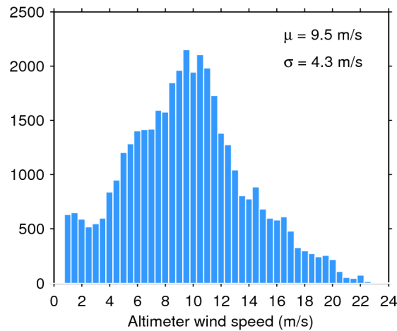
Figure 33. Histogram of flag-valid wind over oceans and lakes for 04/05/2017. The mean ( \mu ) and standard deviation ( \sigma ) are also shown. Note that values larger than 24 m/s are excluded from the histogram for the sake of readability but not from the computation of \mu and \sigma .
