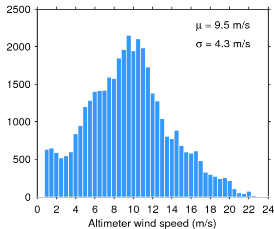
Figure 35. Histogram of science-valid wind over oceans and lakes for 04/05/2017. The mean ( \mu ) and standard deviation ( \sigma ) are also shown. Note that values larger than 24 m/s are excluded from the histogram for the sake of readability but not from the computation of \mu and \sigma .
