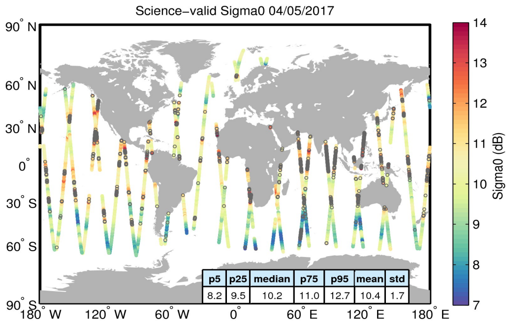
Figure 27. Geographical distribution of science-valid sigma0 data over oceans and lakes for 04/05/2017. The statistical values shown in the table refer to the sigma0 in dB and are calculated over all measurements shown in the figure. Gray circles denote records that have been rejected based on the editing criteria described in Table 4.
