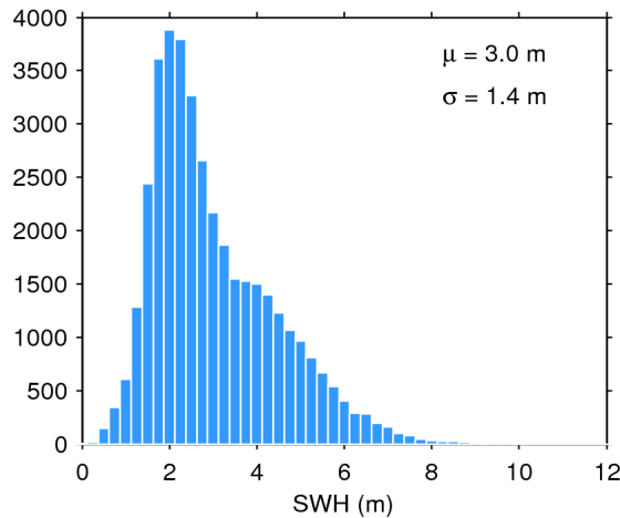
Figure 20. Histogram of science-valid SWH over oceans and lakes for 04/05/2017. The mean ( \mu ) and standard deviation ( \sigma ) are also shown. Note that values larger than 12 m are excluded from the histogram for the sake of readability but not from the computation of \mu and \sigma .
