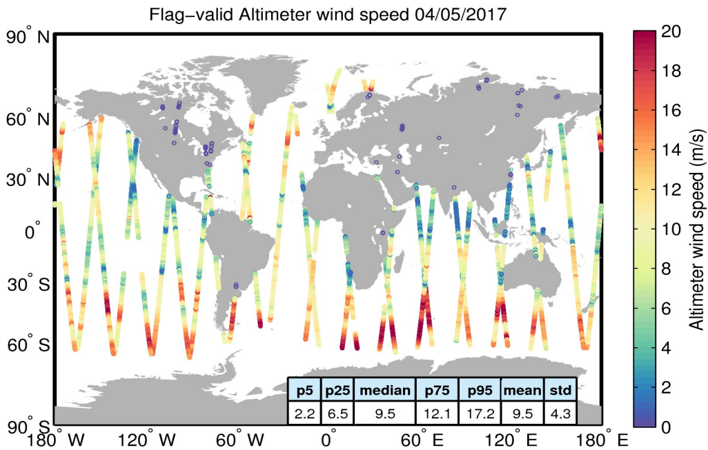
Figure 31. Geographical distribution of flag-valid wind data over oceans and lakes for 04/05/2017. The statistical values shown in the table refer to the wind in m/s and are calculated over all measurements shown in the figure.
