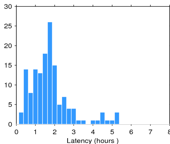
Figure 2. Histogram of the data latency for 04/05/2017. The y-axis denotes the number of files that are made available with a delay of x-hours with respect to the mean time of the records stored in the file.
