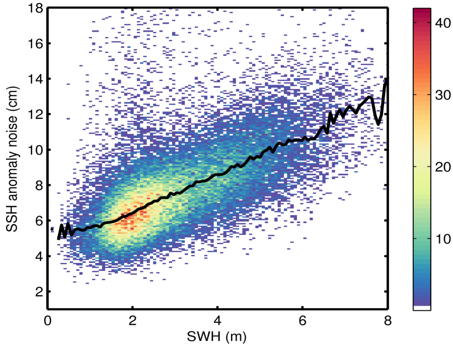
Figure 9. 2D histogram showing flag-valid SSH anomaly noise as a function of SWH for 04/05/2017. The black line denotes the median SSH anomaly noise as a function of SWH.
