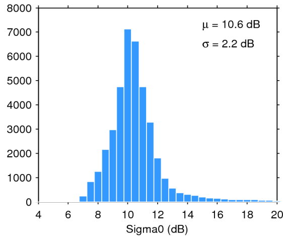
Figure 25. Histogram of flag-valid sigma0 over oceans and lakes for 04/05/2017. The mean ( \mu ) and standard deviation ( \sigma ) are also shown. Note that values outside [4 20] dB are excluded from the histogram for the sake of readability but not from the computation of \mu and \sigma .
