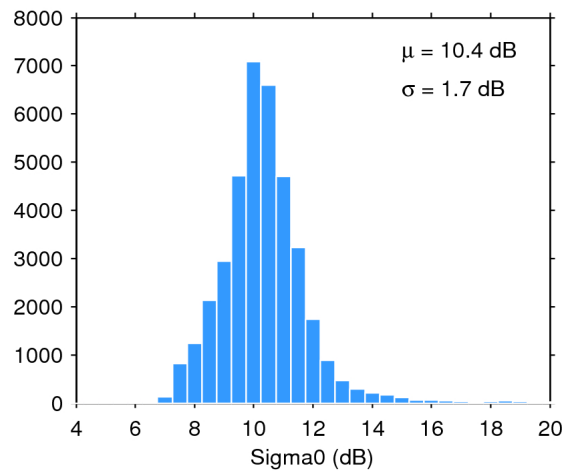
Figure 28. Histogram of science-valid sigma0 over oceans and lakes for 04/05/2017. The mean ( \mu ) and standard deviation ( \sigma ) are also shown. Note that values outside [4 20] dB are excluded from the histogram for the sake of readability but not from the computation of \mu and \sigma .
