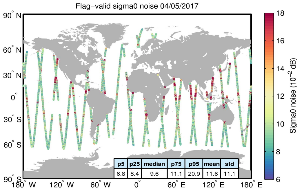
Figure 26. Geographical distribution of flag-valid 20-Hz sigma0 measurement noise over oceans and lakes for 04/05/2017. The statistical values shown in the table refer to the sigma0 noise and are calculated over all measurements shown in the figure.
