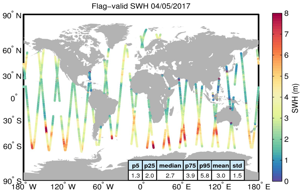
Figure 15. Geographical distribution of flag-valid SWH data over oceans and lakes for 04/05/2017. The statistical values shown in the table refer to the SWH in m and are calculated over all measurements shown in the figure.
