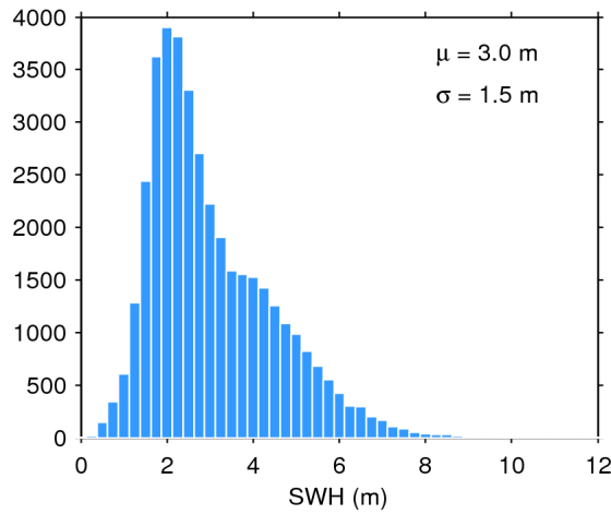
Figure 17. Histogram of flag-valid SWH over oceans and lakes for 04/05/2017. The mean ( \mu ) and standard deviation ( \sigma ) are also shown. Note that values larger than 12 m are excluded from the histogram for the sake of readability but not from the computation of \mu and \sigma .
