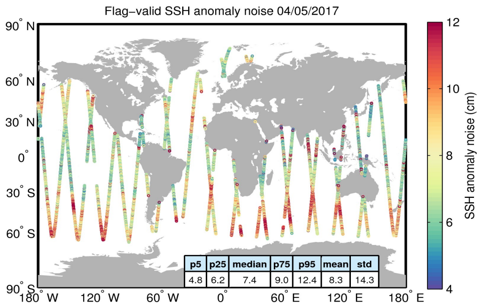
Figure 8. Geographical distribution of flag-valid 20-Hz SSH anomaly measurement noise over oceans and lakes for 04/05/2017. The statistical values shown in the table refer to the SSH anomaly noise and are calculated over all measurements shown in the figure.
