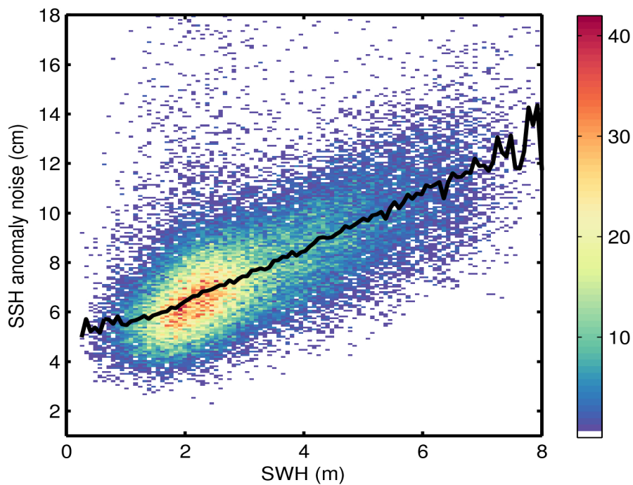
Figure 9. 2D histogram showing flag-valid SSH anomaly noise as a function of SWH for 03/05/2017. The black line denotes the median SSH anomaly noise as a function of SWH.
