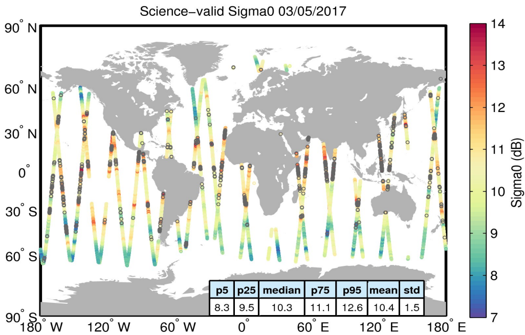
Figure 27. Geographical distribution of science-valid sigma0 data over oceans and lakes for 03/05/2017. The statistical values shown in the table refer to the sigma0 in dB and are calculated over all measurements shown in the figure. Gray circles denote records that have been rejected based on the editing criteria described in Table 4.
