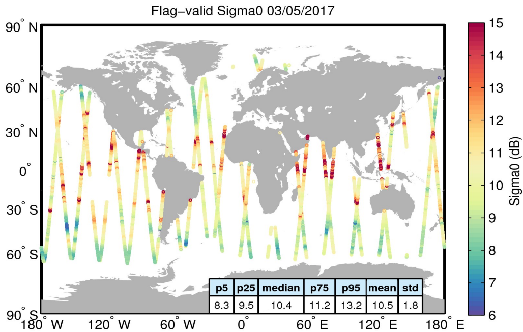
Figure 23. Geographical distribution of flag-valid sigma0 data over oceans and lakes for 03/05/2017. The statistical values shown in the table refer to the sigma0 in dB and are calculated over all measurements shown in the figure.
