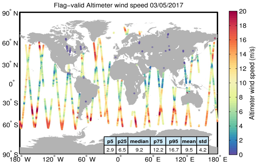
Figure 31. Geographical distribution of flag-valid wind data over oceans and lakes for 03/05/2017. The statistical values shown in the table refer to the wind in m/s and are calculated over all measurements shown in the figure.
