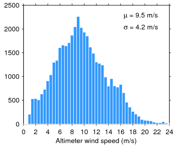
Figure 33. Histogram of flag-valid wind over oceans and lakes for 03/05/2017. The mean ( \mu ) and standard deviation ( \sigma ) are also shown. Note that values larger than 24 m/s are excluded from the histogram for the sake of readability but not from the computation of \mu and \sigma .
