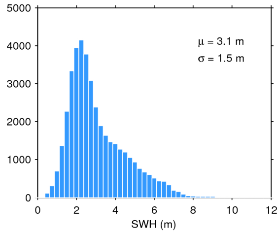
Figure 17. Histogram of flag-valid SWH over oceans and lakes for 03/05/2017. The mean ( \mu ) and standard deviation ( \sigma ) are also shown. Note that values larger than 12 m are excluded from the histogram for the sake of readability but not from the computation of \mu and \sigma .
