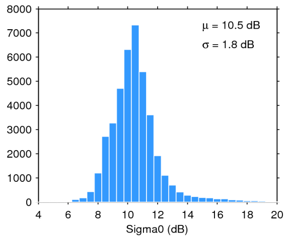
Figure 25. Histogram of flag-valid sigma0 over oceans and lakes for 03/05/2017. The mean ( \mu ) and standard deviation ( \sigma ) are also shown. Note that values outside [4 20] dB are excluded from the histogram for the sake of readability but not from the computation of \mu and \sigma .
