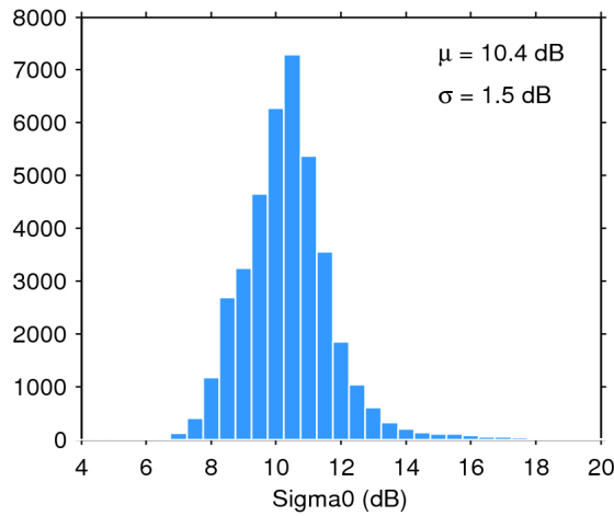
Figure 28. Histogram of science-valid sigma0 over oceans and lakes for 03/05/2017. The mean ( \mu ) and standard deviation ( \sigma ) are also shown. Note that values outside [4 20] dB are excluded from the histogram for the sake of readability but not from the computation of \mu and \sigma .
