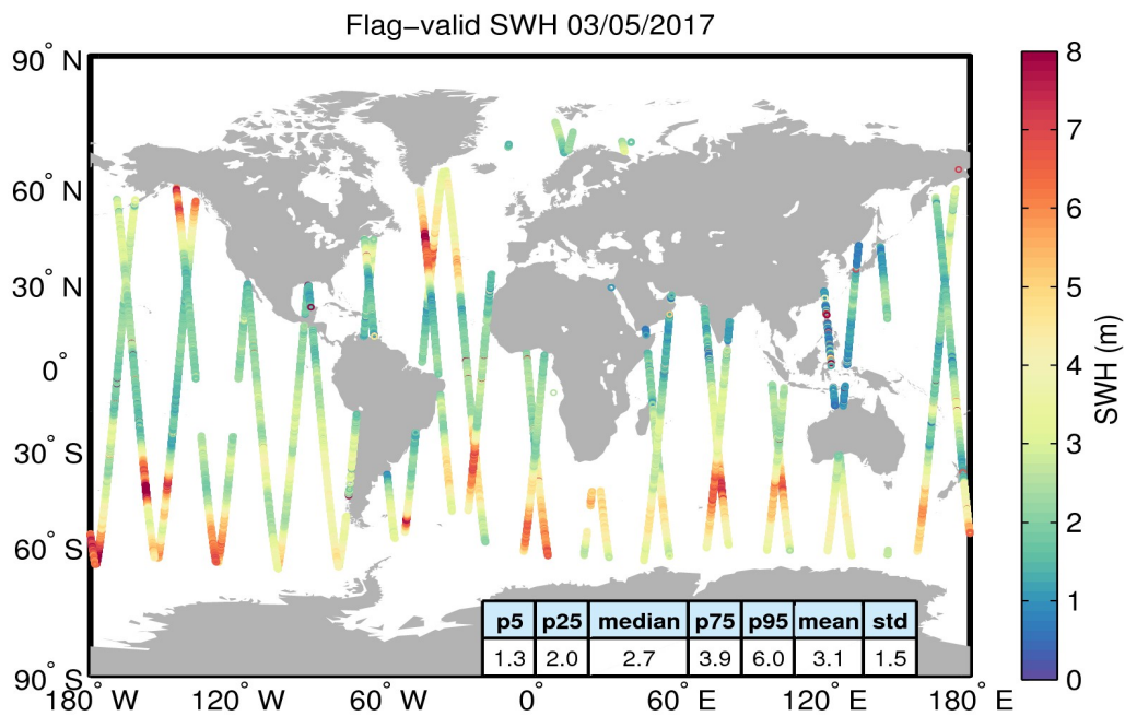
Figure 15. Geographical distribution of flag-valid SWH data over oceans and lakes for 03/05/2017. The statistical values shown in the table refer to the SWH in m and are calculated over all measurements shown in the figure.
