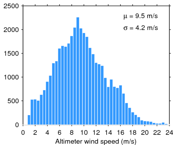
Figure 35. Histogram of science-valid wind over oceans and lakes for 03/05/2017. The mean ( \mu ) and standard deviation ( \sigma ) are also shown. Note that values larger than 24 m/s are excluded from the histogram for the sake of readability but not from the computation of \mu and \sigma .
