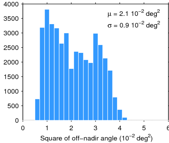
Figure 39. Histogram of flag-valid mispointing over oceans and lakes for 03/05/2017. The mean ( \mu ) and standard deviation ( \sigma ) are also shown. Note that values larger than 6 \cdot 10^{-2} \text{ deg}^2 are excluded from the histogram for the sake of readability but not from the computation of \mu and \sigma .
