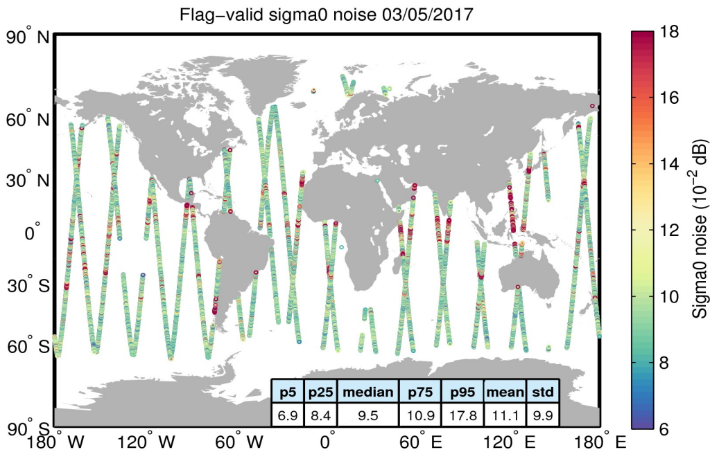
Figure 26. Geographical distribution of flag-valid 20-Hz sigma0 measurement noise over oceans and lakes for 03/05/2017. The statistical values shown in the table refer to the sigma0 noise and are calculated over all measurements shown in the figure.
