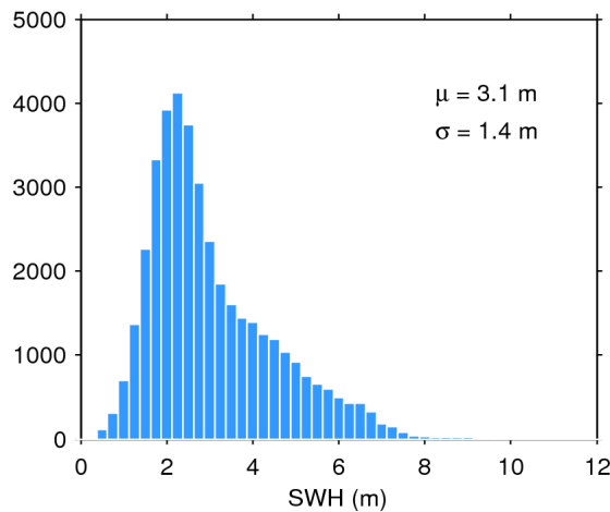
Figure 20. Histogram of science-valid SWH over oceans and lakes for 03/05/2017. The mean ( \mu ) and standard deviation ( \sigma ) are also shown. Note that values larger than 12 m are excluded from the histogram for the sake of readability but not from the computation of \mu and \sigma .
