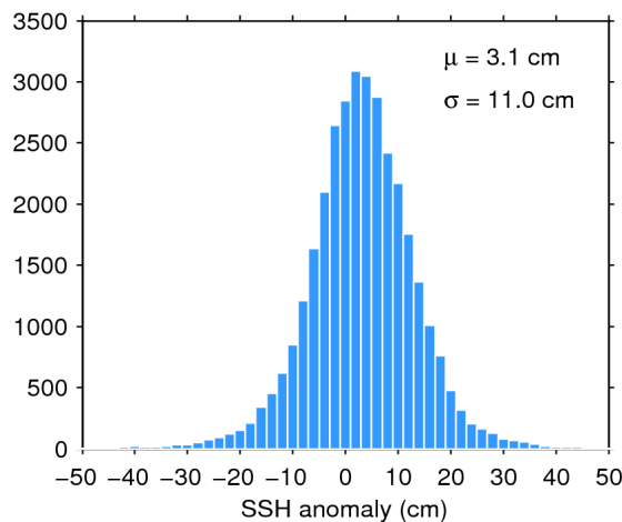
Figure 11. Histogram of science-valid SSH anomaly over oceans and lakes for 03/05/2017. The mean ( \mu ) and standard deviation ( \sigma ) are also shown. Note that values outside [-50 50] cm are excluded from the histogram for the sake of readability but not from the computation of \mu and \sigma .
