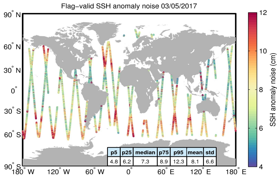
Figure 8. Geographical distribution of flag-valid 20-Hz SSH anomaly measurement noise over oceans and lakes for 03/05/2017. The statistical values shown in the table refer to the SSH anomaly noise and are calculated over all measurements shown in the figure.
