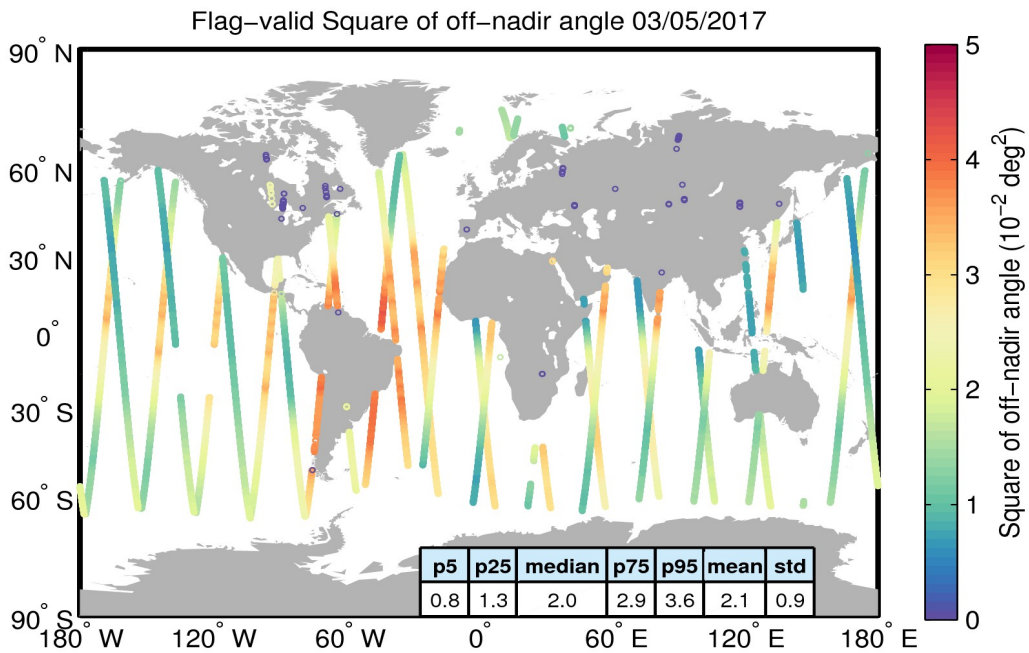
Figure 37. Geographical distribution of flag-valid mispointing data over oceans and lakes for 03/05/2017. The statistical values shown in the table refer to the mispointing in 10^{-2} deg 2 and are calculated over all measurements shown in the figure.
