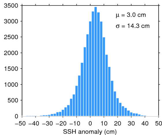
Figure 11. Histogram of science-valid SSH anomaly over oceans and lakes for 02/05/2017. The mean ( \mu ) and standard deviation ( \sigma ) are also shown. Note that values outside [-50 50] cm are excluded from the histogram for the sake of readability but not from the computation of \mu and \sigma .
