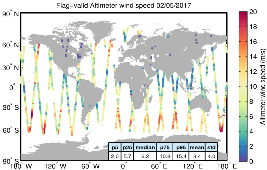
Figure 31. Geographical distribution of flag-valid wind data over oceans and lakes for 02/05/2017. The statistical values shown in the table refer to the wind in m/s and are calculated over all measurements shown in the figure.
