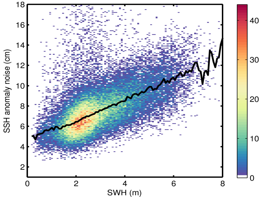
Figure 9. 2D histogram showing flag-valid SSH anomaly noise as a function of SWH for 02/05/2017. The black line denotes the median SSH anomaly noise as a function of SWH.
