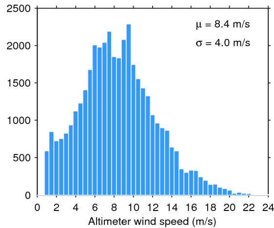
Figure 33. Histogram of flag-valid wind over oceans and lakes for 02/05/2017. The mean ( \mu ) and standard deviation ( \sigma ) are also shown. Note that values larger than 24 m/s are excluded from the histogram for the sake of readability but not from the computation of \mu and \sigma .
