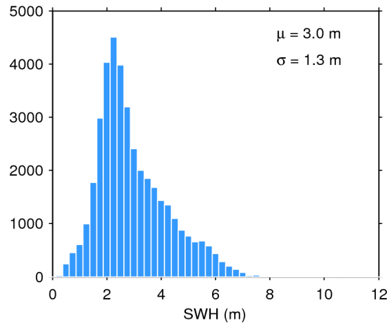
Figure 17. Histogram of flag-valid SWH over oceans and lakes for 02/05/2017. The mean ( \mu ) and standard deviation ( \sigma ) are also shown. Note that values larger than 12 m are excluded from the histogram for the sake of readability but not from the computation of \mu and \sigma .
