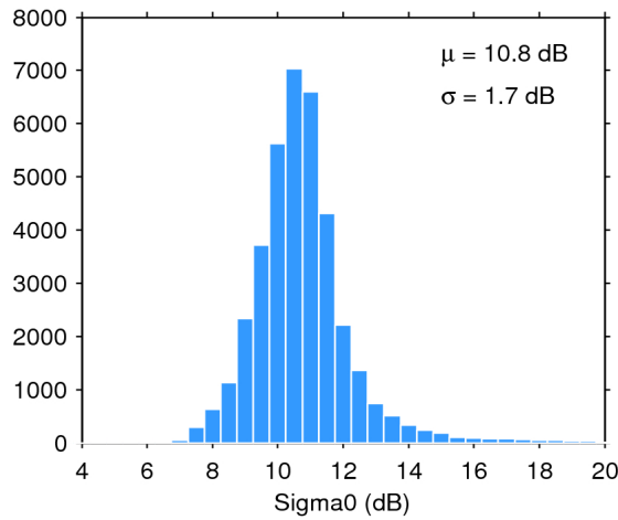
Figure 28. Histogram of science-valid sigma0 over oceans and lakes for 02/05/2017. The mean ( \mu ) and standard deviation ( \sigma ) are also shown. Note that values outside [4 20] dB are excluded from the histogram for the sake of readability but not from the computation of \mu and \sigma .
