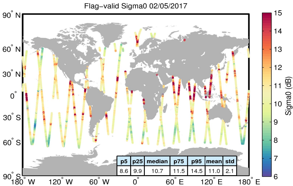
Figure 23. Geographical distribution of flag-valid sigma0 data over oceans and lakes for 02/05/2017. The statistical values shown in the table refer to the sigma0 in dB and are calculated over all measurements shown in the figure.
