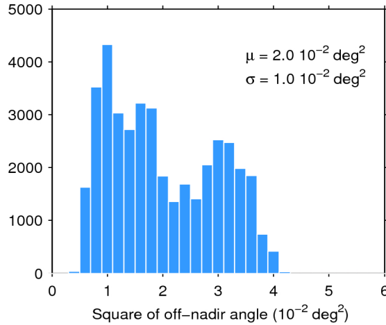
Figure 39. Histogram of flag-valid mispointing over oceans and lakes for 02/05/2017. The mean ( \mu ) and standard deviation ( \sigma ) are also shown. Note that values larger than 6 \cdot 10^{-2} \text{ deg}^2 are excluded from the histogram for the sake of readability but not from the computation of \mu and \sigma .
