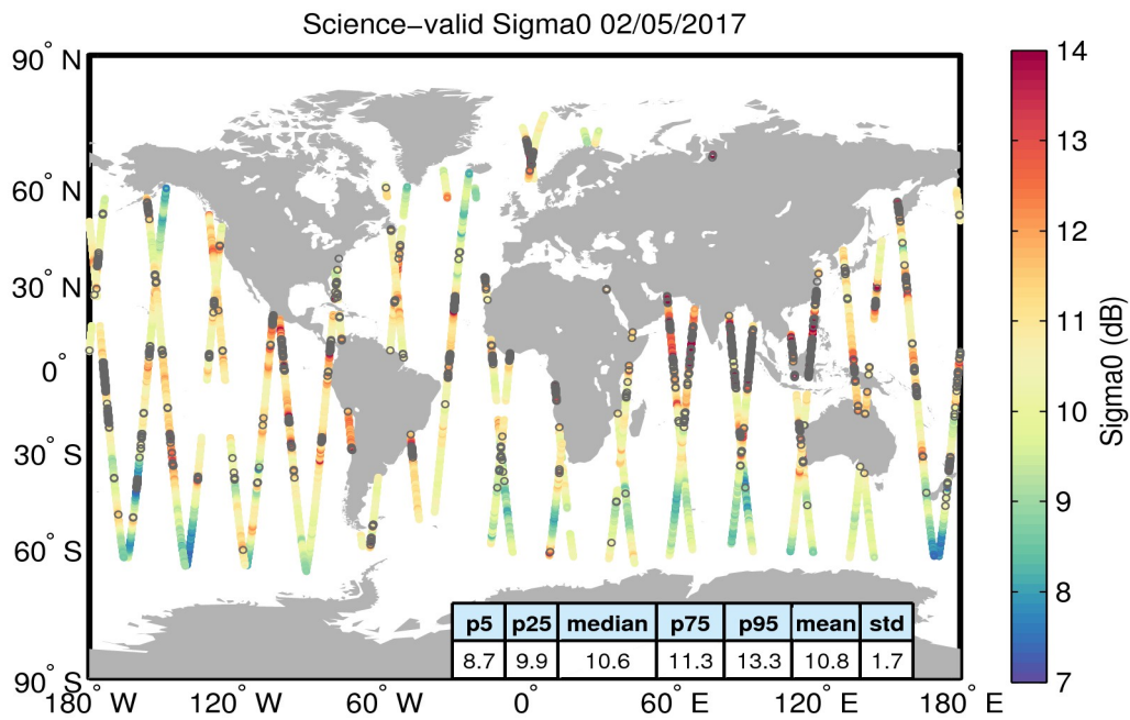
Figure 27. Geographical distribution of science-valid sigma0 data over oceans and lakes for 02/05/2017. The statistical values shown in the table refer to the sigma0 in dB and are calculated over all measurements shown in the figure. Gray circles denote records that have been rejected based on the editing criteria described in Table 4.
