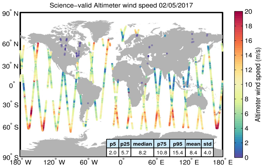
Figure 34. Geographical distribution of science-valid wind data over oceans and lakes for 02/05/2017. The statistical values shown in the table refer to the wind in m/s and are calculated over all measurements shown in the figure. Gray circles denote records that have been rejected based on the editing criteria described in Table 5.
