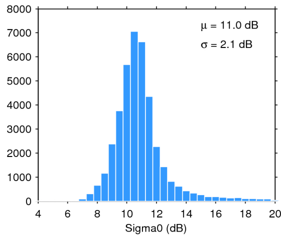
Figure 25. Histogram of flag-valid sigma0 over oceans and lakes for 02/05/2017. The mean ( \mu ) and standard deviation ( \sigma ) are also shown. Note that values outside [4 20] dB are excluded from the histogram for the sake of readability but not from the computation of \mu and \sigma .
