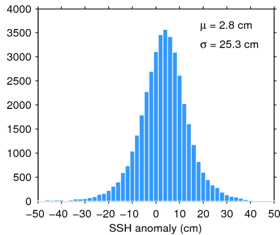
Figure 7. Histogram of flag-valid SSH anomaly over oceans and lakes for 02/05/2017. The mean ( \mu ) and standard deviation ( \sigma ) are also shown. Note that values outside [-50\ 50] cm are excluded from the histogram for the sake of readability but not from the computation of \mu and \sigma .
