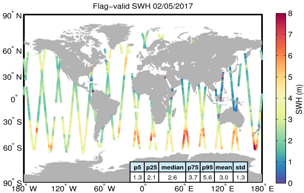
Figure 15. Geographical distribution of flag-valid SWH data over oceans and lakes for 02/05/2017. The statistical values shown in the table refer to the SWH in m and are calculated over all measurements shown in the figure.
