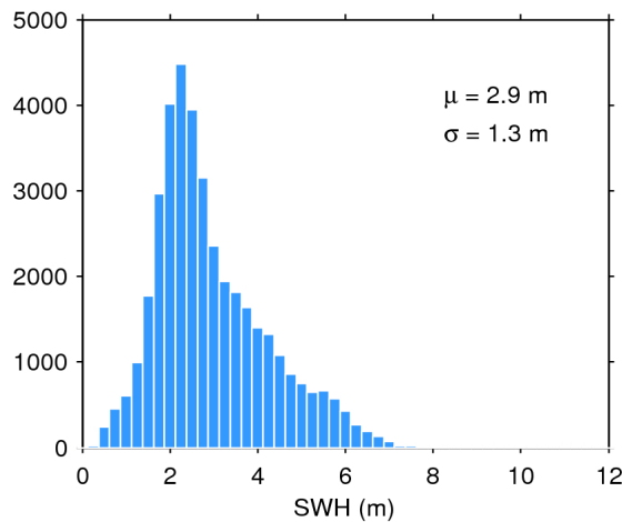
Figure 20. Histogram of science-valid SWH over oceans and lakes for 02/05/2017. The mean ( \mu ) and standard deviation ( \sigma ) are also shown. Note that values larger than 12 m are excluded from the histogram for the sake of readability but not from the computation of \mu and \sigma .
