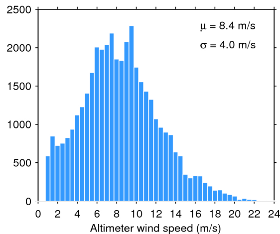
Figure 35. Histogram of science-valid wind over oceans and lakes for 02/05/2017. The mean ( \mu ) and standard deviation ( \sigma ) are also shown. Note that values larger than 24 m/s are excluded from the histogram for the sake of readability but not from the computation of \mu and \sigma .
