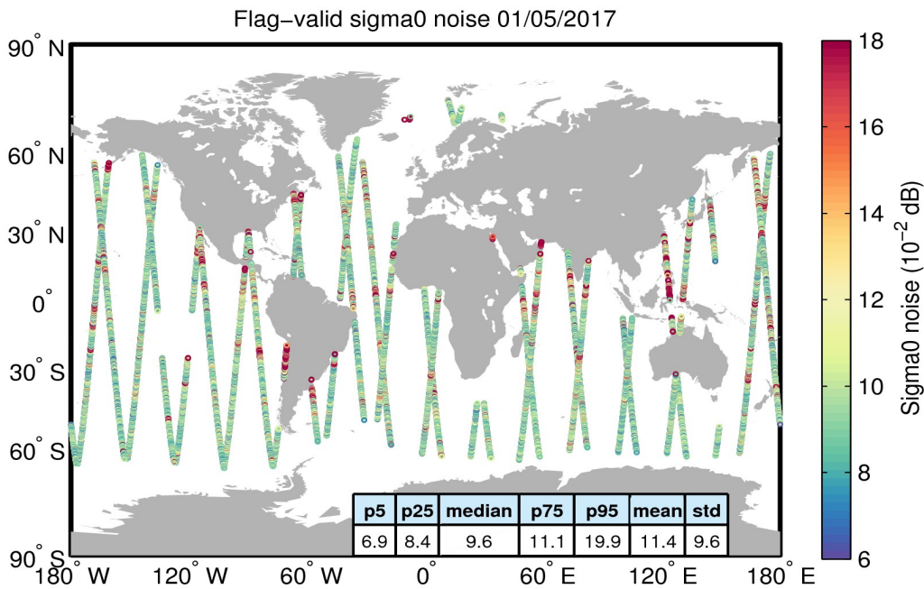
Figure 26. Geographical distribution of flag-valid 20-Hz sigma0 measurement noise over oceans and lakes for 01/05/2017. The statistical values shown in the table refer to the sigma0 noise and are calculated over all measurements shown in the figure.
