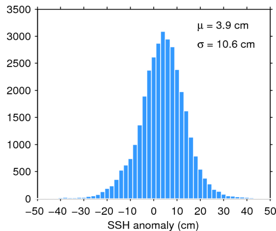
Figure 11. Histogram of science-valid SSH anomaly over oceans and lakes for 01/05/2017. The mean ( \mu ) and standard deviation ( \sigma ) are also shown. Note that values outside [-50 50] cm are excluded from the histogram for the sake of readability but not from the computation of \mu and \sigma .
