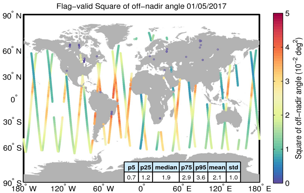
Figure 37. Geographical distribution of flag-valid mispointing data over oceans and lakes for 01/05/2017. The statistical values shown in the table refer to the mispointing in 10^{-2} deg 2 and are calculated over all measurements shown in the figure.
