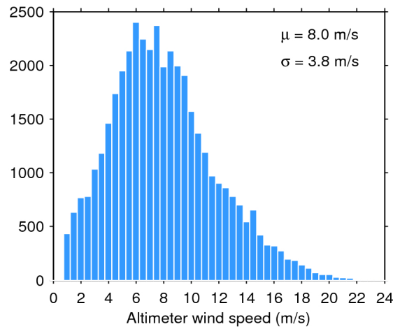
Figure 33. Histogram of flag-valid wind over oceans and lakes for 01/05/2017. The mean ( \mu ) and standard deviation ( \sigma ) are also shown. Note that values larger than 24 m/s are excluded from the histogram for the sake of readability but not from the computation of \mu and \sigma .
