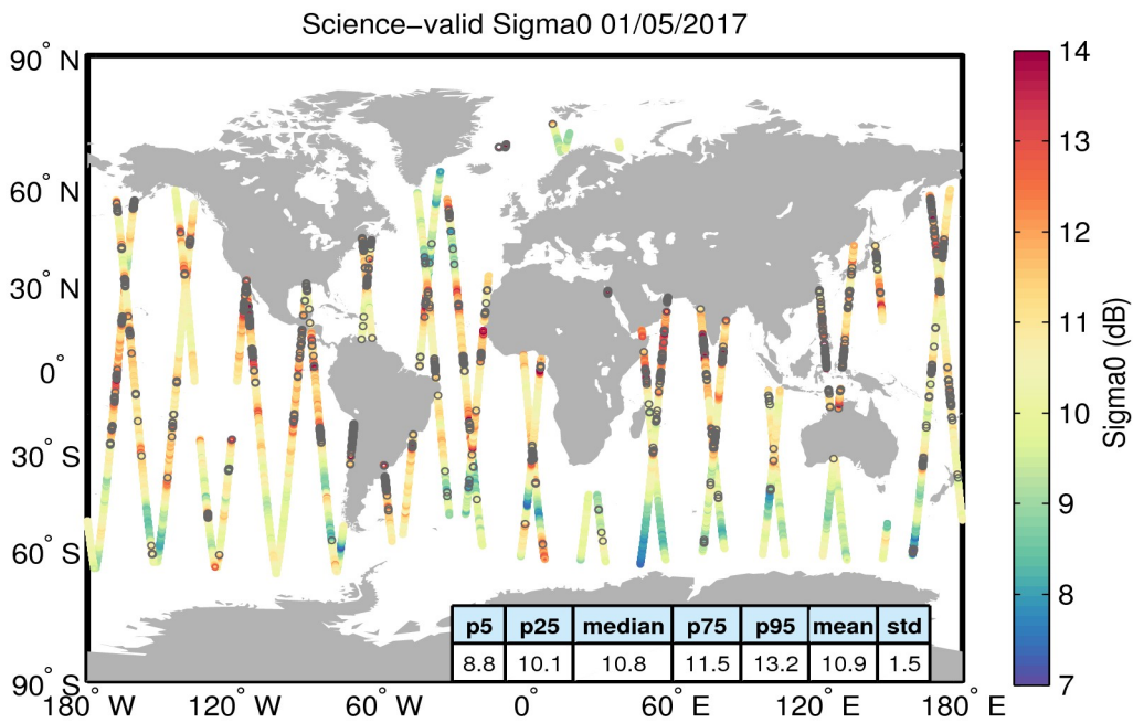
Figure 27. Geographical distribution of science-valid sigma0 data over oceans and lakes for 01/05/2017. The statistical values shown in the table refer to the sigma0 in dB and are calculated over all measurements shown in the figure. Gray circles denote records that have been rejected based on the editing criteria described in Table 4.
