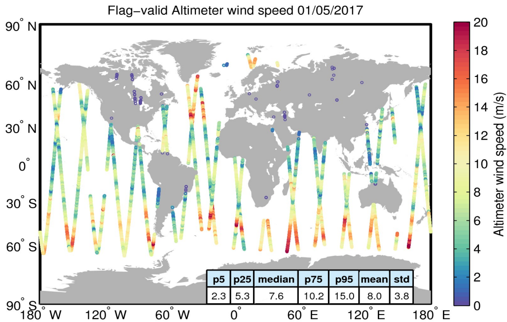
Figure 31. Geographical distribution of flag-valid wind data over oceans and lakes for 01/05/2017. The statistical values shown in the table refer to the wind in m/s and are calculated over all measurements shown in the figure.
