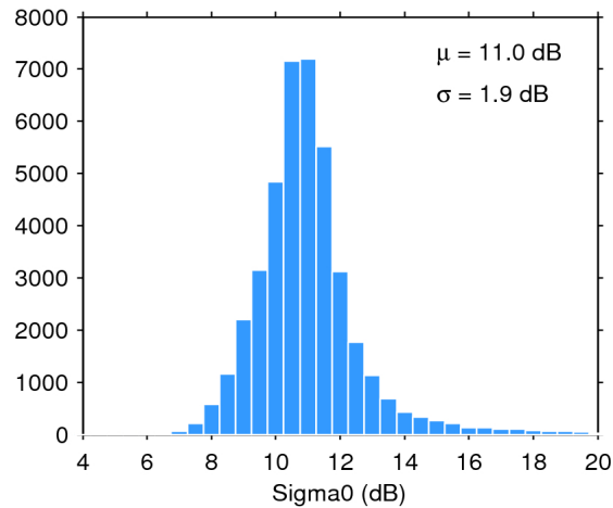
Figure 25. Histogram of flag-valid sigma0 over oceans and lakes for 01/05/2017. The mean ( \mu ) and standard deviation ( \sigma ) are also shown. Note that values outside [4 20] dB are excluded from the histogram for the sake of readability but not from the computation of \mu and \sigma .
