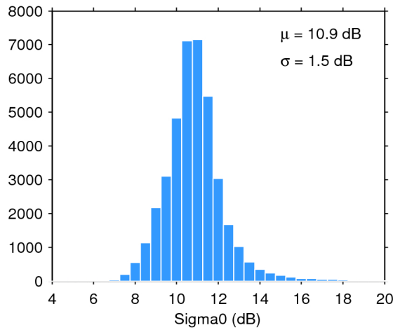
Figure 28. Histogram of science-valid sigma0 over oceans and lakes for 01/05/2017. The mean ( \mu ) and standard deviation ( \sigma ) are also shown. Note that values outside [4 20] dB are excluded from the histogram for the sake of readability but not from the computation of \mu and \sigma .
