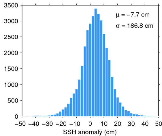
Figure 7. Histogram of flag-valid SSH anomaly over oceans and lakes for 01/05/2017. The mean ( \mu ) and standard deviation ( \sigma ) are also shown. Note that values outside [-50 50] cm are excluded from the histogram for the sake of readability but not from the computation of \mu and \sigma .
