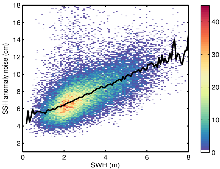
Figure 9. 2D histogram showing flag-valid SSH anomaly noise as a function of SWH for 01/05/2017. The black line denotes the median SSH anomaly noise as a function of SWH.
