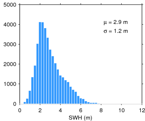
Figure 20. Histogram of science-valid SWH over oceans and lakes for 01/05/2017. The mean ( \mu ) and standard deviation ( \sigma ) are also shown. Note that values larger than 12 m are excluded from the histogram for the sake of readability but not from the computation of \mu and \sigma .
