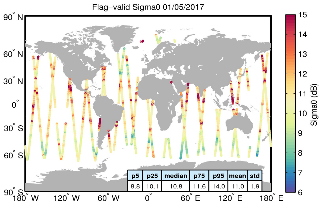
Figure 23. Geographical distribution of flag-valid sigma0 data over oceans and lakes for 01/05/2017. The statistical values shown in the table refer to the sigma0 in dB and are calculated over all measurements shown in the figure.
