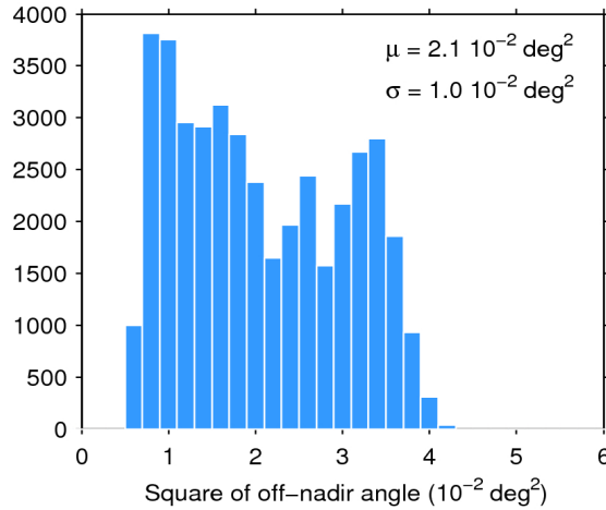
Figure 39. Histogram of flag-valid mispointing over oceans and lakes for 01/05/2017. The mean ( \mu ) and standard deviation ( \sigma ) are also shown. Note that values larger than 6 \cdot 10^{-2} \text{ deg}^2 are excluded from the histogram for the sake of readability but not from the computation of \mu and \sigma .
