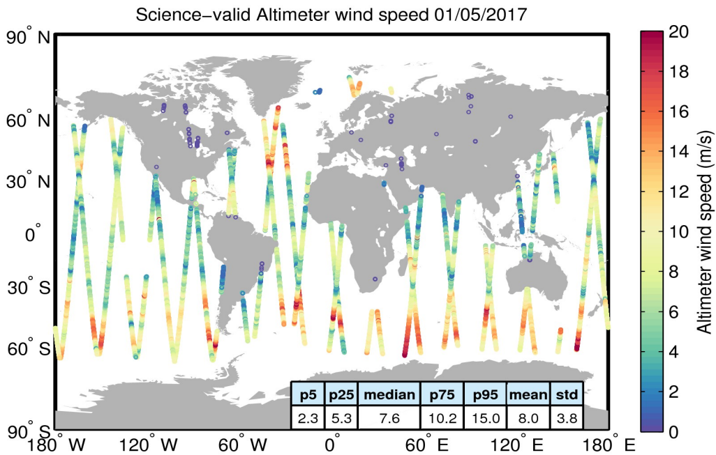
Figure 34. Geographical distribution of science-valid wind data over oceans and lakes for 01/05/2017. The statistical values shown in the table refer to the wind in m/s and are calculated over all measurements shown in the figure. Gray circles denote records that have been rejected based on the editing criteria described in Table 5.
