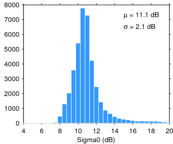
Figure 25. Histogram of flag-valid sigma0 over oceans and lakes for 30/04/2017. The mean ( \mu ) and standard deviation ( \sigma ) are also shown. Note that values outside [4 20] dB are excluded from the histogram for the sake of readability but not from the computation of \mu and \sigma .
