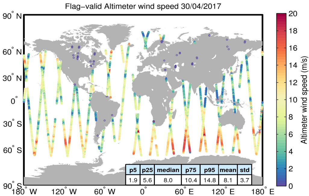
Figure 31. Geographical distribution of flag-valid wind data over oceans and lakes for 30/04/2017. The statistical values shown in the table refer to the wind in m/s and are calculated over all measurements shown in the figure.
