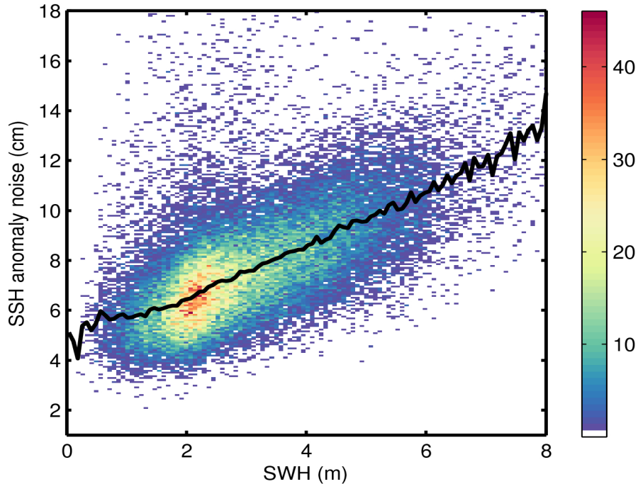
Figure 9. 2D histogram showing flag-valid SSH anomaly noise as a function of SWH for 30/04/2017. The black line denotes the median SSH anomaly noise as a function of SWH.
