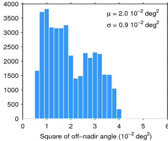
Figure 39. Histogram of flag-valid mispointing over oceans and lakes for 30/04/2017. The mean ( \mu ) and standard deviation ( \sigma ) are also shown. Note that values larger than 6 \cdot 10^{-2} \text{ deg}^2 are excluded from the histogram for the sake of readability but not from the computation of \mu and \sigma .
