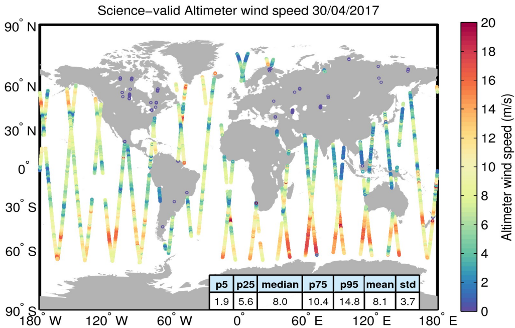
Figure 34. Geographical distribution of science-valid wind data over oceans and lakes for 30/04/2017. The statistical values shown in the table refer to the wind in m/s and are calculated over all measurements shown in the figure. Gray circles denote records that have been rejected based on the editing criteria described in Table 5.
