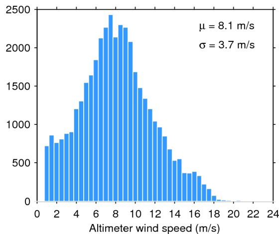
Figure 35. Histogram of science-valid wind over oceans and lakes for 30/04/2017. The mean ( \mu ) and standard deviation ( \sigma ) are also shown. Note that values larger than 24 m/s are excluded from the histogram for the sake of readability but not from the computation of \mu and \sigma .
