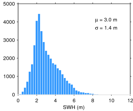
Figure 17. Histogram of flag-valid SWH over oceans and lakes for 30/04/2017. The mean ( \mu ) and standard deviation ( \sigma ) are also shown. Note that values larger than 12 m are excluded from the histogram for the sake of readability but not from the computation of \mu and \sigma .
