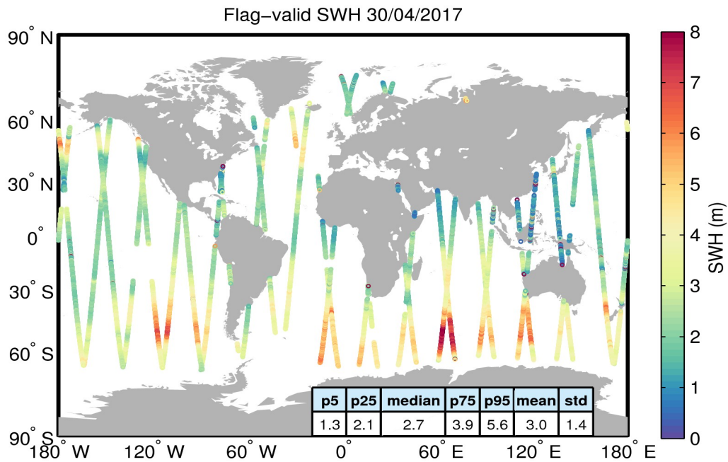
Figure 15. Geographical distribution of flag-valid SWH data over oceans and lakes for 30/04/2017. The statistical values shown in the table refer to the SWH in m and are calculated over all measurements shown in the figure.
