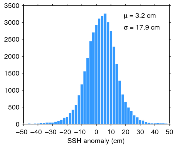
Figure 7. Histogram of flag-valid SSH anomaly over oceans and lakes for 30/04/2017. The mean ( \mu ) and standard deviation ( \sigma ) are also shown. Note that values outside [-50 50] cm are excluded from the histogram for the sake of readability but not from the computation of \mu and \sigma .
