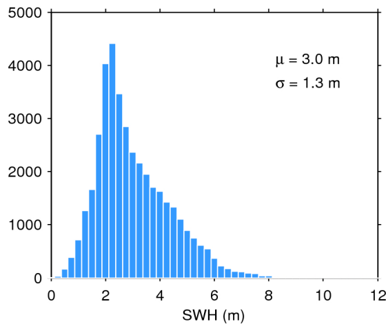
Figure 20. Histogram of science-valid SWH over oceans and lakes for 30/04/2017. The mean ( \mu ) and standard deviation ( \sigma ) are also shown. Note that values larger than 12 m are excluded from the histogram for the sake of readability but not from the computation of \mu and \sigma .
