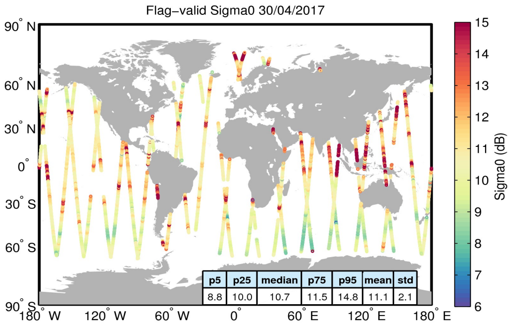
Figure 23. Geographical distribution of flag-valid sigma0 data over oceans and lakes for 30/04/2017. The statistical values shown in the table refer to the sigma0 in dB and are calculated over all measurements shown in the figure.
