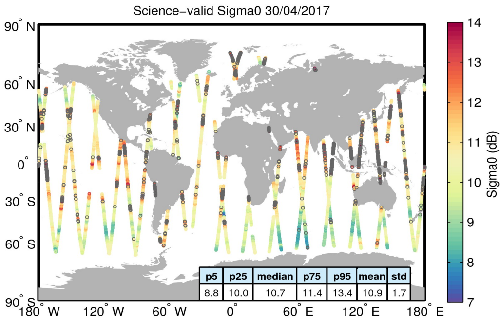
Figure 27. Geographical distribution of science-valid sigma0 data over oceans and lakes for 30/04/2017. The statistical values shown in the table refer to the sigma0 in dB and are calculated over all measurements shown in the figure. Gray circles denote records that have been rejected based on the editing criteria described in Table 4.
