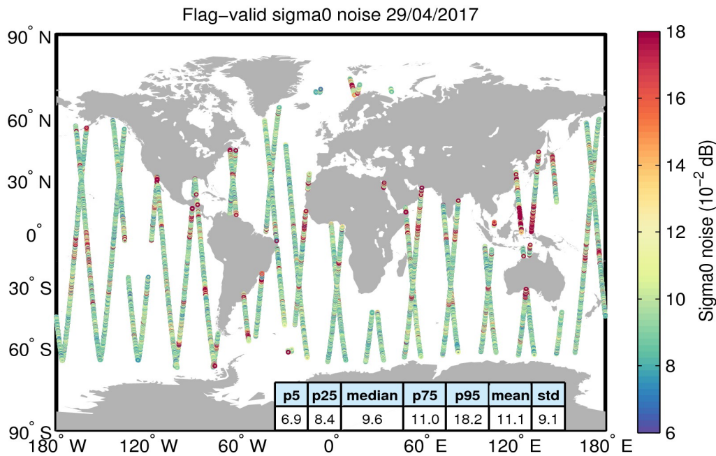
Figure 26. Geographical distribution of flag-valid 20-Hz sigma0 measurement noise over oceans and lakes for 29/04/2017. The statistical values shown in the table refer to the sigma0 noise and are calculated over all measurements shown in the figure.
