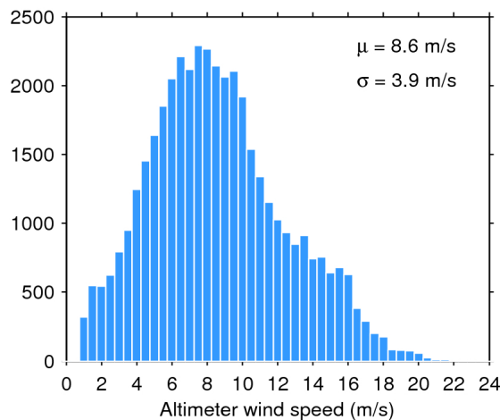
Figure 35. Histogram of science-valid wind over oceans and lakes for 29/04/2017. The mean ( \mu ) and standard deviation ( \sigma ) are also shown. Note that values larger than 24 m/s are excluded from the histogram for the sake of readability but not from the computation of \mu and \sigma .
