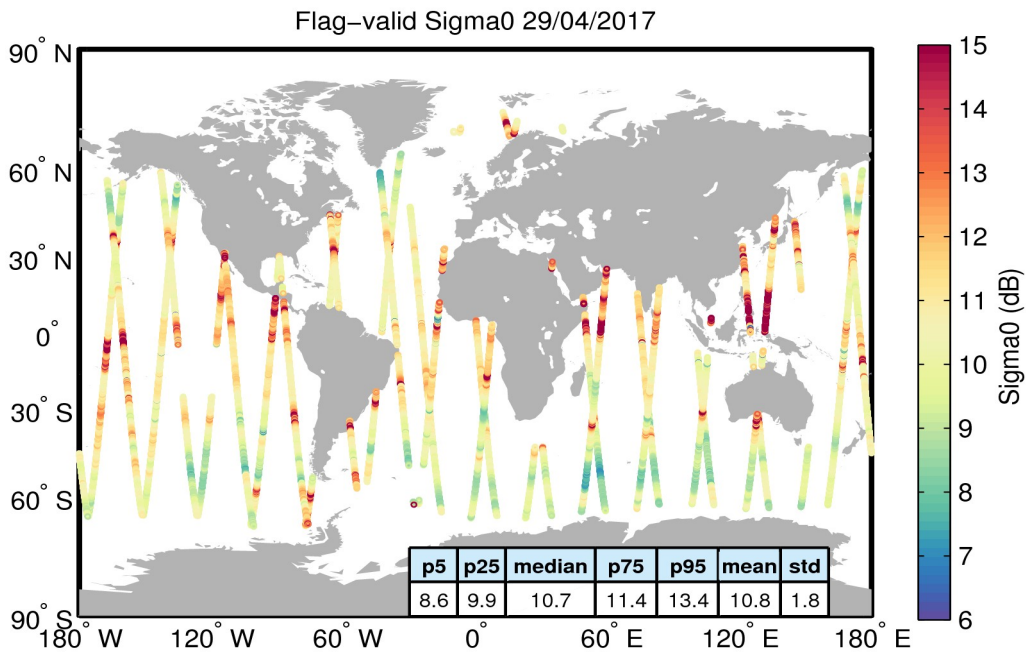
Figure 23. Geographical distribution of flag-valid sigma0 data over oceans and lakes for 29/04/2017. The statistical values shown in the table refer to the sigma0 in dB and are calculated over all measurements shown in the figure.
