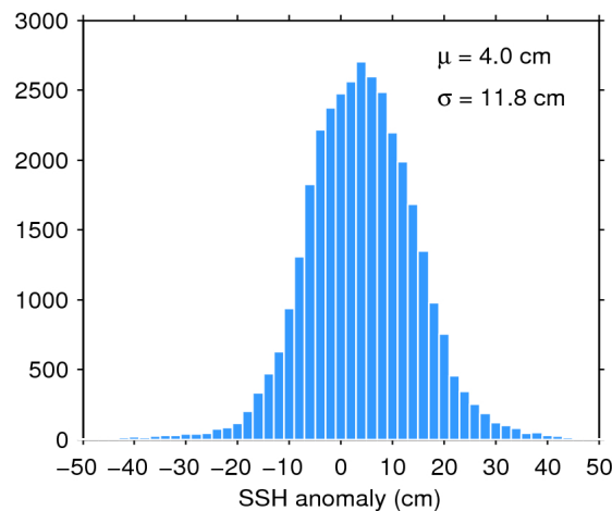
Figure 11. Histogram of science-valid SSH anomaly over oceans and lakes for 29/04/2017. The mean ( \mu ) and standard deviation ( \sigma ) are also shown. Note that values outside [-50 50] cm are excluded from the histogram for the sake of readability but not from the computation of \mu and \sigma .
