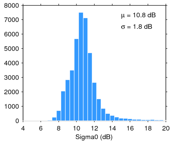
Figure 25. Histogram of flag-valid sigma0 over oceans and lakes for 29/04/2017. The mean ( \mu ) and standard deviation ( \sigma ) are also shown. Note that values outside [4 20] dB are excluded from the histogram for the sake of readability but not from the computation of \mu and \sigma .
