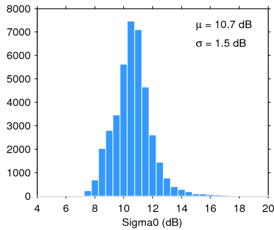
Figure 28. Histogram of science-valid sigma0 over oceans and lakes for 29/04/2017. The mean ( \mu ) and standard deviation ( \sigma ) are also shown. Note that values outside [4 20] dB are excluded from the histogram for the sake of readability but not from the computation of \mu and \sigma .
