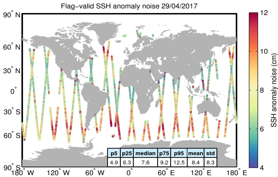
Figure 8. Geographical distribution of flag-valid 20-Hz SSH anomaly measurement noise over oceans and lakes for 29/04/2017. The statistical values shown in the table refer to the SSH anomaly noise and are calculated over all measurements shown in the figure.
