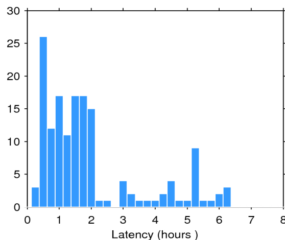
Figure 2. Histogram of the data latency for 29/04/2017. The y-axis denotes the number of files that are made available with a delay of x-hours with respect to the mean time of the records stored in the file.
