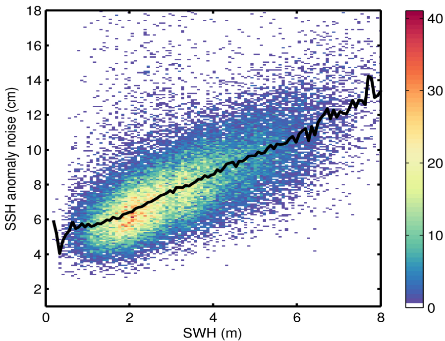
Figure 9. 2D histogram showing flag-valid SSH anomaly noise as a function of SWH for 29/04/2017. The black line denotes the median SSH anomaly noise as a function of SWH.
