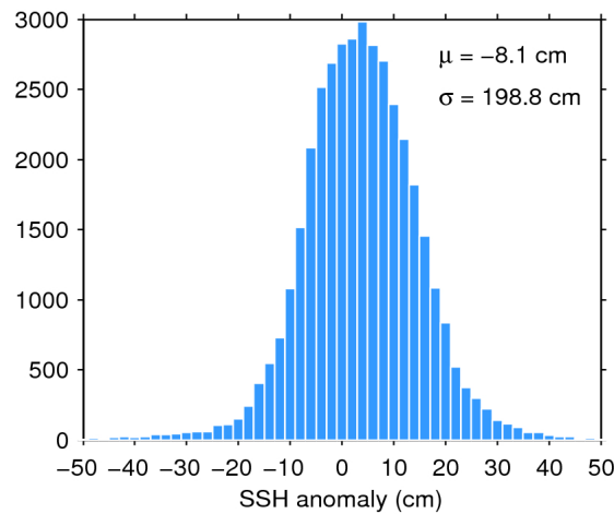
Figure 7. Histogram of flag-valid SSH anomaly over oceans and lakes for 29/04/2017. The mean ( \mu ) and standard deviation ( \sigma ) are also shown. Note that values outside [-50 50] cm are excluded from the histogram for the sake of readability but not from the computation of \mu and \sigma .
