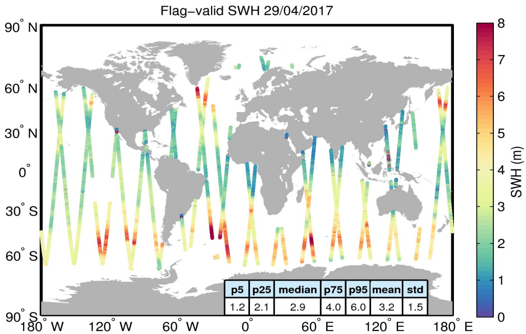
Figure 15. Geographical distribution of flag-valid SWH data over oceans and lakes for 29/04/2017. The statistical values shown in the table refer to the SWH in m and are calculated over all measurements shown in the figure.
