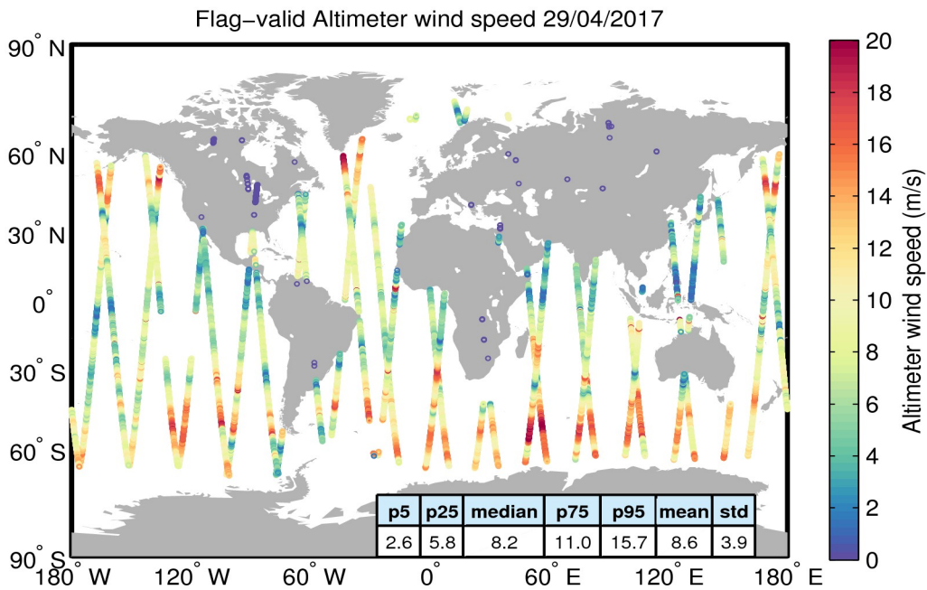
Figure 31. Geographical distribution of flag-valid wind data over oceans and lakes for 29/04/2017. The statistical values shown in the table refer to the wind in m/s and are calculated over all measurements shown in the figure.
