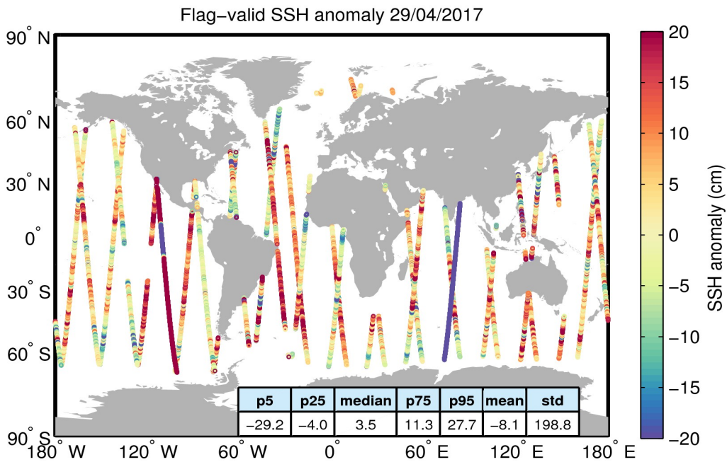
Figure 5. Geographical distribution of flag-valid 1-Hz SSH anomaly data over oceans and lakes for 29/04/2017. The statistical values shown in the table refer to the SSH anomaly in cm and are calculated over all measurements shown in the figure.
