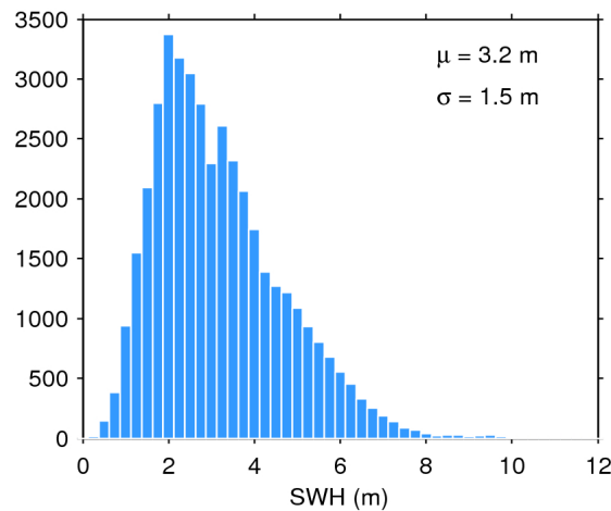
Figure 20. Histogram of science-valid SWH over oceans and lakes for 29/04/2017. The mean ( \mu ) and standard deviation ( \sigma ) are also shown. Note that values larger than 12 m are excluded from the histogram for the sake of readability but not from the computation of \mu and \sigma .
