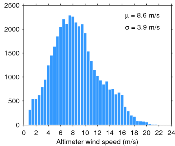
Figure 33. Histogram of flag-valid wind over oceans and lakes for 29/04/2017. The mean ( \mu ) and standard deviation ( \sigma ) are also shown. Note that values larger than 24 m/s are excluded from the histogram for the sake of readability but not from the computation of \mu and \sigma .
