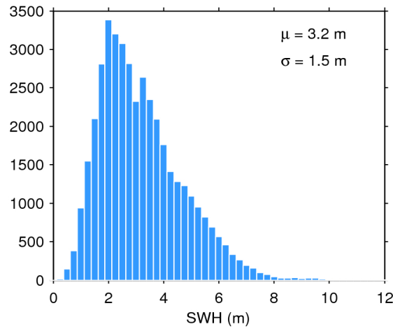
Figure 17. Histogram of flag-valid SWH over oceans and lakes for 29/04/2017. The mean ( \mu ) and standard deviation ( \sigma ) are also shown. Note that values larger than 12 m are excluded from the histogram for the sake of readability but not from the computation of \mu and \sigma .
