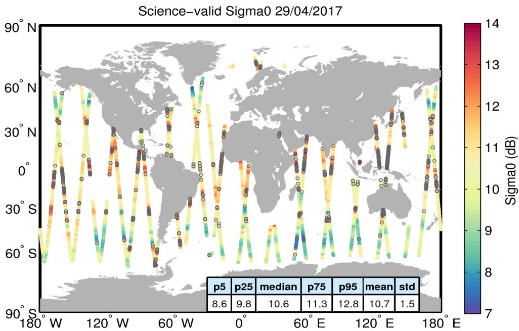
Figure 27. Geographical distribution of science-valid sigma0 data over oceans and lakes for 29/04/2017. The statistical values shown in the table refer to the sigma0 in dB and are calculated over all measurements shown in the figure. Gray circles denote records that have been rejected based on the editing criteria described in Table 4.
