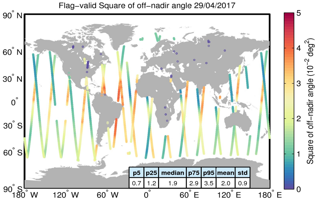
Figure 37. Geographical distribution of flag-valid mispointing data over oceans and lakes for 29/04/2017. The statistical values shown in the table refer to the mispointing in 10^{-2} deg 2 and are calculated over all measurements shown in the figure.
