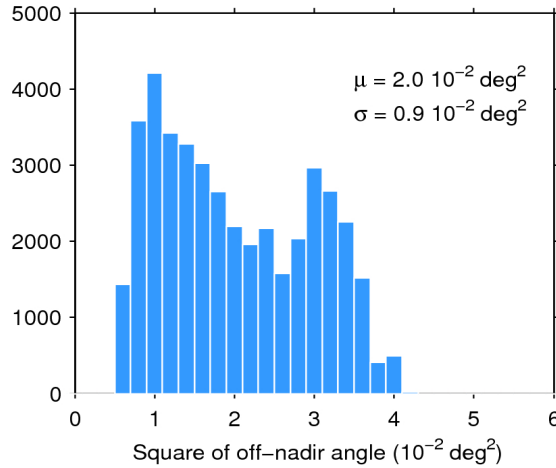
Figure 39. Histogram of flag-valid mispointing over oceans and lakes for 29/04/2017. The mean ( \mu ) and standard deviation ( \sigma ) are also shown. Note that values larger than 6 \cdot 10^{-2} \text{ deg}^2 are excluded from the histogram for the sake of readability but not from the computation of \mu and \sigma .
