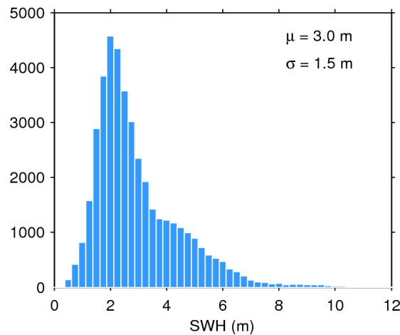
Figure 20. Histogram of science-valid SWH over oceans and lakes for 25/04/2017. The mean ( \mu ) and standard deviation ( \sigma ) are also shown. Note that values larger than 12 m are excluded from the histogram for the sake of readability but not from the computation of \mu and \sigma .
