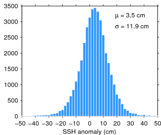
Figure 11. Histogram of science-valid SSH anomaly over oceans and lakes for 25/04/2017. The mean ( \mu ) and standard deviation ( \sigma ) are also shown. Note that values outside [-50 50] cm are excluded from the histogram for the sake of readability but not from the computation of \mu and \sigma .
