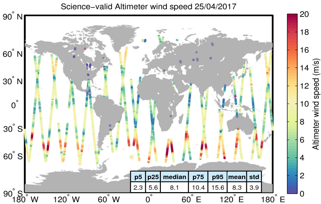
Figure 34. Geographical distribution of science-valid wind data over oceans and lakes for 25/04/2017. The statistical values shown in the table refer to the wind in m/s and are calculated over all measurements shown in the figure. Gray circles denote records that have been rejected based on the editing criteria described in Table 5.
