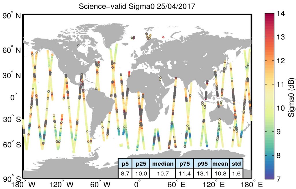
Figure 27. Geographical distribution of science-valid sigma0 data over oceans and lakes for 25/04/2017. The statistical values shown in the table refer to the sigma0 in dB and are calculated over all measurements shown in the figure. Gray circles denote records that have been rejected based on the editing criteria described in Table 4.
