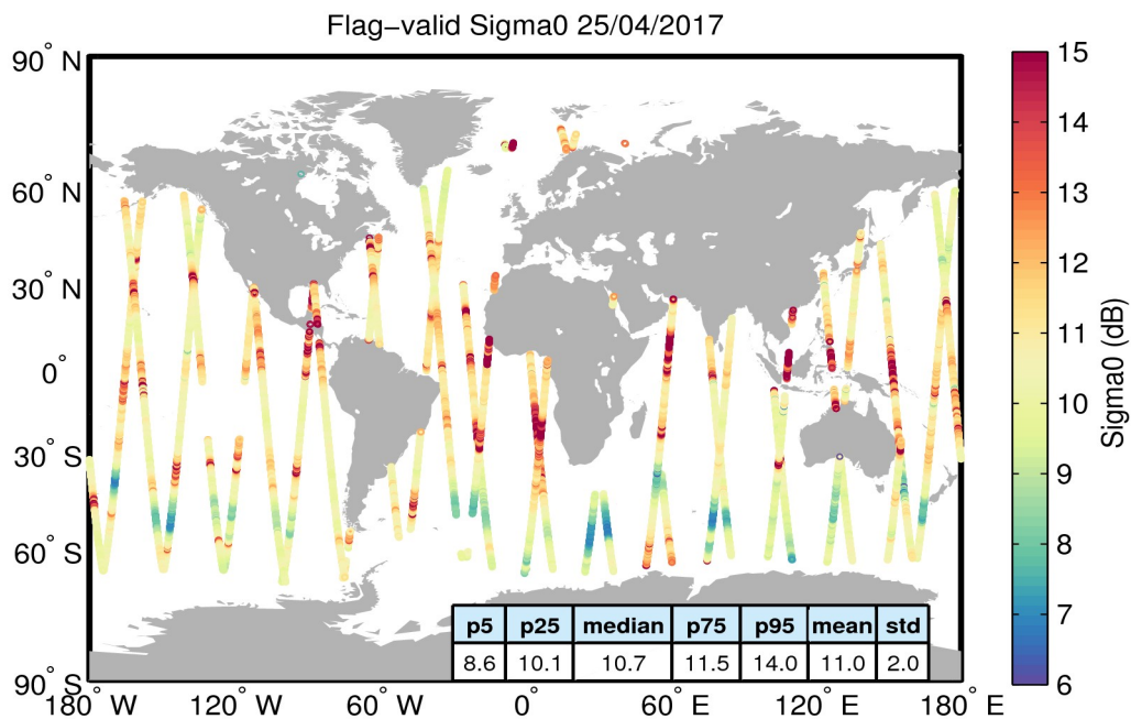
Figure 23. Geographical distribution of flag-valid sigma0 data over oceans and lakes for 25/04/2017. The statistical values shown in the table refer to the sigma0 in dB and are calculated over all measurements shown in the figure.
