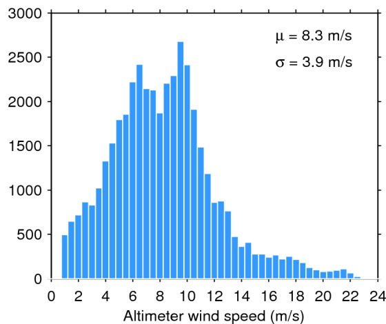
Figure 35. Histogram of science-valid wind over oceans and lakes for 25/04/2017. The mean ( \mu ) and standard deviation ( \sigma ) are also shown. Note that values larger than 24 m/s are excluded from the histogram for the sake of readability but not from the computation of \mu and \sigma .
