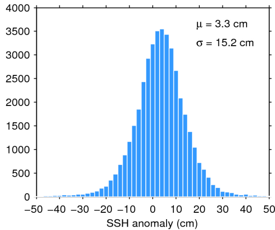
Figure 7. Histogram of flag-valid SSH anomaly over oceans and lakes for 25/04/2017. The mean ( \mu ) and standard deviation ( \sigma ) are also shown. Note that values outside [-50 50] cm are excluded from the histogram for the sake of readability but not from the computation of \mu and \sigma .
