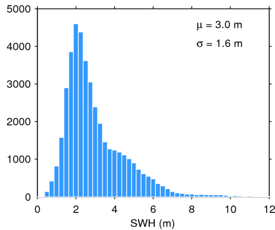
Figure 17. Histogram of flag-valid SWH over oceans and lakes for 25/04/2017. The mean ( \mu ) and standard deviation ( \sigma ) are also shown. Note that values larger than 12 m are excluded from the histogram for the sake of readability but not from the computation of \mu and \sigma .
