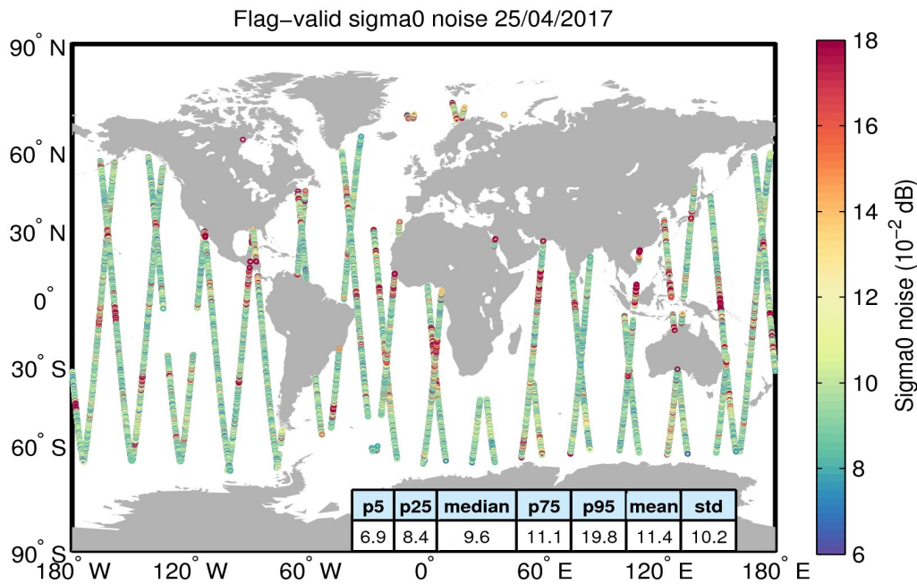
Figure 26. Geographical distribution of flag-valid 20-Hz sigma0 measurement noise over oceans and lakes for 25/04/2017. The statistical values shown in the table refer to the sigma0 noise and are calculated over all measurements shown in the figure.
