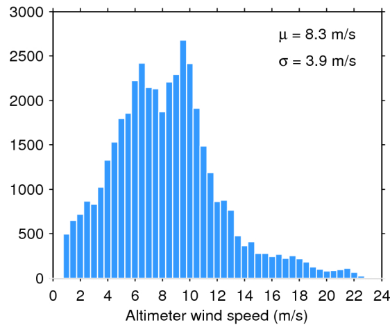
Figure 33. Histogram of flag-valid wind over oceans and lakes for 25/04/2017. The mean ( \mu ) and standard deviation ( \sigma ) are also shown. Note that values larger than 24 m/s are excluded from the histogram for the sake of readability but not from the computation of \mu and \sigma .
