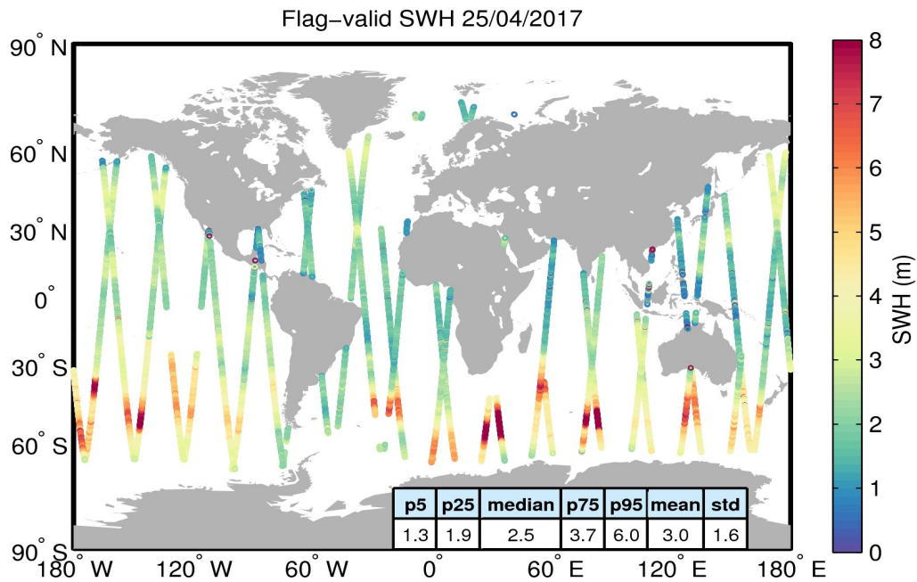
Figure 15. Geographical distribution of flag-valid SWH data over oceans and lakes for 25/04/2017. The statistical values shown in the table refer to the SWH in m and are calculated over all measurements shown in the figure.
