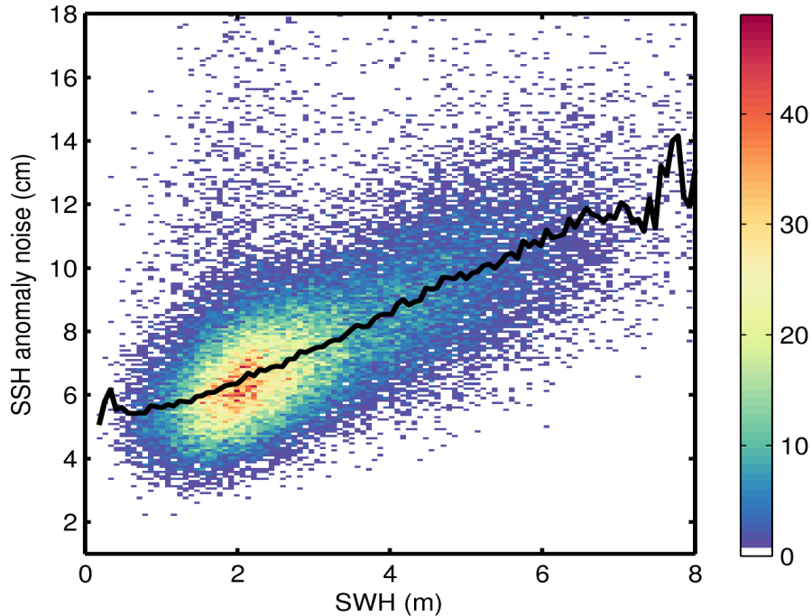
Figure 9. 2D histogram showing flag-valid SSH anomaly noise as a function of SWH for 25/04/2017. The black line denotes the median SSH anomaly noise as a function of SWH.
