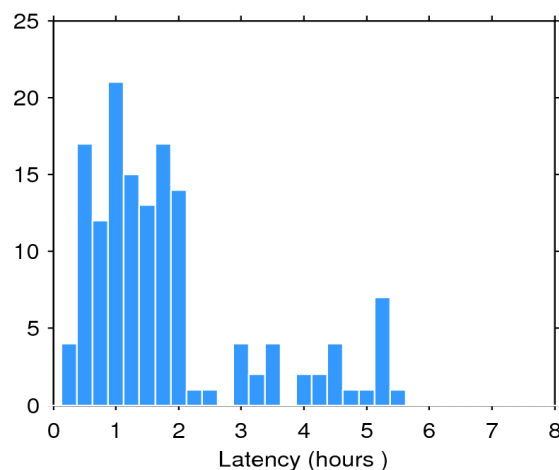
Figure 2. Histogram of the data latency for 25/04/2017. The y-axis denotes the number of files that are made available with a delay of x-hours with respect to the mean time of the records stored in the file.
