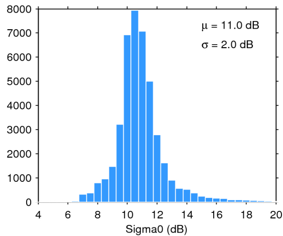
Figure 25. Histogram of flag-valid sigma0 over oceans and lakes for 25/04/2017. The mean ( \mu ) and standard deviation ( \sigma ) are also shown. Note that values outside [4 20] dB are excluded from the histogram for the sake of readability but not from the computation of \mu and \sigma .
