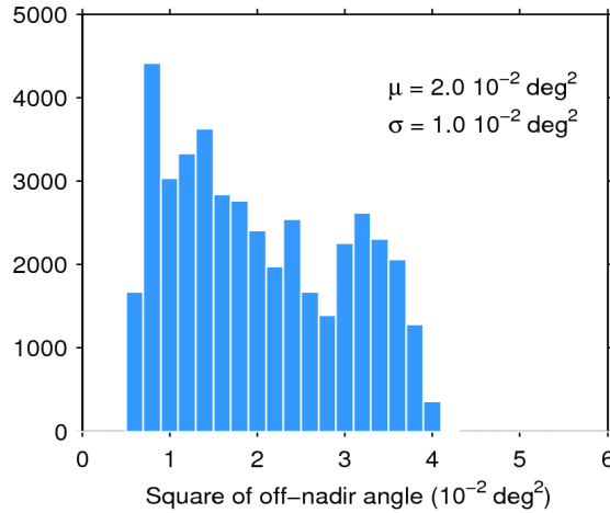
Figure 39. Histogram of flag-valid mispointing over oceans and lakes for 25/04/2017. The mean ( \mu ) and standard deviation ( \sigma ) are also shown. Note that values larger than 6 \cdot 10^{-2} \text{ deg}^2 are excluded from the histogram for the sake of readability but not from the computation of \mu and \sigma .
