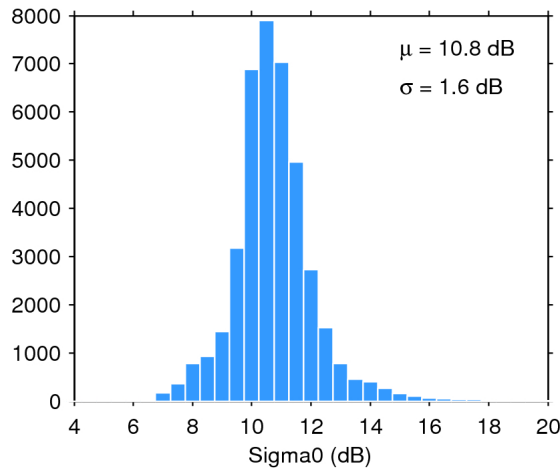
Figure 28. Histogram of science-valid sigma0 over oceans and lakes for 25/04/2017. The mean ( \mu ) and standard deviation ( \sigma ) are also shown. Note that values outside [4 20] dB are excluded from the histogram for the sake of readability but not from the computation of \mu and \sigma .
