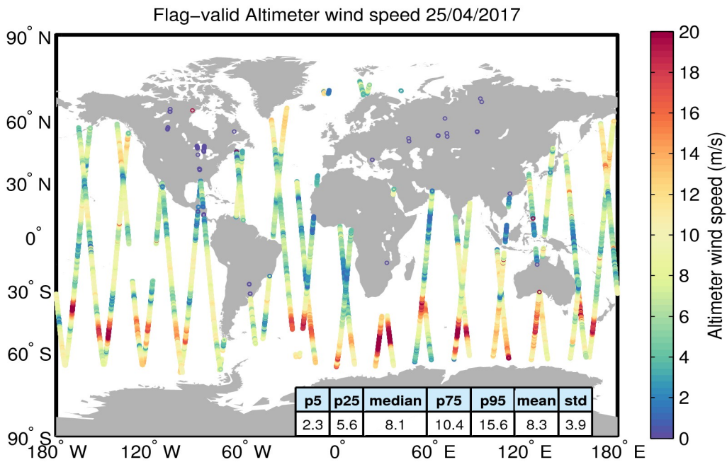
Figure 31. Geographical distribution of flag-valid wind data over oceans and lakes for 25/04/2017. The statistical values shown in the table refer to the wind in m/s and are calculated over all measurements shown in the figure.
