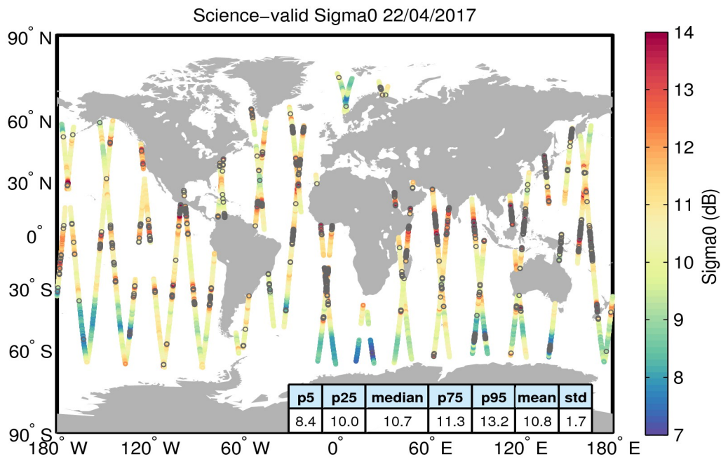
Figure 27. Geographical distribution of science-valid sigma0 data over oceans and lakes for 22/04/2017. The statistical values shown in the table refer to the sigma0 in dB and are calculated over all measurements shown in the figure. Gray circles denote records that have been rejected based on the editing criteria described in Table 4.
