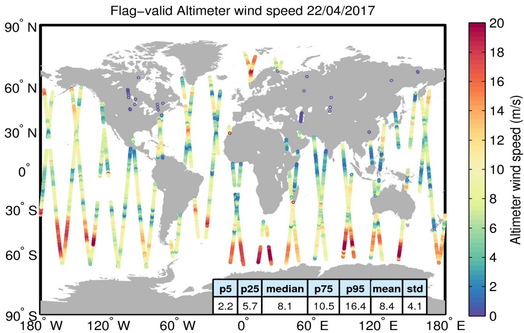
Figure 31. Geographical distribution of flag-valid wind data over oceans and lakes for 22/04/2017. The statistical values shown in the table refer to the wind in m/s and are calculated over all measurements shown in the figure.
