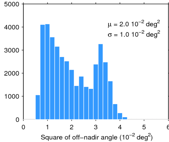
Figure 39. Histogram of flag-valid mispointing over oceans and lakes for 22/04/2017. The mean ( \mu ) and standard deviation ( \sigma ) are also shown. Note that values larger than 6 \cdot 10^{-2} \text{ deg}^2 are excluded from the histogram for the sake of readability but not from the computation of \mu and \sigma .
