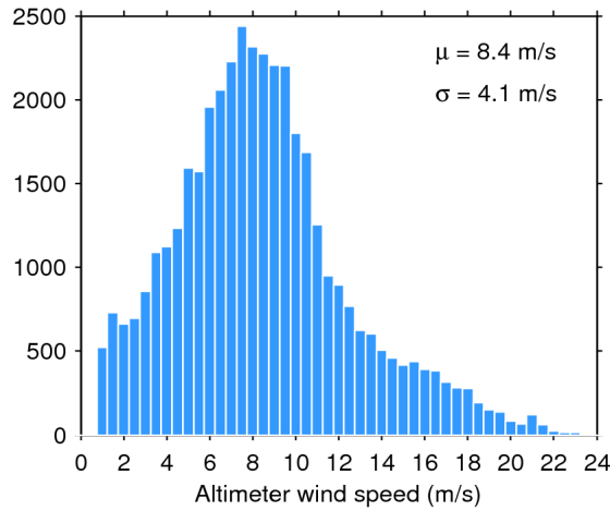
Figure 33. Histogram of flag-valid wind over oceans and lakes for 22/04/2017. The mean ( \mu ) and standard deviation ( \sigma ) are also shown. Note that values larger than 24 m/s are excluded from the histogram for the sake of readability but not from the computation of \mu and \sigma .
