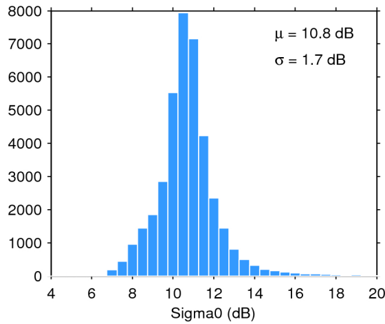
Figure 28. Histogram of science-valid sigma0 over oceans and lakes for 22/04/2017. The mean ( \mu ) and standard deviation ( \sigma ) are also shown. Note that values outside [4 20] dB are excluded from the histogram for the sake of readability but not from the computation of \mu and \sigma .
