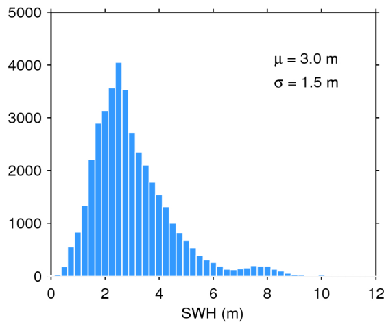
Figure 20. Histogram of science-valid SWH over oceans and lakes for 22/04/2017. The mean ( \mu ) and standard deviation ( \sigma ) are also shown. Note that values larger than 12 m are excluded from the histogram for the sake of readability but not from the computation of \mu and \sigma .
