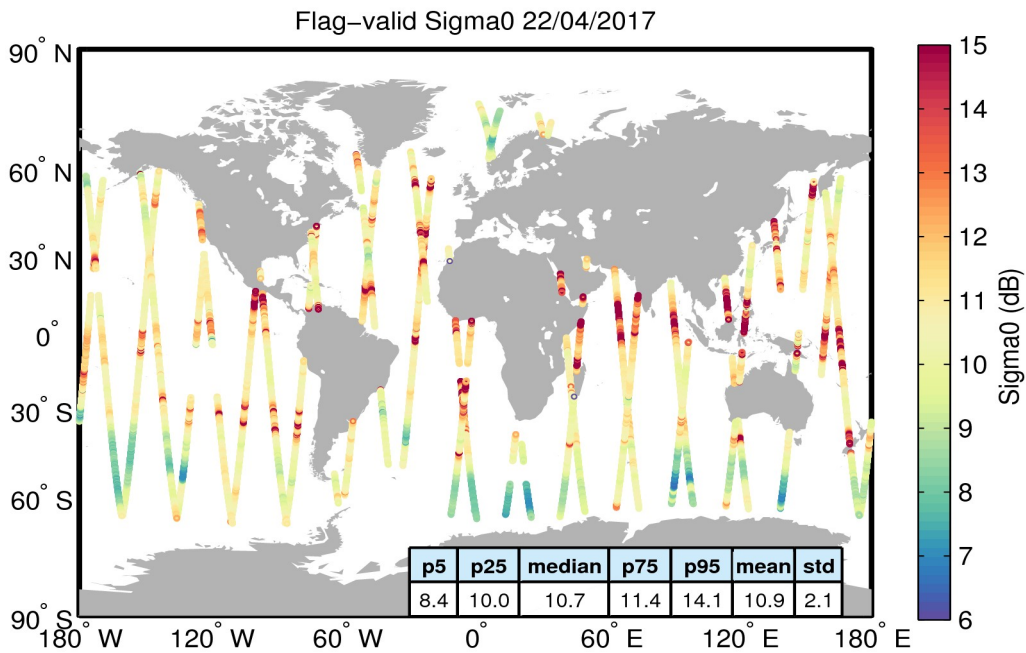
Figure 23. Geographical distribution of flag-valid sigma0 data over oceans and lakes for 22/04/2017. The statistical values shown in the table refer to the sigma0 in dB and are calculated over all measurements shown in the figure.
