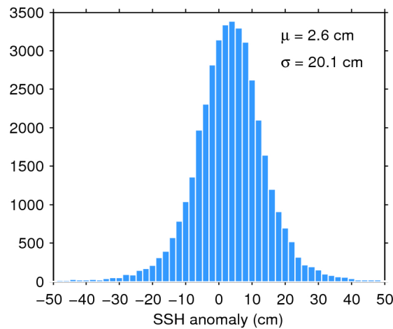
Figure 7. Histogram of flag-valid SSH anomaly over oceans and lakes for 22/04/2017. The mean ( \mu ) and standard deviation ( \sigma ) are also shown. Note that values outside [-50\ 50] cm are excluded from the histogram for the sake of readability but not from the computation of \mu and \sigma .
