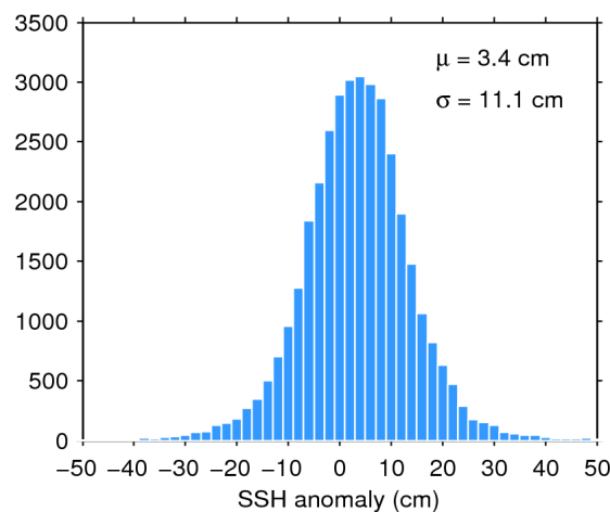
Figure 11. Histogram of science-valid SSH anomaly over oceans and lakes for 22/04/2017. The mean ( \mu ) and standard deviation ( \sigma ) are also shown. Note that values outside [-50 50] cm are excluded from the histogram for the sake of readability but not from the computation of \mu and \sigma .
