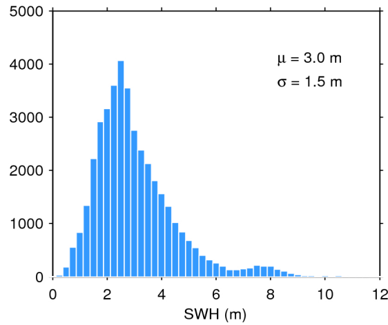
Figure 17. Histogram of flag-valid SWH over oceans and lakes for 22/04/2017. The mean ( \mu ) and standard deviation ( \sigma ) are also shown. Note that values larger than 12 m are excluded from the histogram for the sake of readability but not from the computation of \mu and \sigma .
