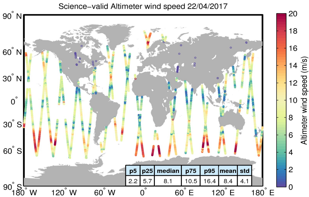
Figure 34. Geographical distribution of science-valid wind data over oceans and lakes for 22/04/2017. The statistical values shown in the table refer to the wind in m/s and are calculated over all measurements shown in the figure. Gray circles denote records that have been rejected based on the editing criteria described in Table 5.
