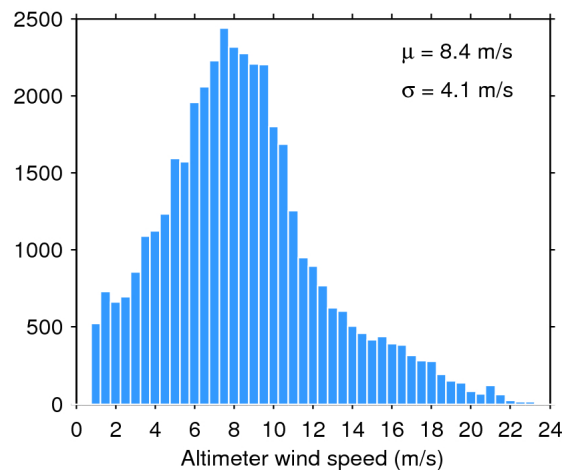
Figure 35. Histogram of science-valid wind over oceans and lakes for 22/04/2017. The mean ( \mu ) and standard deviation ( \sigma ) are also shown. Note that values larger than 24 m/s are excluded from the histogram for the sake of readability but not from the computation of \mu and \sigma .
