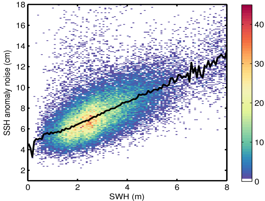
Figure 9. 2D histogram showing flag-valid SSH anomaly noise as a function of SWH for 22/04/2017. The black line denotes the median SSH anomaly noise as a function of SWH.
