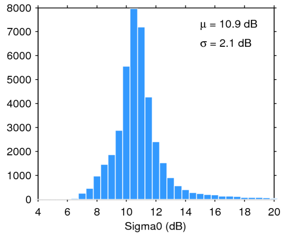
Figure 25. Histogram of flag-valid sigma0 over oceans and lakes for 22/04/2017. The mean ( \mu ) and standard deviation ( \sigma ) are also shown. Note that values outside [4 20] dB are excluded from the histogram for the sake of readability but not from the computation of \mu and \sigma .
