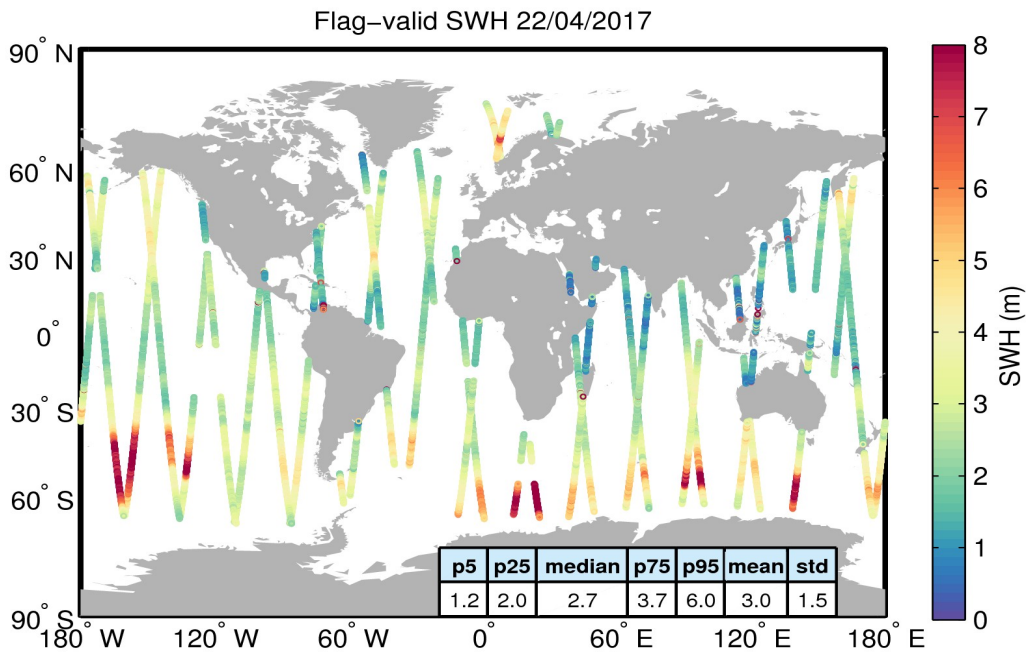
Figure 15. Geographical distribution of flag-valid SWH data over oceans and lakes for 22/04/2017. The statistical values shown in the table refer to the SWH in m and are calculated over all measurements shown in the figure.
