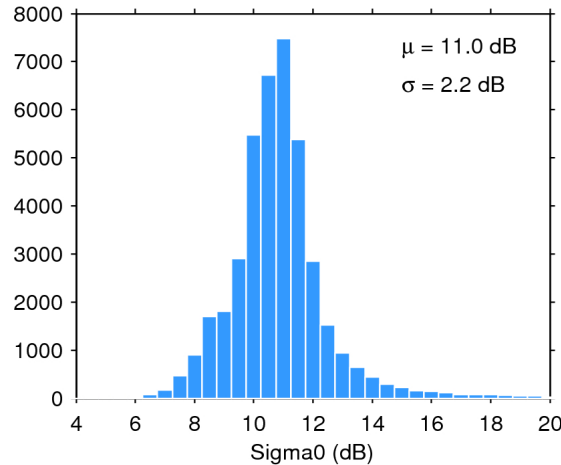
Figure 25. Histogram of flag-valid sigma0 over oceans and lakes for 21/04/2017. The mean ( \mu ) and standard deviation ( \sigma ) are also shown. Note that values outside [4 20] dB are excluded from the histogram for the sake of readability but not from the computation of \mu and \sigma .
