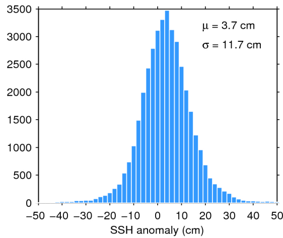
Figure 11. Histogram of science-valid SSH anomaly over oceans and lakes for 21/04/2017. The mean ( \mu ) and standard deviation ( \sigma ) are also shown. Note that values outside [-50 50] cm are excluded from the histogram for the sake of readability but not from the computation of \mu and \sigma .
