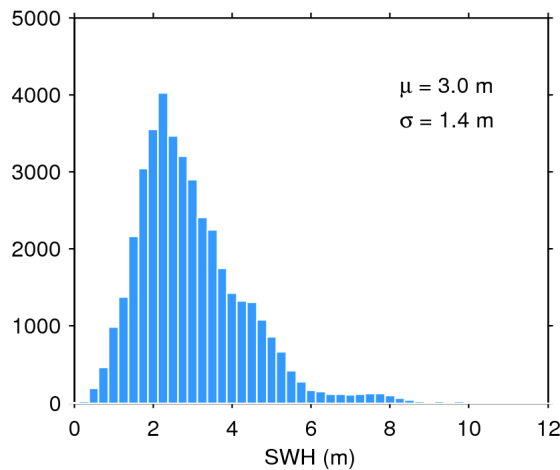
Figure 20. Histogram of science-valid SWH over oceans and lakes for 21/04/2017. The mean ( \mu ) and standard deviation ( \sigma ) are also shown. Note that values larger than 12 m are excluded from the histogram for the sake of readability but not from the computation of \mu and \sigma .
