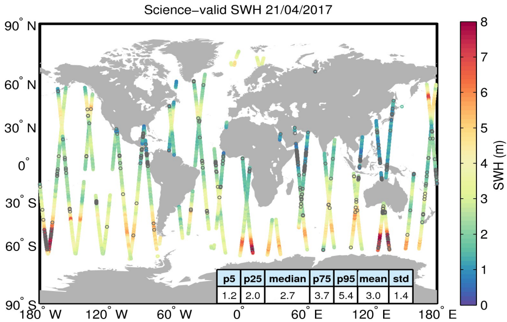
Figure 19. Geographical distribution of science-valid SWH data over oceans and lakes for 21/04/2017. The statistical values shown in the table refer to the SWH in m and are calculated over all measurements shown in the figure. Gray circles denote records that have been rejected based on the editing criteria described in Table 3.
