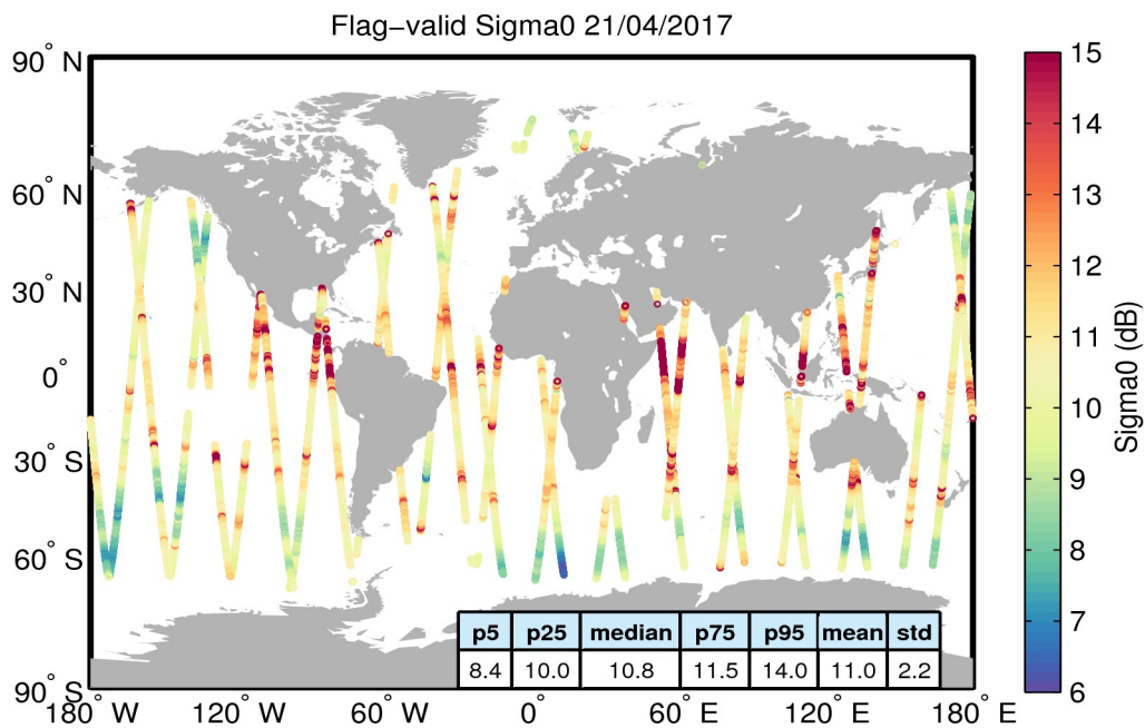
Figure 23. Geographical distribution of flag-valid sigma0 data over oceans and lakes for 21/04/2017. The statistical values shown in the table refer to the sigma0 in dB and are calculated over all measurements shown in the figure.
