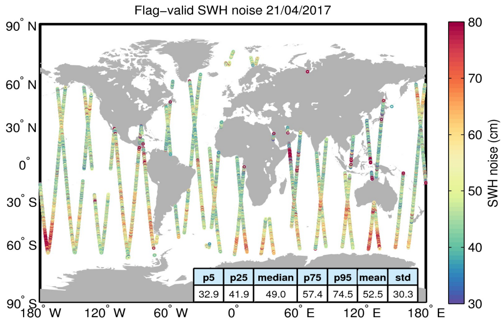
Figure 18. Geographical distribution of flag-valid 20-Hz SWH measurement noise over oceans and lakes for 21/04/2017. The statistical values shown in the table refer to the SWH noise and are calculated over all measurements shown in the figure.
