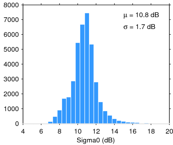
Figure 28. Histogram of science-valid sigma0 over oceans and lakes for 21/04/2017. The mean ( \mu ) and standard deviation ( \sigma ) are also shown. Note that values outside [4 20] dB are excluded from the histogram for the sake of readability but not from the computation of \mu and \sigma .
