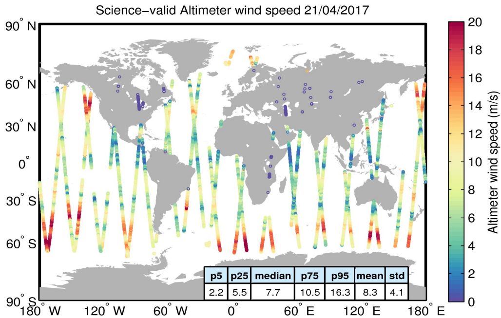
Figure 34. Geographical distribution of science-valid wind data over oceans and lakes for 21/04/2017. The statistical values shown in the table refer to the wind in m/s and are calculated over all measurements shown in the figure. Gray circles denote records that have been rejected based on the editing criteria described in Table 5.
