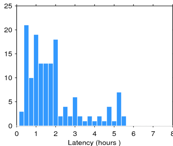
Figure 2. Histogram of the data latency for 21/04/2017. The y-axis denotes the number of files that are made available with a delay of x-hours with respect to the mean time of the records stored in the file.
