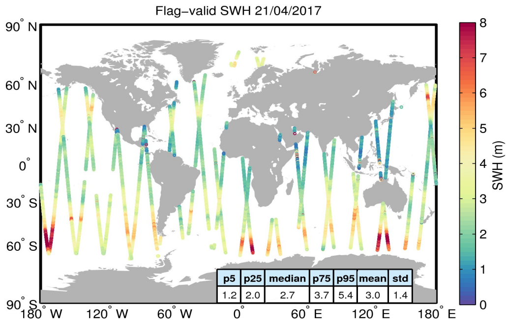
Figure 15. Geographical distribution of flag-valid SWH data over oceans and lakes for 21/04/2017. The statistical values shown in the table refer to the SWH in m and are calculated over all measurements shown in the figure.
