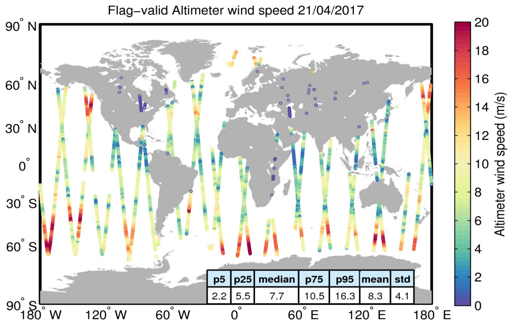
Figure 31. Geographical distribution of flag-valid wind data over oceans and lakes for 21/04/2017. The statistical values shown in the table refer to the wind in m/s and are calculated over all measurements shown in the figure.
