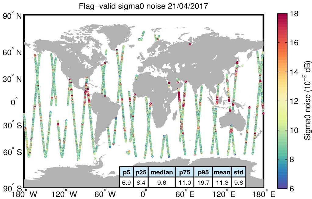
Figure 26. Geographical distribution of flag-valid 20-Hz sigma0 measurement noise over oceans and lakes for 21/04/2017. The statistical values shown in the table refer to the sigma0 noise and are calculated over all measurements shown in the figure.
