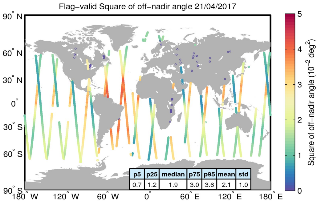
Figure 37. Geographical distribution of flag-valid mispointing data over oceans and lakes for 21/04/2017. The statistical values shown in the table refer to the mispointing in 10^{-2} deg 2 and are calculated over all measurements shown in the figure.
