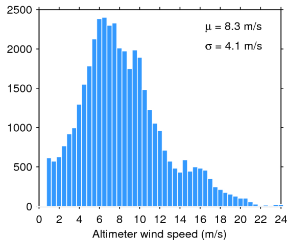
Figure 35. Histogram of science-valid wind over oceans and lakes for 21/04/2017. The mean ( \mu ) and standard deviation ( \sigma ) are also shown. Note that values larger than 24 m/s are excluded from the histogram for the sake of readability but not from the computation of \mu and \sigma .
