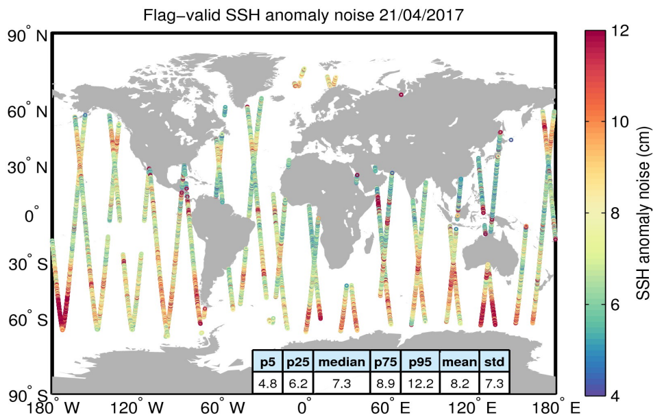
Figure 8. Geographical distribution of flag-valid 20-Hz SSH anomaly measurement noise over oceans and lakes for 21/04/2017. The statistical values shown in the table refer to the SSH anomaly noise and are calculated over all measurements shown in the figure.
