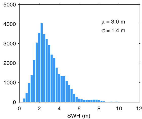
Figure 17. Histogram of flag-valid SWH over oceans and lakes for 21/04/2017. The mean ( \mu ) and standard deviation ( \sigma ) are also shown. Note that values larger than 12 m are excluded from the histogram for the sake of readability but not from the computation of \mu and \sigma .
