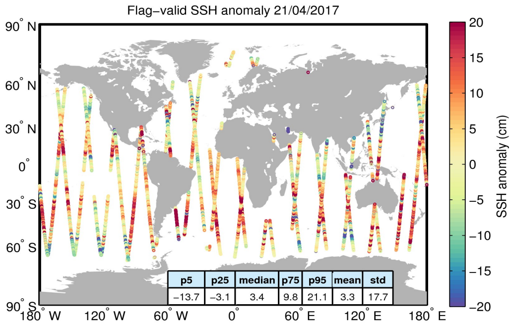
Figure 5. Geographical distribution of flag-valid 1-Hz SSH anomaly data over oceans and lakes for 21/04/2017. The statistical values shown in the table refer to the SSH anomaly in cm and are calculated over all measurements shown in the figure.
