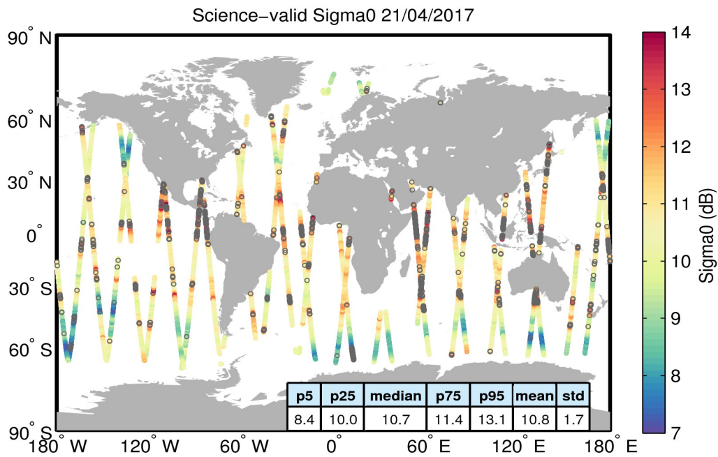
Figure 27. Geographical distribution of science-valid sigma0 data over oceans and lakes for 21/04/2017. The statistical values shown in the table refer to the sigma0 in dB and are calculated over all measurements shown in the figure. Gray circles denote records that have been rejected based on the editing criteria described in Table 4.
