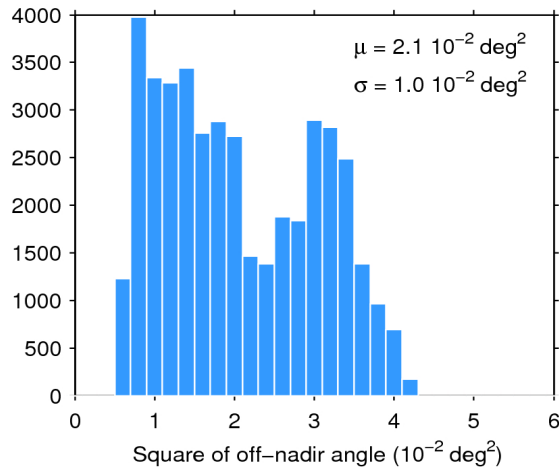
Figure 39. Histogram of flag-valid mispointing over oceans and lakes for 21/04/2017. The mean ( \mu ) and standard deviation ( \sigma ) are also shown. Note that values larger than 6 \cdot 10^{-2} \text{ deg}^2 are excluded from the histogram for the sake of readability but not from the computation of \mu and \sigma .
