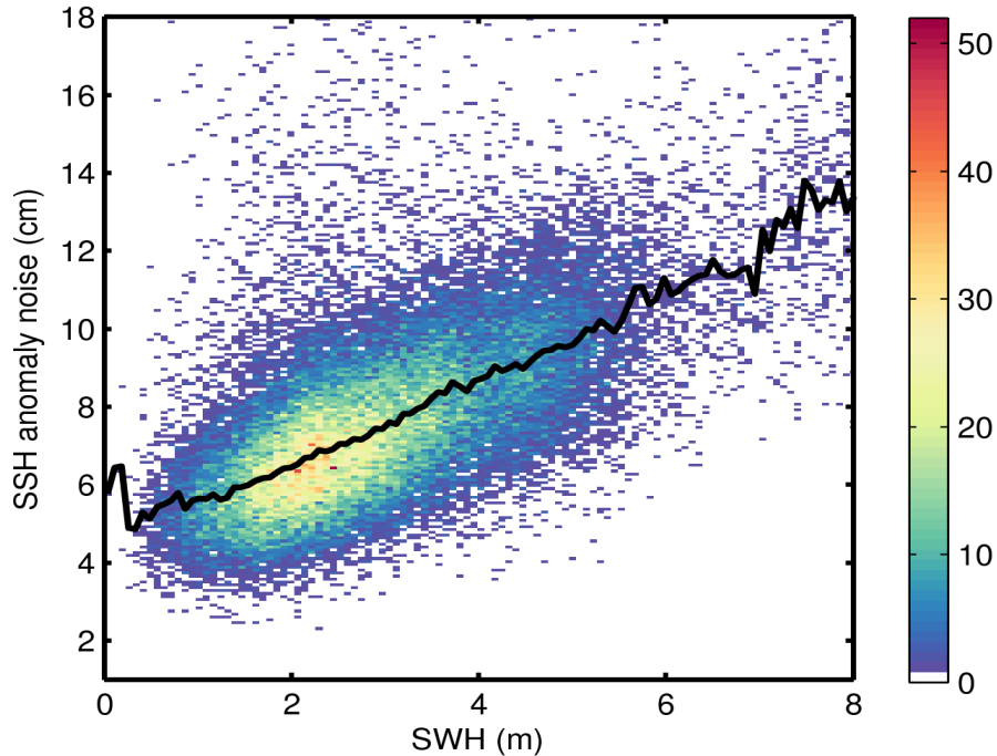
Figure 9. 2D histogram showing flag-valid SSH anomaly noise as a function of SWH for 21/04/2017. The black line denotes the median SSH anomaly noise as a function of SWH.
