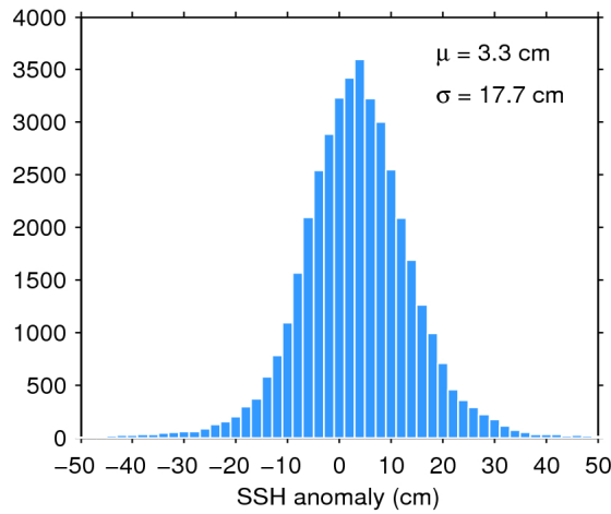
Figure 7. Histogram of flag-valid SSH anomaly over oceans and lakes for 21/04/2017. The mean ( \mu ) and standard deviation ( \sigma ) are also shown. Note that values outside [-50 50] cm are excluded from the histogram for the sake of readability but not from the computation of \mu and \sigma .
