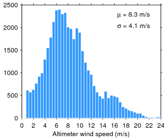
Figure 33. Histogram of flag-valid wind over oceans and lakes for 21/04/2017. The mean ( \mu ) and standard deviation ( \sigma ) are also shown. Note that values larger than 24 m/s are excluded from the histogram for the sake of readability but not from the computation of \mu and \sigma .
