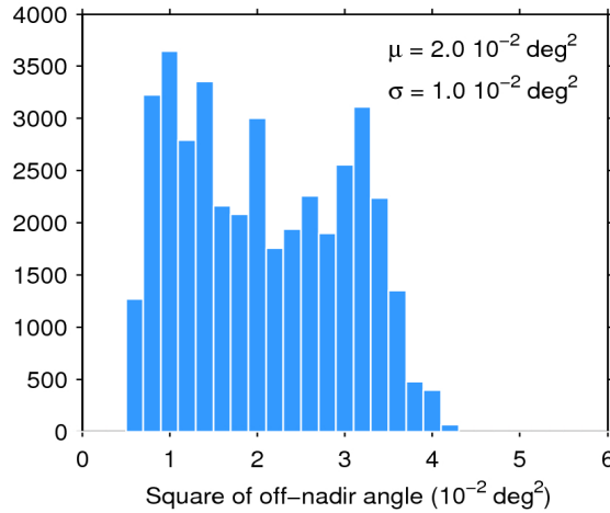
Figure 39. Histogram of flag-valid mispointing over oceans and lakes for 20/04/2017. The mean ( \mu ) and standard deviation ( \sigma ) are also shown. Note that values larger than 6 \cdot 10^{-2} \text{ deg}^2 are excluded from the histogram for the sake of readability but not from the computation of \mu and \sigma .
