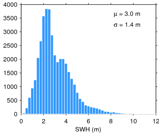
Figure 20. Histogram of science-valid SWH over oceans and lakes for 20/04/2017. The mean ( \mu ) and standard deviation ( \sigma ) are also shown. Note that values larger than 12 m are excluded from the histogram for the sake of readability but not from the computation of \mu and \sigma .
