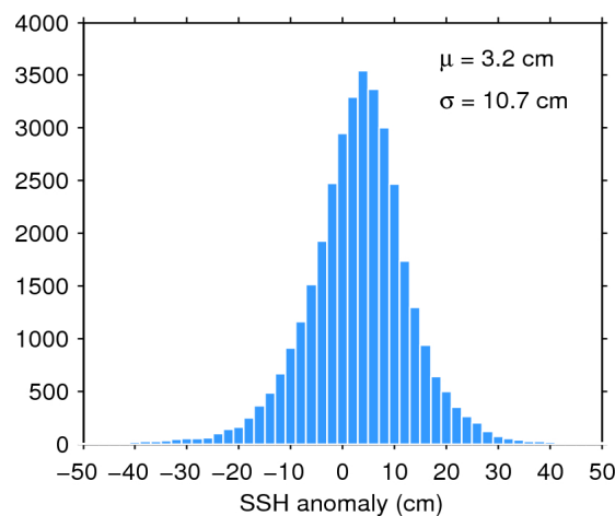
Figure 11. Histogram of science-valid SSH anomaly over oceans and lakes for 20/04/2017. The mean ( \mu ) and standard deviation ( \sigma ) are also shown. Note that values outside [-50 50] cm are excluded from the histogram for the sake of readability but not from the computation of \mu and \sigma .
