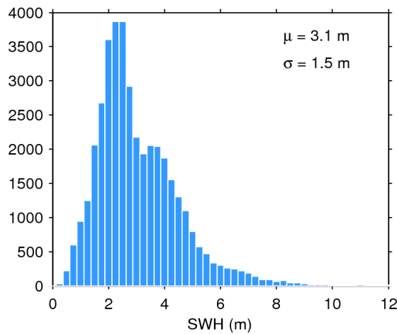
Figure 17. Histogram of flag-valid SWH over oceans and lakes for 20/04/2017. The mean ( \mu ) and standard deviation ( \sigma ) are also shown. Note that values larger than 12 m are excluded from the histogram for the sake of readability but not from the computation of \mu and \sigma .
