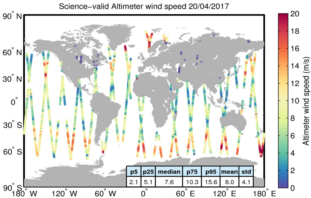
Figure 34. Geographical distribution of science-valid wind data over oceans and lakes for 20/04/2017. The statistical values shown in the table refer to the wind in m/s and are calculated over all measurements shown in the figure. Gray circles denote records that have been rejected based on the editing criteria described in Table 5.
