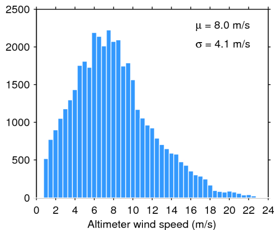
Figure 35. Histogram of science-valid wind over oceans and lakes for 20/04/2017. The mean ( \mu ) and standard deviation ( \sigma ) are also shown. Note that values larger than 24 m/s are excluded from the histogram for the sake of readability but not from the computation of \mu and \sigma .
