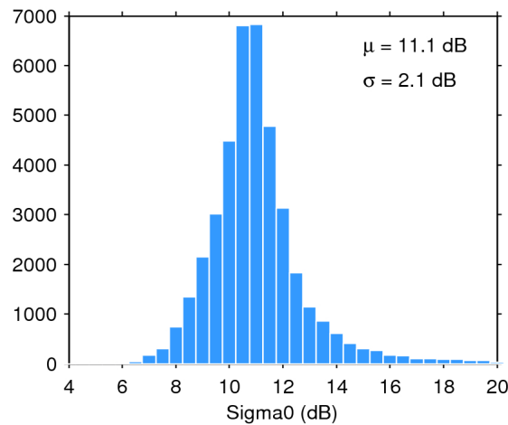
Figure 25. Histogram of flag-valid sigma0 over oceans and lakes for 20/04/2017. The mean ( \mu ) and standard deviation ( \sigma ) are also shown. Note that values outside [4 20] dB are excluded from the histogram for the sake of readability but not from the computation of \mu and \sigma .
