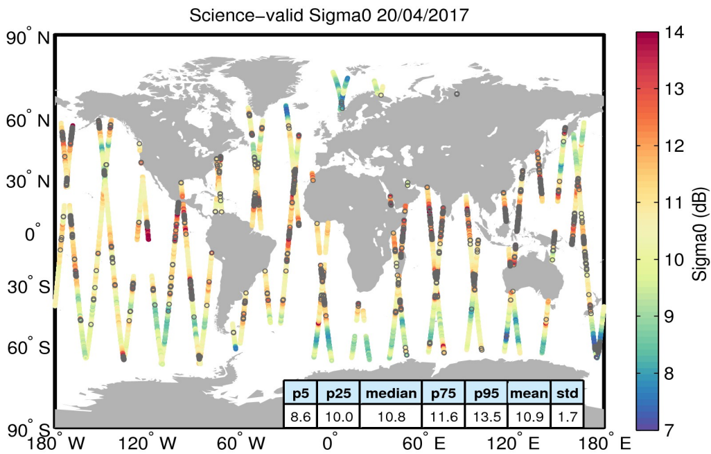
Figure 27. Geographical distribution of science-valid sigma0 data over oceans and lakes for 20/04/2017. The statistical values shown in the table refer to the sigma0 in dB and are calculated over all measurements shown in the figure. Gray circles denote records that have been rejected based on the editing criteria described in Table 4.
