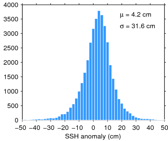
Figure 7. Histogram of flag-valid SSH anomaly over oceans and lakes for 20/04/2017. The mean ( \mu ) and standard deviation ( \sigma ) are also shown. Note that values outside [-50 50] cm are excluded from the histogram for the sake of readability but not from the computation of \mu and \sigma .
