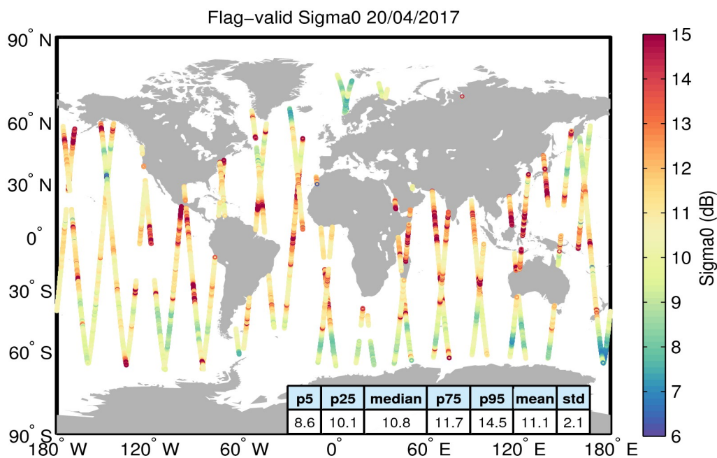
Figure 23. Geographical distribution of flag-valid sigma0 data over oceans and lakes for 20/04/2017. The statistical values shown in the table refer to the sigma0 in dB and are calculated over all measurements shown in the figure.
