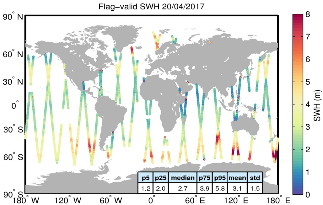
Figure 15. Geographical distribution of flag-valid SWH data over oceans and lakes for 20/04/2017. The statistical values shown in the table refer to the SWH in m and are calculated over all measurements shown in the figure.
