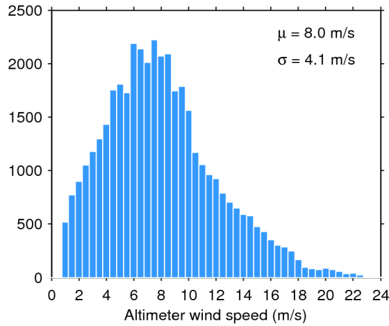
Figure 33. Histogram of flag-valid wind over oceans and lakes for 20/04/2017. The mean ( \mu ) and standard deviation ( \sigma ) are also shown. Note that values larger than 24 m/s are excluded from the histogram for the sake of readability but not from the computation of \mu and \sigma .
