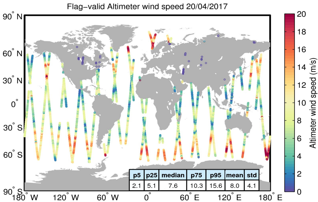
Figure 31. Geographical distribution of flag-valid wind data over oceans and lakes for 20/04/2017. The statistical values shown in the table refer to the wind in m/s and are calculated over all measurements shown in the figure.
