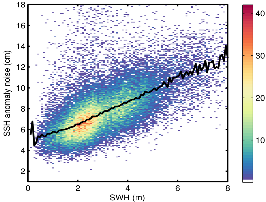
Figure 9. 2D histogram showing flag-valid SSH anomaly noise as a function of SWH for 20/04/2017. The black line denotes the median SSH anomaly noise as a function of SWH.
