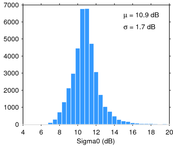
Figure 28. Histogram of science-valid sigma0 over oceans and lakes for 20/04/2017. The mean ( \mu ) and standard deviation ( \sigma ) are also shown. Note that values outside [4 20] dB are excluded from the histogram for the sake of readability but not from the computation of \mu and \sigma .
