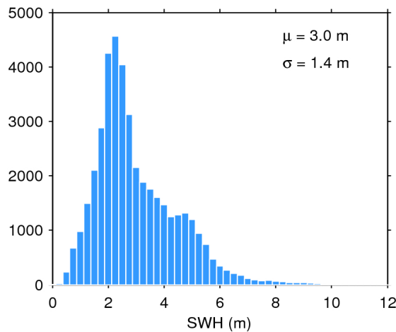
Figure 20. Histogram of science-valid SWH over oceans and lakes for 19/04/2017. The mean ( \mu ) and standard deviation ( \sigma ) are also shown. Note that values larger than 12 m are excluded from the histogram for the sake of readability but not from the computation of \mu and \sigma .
