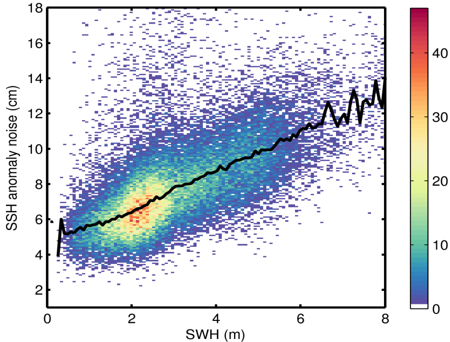
Figure 9. 2D histogram showing flag-valid SSH anomaly noise as a function of SWH for 19/04/2017. The black line denotes the median SSH anomaly noise as a function of SWH.
