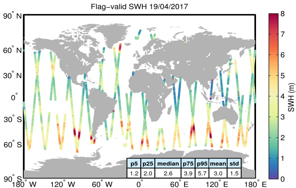
Figure 15. Geographical distribution of flag-valid SWH data over oceans and lakes for 19/04/2017. The statistical values shown in the table refer to the SWH in m and are calculated over all measurements shown in the figure.
