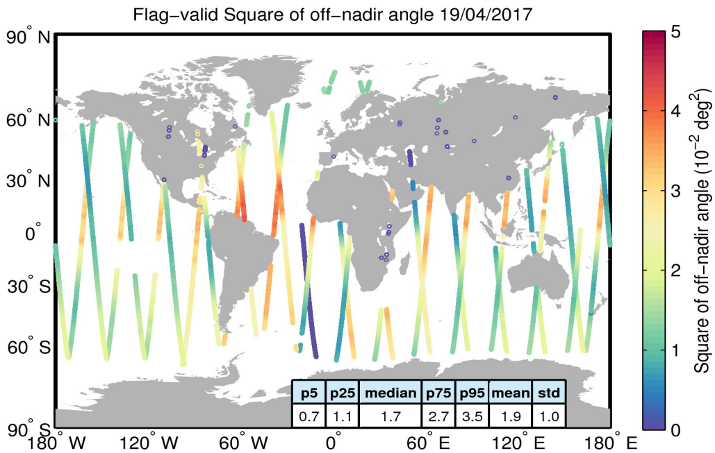
Figure 37. Geographical distribution of flag-valid mispointing data over oceans and lakes for 19/04/2017. The statistical values shown in the table refer to the mispointing in 10^{-2} deg 2 and are calculated over all measurements shown in the figure.
