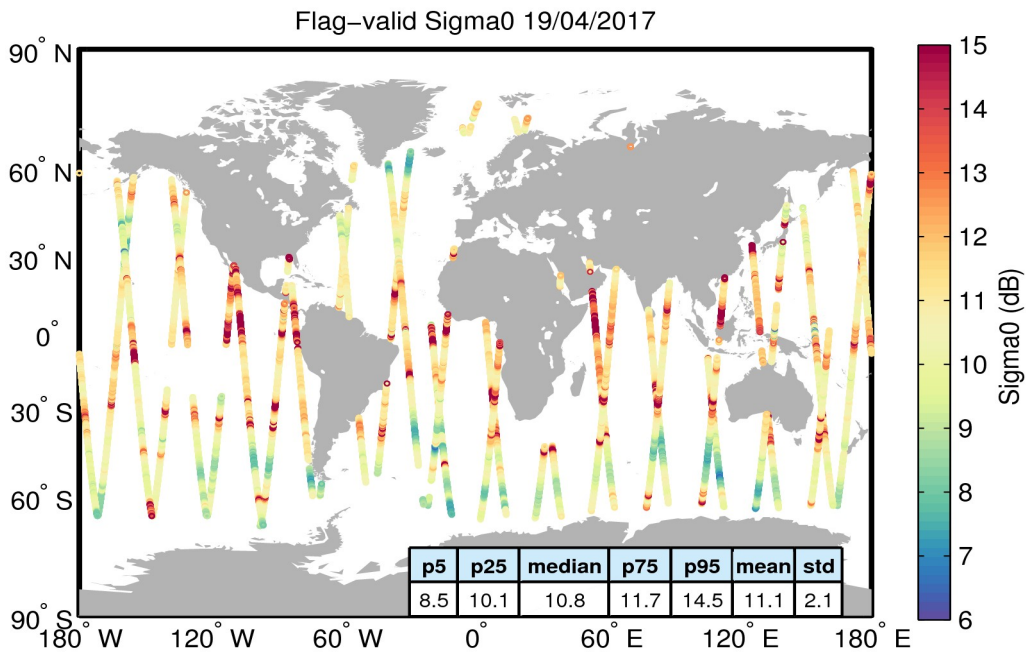
Figure 23. Geographical distribution of flag-valid sigma0 data over oceans and lakes for 19/04/2017. The statistical values shown in the table refer to the sigma0 in dB and are calculated over all measurements shown in the figure.
