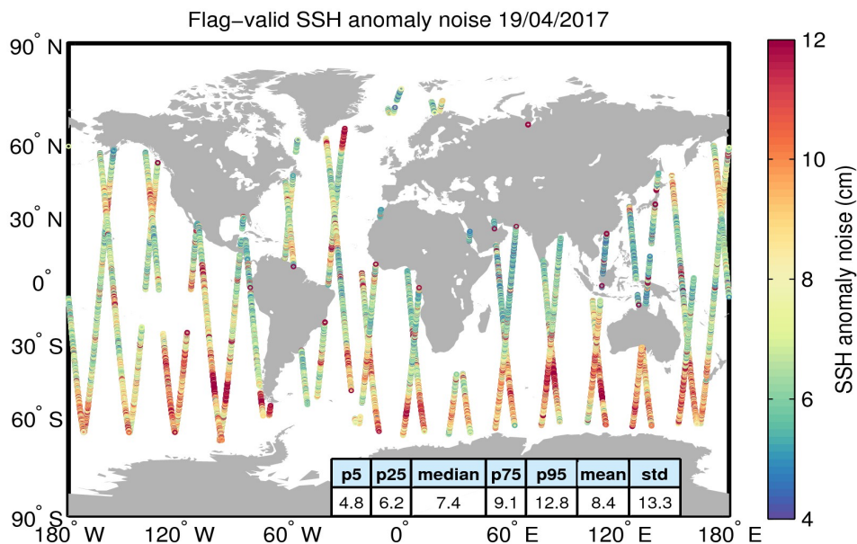
Figure 8. Geographical distribution of flag-valid 20-Hz SSH anomaly measurement noise over oceans and lakes for 19/04/2017. The statistical values shown in the table refer to the SSH anomaly noise and are calculated over all measurements shown in the figure.
