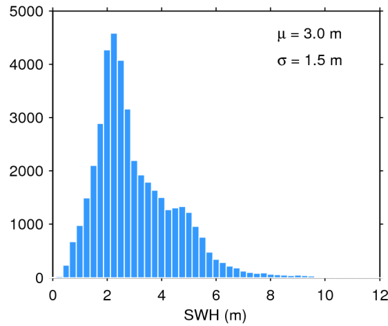
Figure 17. Histogram of flag-valid SWH over oceans and lakes for 19/04/2017. The mean ( \mu ) and standard deviation ( \sigma ) are also shown. Note that values larger than 12 m are excluded from the histogram for the sake of readability but not from the computation of \mu and \sigma .
