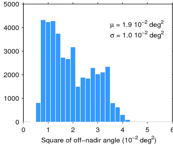
Figure 39. Histogram of flag-valid mispointing over oceans and lakes for 19/04/2017. The mean ( \mu ) and standard deviation ( \sigma ) are also shown. Note that values larger than 6 \cdot 10^{-2} \text{ deg}^2 are excluded from the histogram for the sake of readability but not from the computation of \mu and \sigma .
