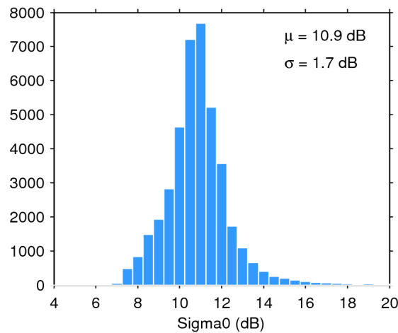
Figure 28. Histogram of science-valid sigma0 over oceans and lakes for 19/04/2017. The mean ( \mu ) and standard deviation ( \sigma ) are also shown. Note that values outside [4 20] dB are excluded from the histogram for the sake of readability but not from the computation of \mu and \sigma .
