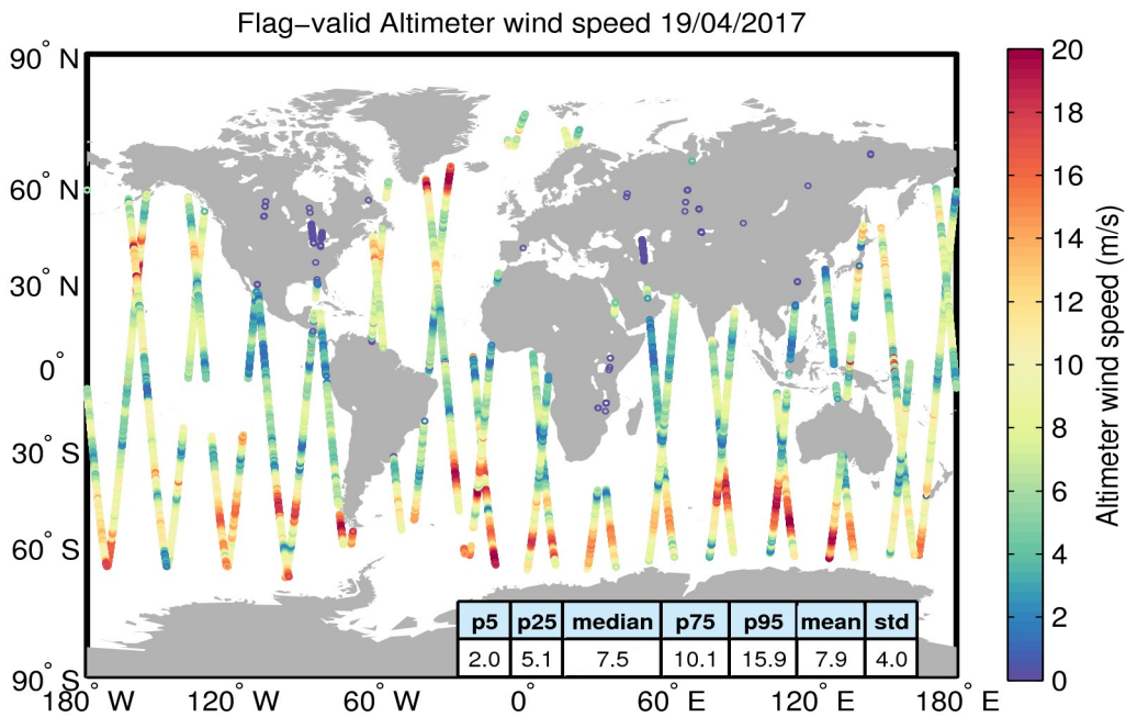
Figure 31. Geographical distribution of flag-valid wind data over oceans and lakes for 19/04/2017. The statistical values shown in the table refer to the wind in m/s and are calculated over all measurements shown in the figure.
