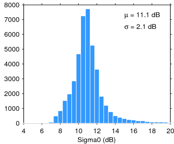
Figure 25. Histogram of flag-valid sigma0 over oceans and lakes for 19/04/2017. The mean ( \mu ) and standard deviation ( \sigma ) are also shown. Note that values outside [4 20] dB are excluded from the histogram for the sake of readability but not from the computation of \mu and \sigma .
