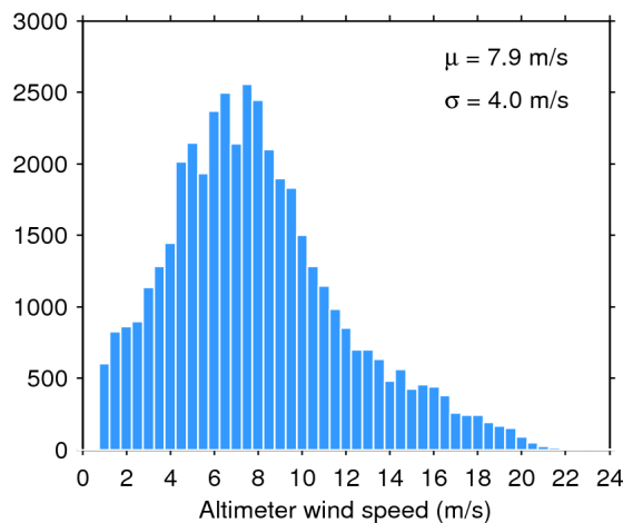
Figure 35. Histogram of science-valid wind over oceans and lakes for 19/04/2017. The mean ( \mu ) and standard deviation ( \sigma ) are also shown. Note that values larger than 24 m/s are excluded from the histogram for the sake of readability but not from the computation of \mu and \sigma .
