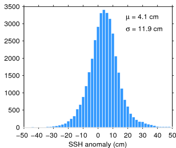
Figure 11. Histogram of science-valid SSH anomaly over oceans and lakes for 19/04/2017. The mean ( \mu ) and standard deviation ( \sigma ) are also shown. Note that values outside [-50 50] cm are excluded from the histogram for the sake of readability but not from the computation of \mu and \sigma .
