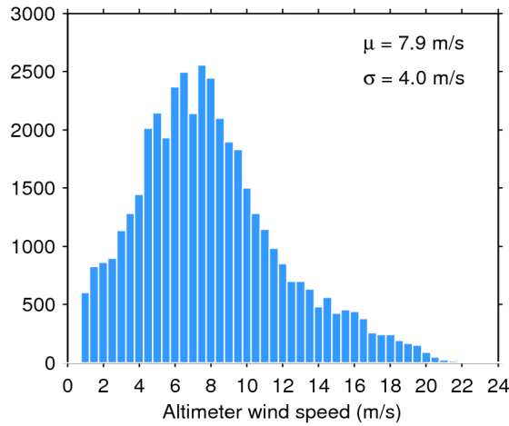
Figure 33. Histogram of flag-valid wind over oceans and lakes for 19/04/2017. The mean ( \mu ) and standard deviation ( \sigma ) are also shown. Note that values larger than 24 m/s are excluded from the histogram for the sake of readability but not from the computation of \mu and \sigma .
