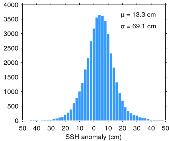
Figure 7. Histogram of flag-valid SSH anomaly over oceans and lakes for 19/04/2017. The mean ( \mu ) and standard deviation ( \sigma ) are also shown. Note that values outside [-50\ 50] cm are excluded from the histogram for the sake of readability but not from the computation of \mu and \sigma .
