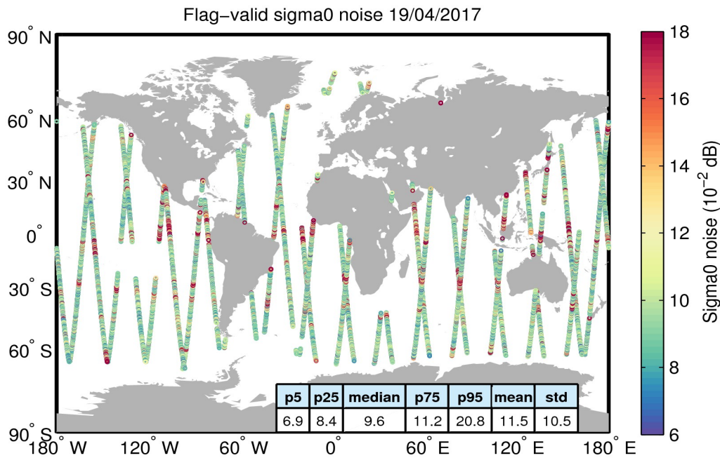
Figure 26. Geographical distribution of flag-valid 20-Hz sigma0 measurement noise over oceans and lakes for 19/04/2017. The statistical values shown in the table refer to the sigma0 noise and are calculated over all measurements shown in the figure.
