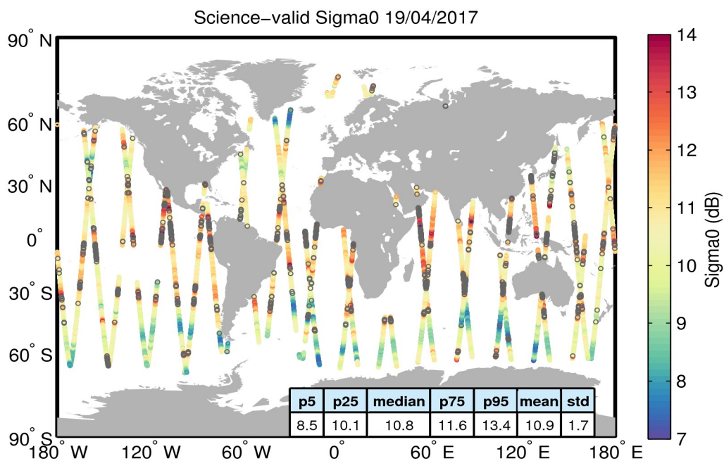
Figure 27. Geographical distribution of science-valid sigma0 data over oceans and lakes for 19/04/2017. The statistical values shown in the table refer to the sigma0 in dB and are calculated over all measurements shown in the figure. Gray circles denote records that have been rejected based on the editing criteria described in Table 4.
