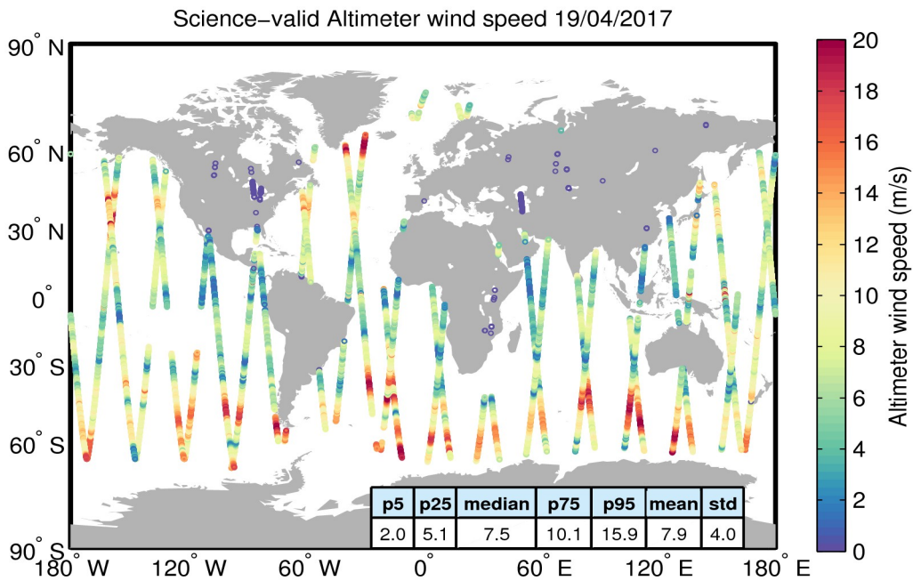
Figure 34. Geographical distribution of science-valid wind data over oceans and lakes for 19/04/2017. The statistical values shown in the table refer to the wind in m/s and are calculated over all measurements shown in the figure. Gray circles denote records that have been rejected based on the editing criteria described in Table 5.
