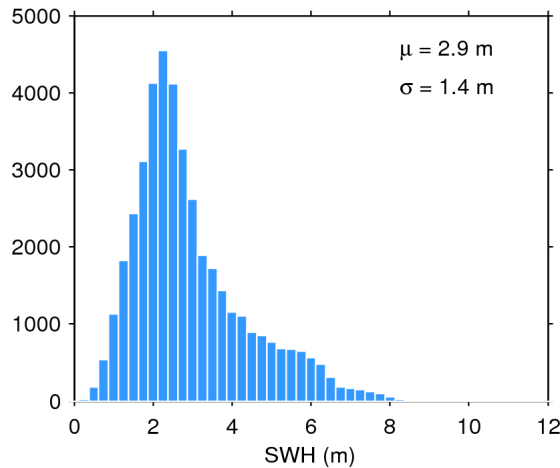
Figure 20. Histogram of science-valid SWH over oceans and lakes for 17/04/2017. The mean ( \mu ) and standard deviation ( \sigma ) are also shown. Note that values larger than 12 m are excluded from the histogram for the sake of readability but not from the computation of \mu and \sigma .
