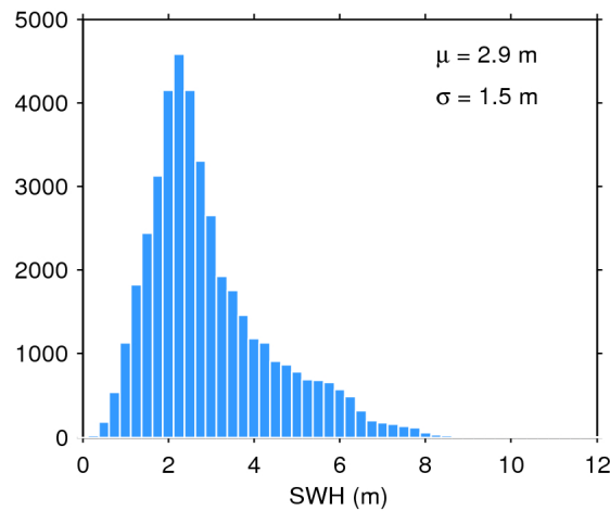
Figure 17. Histogram of flag-valid SWH over oceans and lakes for 17/04/2017. The mean ( \mu ) and standard deviation ( \sigma ) are also shown. Note that values larger than 12 m are excluded from the histogram for the sake of readability but not from the computation of \mu and \sigma .
