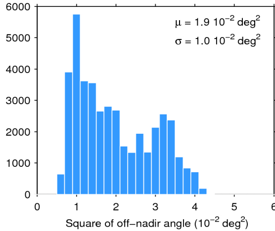
Figure 39. Histogram of flag-valid mispointing over oceans and lakes for 17/04/2017. The mean ( \mu ) and standard deviation ( \sigma ) are also shown. Note that values larger than 6 \cdot 10^{-2} \text{ deg}^2 are excluded from the histogram for the sake of readability but not from the computation of \mu and \sigma .
