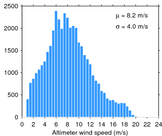
Figure 35. Histogram of science-valid wind over oceans and lakes for 17/04/2017. The mean ( \mu ) and standard deviation ( \sigma ) are also shown. Note that values larger than 24 m/s are excluded from the histogram for the sake of readability but not from the computation of \mu and \sigma .
