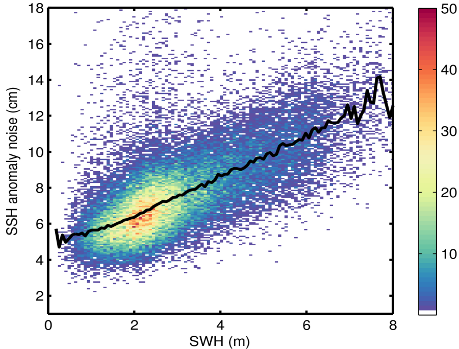
Figure 9. 2D histogram showing flag-valid SSH anomaly noise as a function of SWH for 17/04/2017. The black line denotes the median SSH anomaly noise as a function of SWH.
