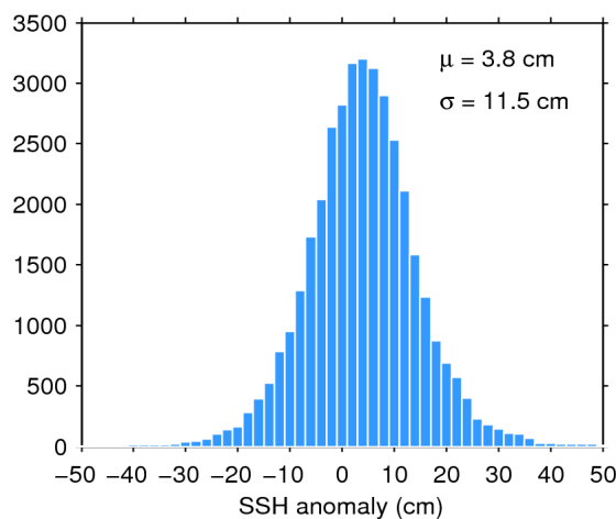
Figure 11. Histogram of science-valid SSH anomaly over oceans and lakes for 17/04/2017. The mean ( \mu ) and standard deviation ( \sigma ) are also shown. Note that values outside [-50 50] cm are excluded from the histogram for the sake of readability but not from the computation of \mu and \sigma .
