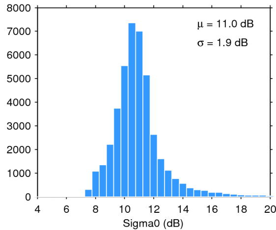
Figure 25. Histogram of flag-valid sigma0 over oceans and lakes for 17/04/2017. The mean ( \mu ) and standard deviation ( \sigma ) are also shown. Note that values outside [4 20] dB are excluded from the histogram for the sake of readability but not from the computation of \mu and \sigma .
