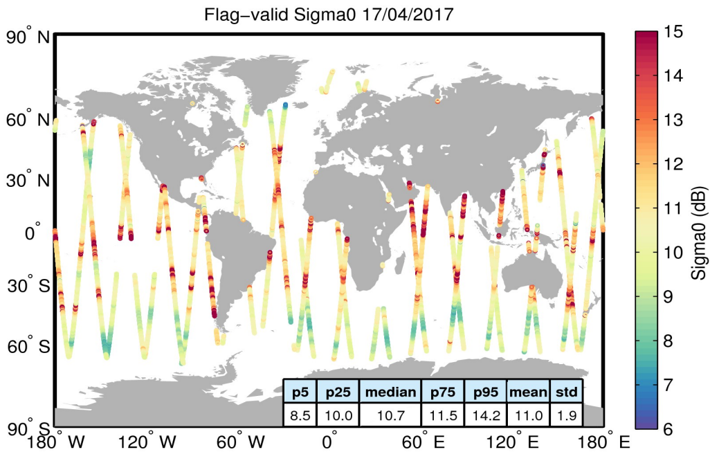
Figure 23. Geographical distribution of flag-valid sigma0 data over oceans and lakes for 17/04/2017. The statistical values shown in the table refer to the sigma0 in dB and are calculated over all measurements shown in the figure.
