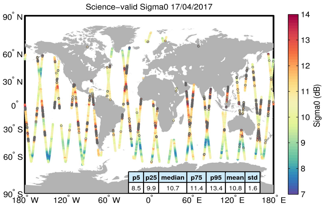
Figure 27. Geographical distribution of science-valid sigma0 data over oceans and lakes for 17/04/2017. The statistical values shown in the table refer to the sigma0 in dB and are calculated over all measurements shown in the figure. Gray circles denote records that have been rejected based on the editing criteria described in Table 4.
