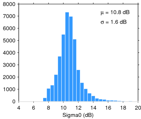
Figure 28. Histogram of science-valid sigma0 over oceans and lakes for 17/04/2017. The mean ( \mu ) and standard deviation ( \sigma ) are also shown. Note that values outside [4 20] dB are excluded from the histogram for the sake of readability but not from the computation of \mu and \sigma .
