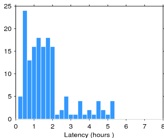
Figure 2. Histogram of the data latency for 17/04/2017. The y-axis denotes the number of files that are made available with a delay of x-hours with respect to the mean time of the records stored in the file.
