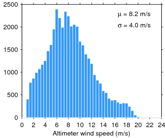
Figure 33. Histogram of flag-valid wind over oceans and lakes for 17/04/2017. The mean ( \mu ) and standard deviation ( \sigma ) are also shown. Note that values larger than 24 m/s are excluded from the histogram for the sake of readability but not from the computation of \mu and \sigma .
