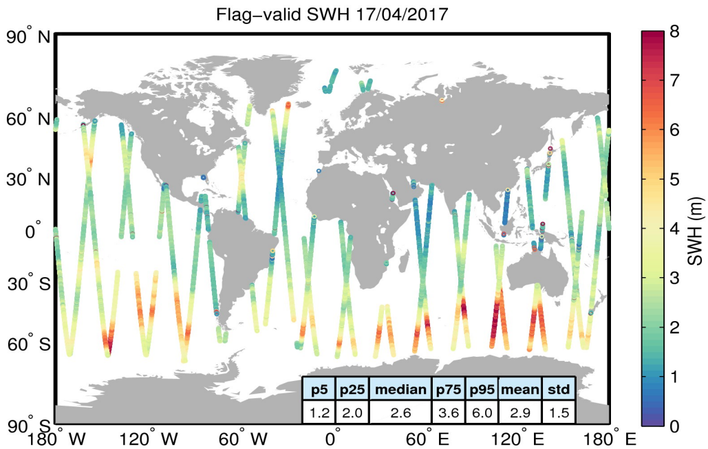
Figure 15. Geographical distribution of flag-valid SWH data over oceans and lakes for 17/04/2017. The statistical values shown in the table refer to the SWH in m and are calculated over all measurements shown in the figure.
