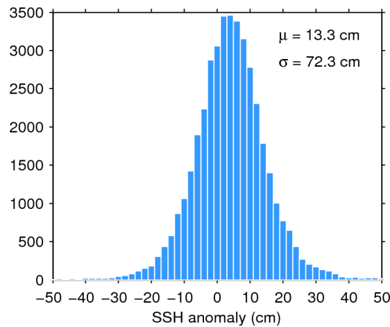
Figure 7. Histogram of flag-valid SSH anomaly over oceans and lakes for 17/04/2017. The mean ( \mu ) and standard deviation ( \sigma ) are also shown. Note that values outside [-50 50] cm are excluded from the histogram for the sake of readability but not from the computation of \mu and \sigma .
