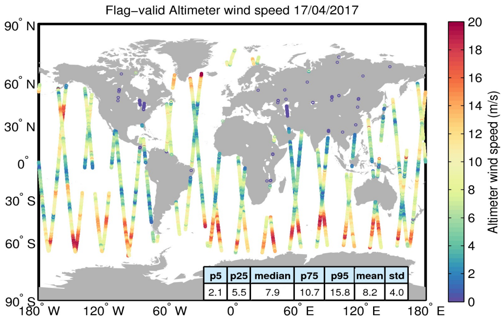
Figure 31. Geographical distribution of flag-valid wind data over oceans and lakes for 17/04/2017. The statistical values shown in the table refer to the wind in m/s and are calculated over all measurements shown in the figure.
