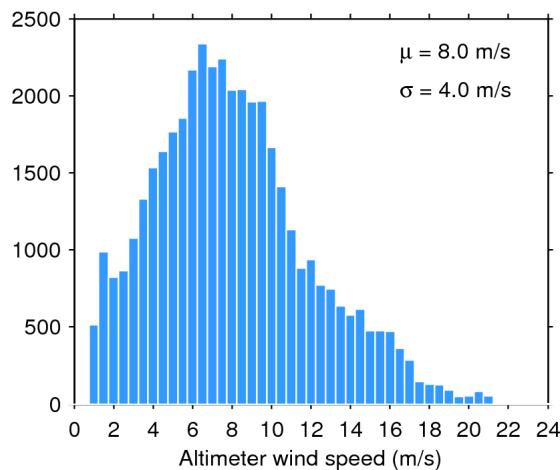
Figure 35. Histogram of science-valid wind over oceans and lakes for 16/04/2017. The mean ( \mu ) and standard deviation ( \sigma ) are also shown. Note that values larger than 24 m/s are excluded from the histogram for the sake of readability but not from the computation of \mu and \sigma .
