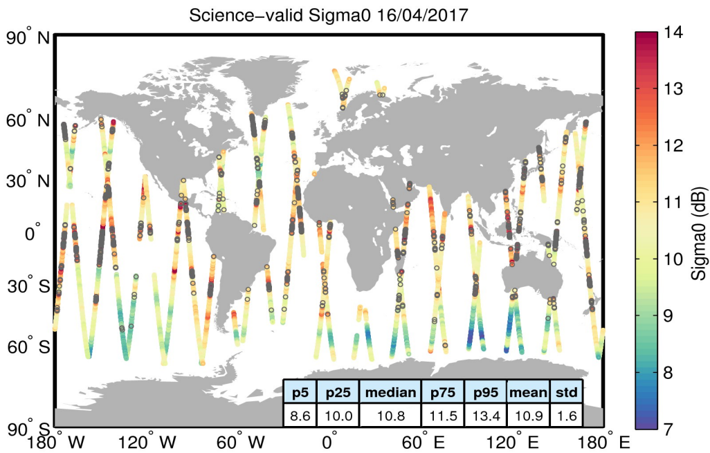
Figure 27. Geographical distribution of science-valid sigma0 data over oceans and lakes for 16/04/2017. The statistical values shown in the table refer to the sigma0 in dB and are calculated over all measurements shown in the figure. Gray circles denote records that have been rejected based on the editing criteria described in Table 4.
