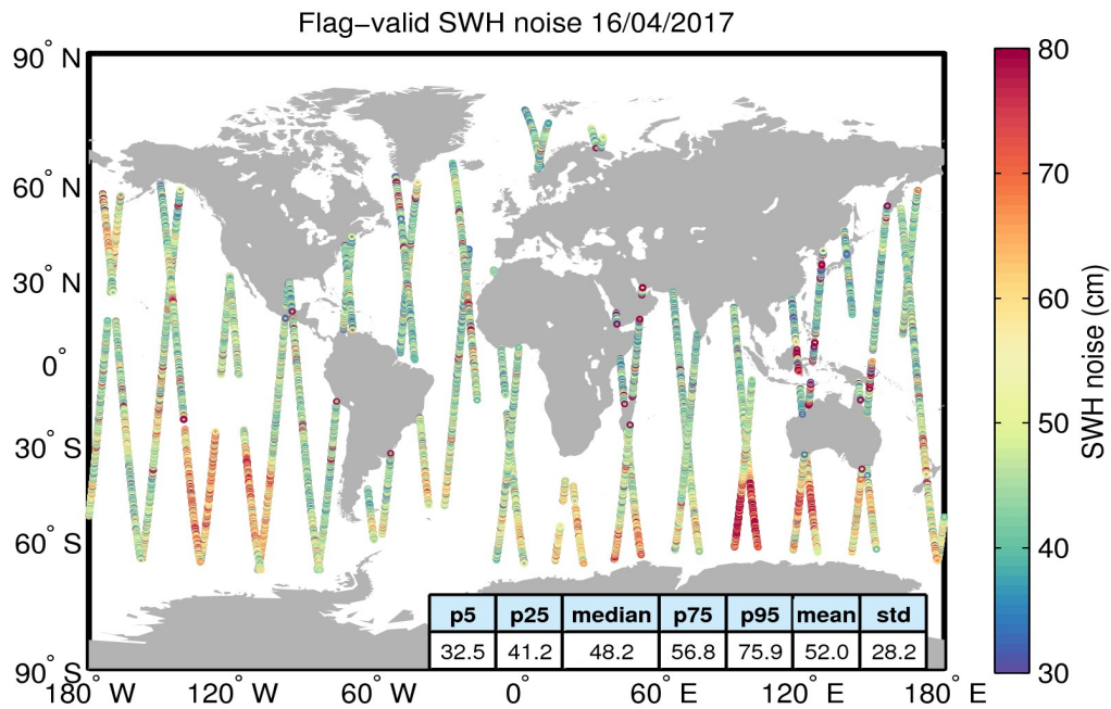
Figure 18. Geographical distribution of flag-valid 20-Hz SWH measurement noise over oceans and lakes for 16/04/2017. The statistical values shown in the table refer to the SWH noise and are calculated over all measurements shown in the figure.
