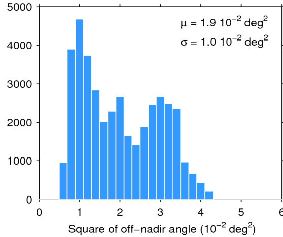
Figure 39. Histogram of flag-valid mispointing over oceans and lakes for 16/04/2017. The mean ( \mu ) and standard deviation ( \sigma ) are also shown. Note that values larger than 6 \cdot 10^{-2} \text{ deg}^2 are excluded from the histogram for the sake of readability but not from the computation of \mu and \sigma .
