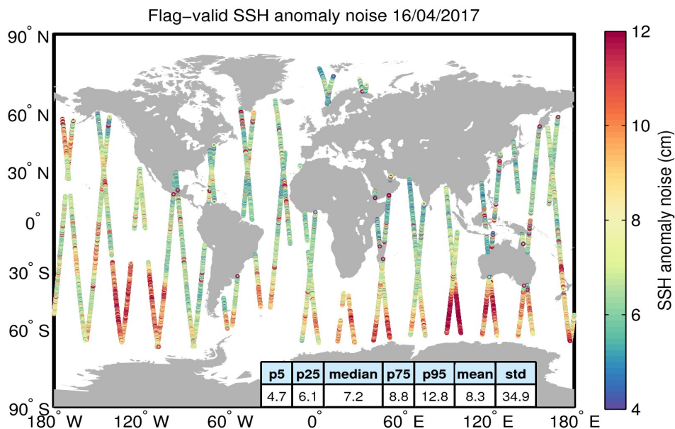
Figure 8. Geographical distribution of flag-valid 20-Hz SSH anomaly measurement noise over oceans and lakes for 16/04/2017. The statistical values shown in the table refer to the SSH anomaly noise and are calculated over all measurements shown in the figure.
