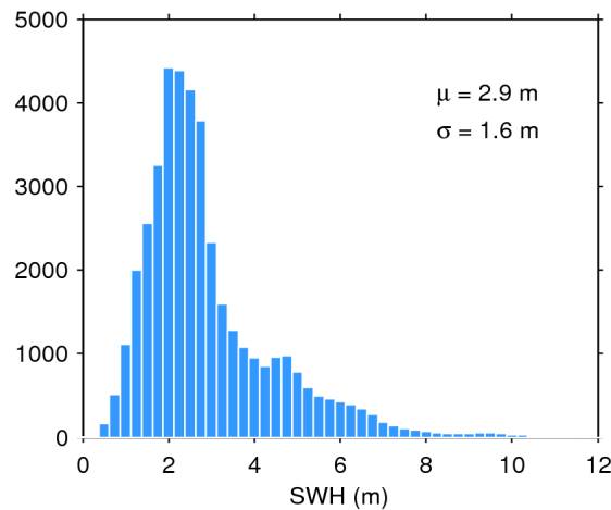
Figure 17. Histogram of flag-valid SWH over oceans and lakes for 16/04/2017. The mean ( \mu ) and standard deviation ( \sigma ) are also shown. Note that values larger than 12 m are excluded from the histogram for the sake of readability but not from the computation of \mu and \sigma .
