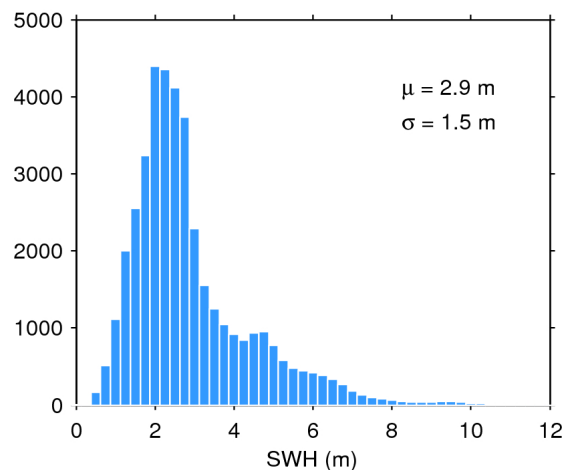
Figure 20. Histogram of science-valid SWH over oceans and lakes for 16/04/2017. The mean ( \mu ) and standard deviation ( \sigma ) are also shown. Note that values larger than 12 m are excluded from the histogram for the sake of readability but not from the computation of \mu and \sigma .
