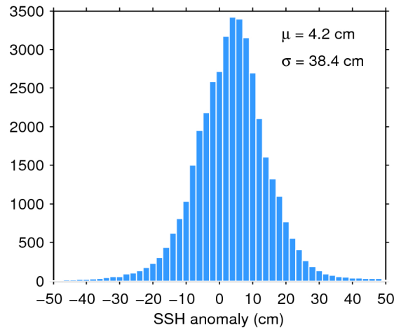
Figure 7. Histogram of flag-valid SSH anomaly over oceans and lakes for 16/04/2017. The mean ( \mu ) and standard deviation ( \sigma ) are also shown. Note that values outside [-50 50] cm are excluded from the histogram for the sake of readability but not from the computation of \mu and \sigma .
