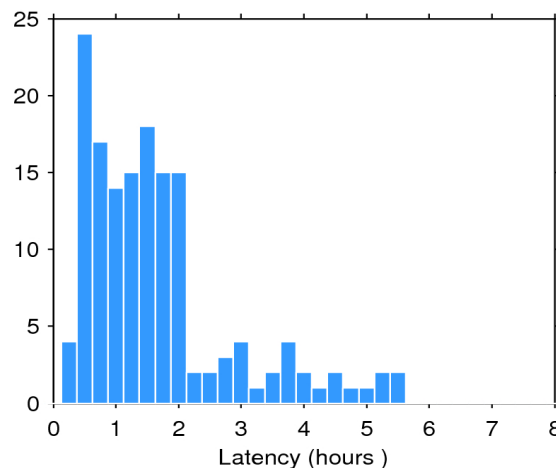
Figure 2. Histogram of the data latency for 16/04/2017. The y-axis denotes the number of files that are made available with a delay of x-hours with respect to the mean time of the records stored in the file.
