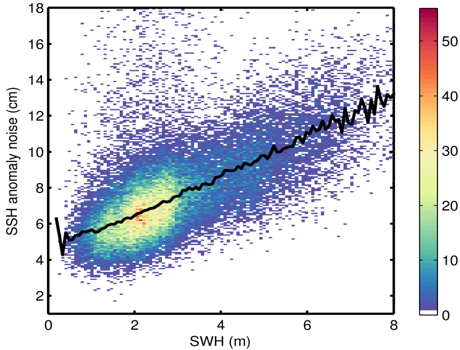
Figure 9. 2D histogram showing flag-valid SSH anomaly noise as a function of SWH for 16/04/2017. The black line denotes the median SSH anomaly noise as a function of SWH.
