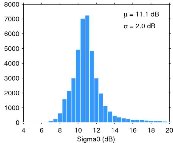
Figure 25. Histogram of flag-valid sigma0 over oceans and lakes for 16/04/2017. The mean ( \mu ) and standard deviation ( \sigma ) are also shown. Note that values outside [4 20] dB are excluded from the histogram for the sake of readability but not from the computation of \mu and \sigma .
