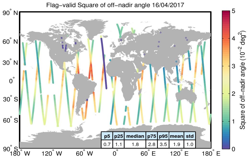
Figure 37. Geographical distribution of flag-valid mispointing data over oceans and lakes for 16/04/2017. The statistical values shown in the table refer to the mispointing in 10^{-2} deg 2 and are calculated over all measurements shown in the figure.
