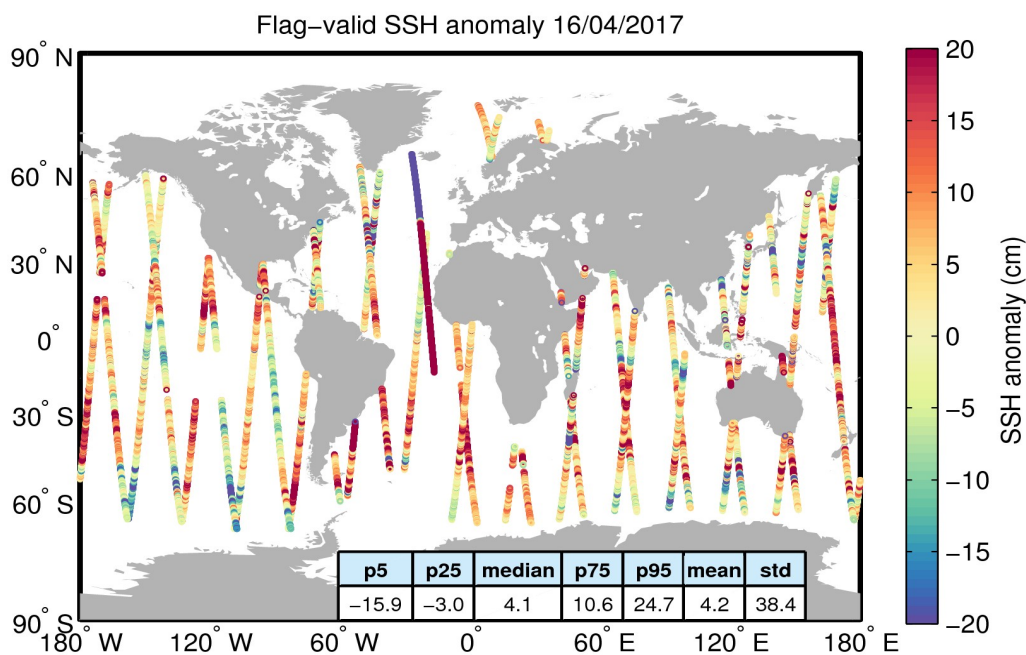
Figure 5. Geographical distribution of flag-valid 1-Hz SSH anomaly data over oceans and lakes for 16/04/2017. The statistical values shown in the table refer to the SSH anomaly in cm and are calculated over all measurements shown in the figure.
