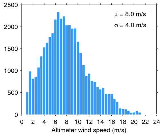
Figure 33. Histogram of flag-valid wind over oceans and lakes for 16/04/2017. The mean ( \mu ) and standard deviation ( \sigma ) are also shown. Note that values larger than 24 m/s are excluded from the histogram for the sake of readability but not from the computation of \mu and \sigma .
