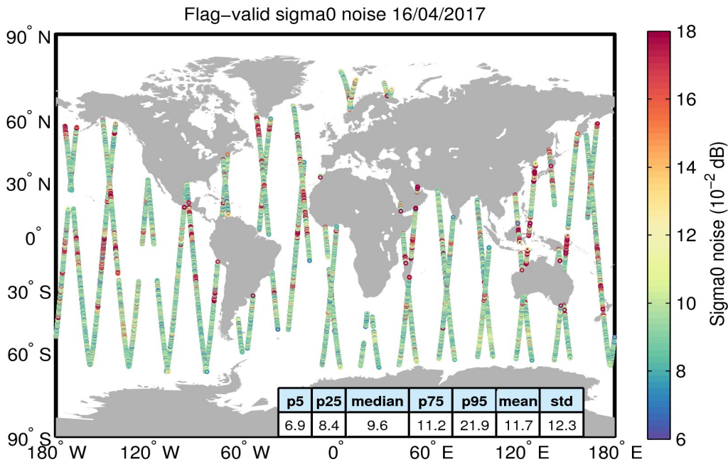
Figure 26. Geographical distribution of flag-valid 20-Hz sigma0 measurement noise over oceans and lakes for 16/04/2017. The statistical values shown in the table refer to the sigma0 noise and are calculated over all measurements shown in the figure.
