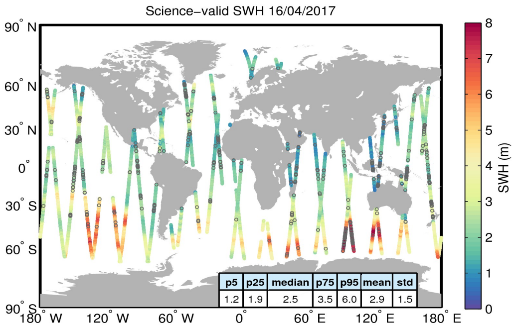
Figure 19. Geographical distribution of science-valid SWH data over oceans and lakes for 16/04/2017. The statistical values shown in the table refer to the SWH in m and are calculated over all measurements shown in the figure. Gray circles denote records that have been rejected based on the editing criteria described in Table 3.
