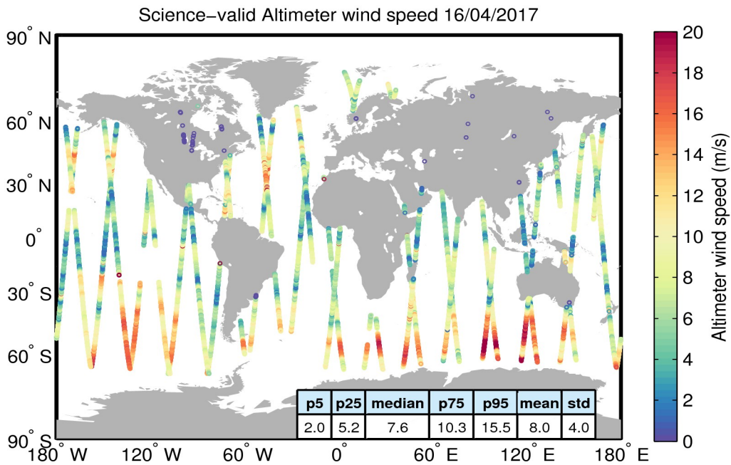
Figure 34. Geographical distribution of science-valid wind data over oceans and lakes for 16/04/2017. The statistical values shown in the table refer to the wind in m/s and are calculated over all measurements shown in the figure. Gray circles denote records that have been rejected based on the editing criteria described in Table 5.
