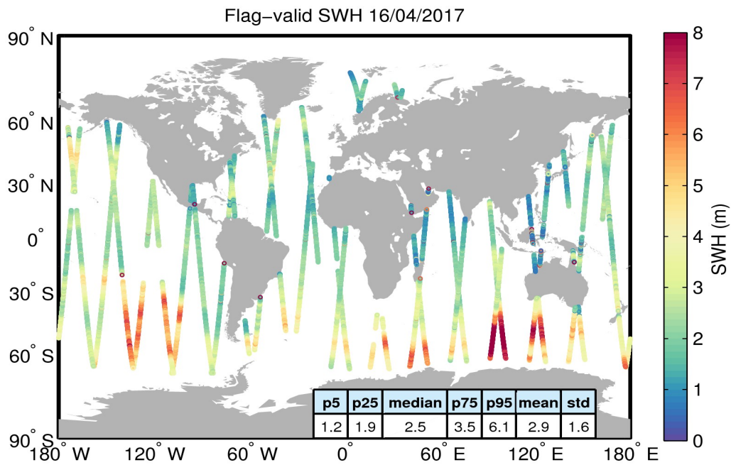
Figure 15. Geographical distribution of flag-valid SWH data over oceans and lakes for 16/04/2017. The statistical values shown in the table refer to the SWH in m and are calculated over all measurements shown in the figure.
