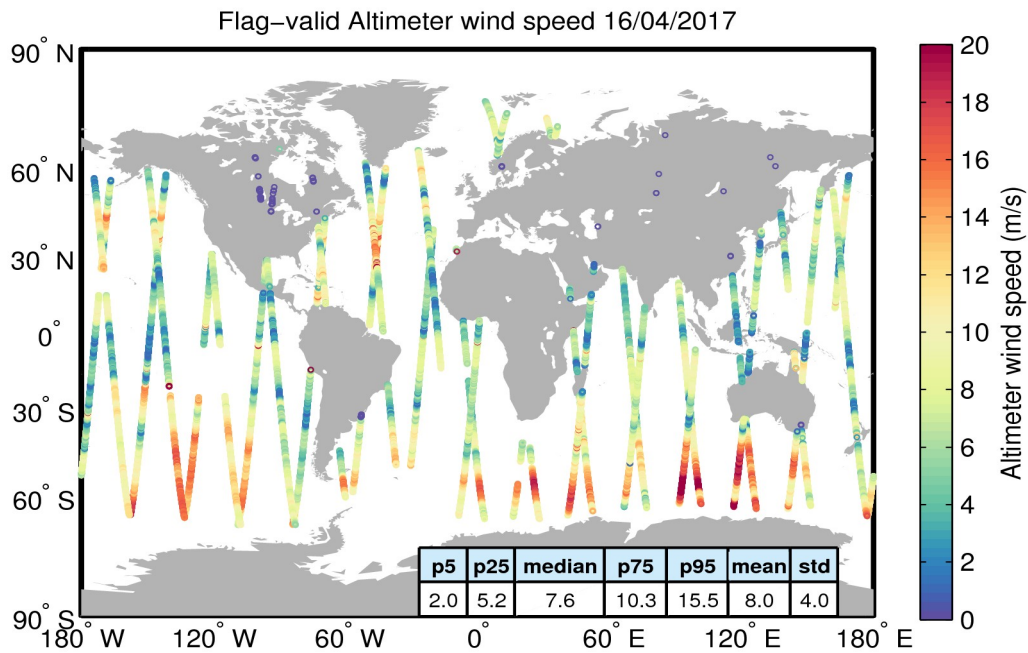
Figure 31. Geographical distribution of flag-valid wind data over oceans and lakes for 16/04/2017. The statistical values shown in the table refer to the wind in m/s and are calculated over all measurements shown in the figure.
