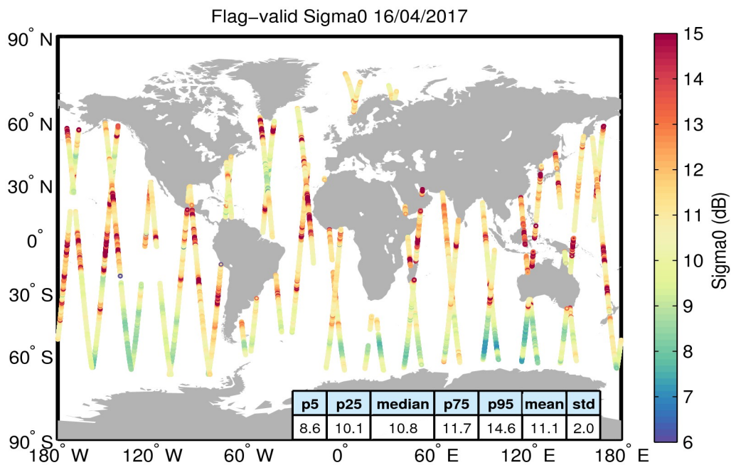
Figure 23. Geographical distribution of flag-valid sigma0 data over oceans and lakes for 16/04/2017. The statistical values shown in the table refer to the sigma0 in dB and are calculated over all measurements shown in the figure.
