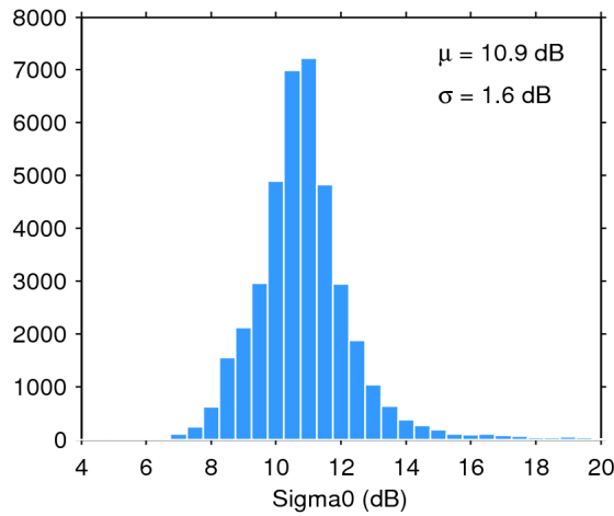
Figure 28. Histogram of science-valid sigma0 over oceans and lakes for 16/04/2017. The mean ( \mu ) and standard deviation ( \sigma ) are also shown. Note that values outside [4 20] dB are excluded from the histogram for the sake of readability but not from the computation of \mu and \sigma .
