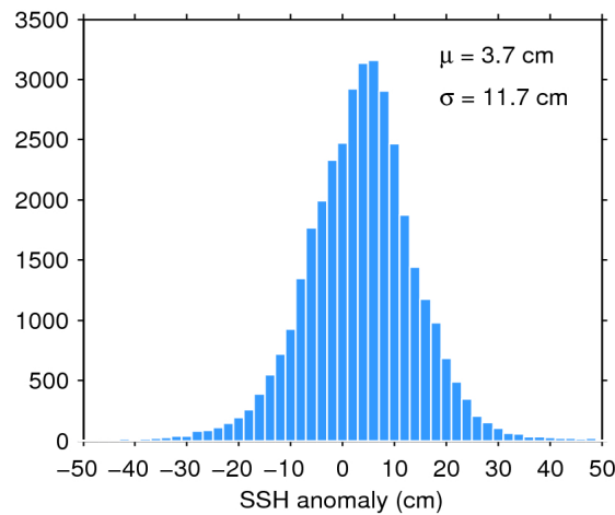
Figure 11. Histogram of science-valid SSH anomaly over oceans and lakes for 16/04/2017. The mean ( \mu ) and standard deviation ( \sigma ) are also shown. Note that values outside [-50 50] cm are excluded from the histogram for the sake of readability but not from the computation of \mu and \sigma .
