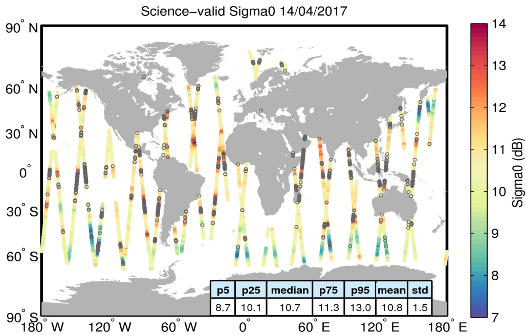
Figure 27. Geographical distribution of science-valid sigma0 data over oceans and lakes for 14/04/2017. The statistical values shown in the table refer to the sigma0 in dB and are calculated over all measurements shown in the figure. Gray circles denote records that have been rejected based on the editing criteria described in Table 4.
