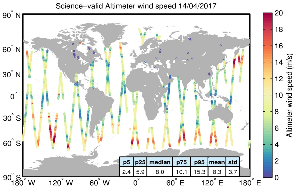
Figure 34. Geographical distribution of science-valid wind data over oceans and lakes for 14/04/2017. The statistical values shown in the table refer to the wind in m/s and are calculated over all measurements shown in the figure. Gray circles denote records that have been rejected based on the editing criteria described in Table 5.
