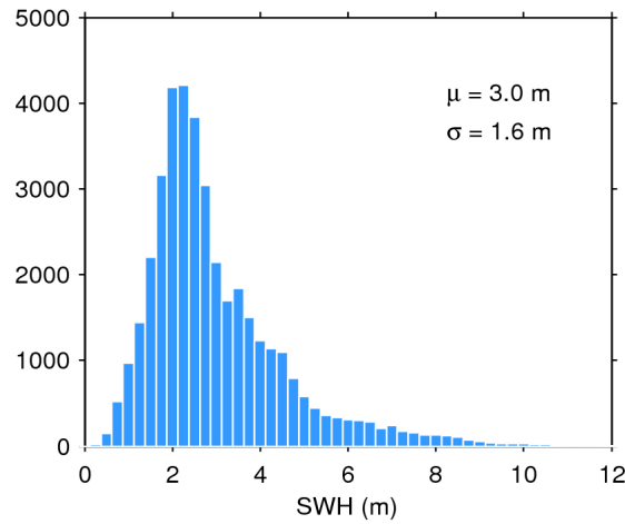
Figure 17. Histogram of flag-valid SWH over oceans and lakes for 14/04/2017. The mean ( \mu ) and standard deviation ( \sigma ) are also shown. Note that values larger than 12 m are excluded from the histogram for the sake of readability but not from the computation of \mu and \sigma .
