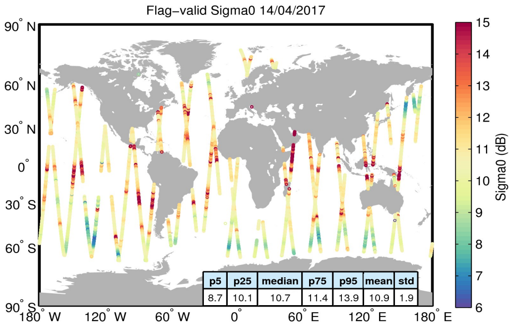
Figure 23. Geographical distribution of flag-valid sigma0 data over oceans and lakes for 14/04/2017. The statistical values shown in the table refer to the sigma0 in dB and are calculated over all measurements shown in the figure.
