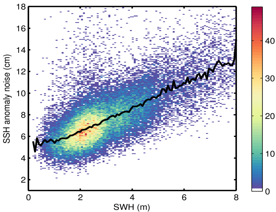
Figure 9. 2D histogram showing flag-valid SSH anomaly noise as a function of SWH for 14/04/2017. The black line denotes the median SSH anomaly noise as a function of SWH.
