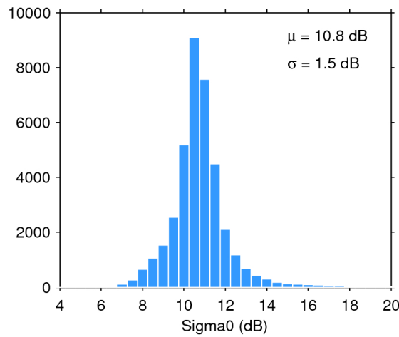
Figure 28. Histogram of science-valid sigma0 over oceans and lakes for 14/04/2017. The mean ( \mu ) and standard deviation ( \sigma ) are also shown. Note that values outside [4 20] dB are excluded from the histogram for the sake of readability but not from the computation of \mu and \sigma .
