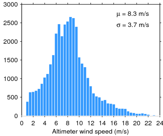
Figure 33. Histogram of flag-valid wind over oceans and lakes for 14/04/2017. The mean ( \mu ) and standard deviation ( \sigma ) are also shown. Note that values larger than 24 m/s are excluded from the histogram for the sake of readability but not from the computation of \mu and \sigma .
