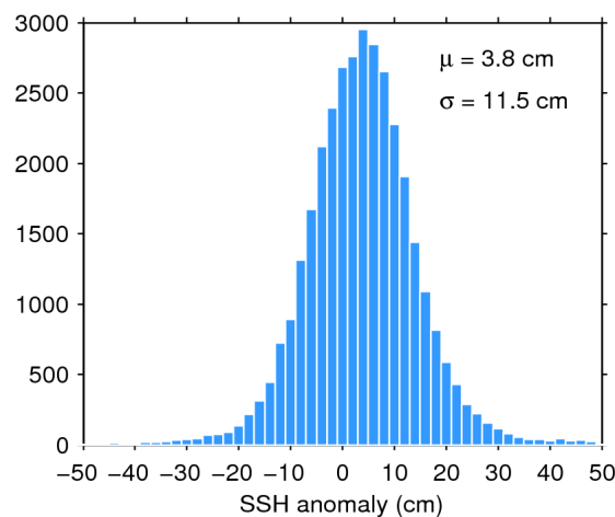
Figure 11. Histogram of science-valid SSH anomaly over oceans and lakes for 14/04/2017. The mean ( \mu ) and standard deviation ( \sigma ) are also shown. Note that values outside [-50 50] cm are excluded from the histogram for the sake of readability but not from the computation of \mu and \sigma .
