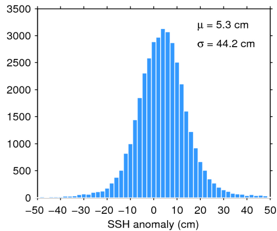
Figure 7. Histogram of flag-valid SSH anomaly over oceans and lakes for 14/04/2017. The mean ( \mu ) and standard deviation ( \sigma ) are also shown. Note that values outside [-50 50] cm are excluded from the histogram for the sake of readability but not from the computation of \mu and \sigma .
