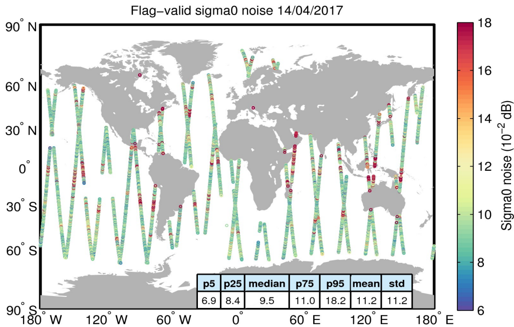
Figure 26. Geographical distribution of flag-valid 20-Hz sigma0 measurement noise over oceans and lakes for 14/04/2017. The statistical values shown in the table refer to the sigma0 noise and are calculated over all measurements shown in the figure.
