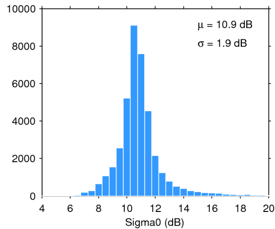
Figure 25. Histogram of flag-valid sigma0 over oceans and lakes for 14/04/2017. The mean ( \mu ) and standard deviation ( \sigma ) are also shown. Note that values outside [4 20] dB are excluded from the histogram for the sake of readability but not from the computation of \mu and \sigma .
