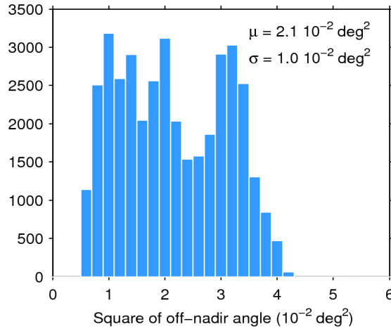
Figure 39. Histogram of flag-valid mispointing over oceans and lakes for 14/04/2017. The mean ( \mu ) and standard deviation ( \sigma ) are also shown. Note that values larger than 6 \cdot 10^{-2} \text{ deg}^2 are excluded from the histogram for the sake of readability but not from the computation of \mu and \sigma .
