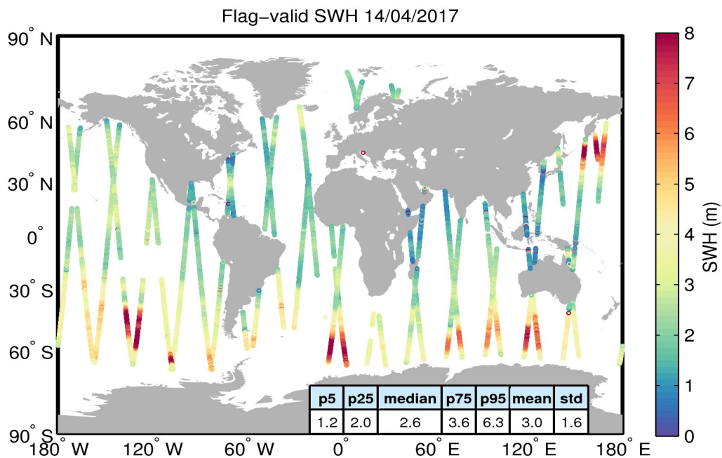
Figure 15. Geographical distribution of flag-valid SWH data over oceans and lakes for 14/04/2017. The statistical values shown in the table refer to the SWH in m and are calculated over all measurements shown in the figure.
