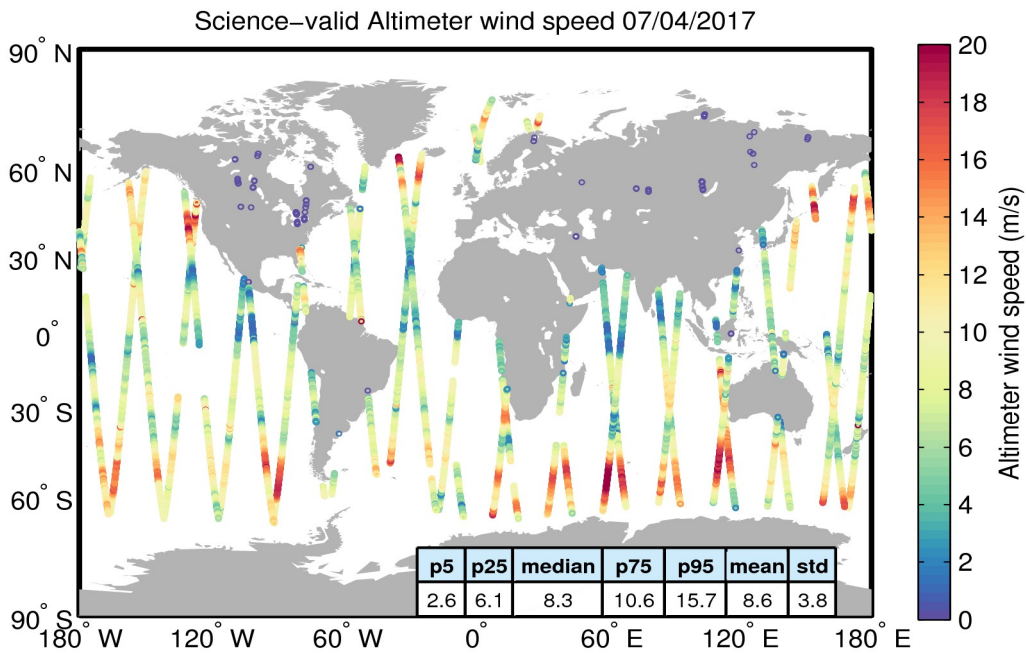
Figure 34. Geographical distribution of science-valid wind data over oceans and lakes for 07/04/2017. The statistical values shown in the table refer to the wind in m/s and are calculated over all measurements shown in the figure. Gray circles denote records that have been rejected based on the editing criteria described in Table 5.
