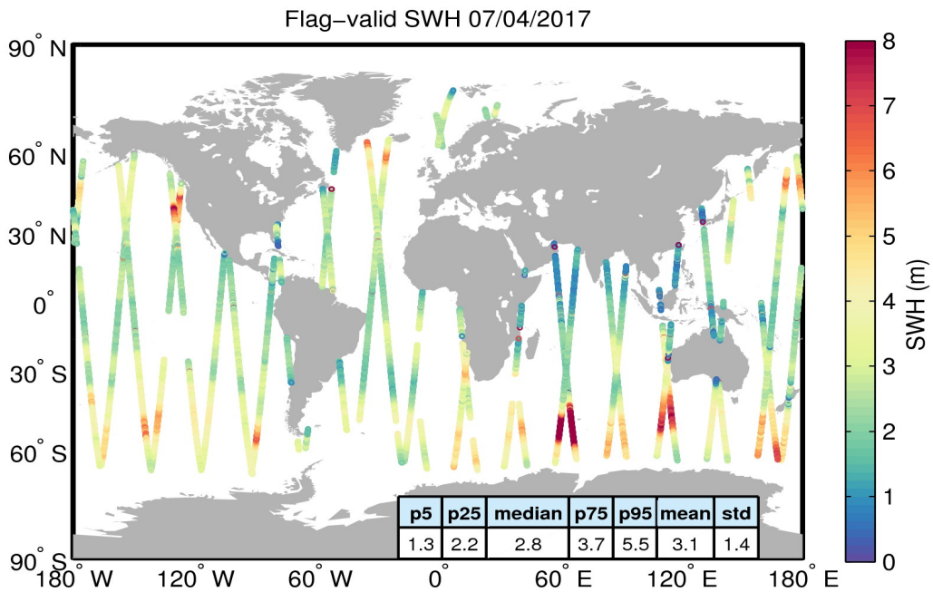
Figure 15. Geographical distribution of flag-valid SWH data over oceans and lakes for 07/04/2017. The statistical values shown in the table refer to the SWH in m and are calculated over all measurements shown in the figure.
