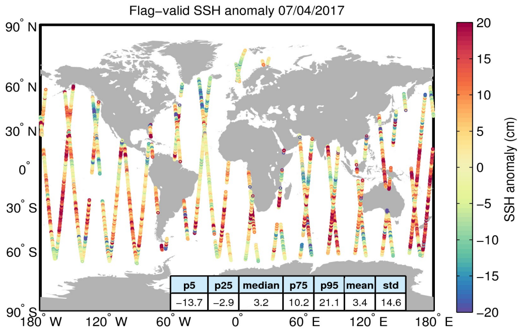
Figure 5. Geographical distribution of flag-valid 1-Hz SSH anomaly data over oceans and lakes for 07/04/2017. The statistical values shown in the table refer to the SSH anomaly in cm and are calculated over all measurements shown in the figure.
