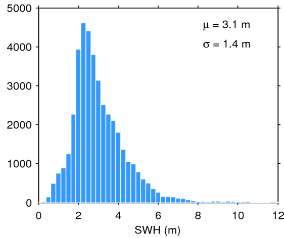
Figure 17. Histogram of flag-valid SWH over oceans and lakes for 07/04/2017. The mean ( \mu ) and standard deviation ( \sigma ) are also shown. Note that values larger than 12 m are excluded from the histogram for the sake of readability but not from the computation of \mu and \sigma .
