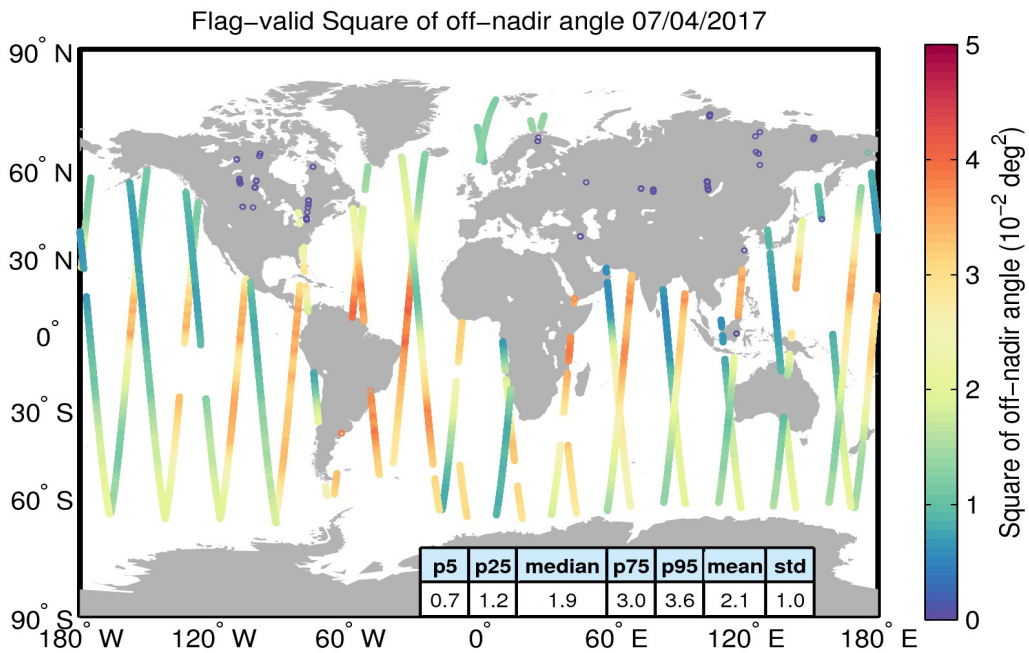
Figure 37. Geographical distribution of flag-valid mispointing data over oceans and lakes for 07/04/2017. The statistical values shown in the table refer to the mispointing in 10^{-2} deg 2 and are calculated over all measurements shown in the figure.
