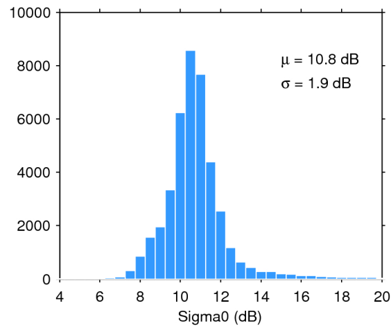
Figure 25. Histogram of flag-valid sigma0 over oceans and lakes for 07/04/2017. The mean ( \mu ) and standard deviation ( \sigma ) are also shown. Note that values outside [4 20] dB are excluded from the histogram for the sake of readability but not from the computation of \mu and \sigma .
