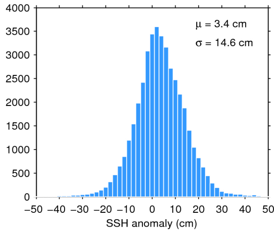
Figure 7. Histogram of flag-valid SSH anomaly over oceans and lakes for 07/04/2017. The mean ( \mu ) and standard deviation ( \sigma ) are also shown. Note that values outside [-50 50] cm are excluded from the histogram for the sake of readability but not from the computation of \mu and \sigma .
