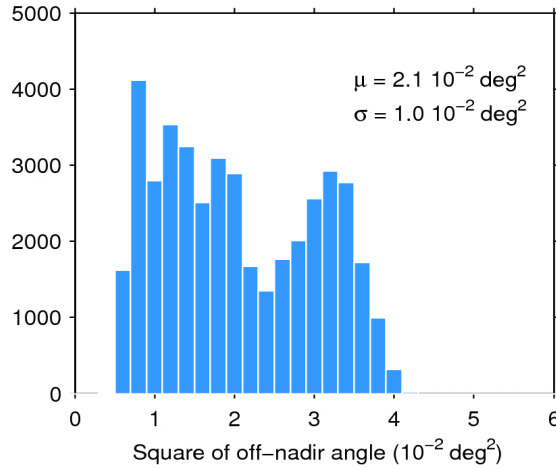
Figure 39. Histogram of flag-valid mispointing over oceans and lakes for 07/04/2017. The mean ( \mu ) and standard deviation ( \sigma ) are also shown. Note that values larger than 6 \cdot 10^{-2} \text{ deg}^2 are excluded from the histogram for the sake of readability but not from the computation of \mu and \sigma .
