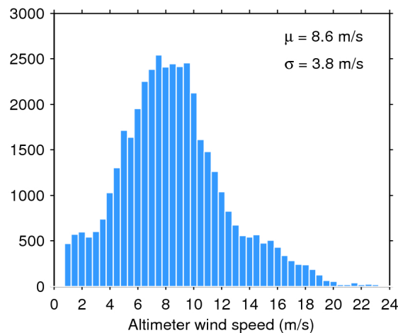
Figure 35. Histogram of science-valid wind over oceans and lakes for 07/04/2017. The mean ( \mu ) and standard deviation ( \sigma ) are also shown. Note that values larger than 24 m/s are excluded from the histogram for the sake of readability but not from the computation of \mu and \sigma .
