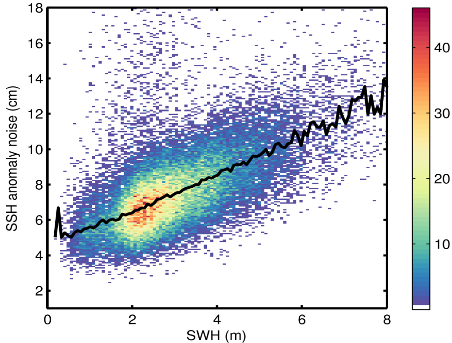
Figure 9. 2D histogram showing flag-valid SSH anomaly noise as a function of SWH for 07/04/2017. The black line denotes the median SSH anomaly noise as a function of SWH.
