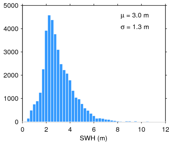
Figure 20. Histogram of science-valid SWH over oceans and lakes for 07/04/2017. The mean ( \mu ) and standard deviation ( \sigma ) are also shown. Note that values larger than 12 m are excluded from the histogram for the sake of readability but not from the computation of \mu and \sigma .
