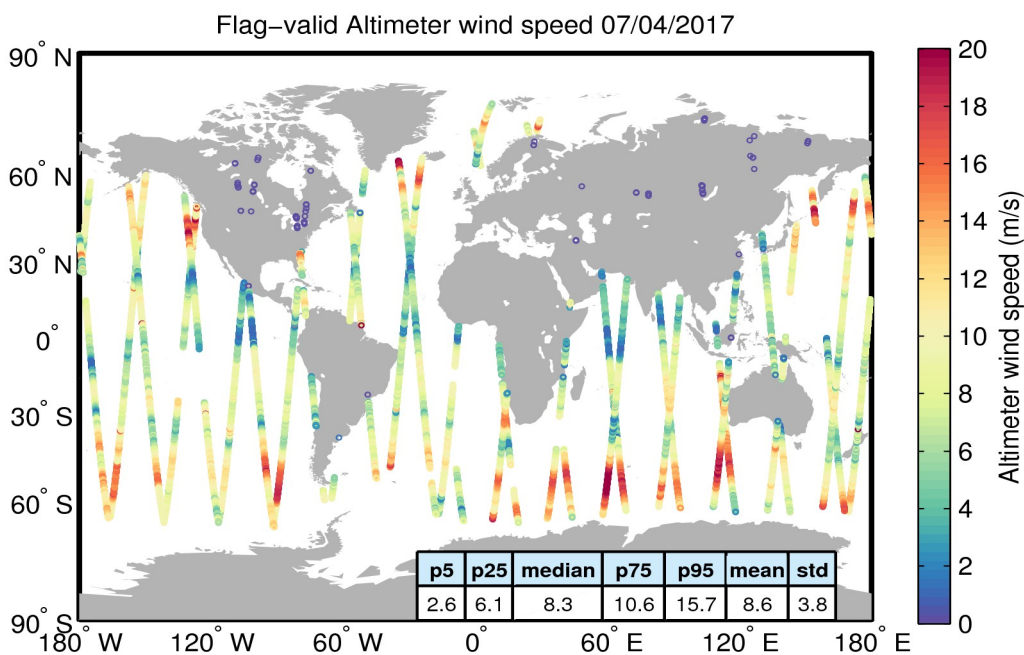
Figure 31. Geographical distribution of flag-valid wind data over oceans and lakes for 07/04/2017. The statistical values shown in the table refer to the wind in m/s and are calculated over all measurements shown in the figure.
