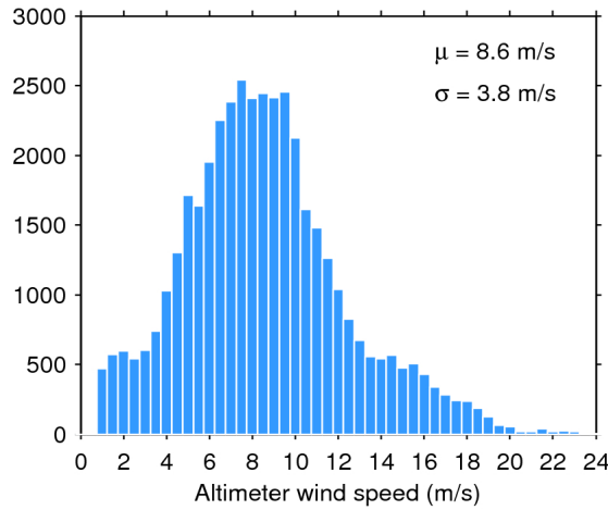
Figure 33. Histogram of flag-valid wind over oceans and lakes for 07/04/2017. The mean ( \mu ) and standard deviation ( \sigma ) are also shown. Note that values larger than 24 m/s are excluded from the histogram for the sake of readability but not from the computation of \mu and \sigma .
