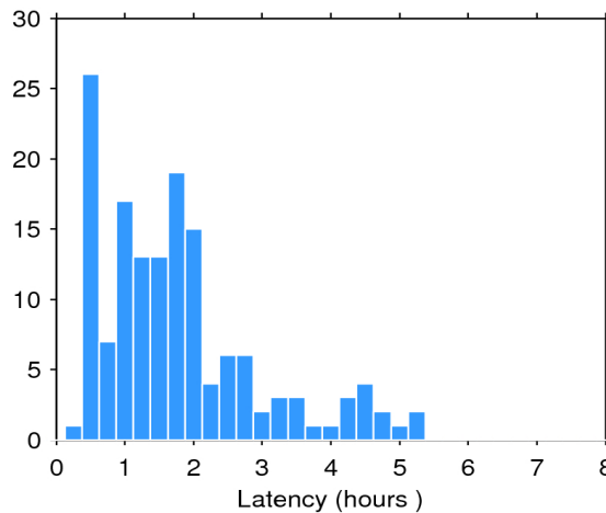
Figure 2. Histogram of the data latency for 07/04/2017. The y-axis denotes the number of files that are made available with a delay of x-hours with respect to the mean time of the records stored in the file.
