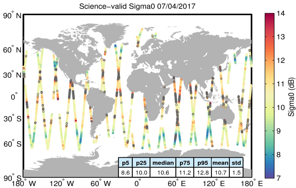
Figure 27. Geographical distribution of science-valid sigma0 data over oceans and lakes for 07/04/2017. The statistical values shown in the table refer to the sigma0 in dB and are calculated over all measurements shown in the figure. Gray circles denote records that have been rejected based on the editing criteria described in Table 4.
