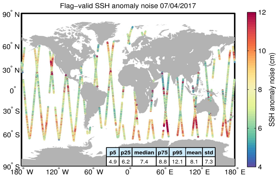
Figure 8. Geographical distribution of flag-valid 20-Hz SSH anomaly measurement noise over oceans and lakes for 07/04/2017. The statistical values shown in the table refer to the SSH anomaly noise and are calculated over all measurements shown in the figure.
