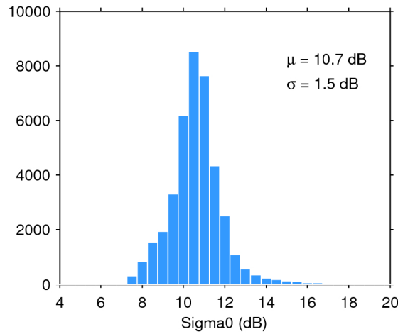
Figure 28. Histogram of science-valid sigma0 over oceans and lakes for 07/04/2017. The mean ( \mu ) and standard deviation ( \sigma ) are also shown. Note that values outside [4 20] dB are excluded from the histogram for the sake of readability but not from the computation of \mu and \sigma .
