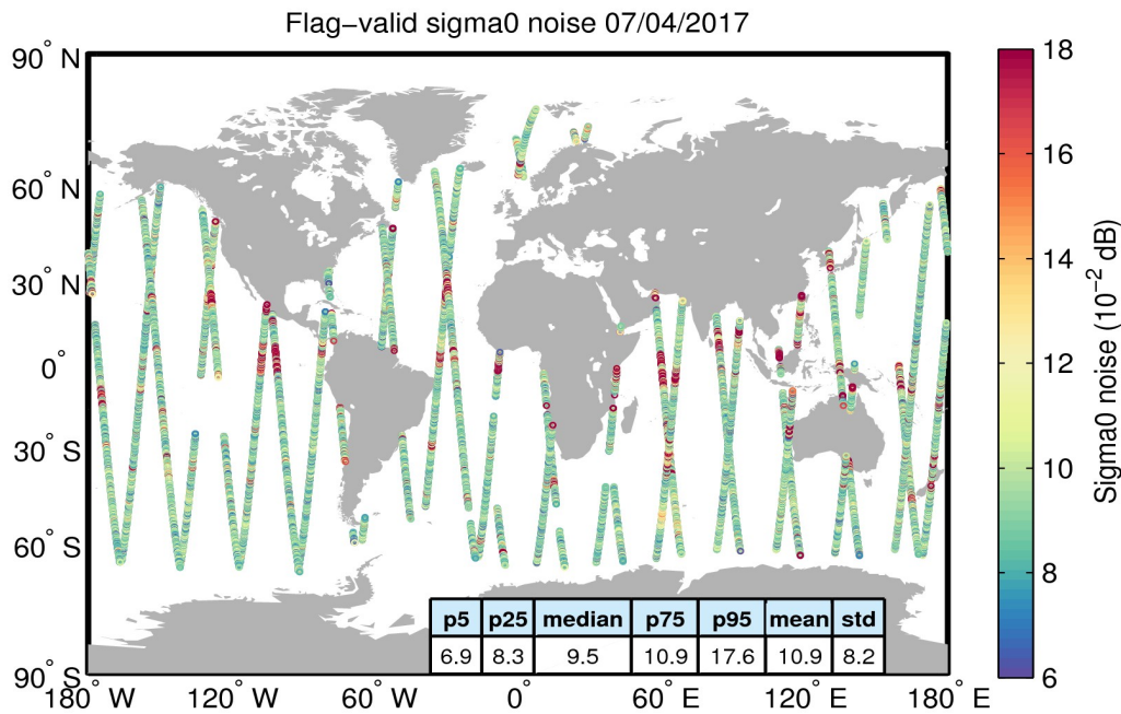
Figure 26. Geographical distribution of flag-valid 20-Hz sigma0 measurement noise over oceans and lakes for 07/04/2017. The statistical values shown in the table refer to the sigma0 noise and are calculated over all measurements shown in the figure.
