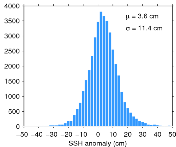
Figure 11. Histogram of science-valid SSH anomaly over oceans and lakes for 05/04/2017. The mean ( \mu ) and standard deviation ( \sigma ) are also shown. Note that values outside [-50 50] cm are excluded from the histogram for the sake of readability but not from the computation of \mu and \sigma .
