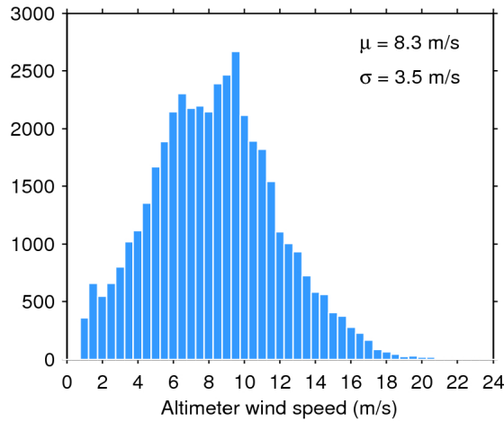
Figure 33. Histogram of flag-valid wind over oceans and lakes for 05/04/2017. The mean ( \mu ) and standard deviation ( \sigma ) are also shown. Note that values larger than 24 m/s are excluded from the histogram for the sake of readability but not from the computation of \mu and \sigma .
