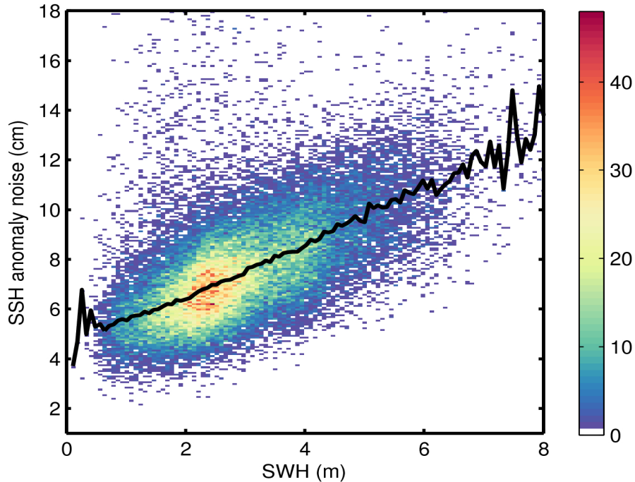
Figure 9. 2D histogram showing flag-valid SSH anomaly noise as a function of SWH for 05/04/2017. The black line denotes the median SSH anomaly noise as a function of SWH.
