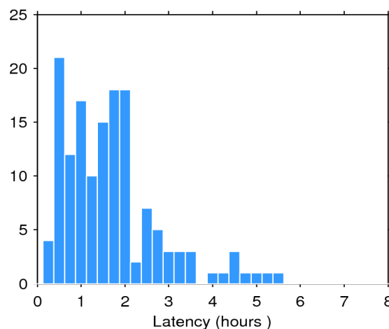
Figure 2. Histogram of the data latency for 05/04/2017. The y-axis denotes the number of files that are made available with a delay of x-hours with respect to the mean time of the records stored in the file.
