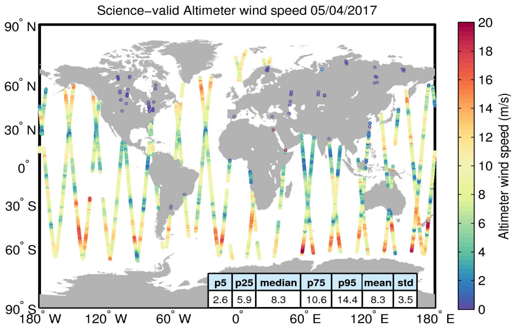
Figure 34. Geographical distribution of science-valid wind data over oceans and lakes for 05/04/2017. The statistical values shown in the table refer to the wind in m/s and are calculated over all measurements shown in the figure. Gray circles denote records that have been rejected based on the editing criteria described in Table 5.
