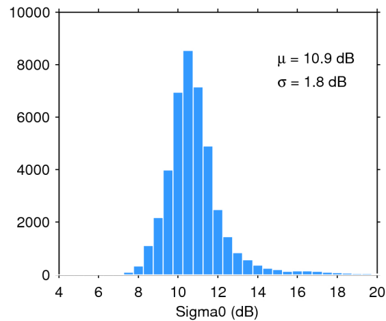
Figure 25. Histogram of flag-valid sigma0 over oceans and lakes for 05/04/2017. The mean ( \mu ) and standard deviation ( \sigma ) are also shown. Note that values outside [4 20] dB are excluded from the histogram for the sake of readability but not from the computation of \mu and \sigma .
