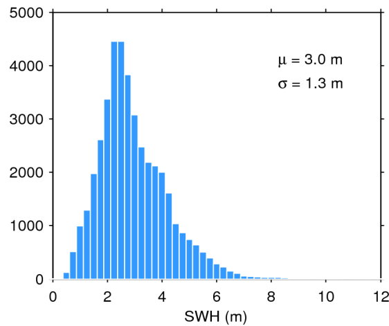
Figure 17. Histogram of flag-valid SWH over oceans and lakes for 05/04/2017. The mean ( \mu ) and standard deviation ( \sigma ) are also shown. Note that values larger than 12 m are excluded from the histogram for the sake of readability but not from the computation of \mu and \sigma .
