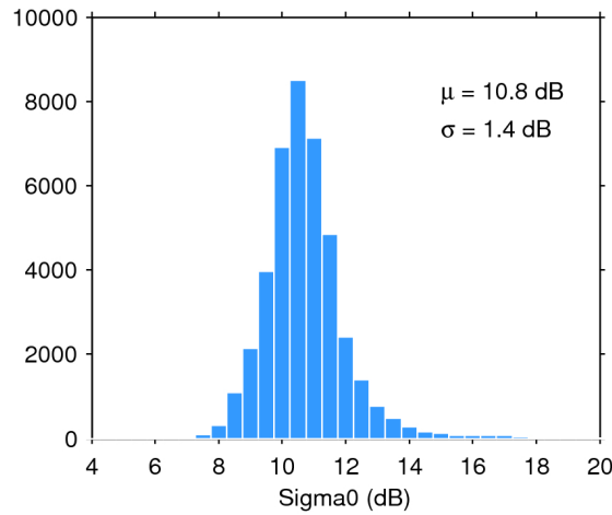
Figure 28. Histogram of science-valid sigma0 over oceans and lakes for 05/04/2017. The mean ( \mu ) and standard deviation ( \sigma ) are also shown. Note that values outside [4 20] dB are excluded from the histogram for the sake of readability but not from the computation of \mu and \sigma .
