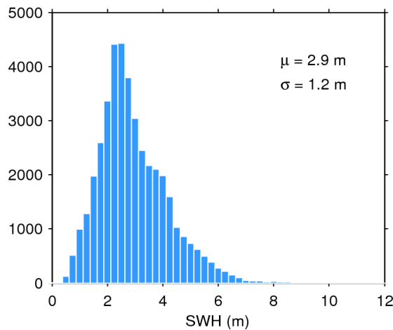
Figure 20. Histogram of science-valid SWH over oceans and lakes for 05/04/2017. The mean ( \mu ) and standard deviation ( \sigma ) are also shown. Note that values larger than 12 m are excluded from the histogram for the sake of readability but not from the computation of \mu and \sigma .
