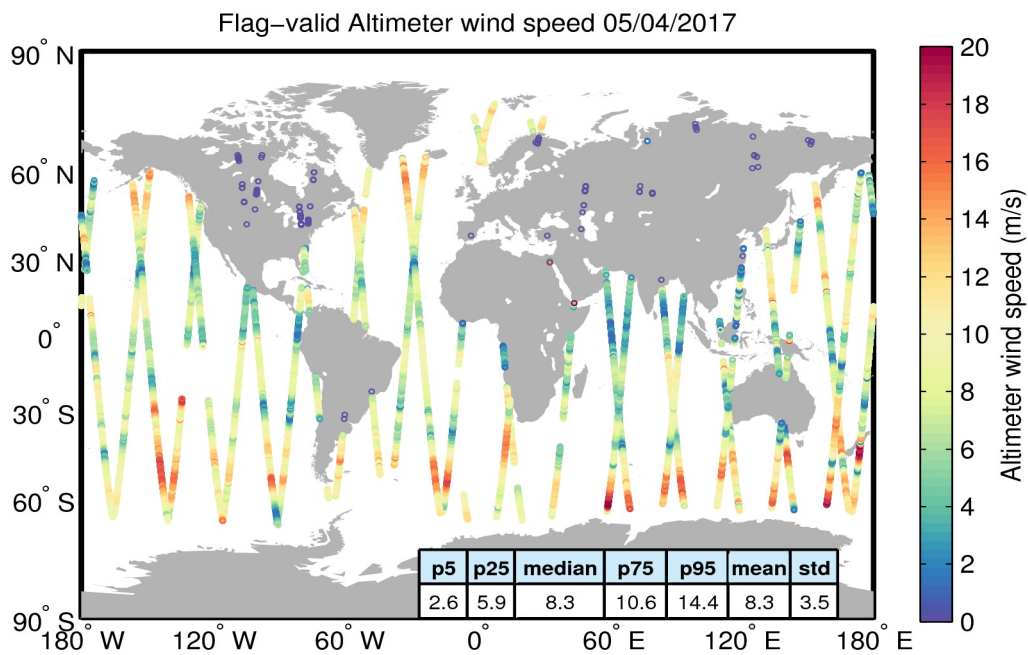
Figure 31. Geographical distribution of flag-valid wind data over oceans and lakes for 05/04/2017. The statistical values shown in the table refer to the wind in m/s and are calculated over all measurements shown in the figure.
