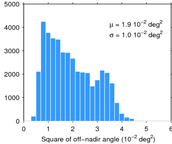
Figure 39. Histogram of flag-valid mispointing over oceans and lakes for 05/04/2017. The mean ( \mu ) and standard deviation ( \sigma ) are also shown. Note that values larger than 6 \cdot 10^{-2} \text{ deg}^2 are excluded from the histogram for the sake of readability but not from the computation of \mu and \sigma .
