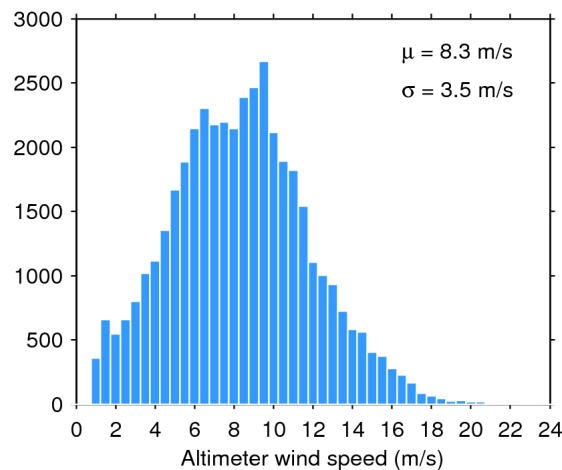
Figure 35. Histogram of science-valid wind over oceans and lakes for 05/04/2017. The mean ( \mu ) and standard deviation ( \sigma ) are also shown. Note that values larger than 24 m/s are excluded from the histogram for the sake of readability but not from the computation of \mu and \sigma .
