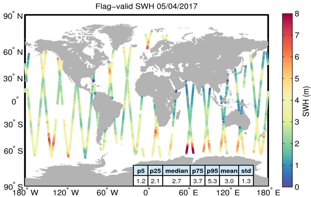
Figure 15. Geographical distribution of flag-valid SWH data over oceans and lakes for 05/04/2017. The statistical values shown in the table refer to the SWH in m and are calculated over all measurements shown in the figure.
