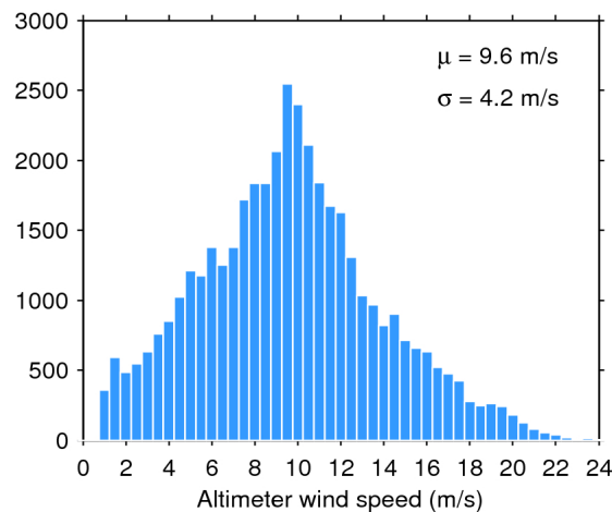
Figure 35. Histogram of science-valid wind over oceans and lakes for 04/04/2017. The mean ( \mu ) and standard deviation ( \sigma ) are also shown. Note that values larger than 24 m/s are excluded from the histogram for the sake of readability but not from the computation of \mu and \sigma .
