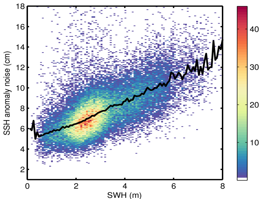
Figure 9. 2D histogram showing flag-valid SSH anomaly noise as a function of SWH for 04/04/2017. The black line denotes the median SSH anomaly noise as a function of SWH.
