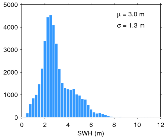
Figure 20. Histogram of science-valid SWH over oceans and lakes for 04/04/2017. The mean ( \mu ) and standard deviation ( \sigma ) are also shown. Note that values larger than 12 m are excluded from the histogram for the sake of readability but not from the computation of \mu and \sigma .
