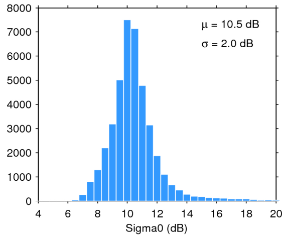
Figure 25. Histogram of flag-valid sigma0 over oceans and lakes for 04/04/2017. The mean ( \mu ) and standard deviation ( \sigma ) are also shown. Note that values outside [4 20] dB are excluded from the histogram for the sake of readability but not from the computation of \mu and \sigma .
