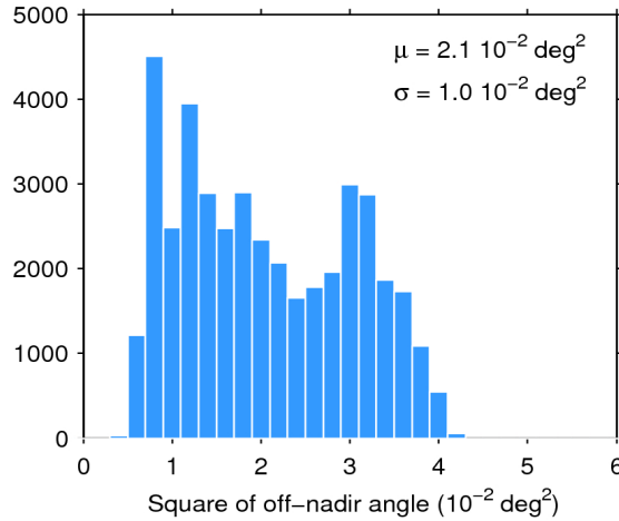
Figure 39. Histogram of flag-valid mispointing over oceans and lakes for 04/04/2017. The mean ( \mu ) and standard deviation ( \sigma ) are also shown. Note that values larger than 6 \cdot 10^{-2} \text{ deg}^2 are excluded from the histogram for the sake of readability but not from the computation of \mu and \sigma .
