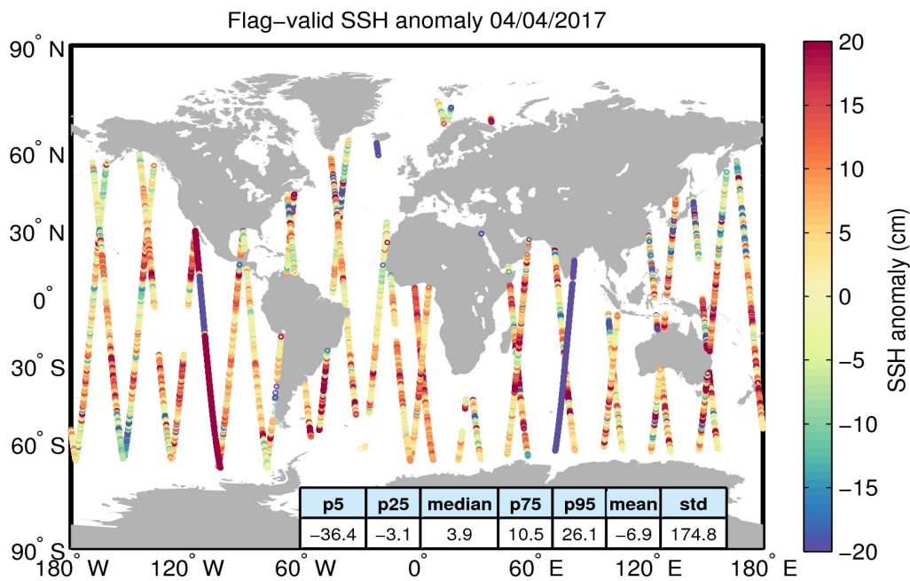
Figure 5. Geographical distribution of flag-valid 1-Hz SSH anomaly data over oceans and lakes for 04/04/2017. The statistical values shown in the table refer to the SSH anomaly in cm and are calculated over all measurements shown in the figure.
