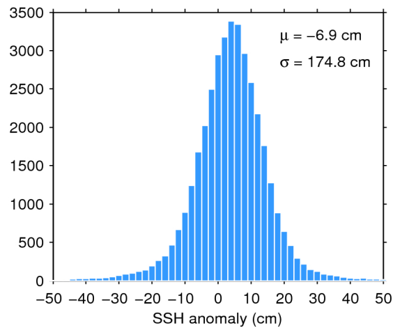
Figure 7. Histogram of flag-valid SSH anomaly over oceans and lakes for 04/04/2017. The mean ( \mu ) and standard deviation ( \sigma ) are also shown. Note that values outside [-50 50] cm are excluded from the histogram for the sake of readability but not from the computation of \mu and \sigma .
