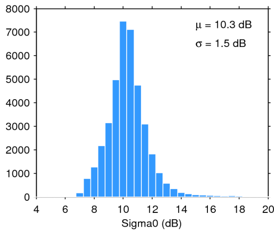
Figure 28. Histogram of science-valid sigma0 over oceans and lakes for 04/04/2017. The mean ( \mu ) and standard deviation ( \sigma ) are also shown. Note that values outside [4 20] dB are excluded from the histogram for the sake of readability but not from the computation of \mu and \sigma .
