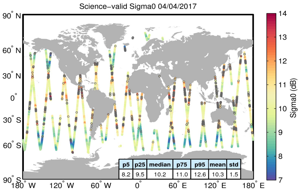
Figure 27. Geographical distribution of science-valid sigma0 data over oceans and lakes for 04/04/2017. The statistical values shown in the table refer to the sigma0 in dB and are calculated over all measurements shown in the figure. Gray circles denote records that have been rejected based on the editing criteria described in Table 4.
