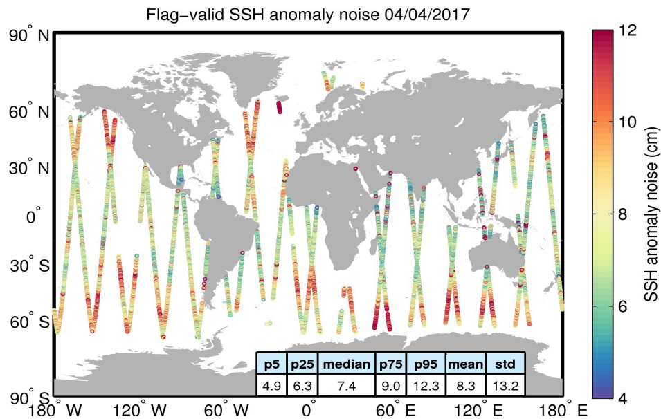
Figure 8. Geographical distribution of flag-valid 20-Hz SSH anomaly measurement noise over oceans and lakes for 04/04/2017. The statistical values shown in the table refer to the SSH anomaly noise and are calculated over all measurements shown in the figure.
