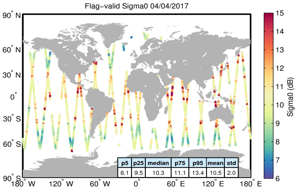
Figure 23. Geographical distribution of flag-valid sigma0 data over oceans and lakes for 04/04/2017. The statistical values shown in the table refer to the sigma0 in dB and are calculated over all measurements shown in the figure.
