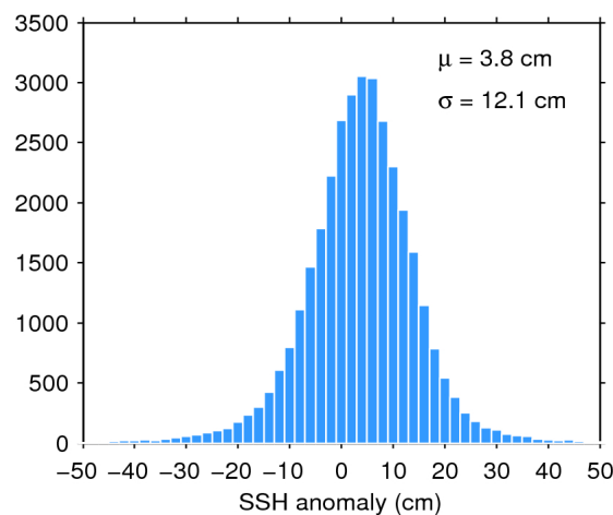
Figure 11. Histogram of science-valid SSH anomaly over oceans and lakes for 04/04/2017. The mean ( \mu ) and standard deviation ( \sigma ) are also shown. Note that values outside [-50 50] cm are excluded from the histogram for the sake of readability but not from the computation of \mu and \sigma .
