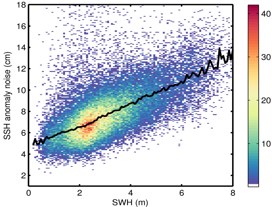
Figure 9. 2D histogram showing flag-valid SSH anomaly noise as a function of SWH for 03/04/2017. The black line denotes the median SSH anomaly noise as a function of SWH.
