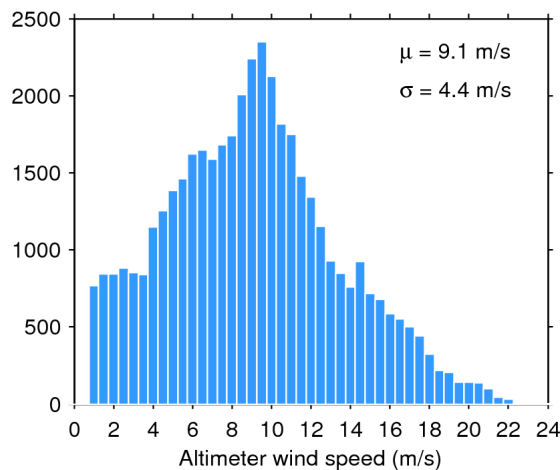
Figure 35. Histogram of science-valid wind over oceans and lakes for 03/04/2017. The mean ( \mu ) and standard deviation ( \sigma ) are also shown. Note that values larger than 24 m/s are excluded from the histogram for the sake of readability but not from the computation of \mu and \sigma .
