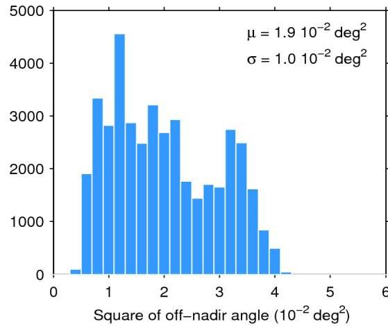
Figure 39. Histogram of flag-valid mispointing over oceans and lakes for 03/04/2017. The mean ( \mu ) and standard deviation ( \sigma ) are also shown. Note that values larger than 6 \cdot 10^{-2} \text{ deg}^2 are excluded from the histogram for the sake of readability but not from the computation of \mu and \sigma .
