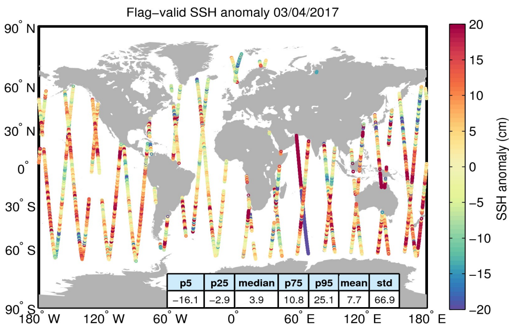
Figure 5. Geographical distribution of flag-valid 1-Hz SSH anomaly data over oceans and lakes for 03/04/2017. The statistical values shown in the table refer to the SSH anomaly in cm and are calculated over all measurements shown in the figure.
