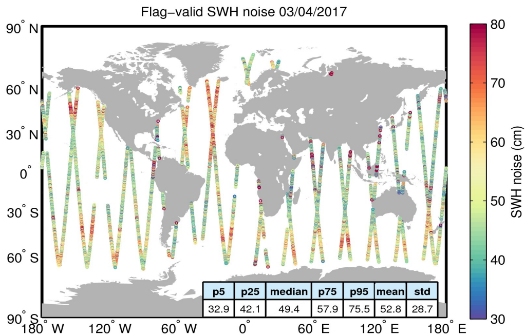
Figure 18. Geographical distribution of flag-valid 20-Hz SWH measurement noise over oceans and lakes for 03/04/2017. The statistical values shown in the table refer to the SWH noise and are calculated over all measurements shown in the figure.
