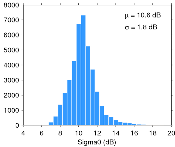
Figure 28. Histogram of science-valid sigma0 over oceans and lakes for 03/04/2017. The mean ( \mu ) and standard deviation ( \sigma ) are also shown. Note that values outside [4 20] dB are excluded from the histogram for the sake of readability but not from the computation of \mu and \sigma .
