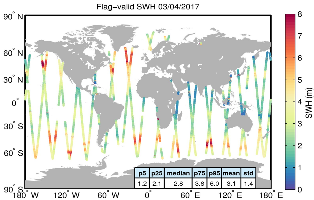
Figure 15. Geographical distribution of flag-valid SWH data over oceans and lakes for 03/04/2017. The statistical values shown in the table refer to the SWH in m and are calculated over all measurements shown in the figure.
