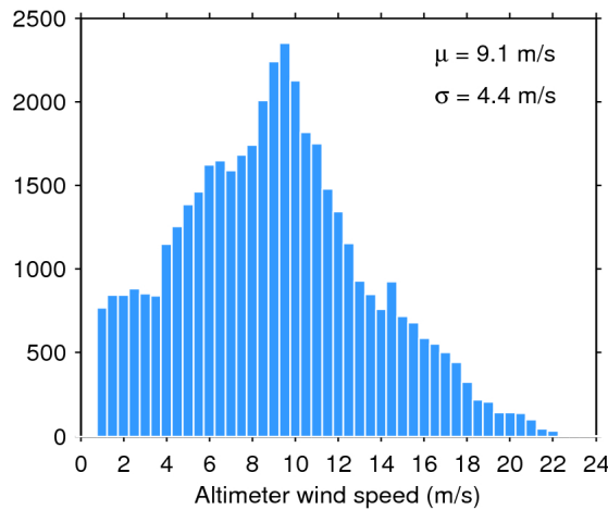
Figure 33. Histogram of flag-valid wind over oceans and lakes for 03/04/2017. The mean ( \mu ) and standard deviation ( \sigma ) are also shown. Note that values larger than 24 m/s are excluded from the histogram for the sake of readability but not from the computation of \mu and \sigma .
