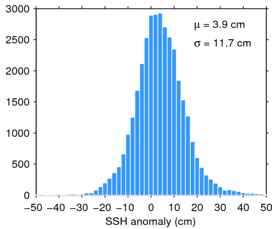
Figure 11. Histogram of science-valid SSH anomaly over oceans and lakes for 03/04/2017. The mean ( \mu ) and standard deviation ( \sigma ) are also shown. Note that values outside [-50 50] cm are excluded from the histogram for the sake of readability but not from the computation of \mu and \sigma .
