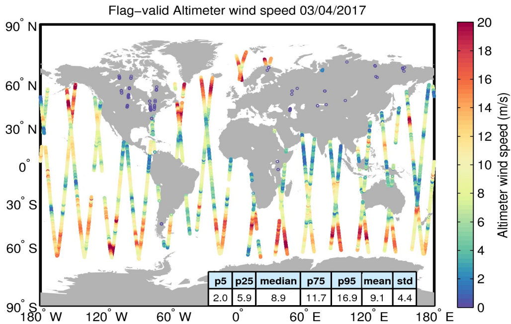
Figure 31. Geographical distribution of flag-valid wind data over oceans and lakes for 03/04/2017. The statistical values shown in the table refer to the wind in m/s and are calculated over all measurements shown in the figure.
