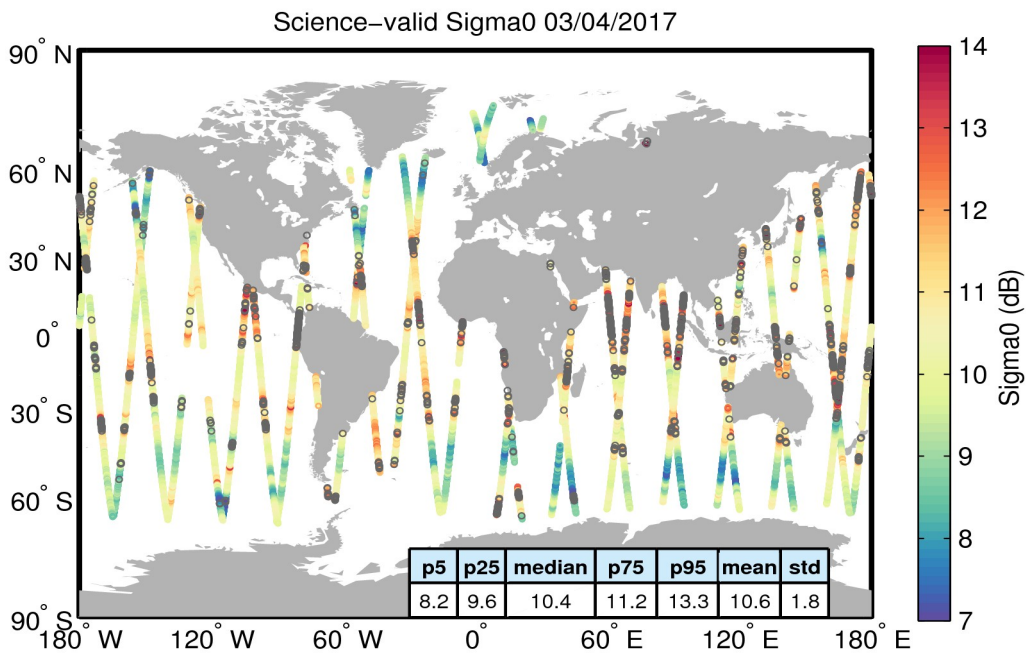
Figure 27. Geographical distribution of science-valid sigma0 data over oceans and lakes for 03/04/2017. The statistical values shown in the table refer to the sigma0 in dB and are calculated over all measurements shown in the figure. Gray circles denote records that have been rejected based on the editing criteria described in Table 4.
