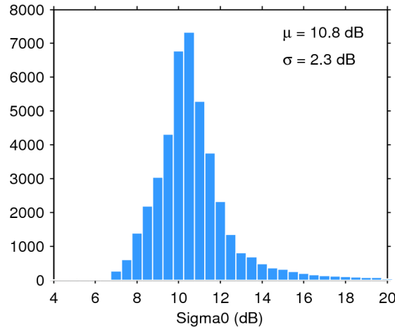
Figure 25. Histogram of flag-valid sigma0 over oceans and lakes for 03/04/2017. The mean ( \mu ) and standard deviation ( \sigma ) are also shown. Note that values outside [4 20] dB are excluded from the histogram for the sake of readability but not from the computation of \mu and \sigma .
