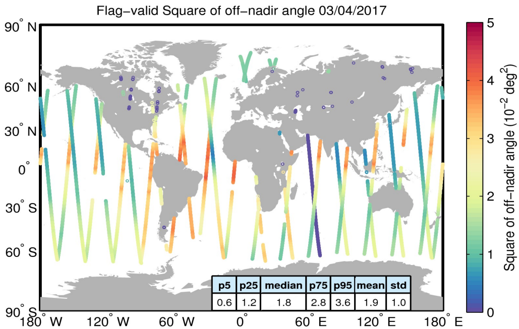
Figure 37. Geographical distribution of flag-valid mispointing data over oceans and lakes for 03/04/2017. The statistical values shown in the table refer to the mispointing in 10^{-2} deg 2 and are calculated over all measurements shown in the figure.
