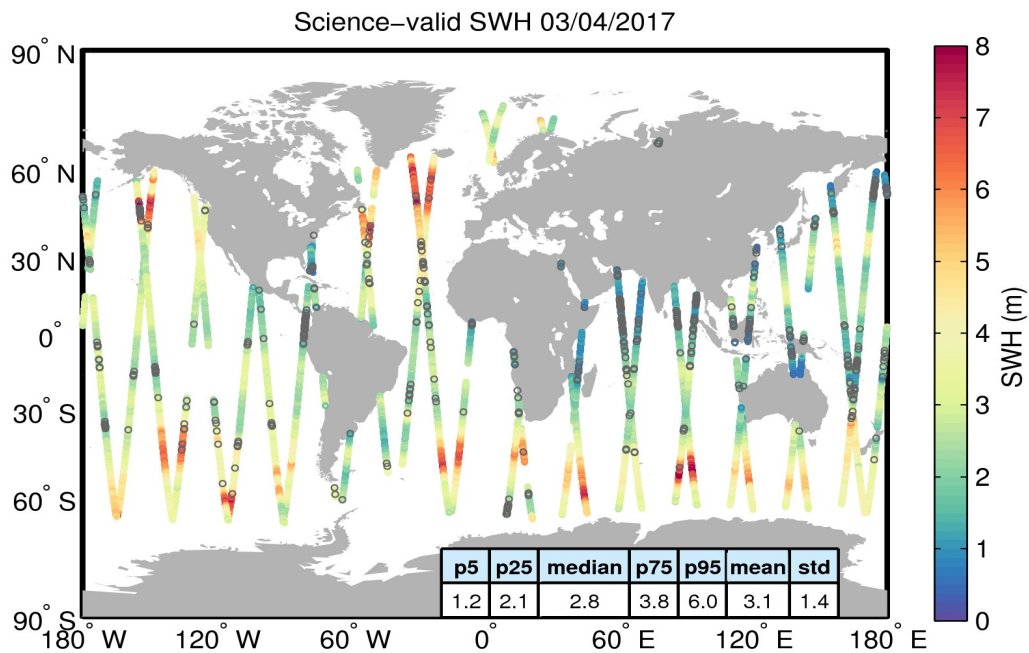
Figure 19. Geographical distribution of science-valid SWH data over oceans and lakes for 03/04/2017. The statistical values shown in the table refer to the SWH in m and are calculated over all measurements shown in the figure. Gray circles denote records that have been rejected based on the editing criteria described in Table 3.
