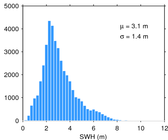
Figure 20. Histogram of science-valid SWH over oceans and lakes for 03/04/2017. The mean ( \mu ) and standard deviation ( \sigma ) are also shown. Note that values larger than 12 m are excluded from the histogram for the sake of readability but not from the computation of \mu and \sigma .
