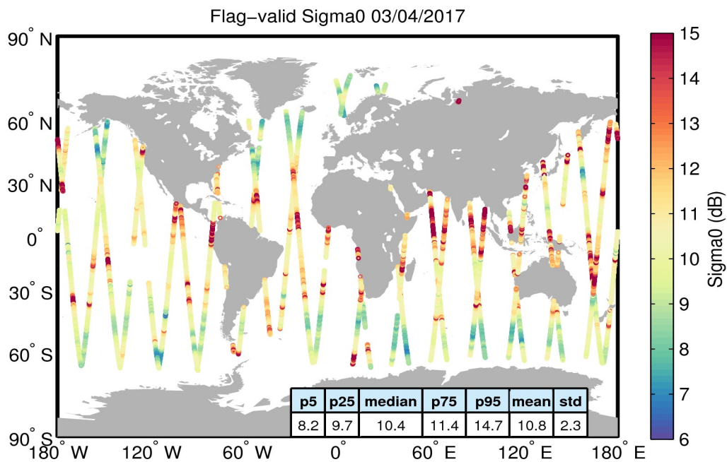
Figure 23. Geographical distribution of flag-valid sigma0 data over oceans and lakes for 03/04/2017. The statistical values shown in the table refer to the sigma0 in dB and are calculated over all measurements shown in the figure.
