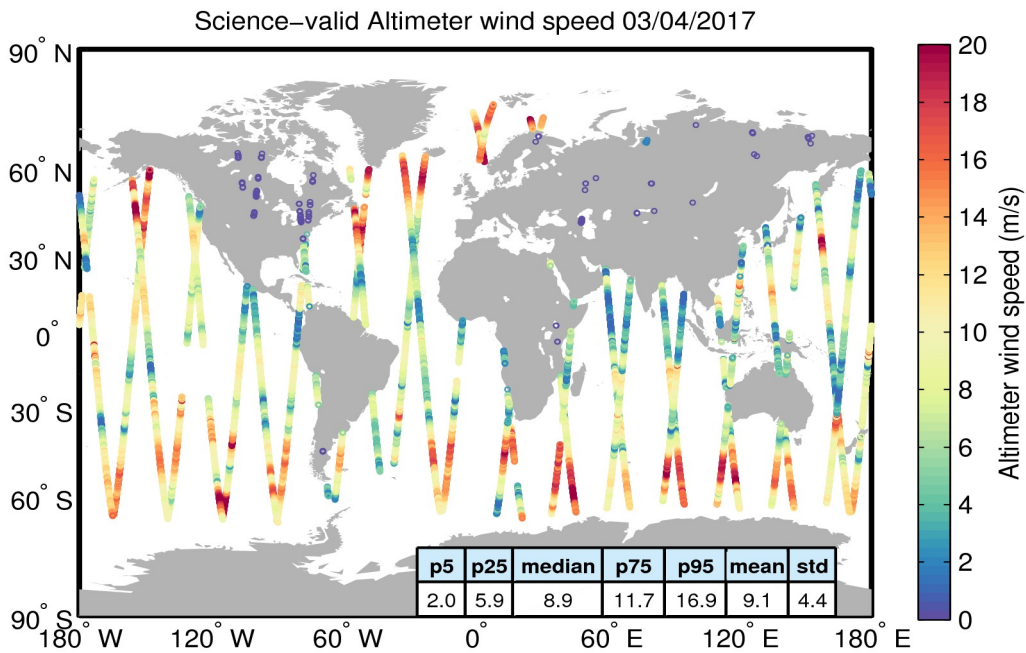
Figure 34. Geographical distribution of science-valid wind data over oceans and lakes for 03/04/2017. The statistical values shown in the table refer to the wind in m/s and are calculated over all measurements shown in the figure. Gray circles denote records that have been rejected based on the editing criteria described in Table 5.
