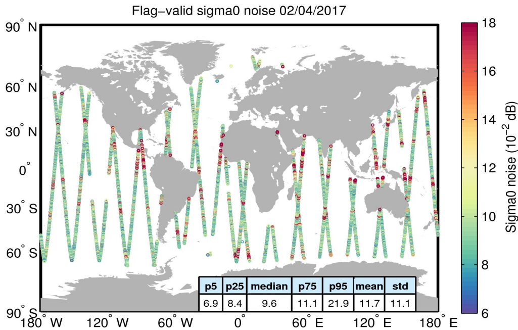
Figure 26. Geographical distribution of flag-valid 20-Hz sigma0 measurement noise over oceans and lakes for 02/04/2017. The statistical values shown in the table refer to the sigma0 noise and are calculated over all measurements shown in the figure.
