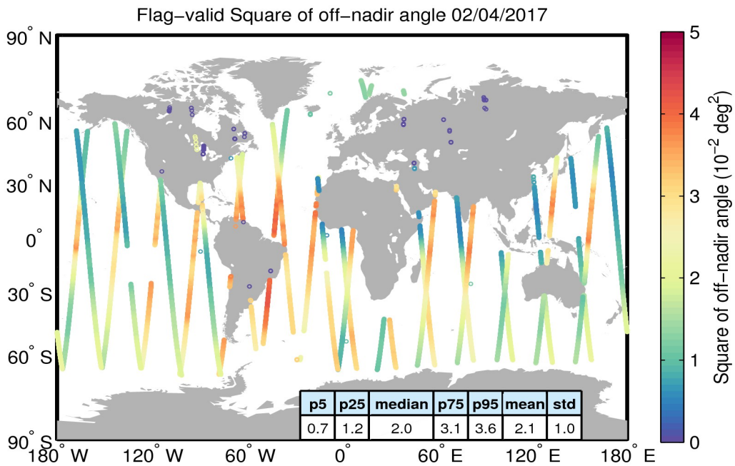
Figure 37. Geographical distribution of flag-valid mispointing data over oceans and lakes for 02/04/2017. The statistical values shown in the table refer to the mispointing in 10^{-2} deg 2 and are calculated over all measurements shown in the figure.
