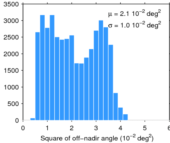
Figure 39. Histogram of flag-valid mispointing over oceans and lakes for 02/04/2017. The mean ( \mu ) and standard deviation ( \sigma ) are also shown. Note that values larger than 6 \cdot 10^{-2} \text{ deg}^2 are excluded from the histogram for the sake of readability but not from the computation of \mu and \sigma .
