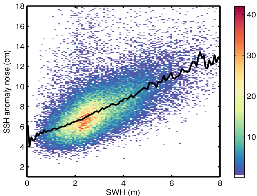
Figure 9. 2D histogram showing flag-valid SSH anomaly noise as a function of SWH for 02/04/2017. The black line denotes the median SSH anomaly noise as a function of SWH.
