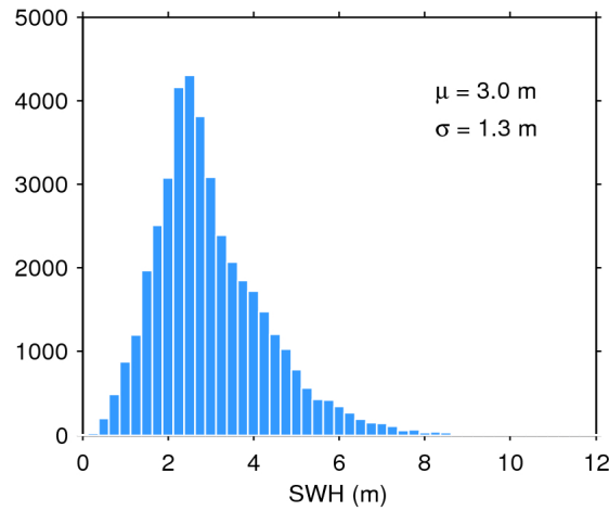
Figure 17. Histogram of flag-valid SWH over oceans and lakes for 02/04/2017. The mean ( \mu ) and standard deviation ( \sigma ) are also shown. Note that values larger than 12 m are excluded from the histogram for the sake of readability but not from the computation of \mu and \sigma .
