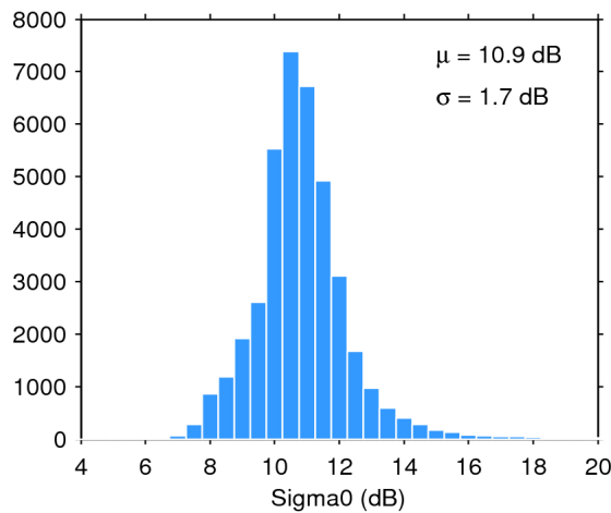
Figure 28. Histogram of science-valid sigma0 over oceans and lakes for 02/04/2017. The mean ( \mu ) and standard deviation ( \sigma ) are also shown. Note that values outside [4 20] dB are excluded from the histogram for the sake of readability but not from the computation of \mu and \sigma .
