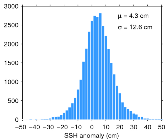
Figure 11. Histogram of science-valid SSH anomaly over oceans and lakes for 02/04/2017. The mean ( \mu ) and standard deviation ( \sigma ) are also shown. Note that values outside [-50 50] cm are excluded from the histogram for the sake of readability but not from the computation of \mu and \sigma .
