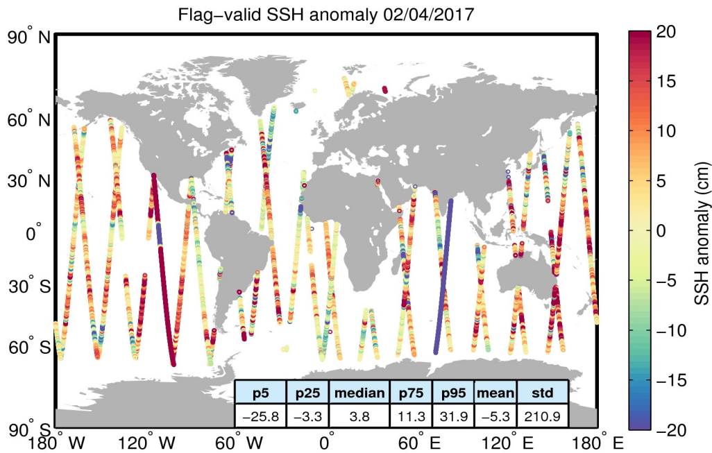
Figure 5. Geographical distribution of flag-valid 1-Hz SSH anomaly data over oceans and lakes for 02/04/2017. The statistical values shown in the table refer to the SSH anomaly in cm and are calculated over all measurements shown in the figure.
