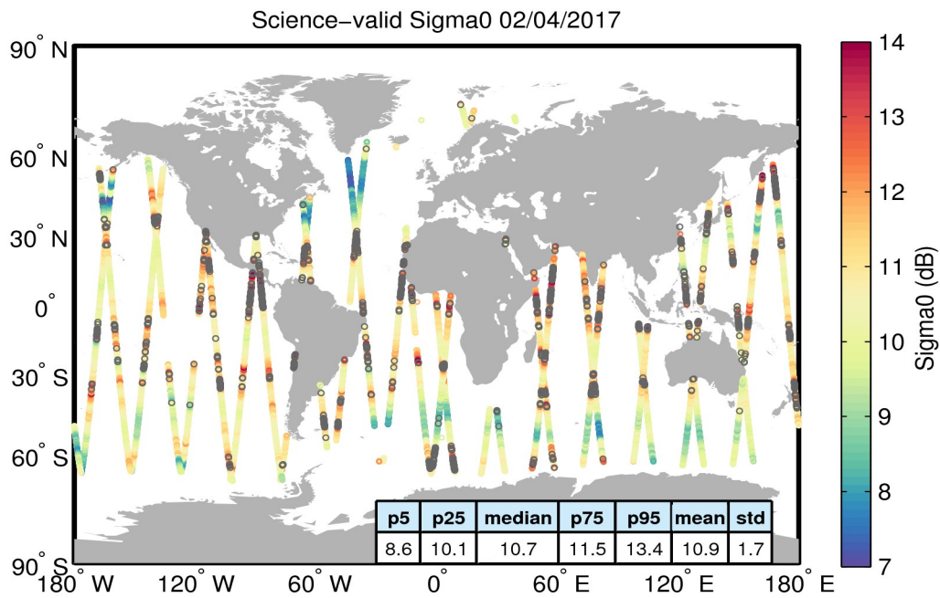
Figure 27. Geographical distribution of science-valid sigma0 data over oceans and lakes for 02/04/2017. The statistical values shown in the table refer to the sigma0 in dB and are calculated over all measurements shown in the figure. Gray circles denote records that have been rejected based on the editing criteria described in Table 4.
