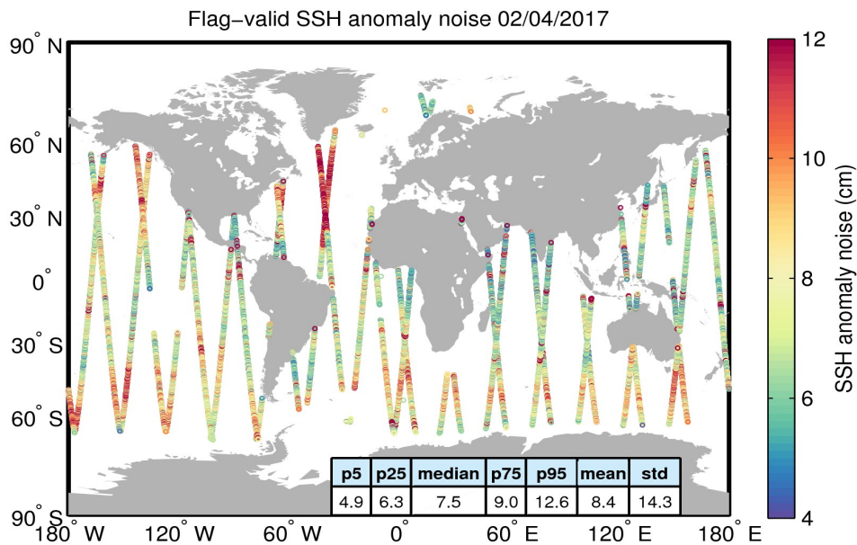
Figure 8. Geographical distribution of flag-valid 20-Hz SSH anomaly measurement noise over oceans and lakes for 02/04/2017. The statistical values shown in the table refer to the SSH anomaly noise and are calculated over all measurements shown in the figure.
