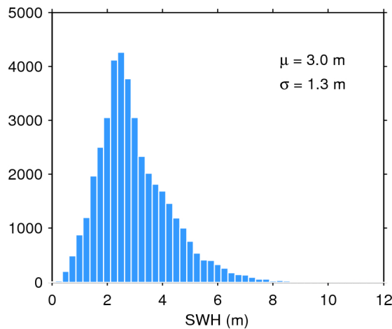
Figure 20. Histogram of science-valid SWH over oceans and lakes for 02/04/2017. The mean ( \mu ) and standard deviation ( \sigma ) are also shown. Note that values larger than 12 m are excluded from the histogram for the sake of readability but not from the computation of \mu and \sigma .
