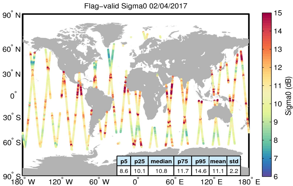
Figure 23. Geographical distribution of flag-valid sigma0 data over oceans and lakes for 02/04/2017. The statistical values shown in the table refer to the sigma0 in dB and are calculated over all measurements shown in the figure.
