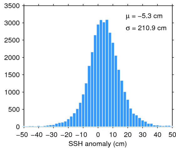
Figure 7. Histogram of flag-valid SSH anomaly over oceans and lakes for 02/04/2017. The mean ( \mu ) and standard deviation ( \sigma ) are also shown. Note that values outside [-50 50] cm are excluded from the histogram for the sake of readability but not from the computation of \mu and \sigma .
