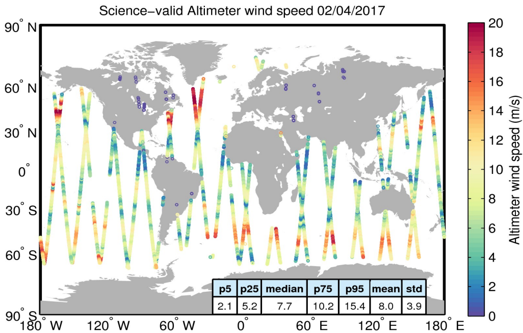
Figure 34. Geographical distribution of science-valid wind data over oceans and lakes for 02/04/2017. The statistical values shown in the table refer to the wind in m/s and are calculated over all measurements shown in the figure. Gray circles denote records that have been rejected based on the editing criteria described in Table 5.
