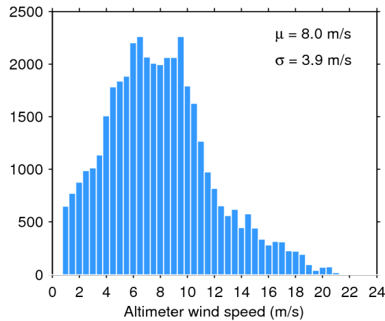
Figure 33. Histogram of flag-valid wind over oceans and lakes for 02/04/2017. The mean ( \mu ) and standard deviation ( \sigma ) are also shown. Note that values larger than 24 m/s are excluded from the histogram for the sake of readability but not from the computation of \mu and \sigma .
