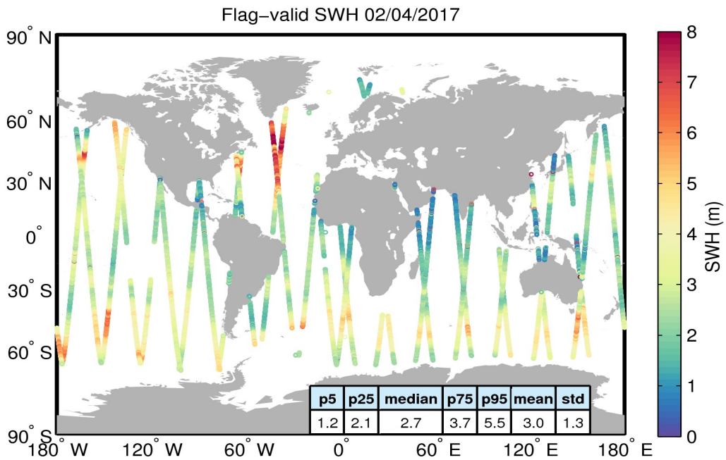
Figure 15. Geographical distribution of flag-valid SWH data over oceans and lakes for 02/04/2017. The statistical values shown in the table refer to the SWH in m and are calculated over all measurements shown in the figure.
