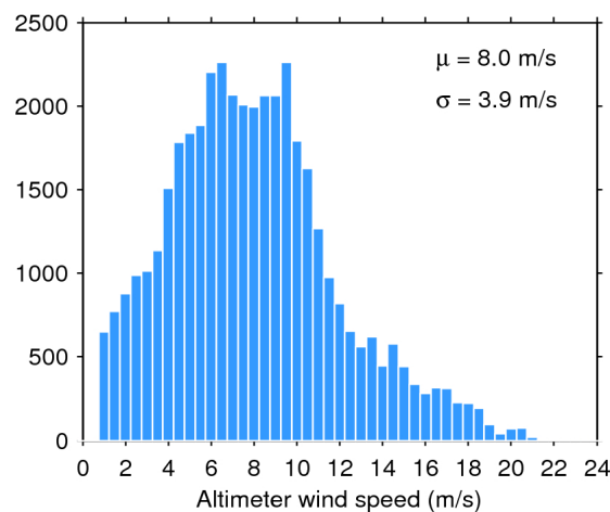
Figure 35. Histogram of science-valid wind over oceans and lakes for 02/04/2017. The mean ( \mu ) and standard deviation ( \sigma ) are also shown. Note that values larger than 24 m/s are excluded from the histogram for the sake of readability but not from the computation of \mu and \sigma .
