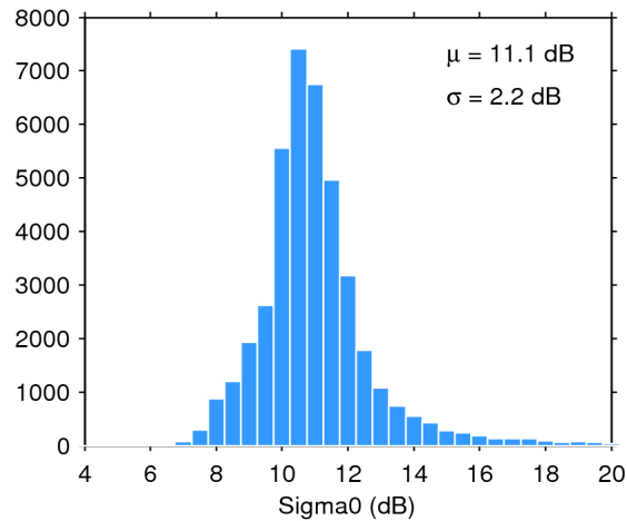
Figure 25. Histogram of flag-valid sigma0 over oceans and lakes for 02/04/2017. The mean ( \mu ) and standard deviation ( \sigma ) are also shown. Note that values outside [4 20] dB are excluded from the histogram for the sake of readability but not from the computation of \mu and \sigma .
