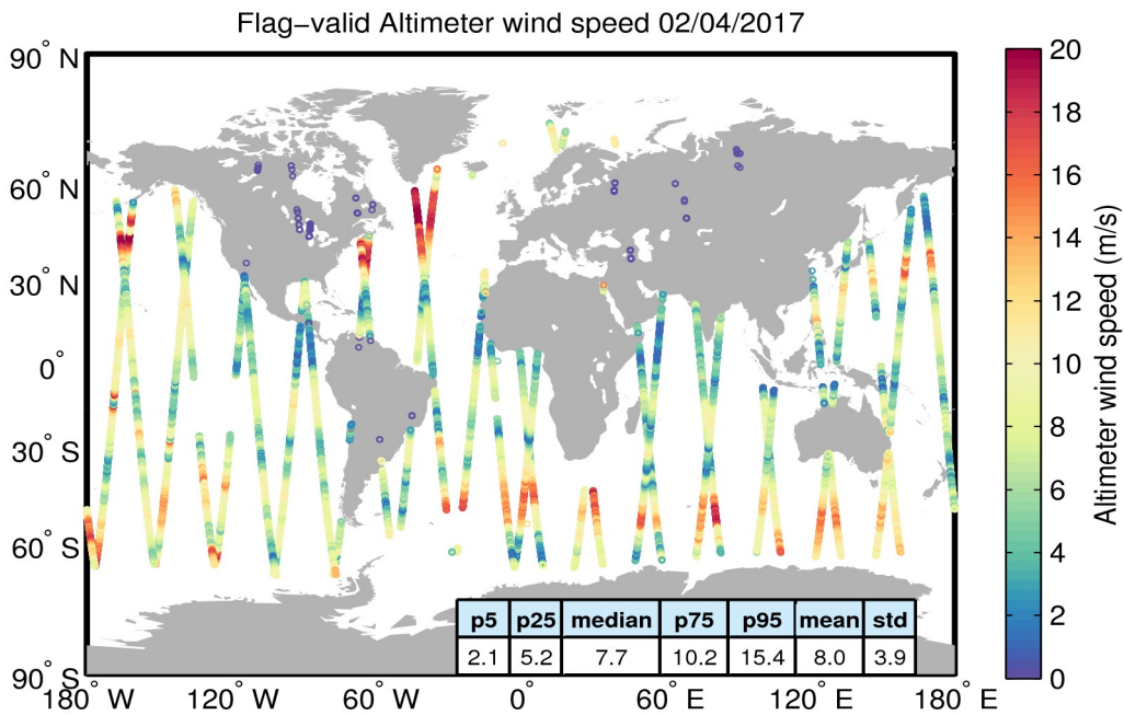
Figure 31. Geographical distribution of flag-valid wind data over oceans and lakes for 02/04/2017. The statistical values shown in the table refer to the wind in m/s and are calculated over all measurements shown in the figure.
