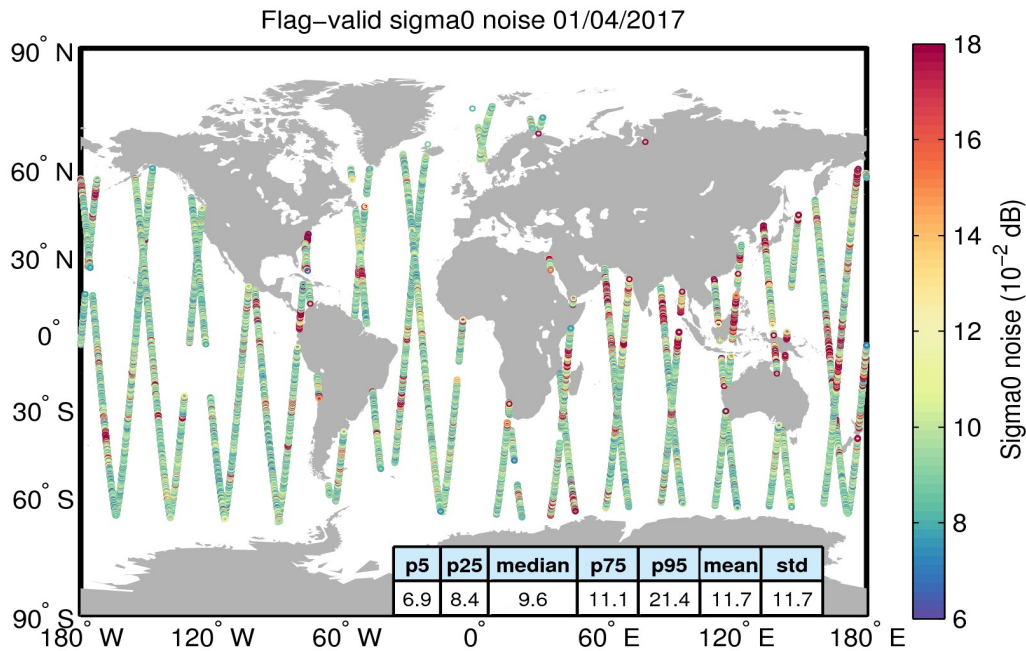
Figure 26. Geographical distribution of flag-valid 20-Hz sigma0 measurement noise over oceans and lakes for 01/04/2017. The statistical values shown in the table refer to the sigma0 noise and are calculated over all measurements shown in the figure.
