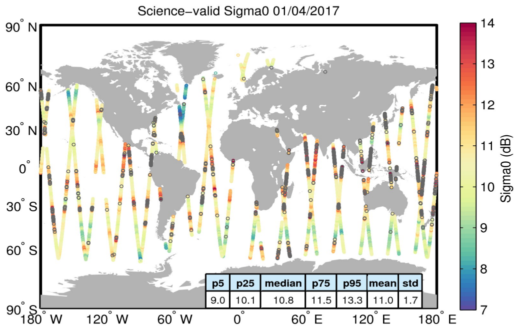
Figure 27. Geographical distribution of science-valid sigma0 data over oceans and lakes for 01/04/2017. The statistical values shown in the table refer to the sigma0 in dB and are calculated over all measurements shown in the figure. Gray circles denote records that have been rejected based on the editing criteria described in Table 4.
