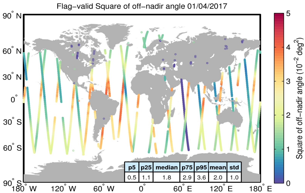
Figure 37. Geographical distribution of flag-valid mispointing data over oceans and lakes for 01/04/2017. The statistical values shown in the table refer to the mispointing in 10^{-2} deg 2 and are calculated over all measurements shown in the figure.
