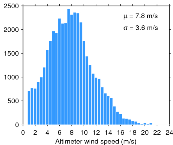
Figure 35. Histogram of science-valid wind over oceans and lakes for 01/04/2017. The mean ( \mu ) and standard deviation ( \sigma ) are also shown. Note that values larger than 24 m/s are excluded from the histogram for the sake of readability but not from the computation of \mu and \sigma .
