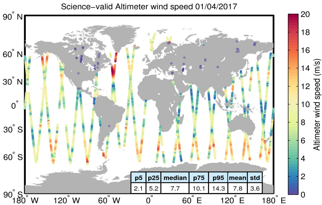
Figure 34. Geographical distribution of science-valid wind data over oceans and lakes for 01/04/2017. The statistical values shown in the table refer to the wind in m/s and are calculated over all measurements shown in the figure. Gray circles denote records that have been rejected based on the editing criteria described in Table 5.
