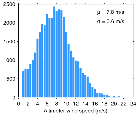
Figure 33. Histogram of flag-valid wind over oceans and lakes for 01/04/2017. The mean ( \mu ) and standard deviation ( \sigma ) are also shown. Note that values larger than 24 m/s are excluded from the histogram for the sake of readability but not from the computation of \mu and \sigma .
