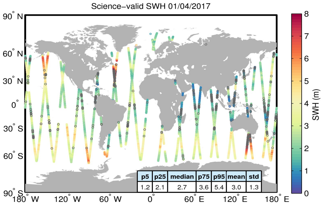
Figure 19. Geographical distribution of science-valid SWH data over oceans and lakes for 01/04/2017. The statistical values shown in the table refer to the SWH in m and are calculated over all measurements shown in the figure. Gray circles denote records that have been rejected based on the editing criteria described in Table 3.
