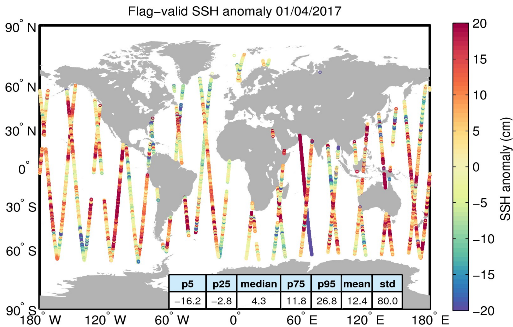
Figure 5. Geographical distribution of flag-valid 1-Hz SSH anomaly data over oceans and lakes for 01/04/2017. The statistical values shown in the table refer to the SSH anomaly in cm and are calculated over all measurements shown in the figure.
