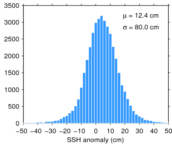
Figure 7. Histogram of flag-valid SSH anomaly over oceans and lakes for 01/04/2017. The mean ( \mu ) and standard deviation ( \sigma ) are also shown. Note that values outside [-50\ 50] cm are excluded from the histogram for the sake of readability but not from the computation of \mu and \sigma .
