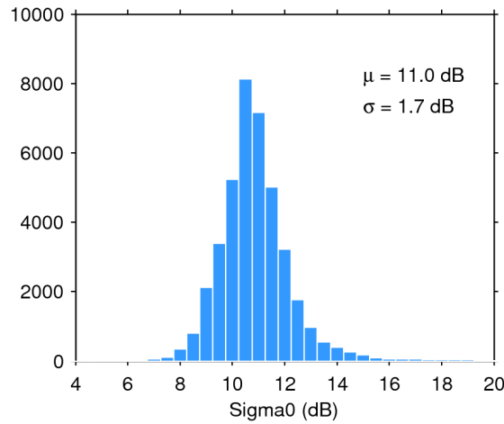
Figure 28. Histogram of science-valid sigma0 over oceans and lakes for 01/04/2017. The mean ( \mu ) and standard deviation ( \sigma ) are also shown. Note that values outside [4 20] dB are excluded from the histogram for the sake of readability but not from the computation of \mu and \sigma .
