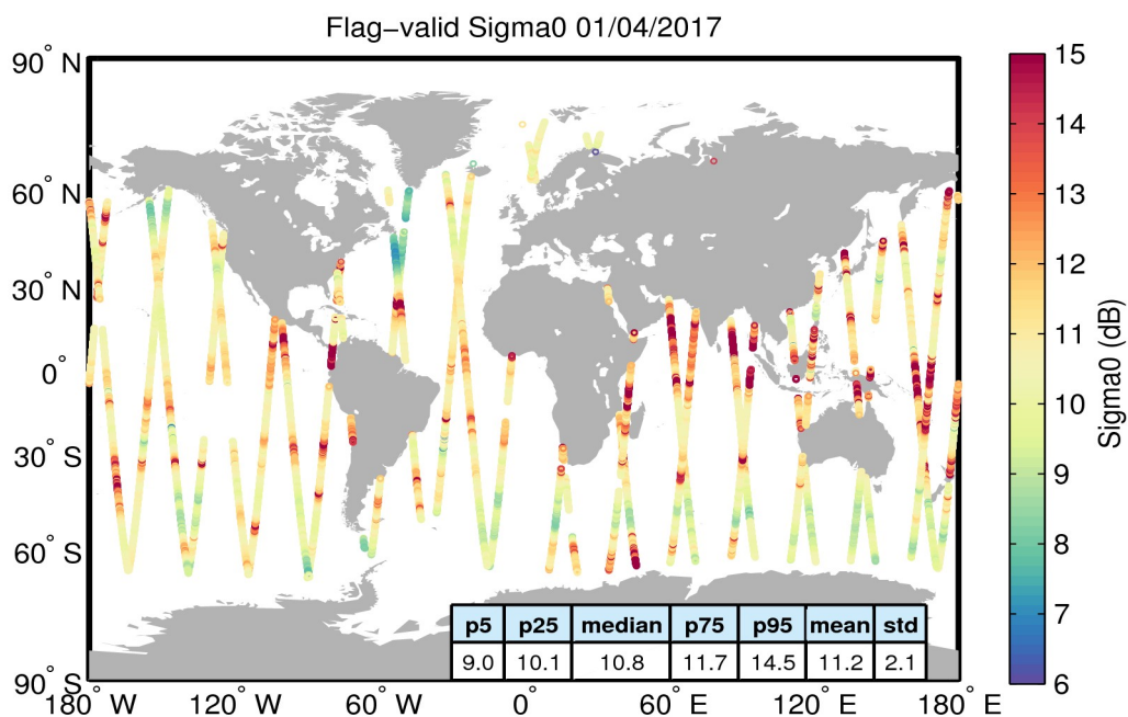
Figure 23. Geographical distribution of flag-valid sigma0 data over oceans and lakes for 01/04/2017. The statistical values shown in the table refer to the sigma0 in dB and are calculated over all measurements shown in the figure.
