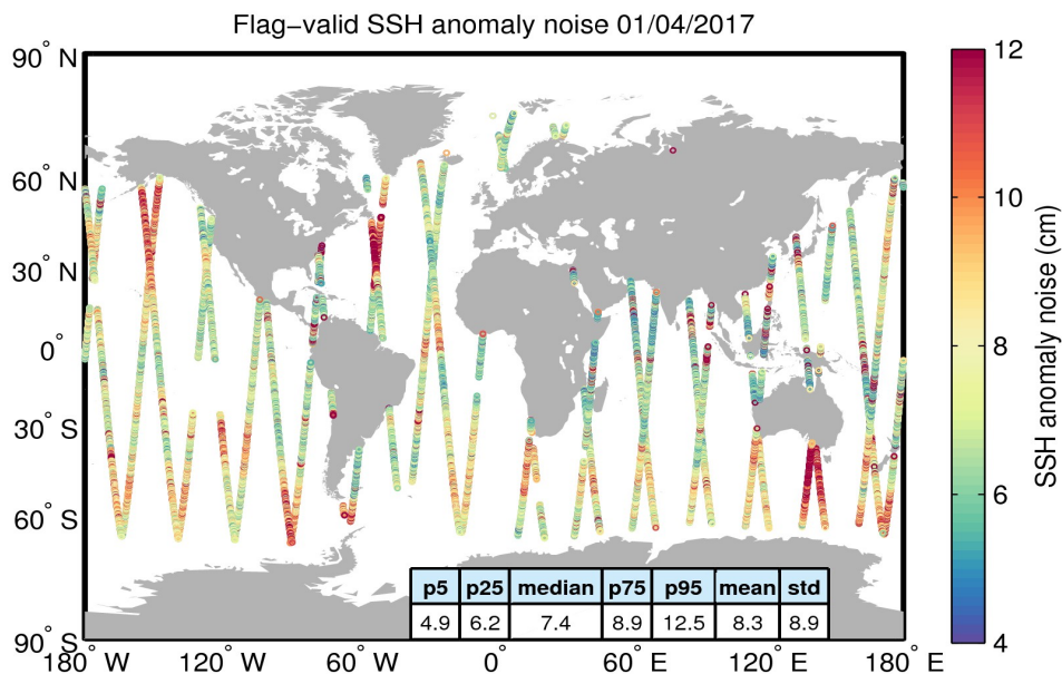
Figure 8. Geographical distribution of flag-valid 20-Hz SSH anomaly measurement noise over oceans and lakes for 01/04/2017. The statistical values shown in the table refer to the SSH anomaly noise and are calculated over all measurements shown in the figure.
