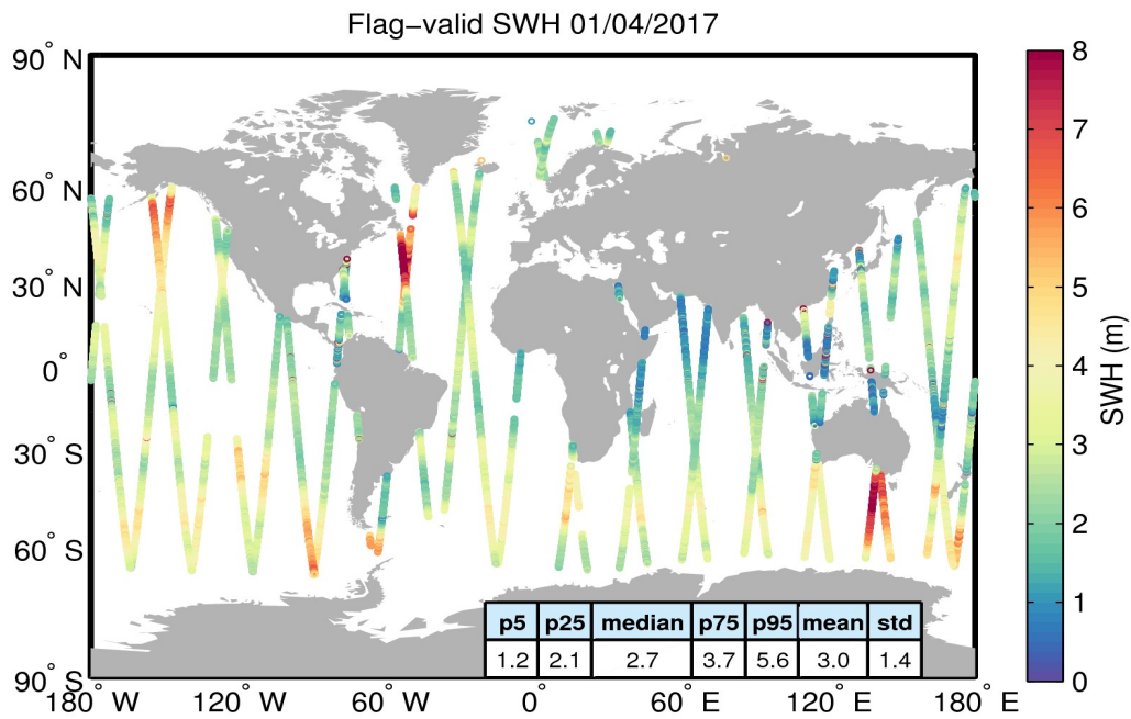
Figure 15. Geographical distribution of flag-valid SWH data over oceans and lakes for 01/04/2017. The statistical values shown in the table refer to the SWH in m and are calculated over all measurements shown in the figure.
