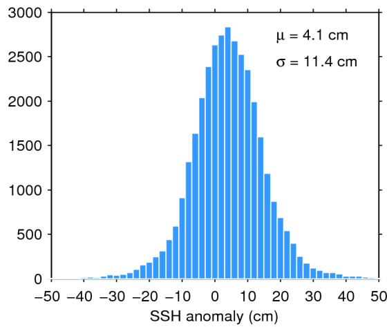
Figure 11. Histogram of science-valid SSH anomaly over oceans and lakes for 01/04/2017. The mean ( \mu ) and standard deviation ( \sigma ) are also shown. Note that values outside [-50 50] cm are excluded from the histogram for the sake of readability but not from the computation of \mu and \sigma .
