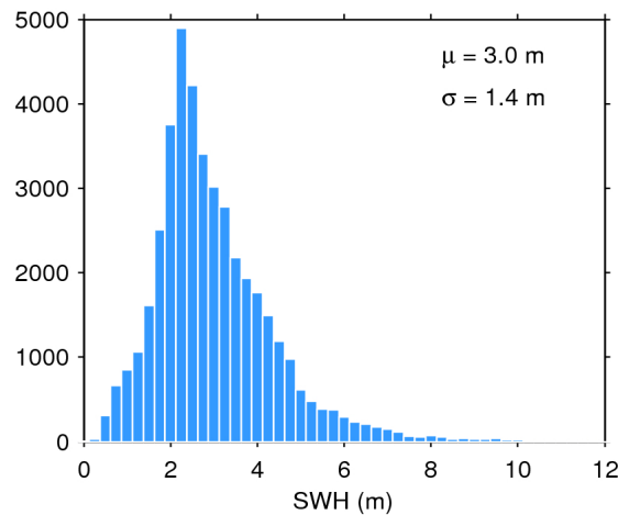
Figure 17. Histogram of flag-valid SWH over oceans and lakes for 01/04/2017. The mean ( \mu ) and standard deviation ( \sigma ) are also shown. Note that values larger than 12 m are excluded from the histogram for the sake of readability but not from the computation of \mu and \sigma .
