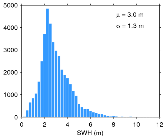
Figure 20. Histogram of science-valid SWH over oceans and lakes for 01/04/2017. The mean ( \mu ) and standard deviation ( \sigma ) are also shown. Note that values larger than 12 m are excluded from the histogram for the sake of readability but not from the computation of \mu and \sigma .
