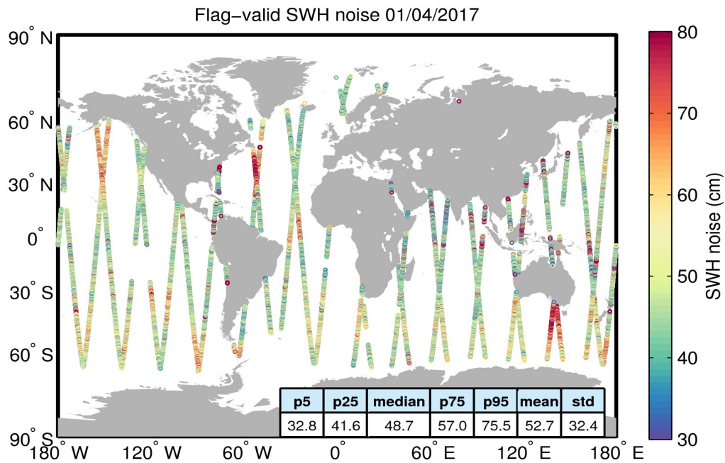
Figure 18. Geographical distribution of flag-valid 20-Hz SWH measurement noise over oceans and lakes for 01/04/2017. The statistical values shown in the table refer to the SWH noise and are calculated over all measurements shown in the figure.
