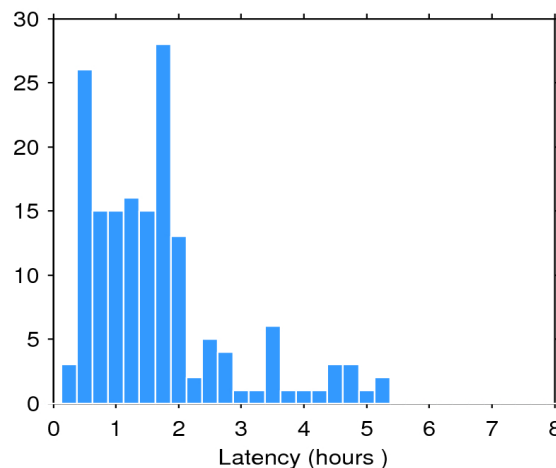
Figure 2. Histogram of the data latency for 01/04/2017. The y-axis denotes the number of files that are made available with a delay of x-hours with respect to the mean time of the records stored in the file.
