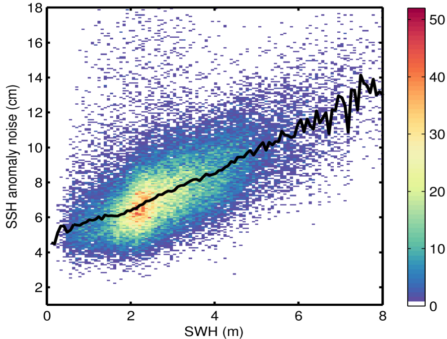
Figure 9. 2D histogram showing flag-valid SSH anomaly noise as a function of SWH for 01/04/2017. The black line denotes the median SSH anomaly noise as a function of SWH.
