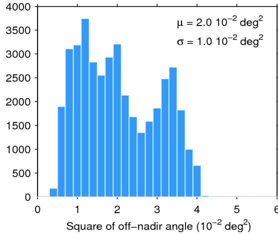
Figure 39. Histogram of flag-valid mispointing over oceans and lakes for 01/04/2017. The mean ( \mu ) and standard deviation ( \sigma ) are also shown. Note that values larger than 6 \cdot 10^{-2} \text{ deg}^2 are excluded from the histogram for the sake of readability but not from the computation of \mu and \sigma .
