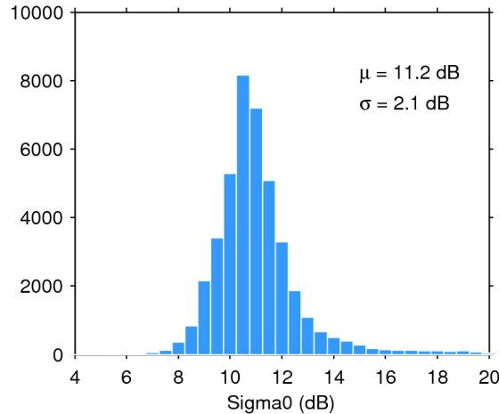
Figure 25. Histogram of flag-valid sigma0 over oceans and lakes for 01/04/2017. The mean ( \mu ) and standard deviation ( \sigma ) are also shown. Note that values outside [4 20] dB are excluded from the histogram for the sake of readability but not from the computation of \mu and \sigma .
