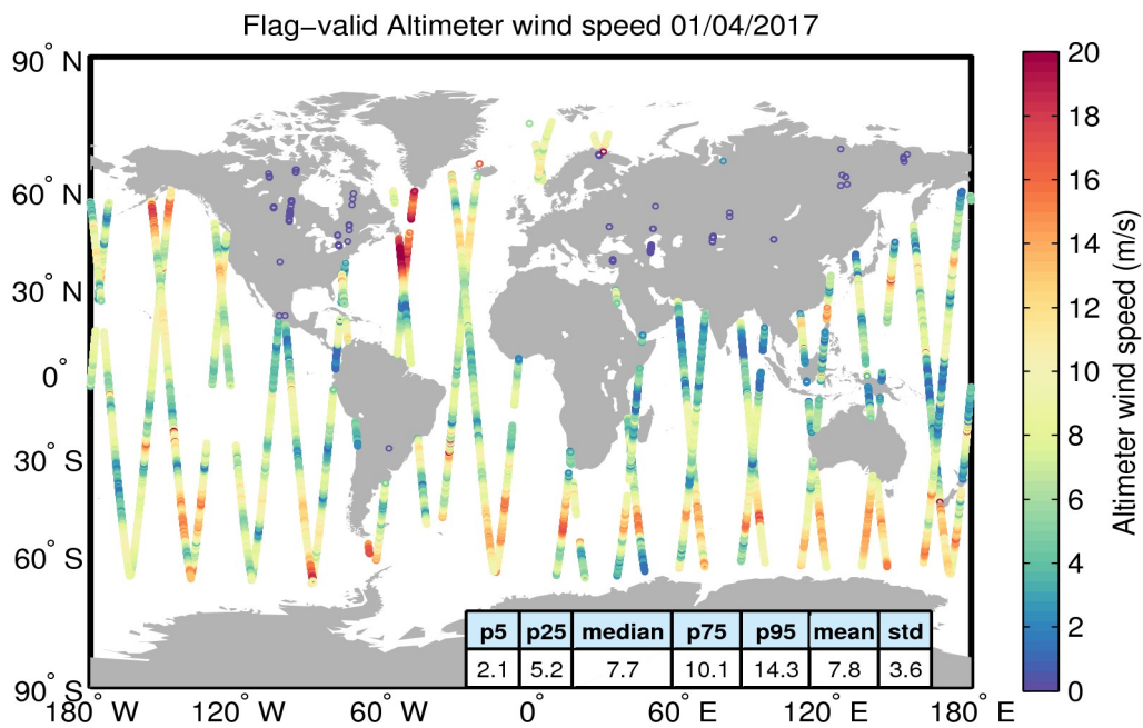
Figure 31. Geographical distribution of flag-valid wind data over oceans and lakes for 01/04/2017. The statistical values shown in the table refer to the wind in m/s and are calculated over all measurements shown in the figure.
