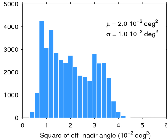
Figure 39. Histogram of flag-valid mispointing over oceans and lakes for 31/03/2017. The mean ( \mu ) and standard deviation ( \sigma ) are also shown. Note that values larger than 6 \cdot 10^{-2} \text{ deg}^2 are excluded from the histogram for the sake of readability but not from the computation of \mu and \sigma .
