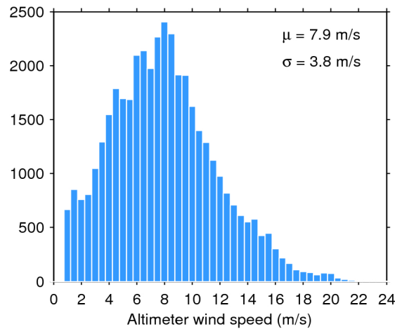
Figure 33. Histogram of flag-valid wind over oceans and lakes for 31/03/2017. The mean ( \mu ) and standard deviation ( \sigma ) are also shown. Note that values larger than 24 m/s are excluded from the histogram for the sake of readability but not from the computation of \mu and \sigma .
