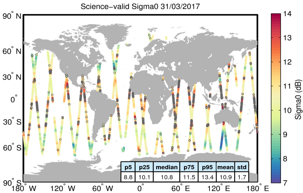
Figure 27. Geographical distribution of science-valid sigma0 data over oceans and lakes for 31/03/2017. The statistical values shown in the table refer to the sigma0 in dB and are calculated over all measurements shown in the figure. Gray circles denote records that have been rejected based on the editing criteria described in Table 4.
