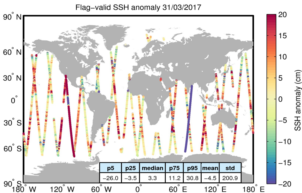
Figure 5. Geographical distribution of flag-valid 1-Hz SSH anomaly data over oceans and lakes for 31/03/2017. The statistical values shown in the table refer to the SSH anomaly in cm and are calculated over all measurements shown in the figure.
