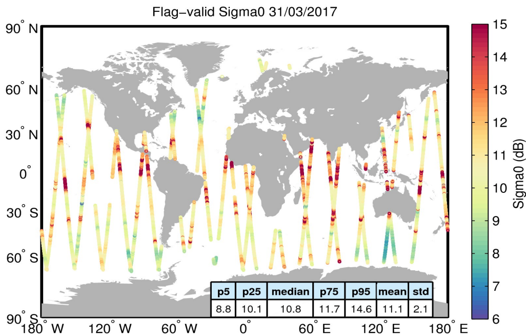
Figure 23. Geographical distribution of flag-valid sigma0 data over oceans and lakes for 31/03/2017. The statistical values shown in the table refer to the sigma0 in dB and are calculated over all measurements shown in the figure.
