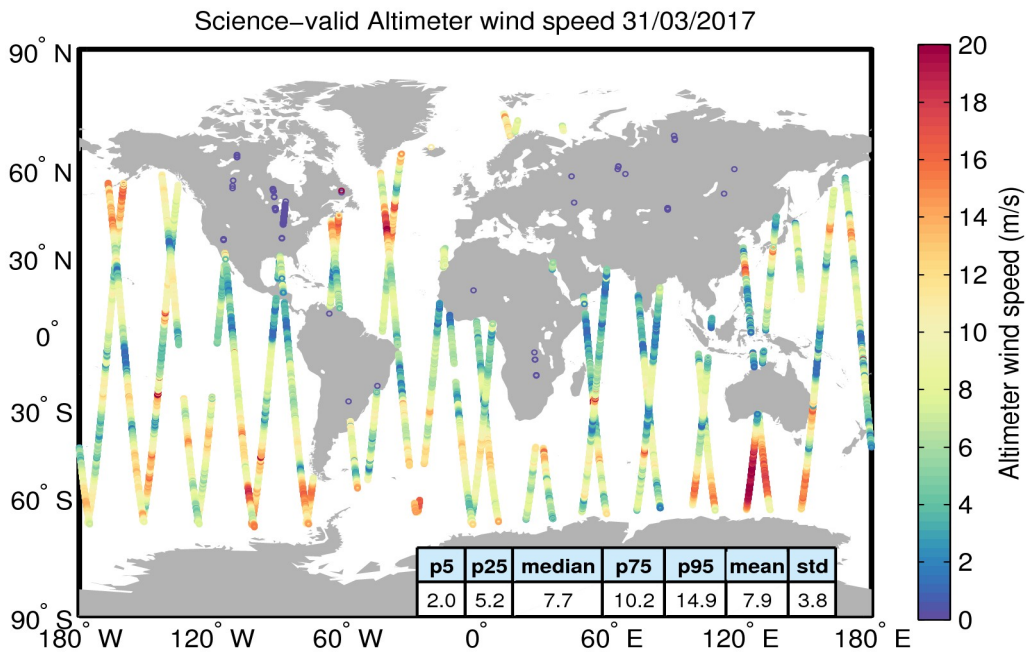
Figure 34. Geographical distribution of science-valid wind data over oceans and lakes for 31/03/2017. The statistical values shown in the table refer to the wind in m/s and are calculated over all measurements shown in the figure. Gray circles denote records that have been rejected based on the editing criteria described in Table 5.
