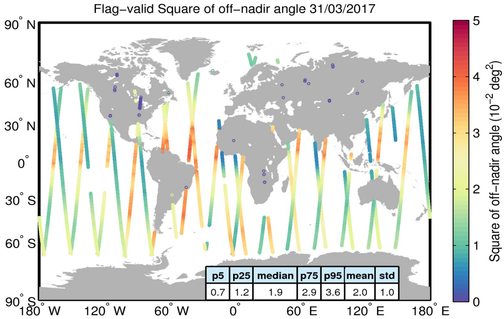
Figure 37. Geographical distribution of flag-valid mispointing data over oceans and lakes for 31/03/2017. The statistical values shown in the table refer to the mispointing in 10^{-2} deg 2 and are calculated over all measurements shown in the figure.
