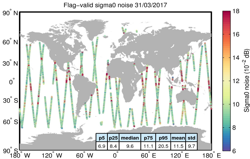
Figure 26. Geographical distribution of flag-valid 20-Hz sigma0 measurement noise over oceans and lakes for 31/03/2017. The statistical values shown in the table refer to the sigma0 noise and are calculated over all measurements shown in the figure.
