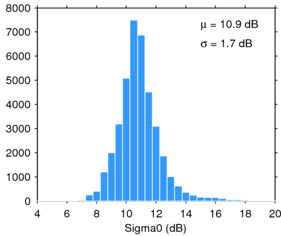
Figure 28. Histogram of science-valid sigma0 over oceans and lakes for 31/03/2017. The mean ( \mu ) and standard deviation ( \sigma ) are also shown. Note that values outside [4 20] dB are excluded from the histogram for the sake of readability but not from the computation of \mu and \sigma .
