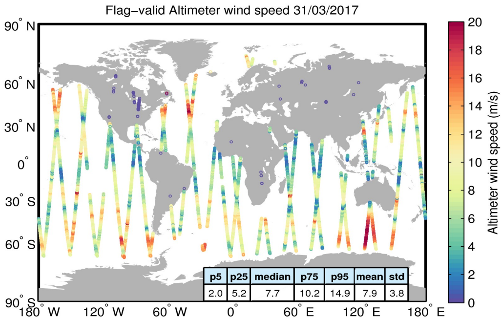
Figure 31. Geographical distribution of flag-valid wind data over oceans and lakes for 31/03/2017. The statistical values shown in the table refer to the wind in m/s and are calculated over all measurements shown in the figure.
