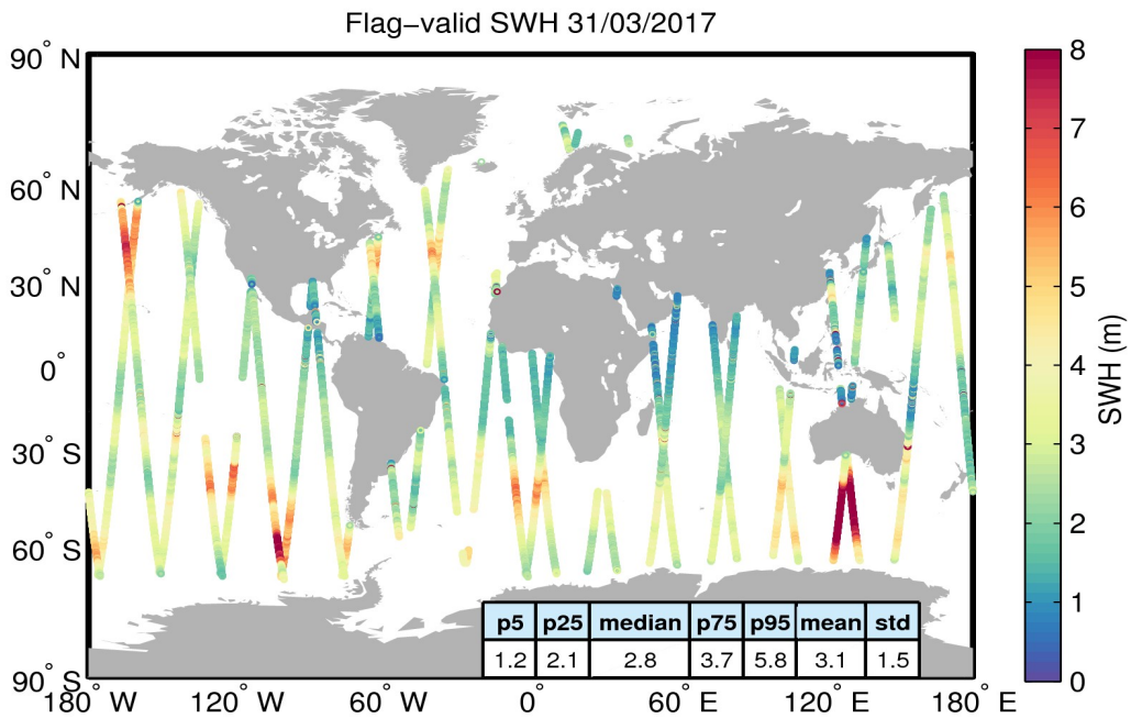
Figure 15. Geographical distribution of flag-valid SWH data over oceans and lakes for 31/03/2017. The statistical values shown in the table refer to the SWH in m and are calculated over all measurements shown in the figure.
