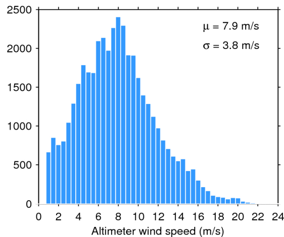
Figure 35. Histogram of science-valid wind over oceans and lakes for 31/03/2017. The mean ( \mu ) and standard deviation ( \sigma ) are also shown. Note that values larger than 24 m/s are excluded from the histogram for the sake of readability but not from the computation of \mu and \sigma .
