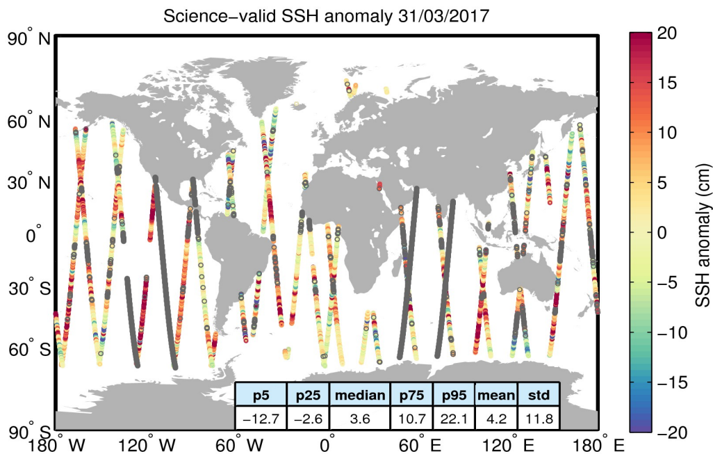
Figure 10. Geographical distribution of science-valid SSH anomaly data over oceans and lakes for 31/03/2017. The statistical values shown in the table refer to the SSH anomaly in cm and are calculated over all measurements shown in the figure. Gray circles denote records that have been rejected based on the editing criteria described in Table 2.
