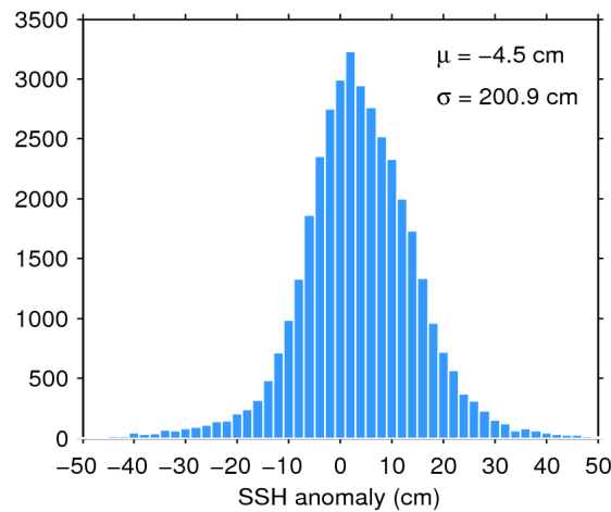
Figure 7. Histogram of flag-valid SSH anomaly over oceans and lakes for 31/03/2017. The mean ( \mu ) and standard deviation ( \sigma ) are also shown. Note that values outside [-50 50] cm are excluded from the histogram for the sake of readability but not from the computation of \mu and \sigma .
