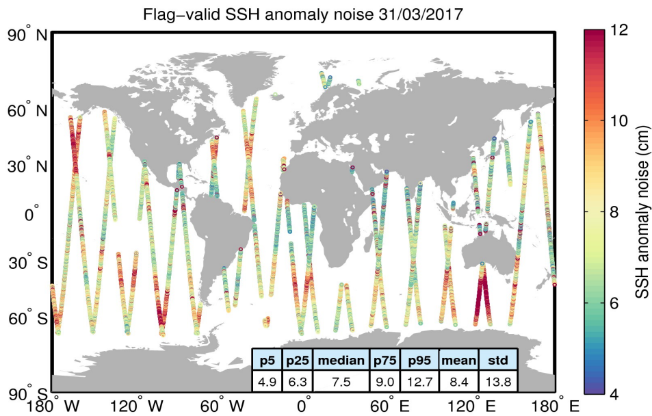
Figure 8. Geographical distribution of flag-valid 20-Hz SSH anomaly measurement noise over oceans and lakes for 31/03/2017. The statistical values shown in the table refer to the SSH anomaly noise and are calculated over all measurements shown in the figure.
