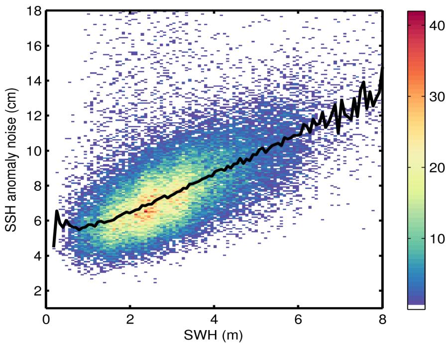
Figure 9. 2D histogram showing flag-valid SSH anomaly noise as a function of SWH for 31/03/2017. The black line denotes the median SSH anomaly noise as a function of SWH.
