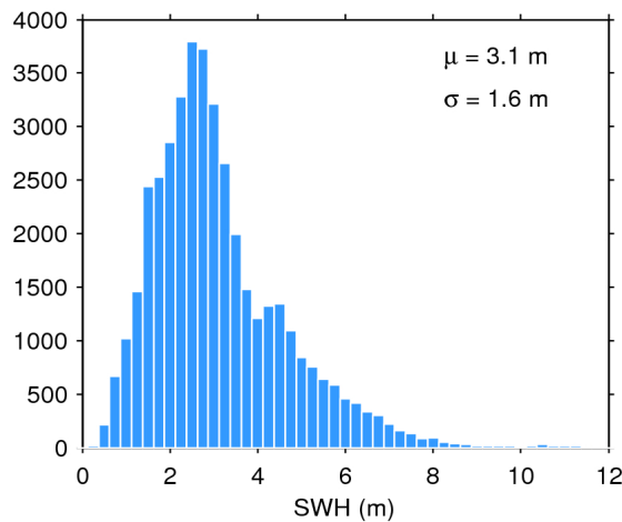
Figure 20. Histogram of science-valid SWH over oceans and lakes for 30/03/2017. The mean ( \mu ) and standard deviation ( \sigma ) are also shown. Note that values larger than 12 m are excluded from the histogram for the sake of readability but not from the computation of \mu and \sigma .
