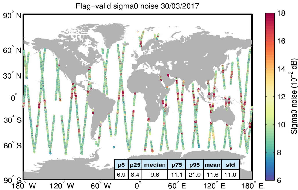
Figure 26. Geographical distribution of flag-valid 20-Hz sigma0 measurement noise over oceans and lakes for 30/03/2017. The statistical values shown in the table refer to the sigma0 noise and are calculated over all measurements shown in the figure.
