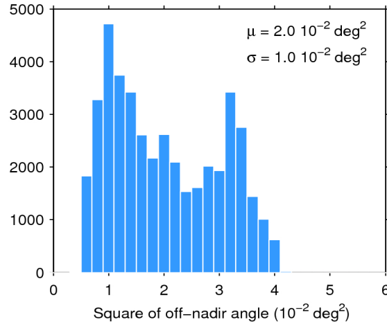
Figure 39. Histogram of flag-valid mispointing over oceans and lakes for 30/03/2017. The mean ( \mu ) and standard deviation ( \sigma ) are also shown. Note that values larger than 6 \cdot 10^{-2} \text{ deg}^2 are excluded from the histogram for the sake of readability but not from the computation of \mu and \sigma .
