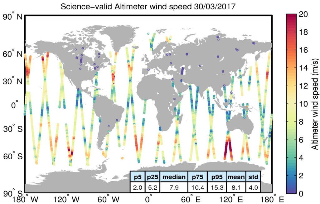
Figure 34. Geographical distribution of science-valid wind data over oceans and lakes for 30/03/2017. The statistical values shown in the table refer to the wind in m/s and are calculated over all measurements shown in the figure. Gray circles denote records that have been rejected based on the editing criteria described in Table 5.
