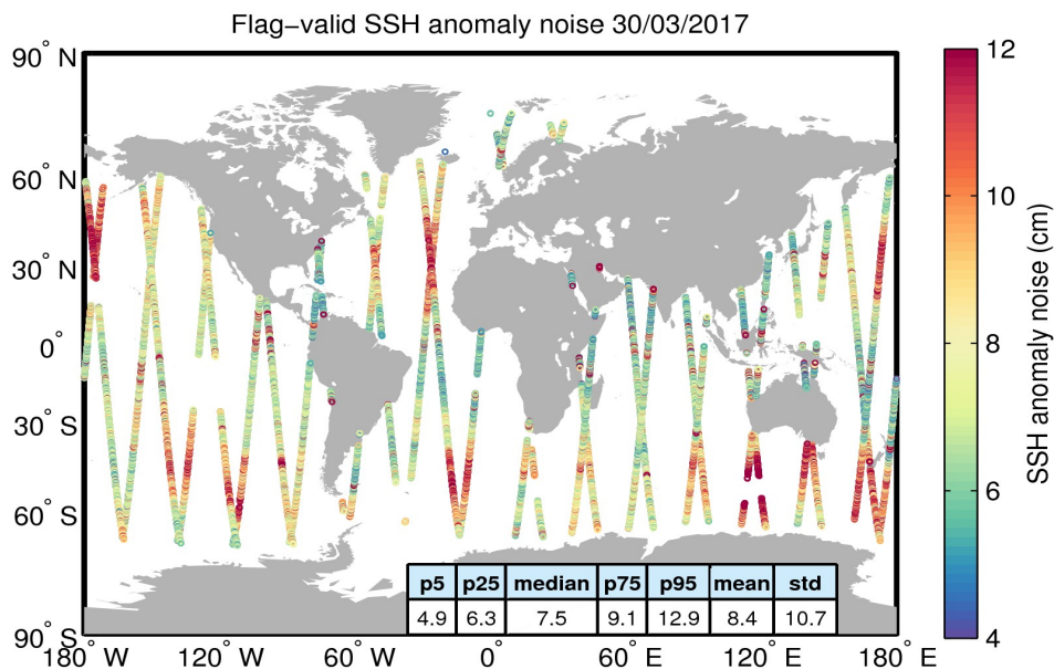
Figure 8. Geographical distribution of flag-valid 20-Hz SSH anomaly measurement noise over oceans and lakes for 30/03/2017. The statistical values shown in the table refer to the SSH anomaly noise and are calculated over all measurements shown in the figure.
