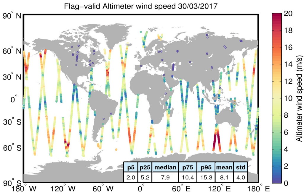
Figure 31. Geographical distribution of flag-valid wind data over oceans and lakes for 30/03/2017. The statistical values shown in the table refer to the wind in m/s and are calculated over all measurements shown in the figure.
