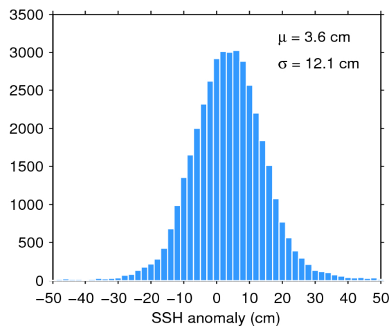
Figure 11. Histogram of science-valid SSH anomaly over oceans and lakes for 30/03/2017. The mean ( \mu ) and standard deviation ( \sigma ) are also shown. Note that values outside [-50 50] cm are excluded from the histogram for the sake of readability but not from the computation of \mu and \sigma .
