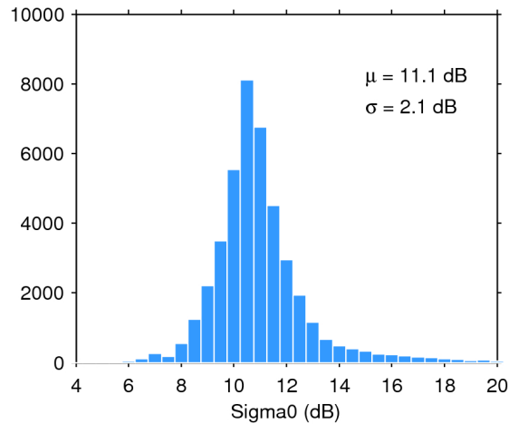
Figure 25. Histogram of flag-valid sigma0 over oceans and lakes for 30/03/2017. The mean ( \mu ) and standard deviation ( \sigma ) are also shown. Note that values outside [4 20] dB are excluded from the histogram for the sake of readability but not from the computation of \mu and \sigma .
