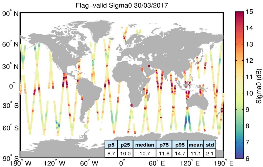
Figure 23. Geographical distribution of flag-valid sigma0 data over oceans and lakes for 30/03/2017. The statistical values shown in the table refer to the sigma0 in dB and are calculated over all measurements shown in the figure.
