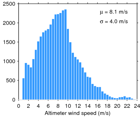
Figure 33. Histogram of flag-valid wind over oceans and lakes for 30/03/2017. The mean ( \mu ) and standard deviation ( \sigma ) are also shown. Note that values larger than 24 m/s are excluded from the histogram for the sake of readability but not from the computation of \mu and \sigma .
