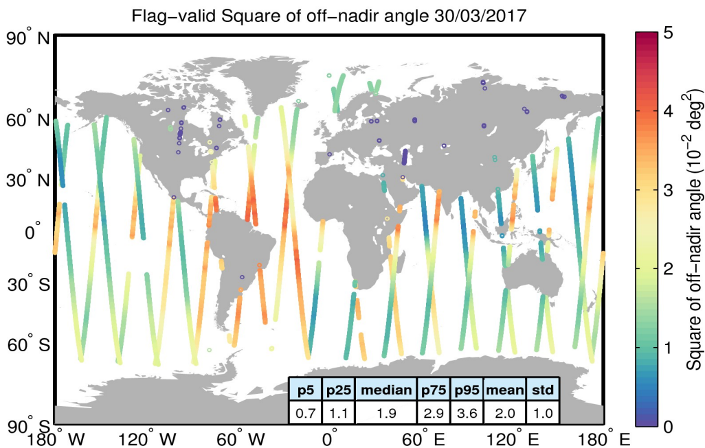
Figure 37. Geographical distribution of flag-valid mispointing data over oceans and lakes for 30/03/2017. The statistical values shown in the table refer to the mispointing in 10^{-2} deg 2 and are calculated over all measurements shown in the figure.
