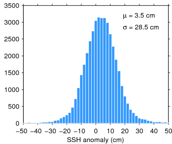
Figure 7. Histogram of flag-valid SSH anomaly over oceans and lakes for 30/03/2017. The mean ( \mu ) and standard deviation ( \sigma ) are also shown. Note that values outside [-50 50] cm are excluded from the histogram for the sake of readability but not from the computation of \mu and \sigma .
