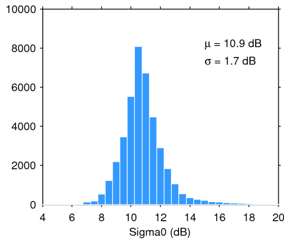
Figure 28. Histogram of science-valid sigma0 over oceans and lakes for 30/03/2017. The mean ( \mu ) and standard deviation ( \sigma ) are also shown. Note that values outside [4 20] dB are excluded from the histogram for the sake of readability but not from the computation of \mu and \sigma .
