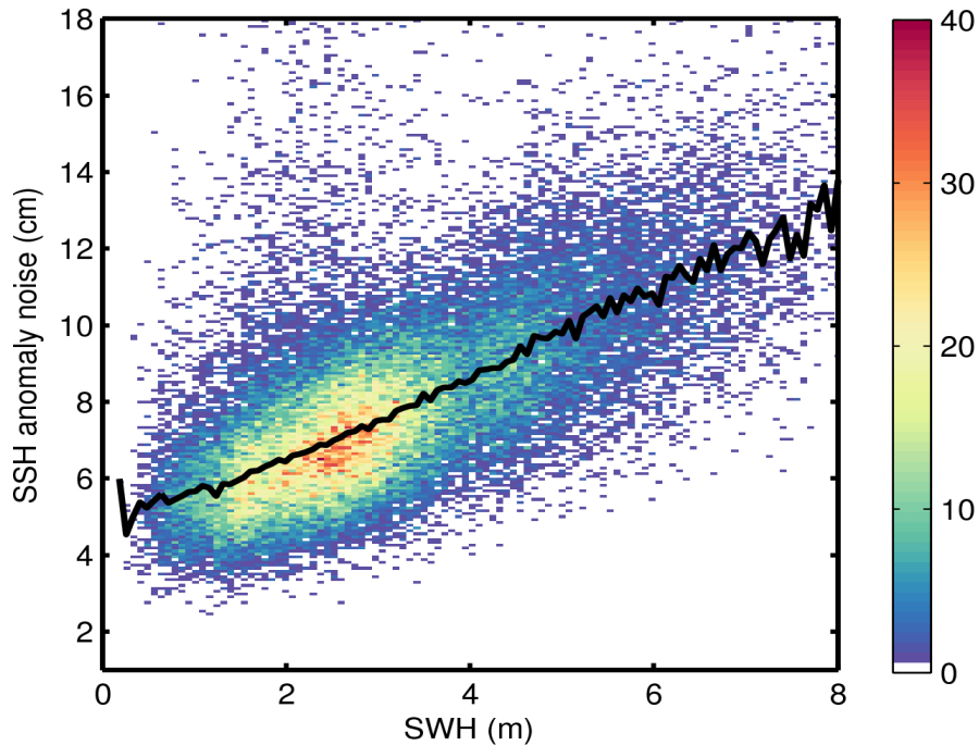
Figure 9. 2D histogram showing flag-valid SSH anomaly noise as a function of SWH for 30/03/2017. The black line denotes the median SSH anomaly noise as a function of SWH.
