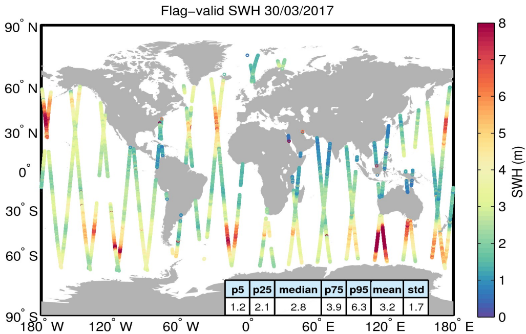
Figure 15. Geographical distribution of flag-valid SWH data over oceans and lakes for 30/03/2017. The statistical values shown in the table refer to the SWH in m and are calculated over all measurements shown in the figure.
