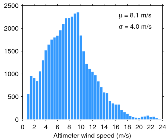
Figure 35. Histogram of science-valid wind over oceans and lakes for 30/03/2017. The mean ( \mu ) and standard deviation ( \sigma ) are also shown. Note that values larger than 24 m/s are excluded from the histogram for the sake of readability but not from the computation of \mu and \sigma .
