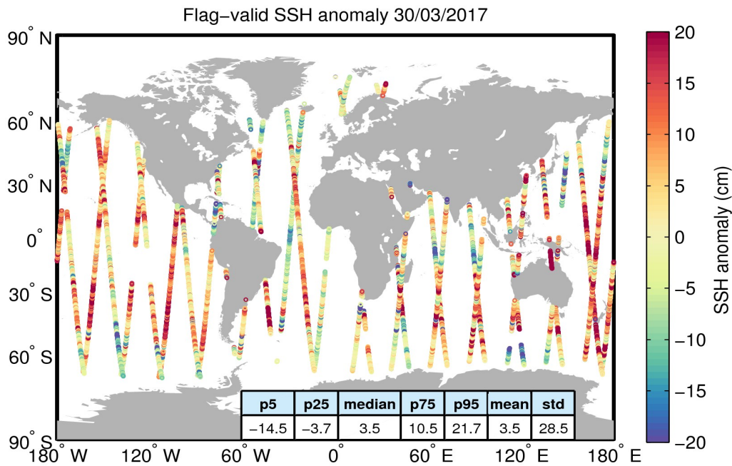
Figure 5. Geographical distribution of flag-valid 1-Hz SSH anomaly data over oceans and lakes for 30/03/2017. The statistical values shown in the table refer to the SSH anomaly in cm and are calculated over all measurements shown in the figure.
