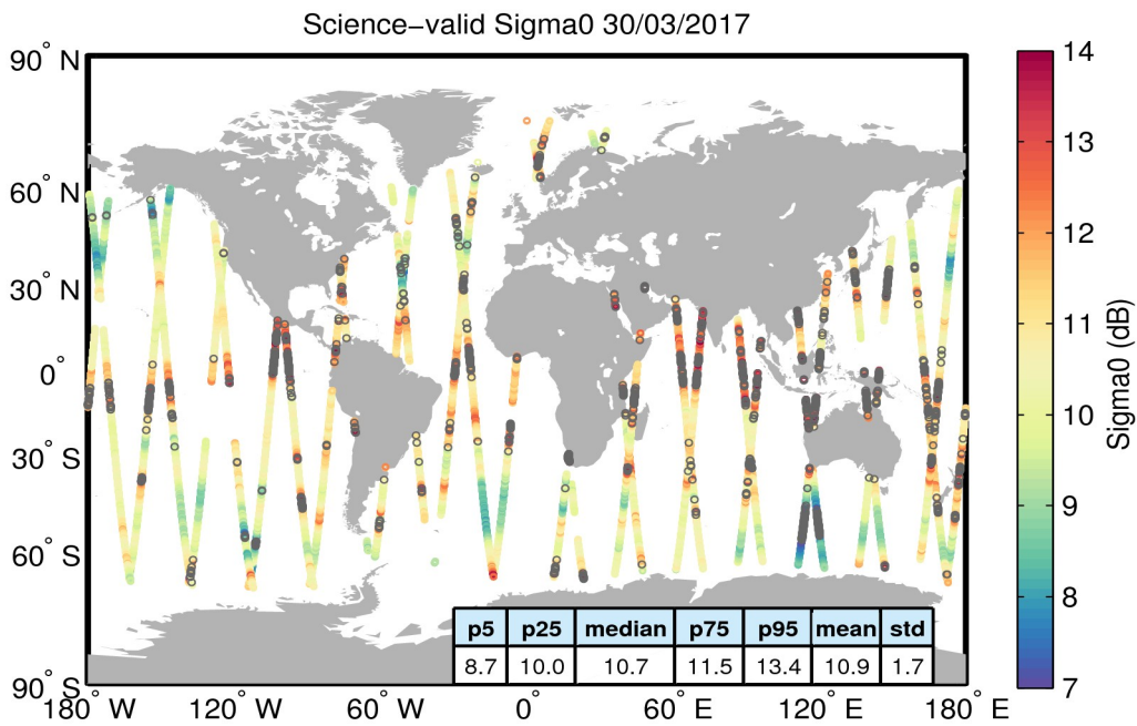
Figure 27. Geographical distribution of science-valid sigma0 data over oceans and lakes for 30/03/2017. The statistical values shown in the table refer to the sigma0 in dB and are calculated over all measurements shown in the figure. Gray circles denote records that have been rejected based on the editing criteria described in Table 4.
