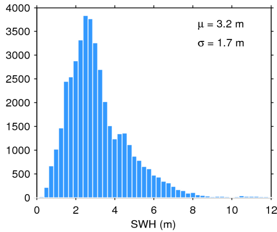
Figure 17. Histogram of flag-valid SWH over oceans and lakes for 30/03/2017. The mean ( \mu ) and standard deviation ( \sigma ) are also shown. Note that values larger than 12 m are excluded from the histogram for the sake of readability but not from the computation of \mu and \sigma .
