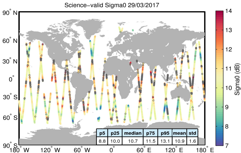
Figure 27. Geographical distribution of science-valid sigma0 data over oceans and lakes for 29/03/2017. The statistical values shown in the table refer to the sigma0 in dB and are calculated over all measurements shown in the figure. Gray circles denote records that have been rejected based on the editing criteria described in Table 4.
