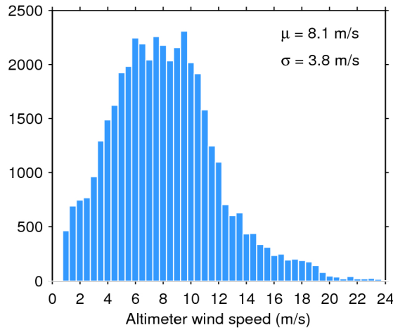
Figure 33. Histogram of flag-valid wind over oceans and lakes for 29/03/2017. The mean ( \mu ) and standard deviation ( \sigma ) are also shown. Note that values larger than 24 m/s are excluded from the histogram for the sake of readability but not from the computation of \mu and \sigma .
