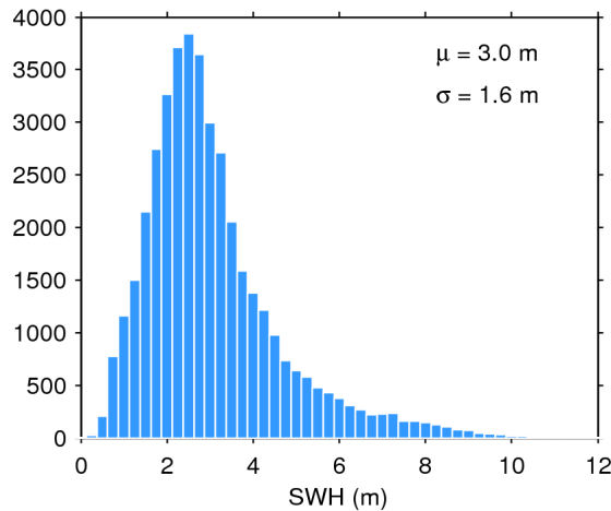
Figure 20. Histogram of science-valid SWH over oceans and lakes for 29/03/2017. The mean ( \mu ) and standard deviation ( \sigma ) are also shown. Note that values larger than 12 m are excluded from the histogram for the sake of readability but not from the computation of \mu and \sigma .
