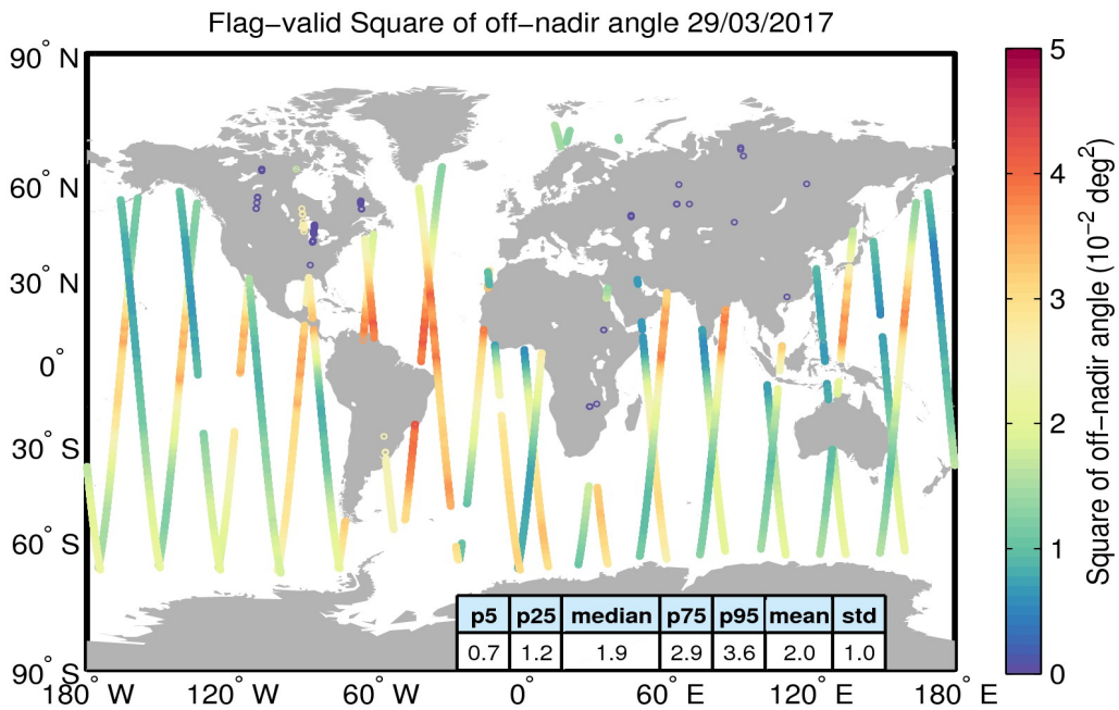
Figure 37. Geographical distribution of flag-valid mispointing data over oceans and lakes for 29/03/2017. The statistical values shown in the table refer to the mispointing in 10^{-2} deg 2 and are calculated over all measurements shown in the figure.
