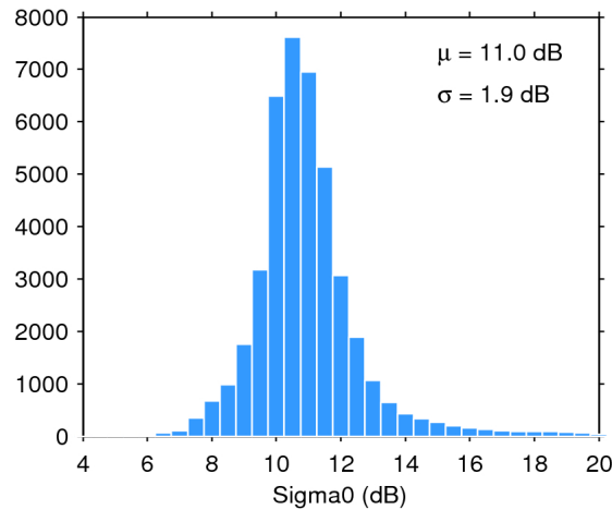
Figure 25. Histogram of flag-valid sigma0 over oceans and lakes for 29/03/2017. The mean ( \mu ) and standard deviation ( \sigma ) are also shown. Note that values outside [4 20] dB are excluded from the histogram for the sake of readability but not from the computation of \mu and \sigma .
