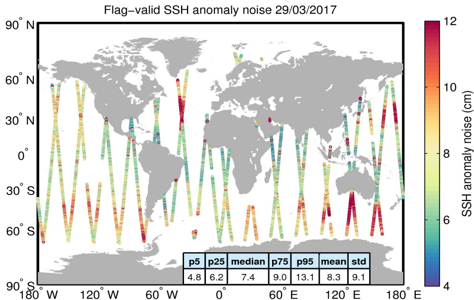
Figure 8. Geographical distribution of flag-valid 20-Hz SSH anomaly measurement noise over oceans and lakes for 29/03/2017. The statistical values shown in the table refer to the SSH anomaly noise and are calculated over all measurements shown in the figure.
