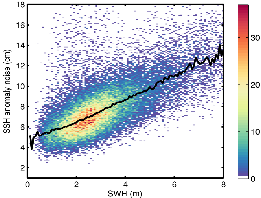
Figure 9. 2D histogram showing flag-valid SSH anomaly noise as a function of SWH for 29/03/2017. The black line denotes the median SSH anomaly noise as a function of SWH.
