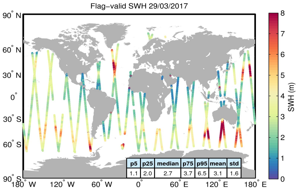
Figure 15. Geographical distribution of flag-valid SWH data over oceans and lakes for 29/03/2017. The statistical values shown in the table refer to the SWH in m and are calculated over all measurements shown in the figure.
