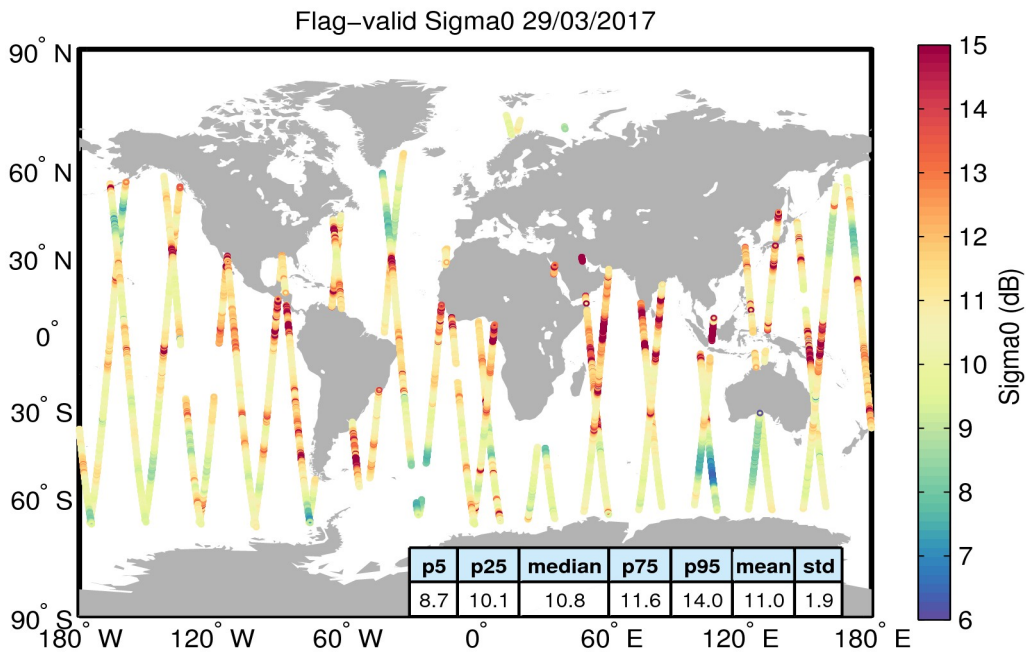
Figure 23. Geographical distribution of flag-valid sigma0 data over oceans and lakes for 29/03/2017. The statistical values shown in the table refer to the sigma0 in dB and are calculated over all measurements shown in the figure.
