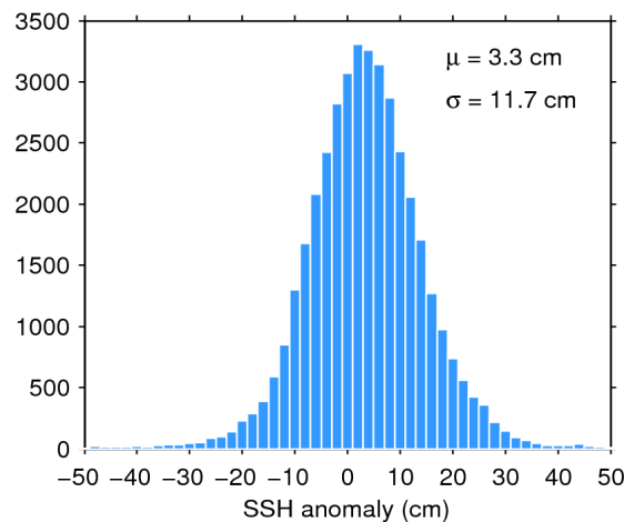
Figure 11. Histogram of science-valid SSH anomaly over oceans and lakes for 29/03/2017. The mean ( \mu ) and standard deviation ( \sigma ) are also shown. Note that values outside [-50 50] cm are excluded from the histogram for the sake of readability but not from the computation of \mu and \sigma .
