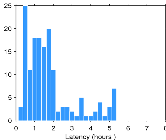
Figure 2. Histogram of the data latency for 29/03/2017. The y-axis denotes the number of files that are made available with a delay of x-hours with respect to the mean time of the records stored in the file.
