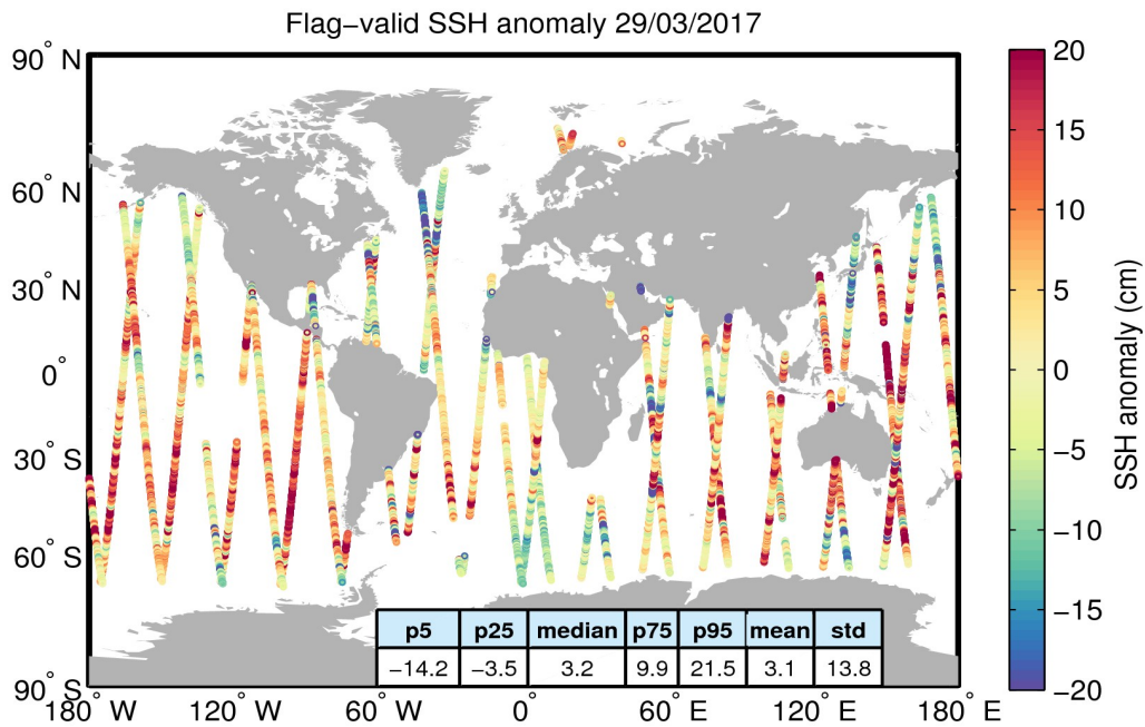
Figure 5. Geographical distribution of flag-valid 1-Hz SSH anomaly data over oceans and lakes for 29/03/2017. The statistical values shown in the table refer to the SSH anomaly in cm and are calculated over all measurements shown in the figure.
