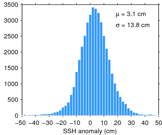
Figure 7. Histogram of flag-valid SSH anomaly over oceans and lakes for 29/03/2017. The mean ( \mu ) and standard deviation ( \sigma ) are also shown. Note that values outside [-50 50] cm are excluded from the histogram for the sake of readability but not from the computation of \mu and \sigma .
