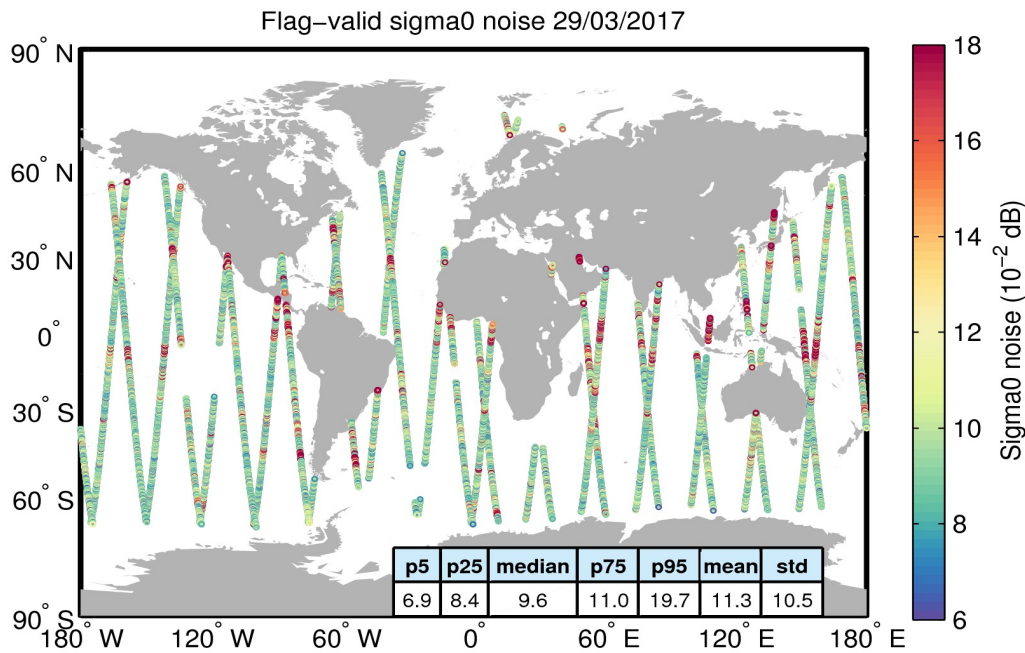
Figure 26. Geographical distribution of flag-valid 20-Hz sigma0 measurement noise over oceans and lakes for 29/03/2017. The statistical values shown in the table refer to the sigma0 noise and are calculated over all measurements shown in the figure.
