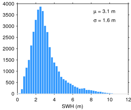
Figure 17. Histogram of flag-valid SWH over oceans and lakes for 29/03/2017. The mean ( \mu ) and standard deviation ( \sigma ) are also shown. Note that values larger than 12 m are excluded from the histogram for the sake of readability but not from the computation of \mu and \sigma .
