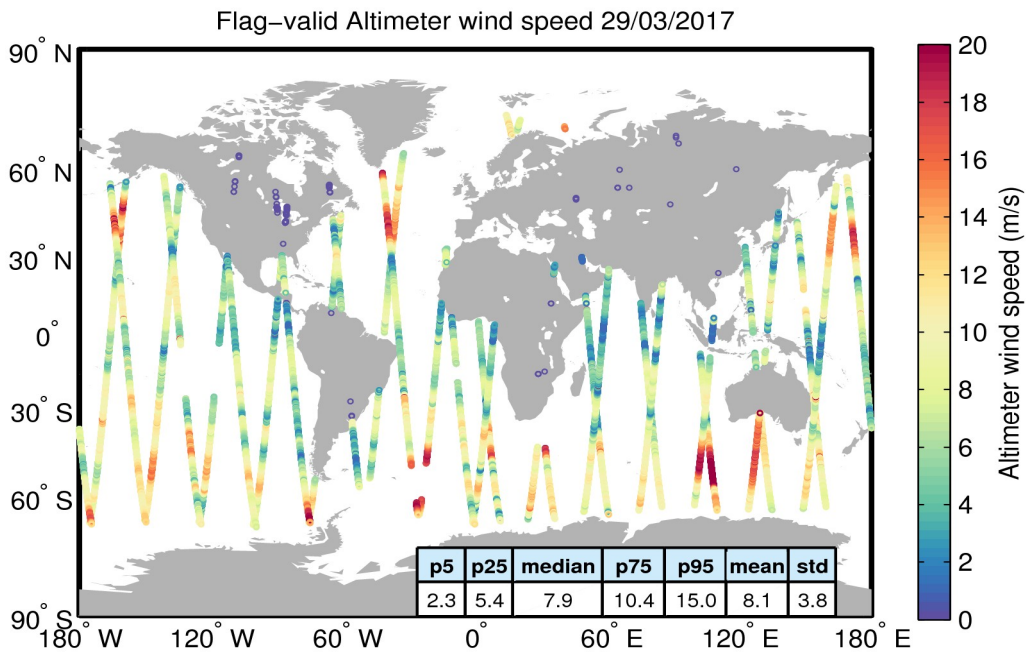
Figure 31. Geographical distribution of flag-valid wind data over oceans and lakes for 29/03/2017. The statistical values shown in the table refer to the wind in m/s and are calculated over all measurements shown in the figure.
