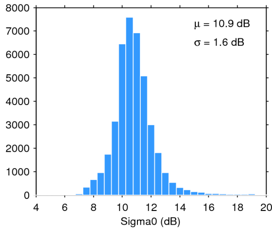
Figure 28. Histogram of science-valid sigma0 over oceans and lakes for 29/03/2017. The mean ( \mu ) and standard deviation ( \sigma ) are also shown. Note that values outside [4 20] dB are excluded from the histogram for the sake of readability but not from the computation of \mu and \sigma .
