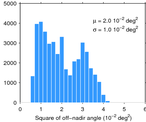
Figure 39. Histogram of flag-valid mispointing over oceans and lakes for 29/03/2017. The mean ( \mu ) and standard deviation ( \sigma ) are also shown. Note that values larger than 6 \cdot 10^{-2} \text{ deg}^2 are excluded from the histogram for the sake of readability but not from the computation of \mu and \sigma .
