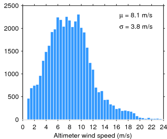
Figure 35. Histogram of science-valid wind over oceans and lakes for 29/03/2017. The mean ( \mu ) and standard deviation ( \sigma ) are also shown. Note that values larger than 24 m/s are excluded from the histogram for the sake of readability but not from the computation of \mu and \sigma .
