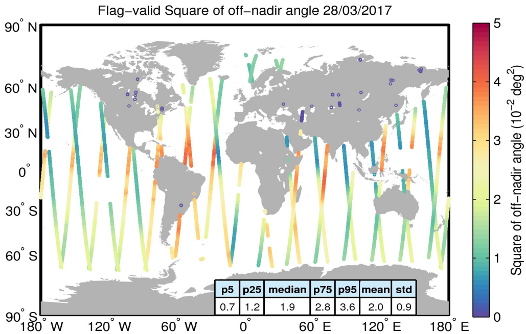
Figure 37. Geographical distribution of flag-valid mispointing data over oceans and lakes for 28/03/2017. The statistical values shown in the table refer to the mispointing in 10^{-2} deg 2 and are calculated over all measurements shown in the figure.
