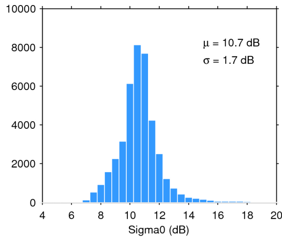
Figure 28. Histogram of science-valid sigma0 over oceans and lakes for 28/03/2017. The mean ( \mu ) and standard deviation ( \sigma ) are also shown. Note that values outside [4 20] dB are excluded from the histogram for the sake of readability but not from the computation of \mu and \sigma .
