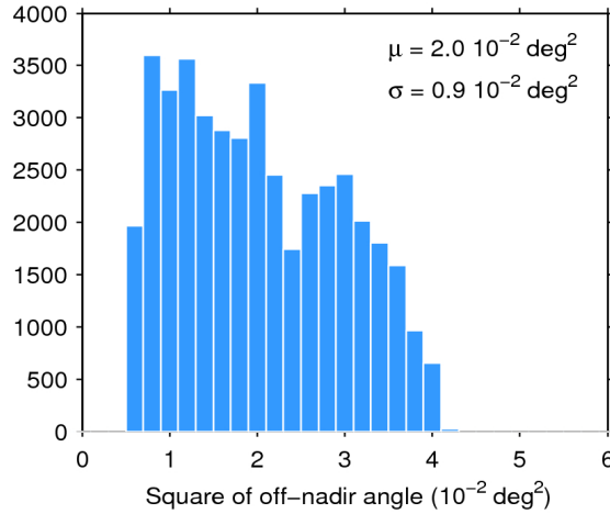
Figure 39. Histogram of flag-valid mispointing over oceans and lakes for 28/03/2017. The mean ( \mu ) and standard deviation ( \sigma ) are also shown. Note that values larger than 6 \cdot 10^{-2} \text{ deg}^2 are excluded from the histogram for the sake of readability but not from the computation of \mu and \sigma .
