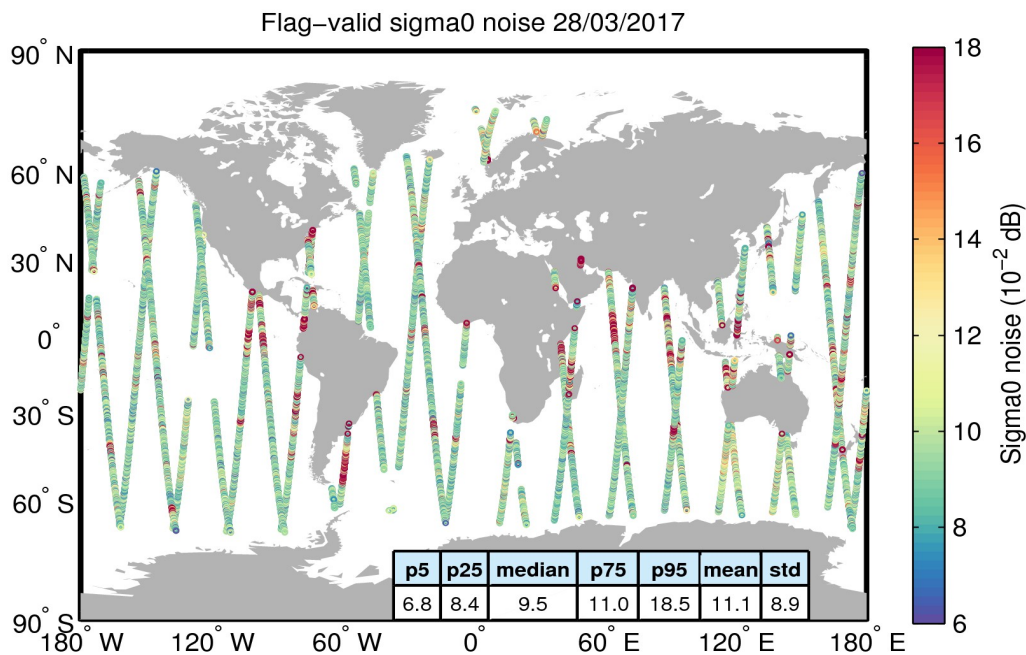
Figure 26. Geographical distribution of flag-valid 20-Hz sigma0 measurement noise over oceans and lakes for 28/03/2017. The statistical values shown in the table refer to the sigma0 noise and are calculated over all measurements shown in the figure.
