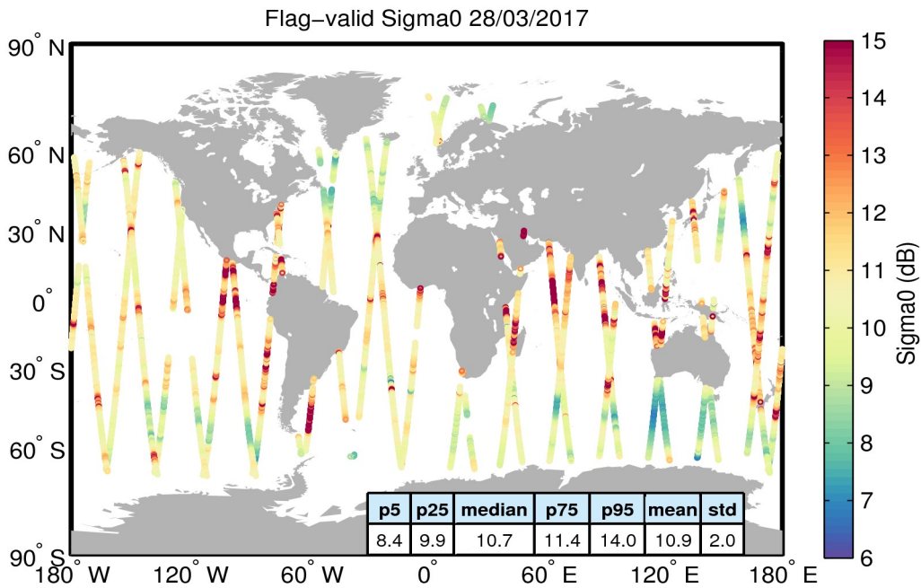
Figure 23. Geographical distribution of flag-valid sigma0 data over oceans and lakes for 28/03/2017. The statistical values shown in the table refer to the sigma0 in dB and are calculated over all measurements shown in the figure.
