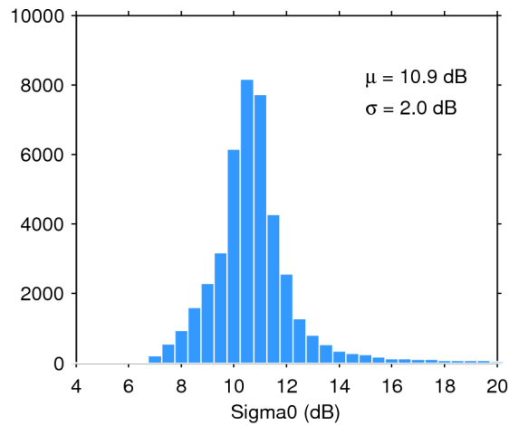
Figure 25. Histogram of flag-valid sigma0 over oceans and lakes for 28/03/2017. The mean ( \mu ) and standard deviation ( \sigma ) are also shown. Note that values outside [4 20] dB are excluded from the histogram for the sake of readability but not from the computation of \mu and \sigma .
