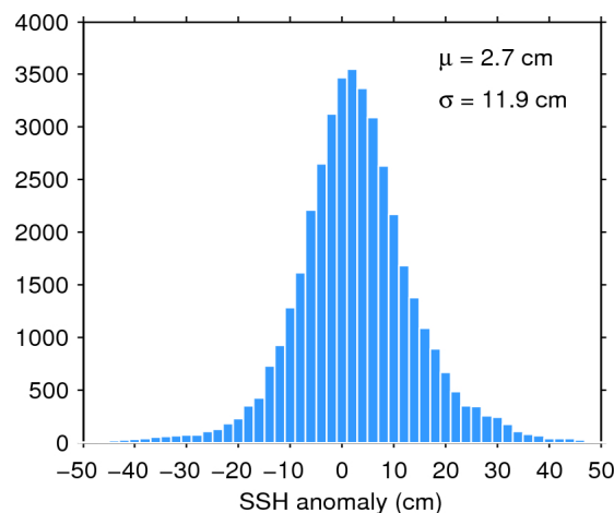
Figure 11. Histogram of science-valid SSH anomaly over oceans and lakes for 28/03/2017. The mean ( \mu ) and standard deviation ( \sigma ) are also shown. Note that values outside [-50 50] cm are excluded from the histogram for the sake of readability but not from the computation of \mu and \sigma .
