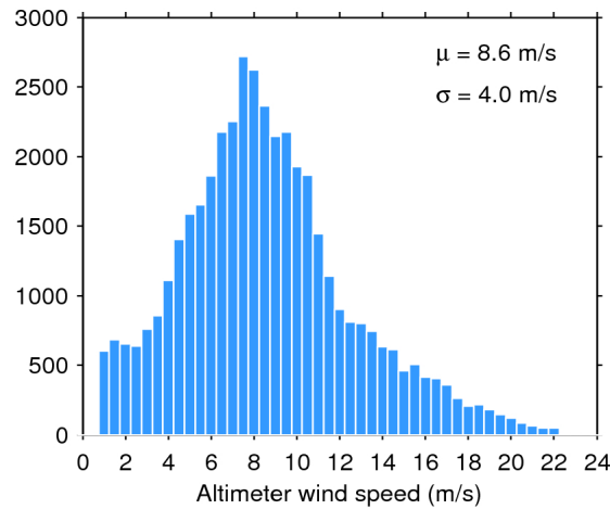
Figure 33. Histogram of flag-valid wind over oceans and lakes for 28/03/2017. The mean ( \mu ) and standard deviation ( \sigma ) are also shown. Note that values larger than 24 m/s are excluded from the histogram for the sake of readability but not from the computation of \mu and \sigma .
