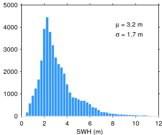
Figure 20. Histogram of science-valid SWH over oceans and lakes for 28/03/2017. The mean ( \mu ) and standard deviation ( \sigma ) are also shown. Note that values larger than 12 m are excluded from the histogram for the sake of readability but not from the computation of \mu and \sigma .
