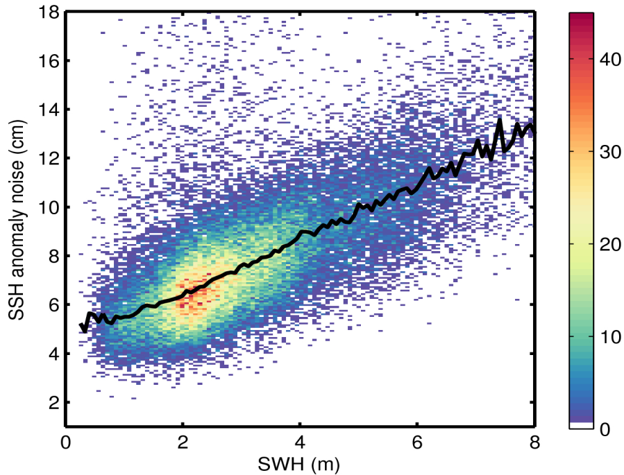
Figure 9. 2D histogram showing flag-valid SSH anomaly noise as a function of SWH for 28/03/2017. The black line denotes the median SSH anomaly noise as a function of SWH.
