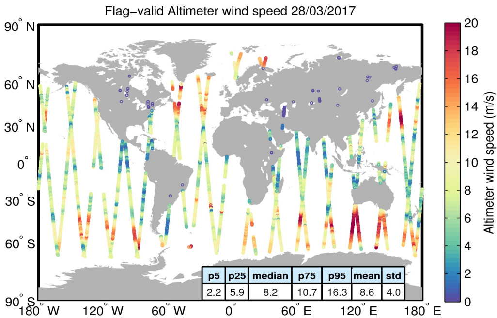
Figure 31. Geographical distribution of flag-valid wind data over oceans and lakes for 28/03/2017. The statistical values shown in the table refer to the wind in m/s and are calculated over all measurements shown in the figure.
