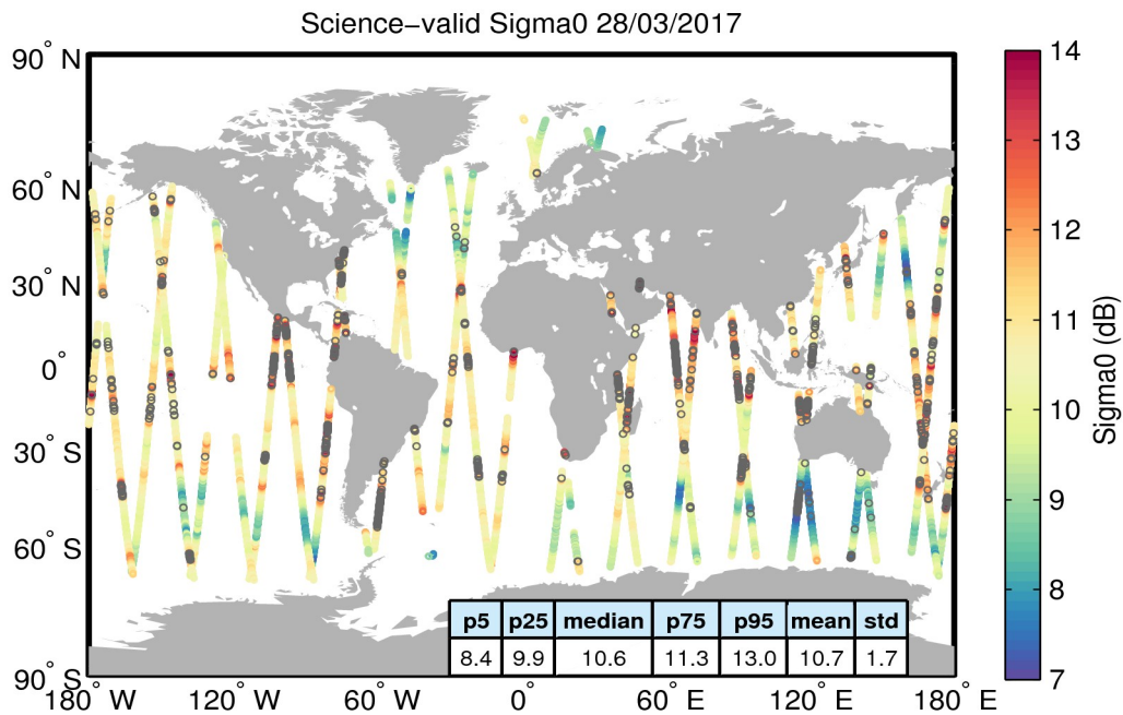
Figure 27. Geographical distribution of science-valid sigma0 data over oceans and lakes for 28/03/2017. The statistical values shown in the table refer to the sigma0 in dB and are calculated over all measurements shown in the figure. Gray circles denote records that have been rejected based on the editing criteria described in Table 4.
