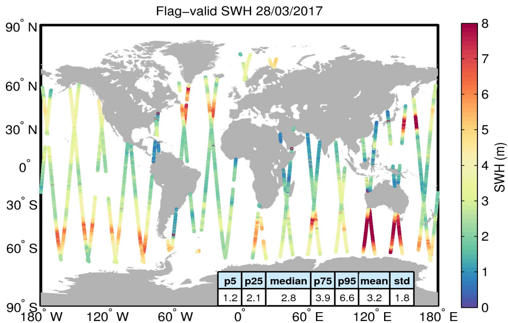
Figure 15. Geographical distribution of flag-valid SWH data over oceans and lakes for 28/03/2017. The statistical values shown in the table refer to the SWH in m and are calculated over all measurements shown in the figure.
