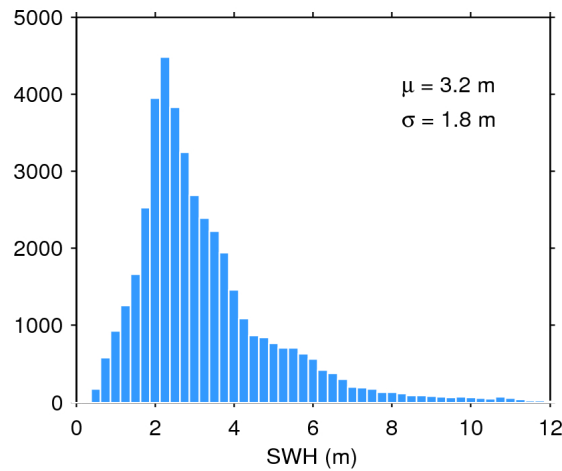
Figure 17. Histogram of flag-valid SWH over oceans and lakes for 28/03/2017. The mean ( \mu ) and standard deviation ( \sigma ) are also shown. Note that values larger than 12 m are excluded from the histogram for the sake of readability but not from the computation of \mu and \sigma .
