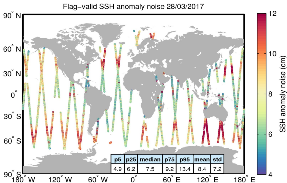
Figure 8. Geographical distribution of flag-valid 20-Hz SSH anomaly measurement noise over oceans and lakes for 28/03/2017. The statistical values shown in the table refer to the SSH anomaly noise and are calculated over all measurements shown in the figure.
