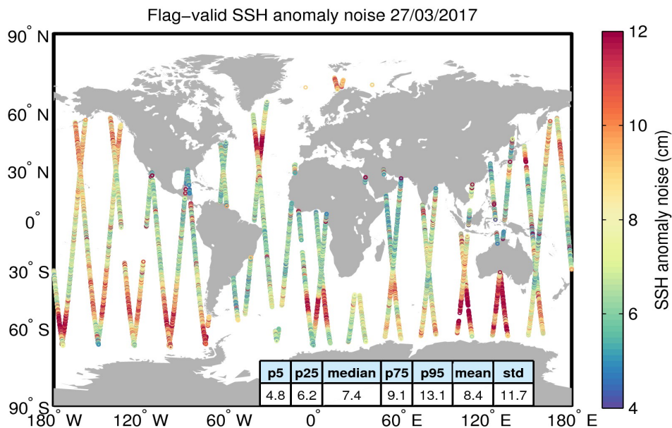
Figure 8. Geographical distribution of flag-valid 20-Hz SSH anomaly measurement noise over oceans and lakes for 27/03/2017. The statistical values shown in the table refer to the SSH anomaly noise and are calculated over all measurements shown in the figure.
