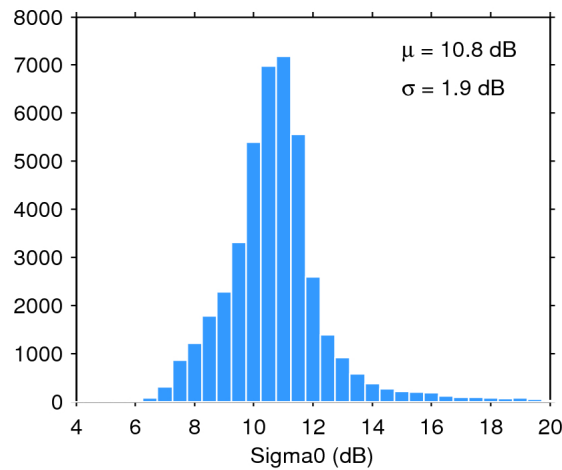
Figure 25. Histogram of flag-valid sigma0 over oceans and lakes for 27/03/2017. The mean ( \mu ) and standard deviation ( \sigma ) are also shown. Note that values outside [4 20] dB are excluded from the histogram for the sake of readability but not from the computation of \mu and \sigma .
