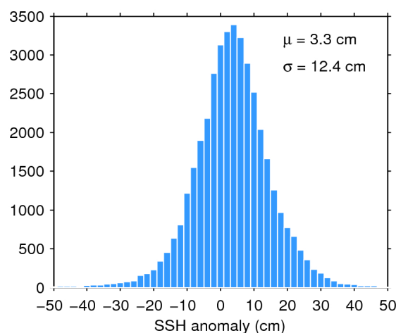
Figure 11. Histogram of science-valid SSH anomaly over oceans and lakes for 27/03/2017. The mean ( \mu ) and standard deviation ( \sigma ) are also shown. Note that values outside [-50 50] cm are excluded from the histogram for the sake of readability but not from the computation of \mu and \sigma .
