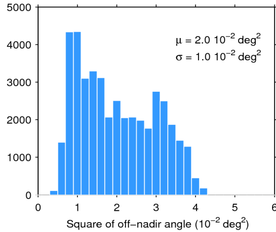
Figure 39. Histogram of flag-valid mispointing over oceans and lakes for 27/03/2017. The mean ( \mu ) and standard deviation ( \sigma ) are also shown. Note that values larger than 6 \cdot 10^{-2} \text{ deg}^2 are excluded from the histogram for the sake of readability but not from the computation of \mu and \sigma .
