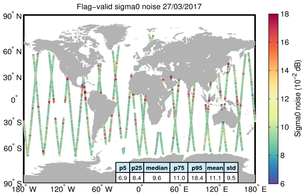
Figure 26. Geographical distribution of flag-valid 20-Hz sigma0 measurement noise over oceans and lakes for 27/03/2017. The statistical values shown in the table refer to the sigma0 noise and are calculated over all measurements shown in the figure.
