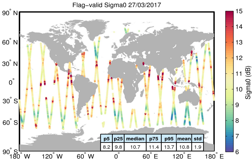
Figure 23. Geographical distribution of flag-valid sigma0 data over oceans and lakes for 27/03/2017. The statistical values shown in the table refer to the sigma0 in dB and are calculated over all measurements shown in the figure.
