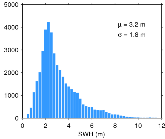
Figure 17. Histogram of flag-valid SWH over oceans and lakes for 27/03/2017. The mean ( \mu ) and standard deviation ( \sigma ) are also shown. Note that values larger than 12 m are excluded from the histogram for the sake of readability but not from the computation of \mu and \sigma .
