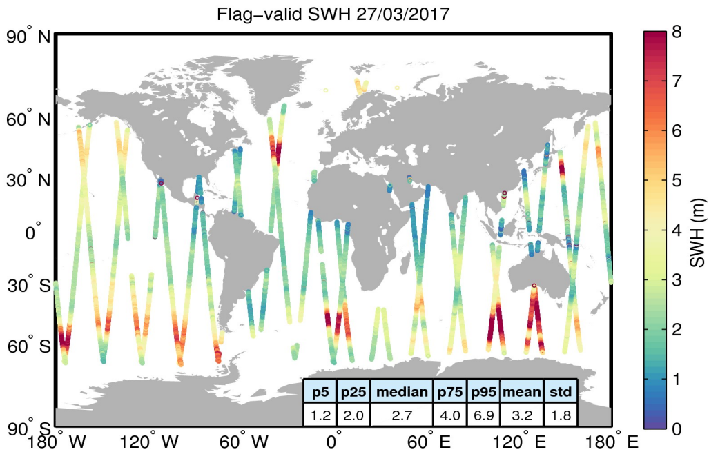
Figure 15. Geographical distribution of flag-valid SWH data over oceans and lakes for 27/03/2017. The statistical values shown in the table refer to the SWH in m and are calculated over all measurements shown in the figure.
