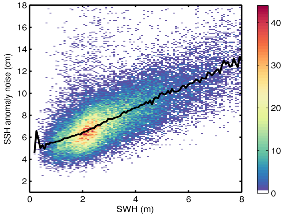
Figure 9. 2D histogram showing flag-valid SSH anomaly noise as a function of SWH for 27/03/2017. The black line denotes the median SSH anomaly noise as a function of SWH.
