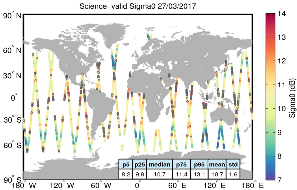
Figure 27. Geographical distribution of science-valid sigma0 data over oceans and lakes for 27/03/2017. The statistical values shown in the table refer to the sigma0 in dB and are calculated over all measurements shown in the figure. Gray circles denote records that have been rejected based on the editing criteria described in Table 4.
