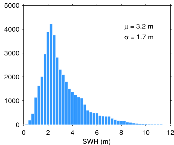
Figure 20. Histogram of science-valid SWH over oceans and lakes for 27/03/2017. The mean ( \mu ) and standard deviation ( \sigma ) are also shown. Note that values larger than 12 m are excluded from the histogram for the sake of readability but not from the computation of \mu and \sigma .
