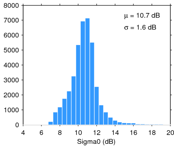
Figure 28. Histogram of science-valid sigma0 over oceans and lakes for 27/03/2017. The mean ( \mu ) and standard deviation ( \sigma ) are also shown. Note that values outside [4 20] dB are excluded from the histogram for the sake of readability but not from the computation of \mu and \sigma .
