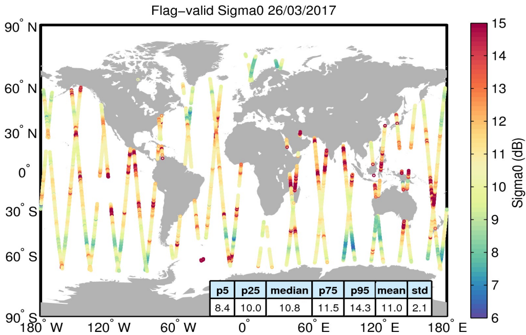
Figure 23. Geographical distribution of flag-valid sigma0 data over oceans and lakes for 26/03/2017. The statistical values shown in the table refer to the sigma0 in dB and are calculated over all measurements shown in the figure.
