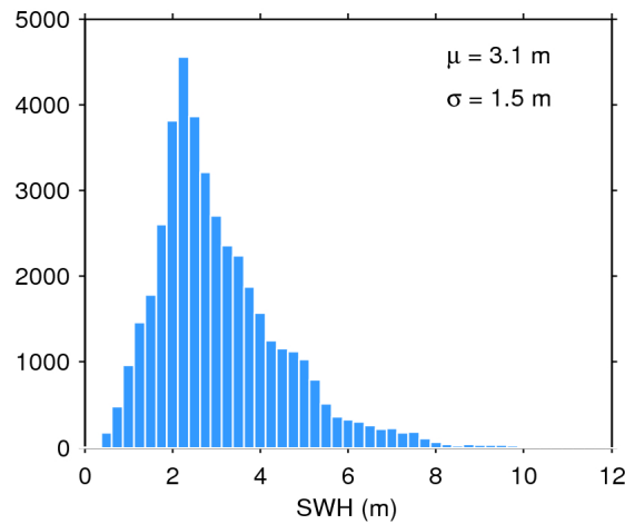
Figure 17. Histogram of flag-valid SWH over oceans and lakes for 26/03/2017. The mean ( \mu ) and standard deviation ( \sigma ) are also shown. Note that values larger than 12 m are excluded from the histogram for the sake of readability but not from the computation of \mu and \sigma .
