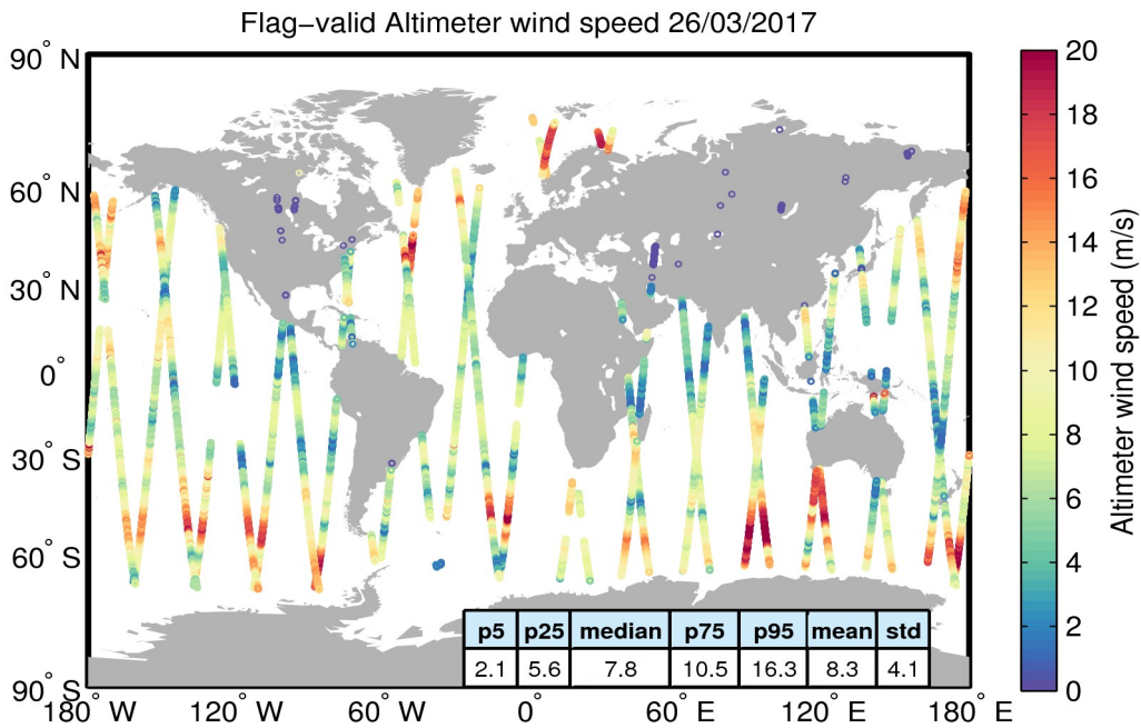
Figure 31. Geographical distribution of flag-valid wind data over oceans and lakes for 26/03/2017. The statistical values shown in the table refer to the wind in m/s and are calculated over all measurements shown in the figure.
