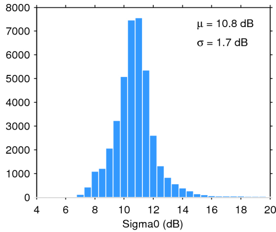
Figure 28. Histogram of science-valid sigma0 over oceans and lakes for 26/03/2017. The mean ( \mu ) and standard deviation ( \sigma ) are also shown. Note that values outside [4 20] dB are excluded from the histogram for the sake of readability but not from the computation of \mu and \sigma .
