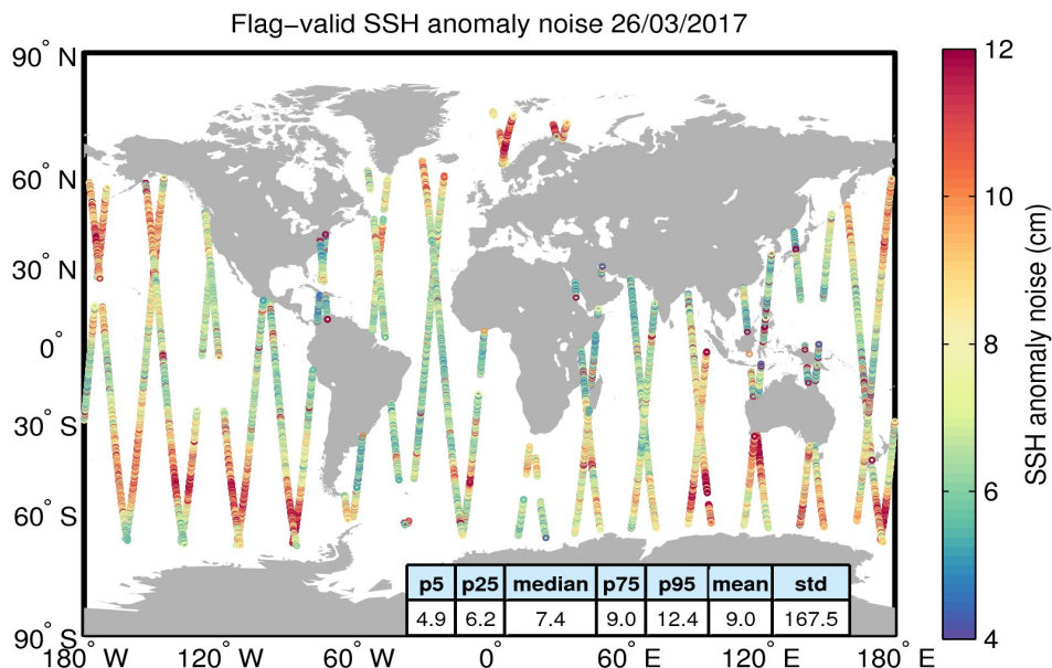
Figure 8. Geographical distribution of flag-valid 20-Hz SSH anomaly measurement noise over oceans and lakes for 26/03/2017. The statistical values shown in the table refer to the SSH anomaly noise and are calculated over all measurements shown in the figure.
