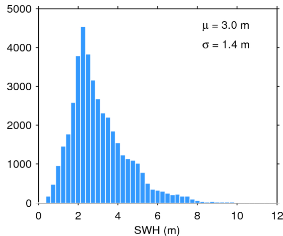
Figure 20. Histogram of science-valid SWH over oceans and lakes for 26/03/2017. The mean ( \mu ) and standard deviation ( \sigma ) are also shown. Note that values larger than 12 m are excluded from the histogram for the sake of readability but not from the computation of \mu and \sigma .
