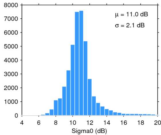
Figure 25. Histogram of flag-valid sigma0 over oceans and lakes for 26/03/2017. The mean ( \mu ) and standard deviation ( \sigma ) are also shown. Note that values outside [4 20] dB are excluded from the histogram for the sake of readability but not from the computation of \mu and \sigma .
