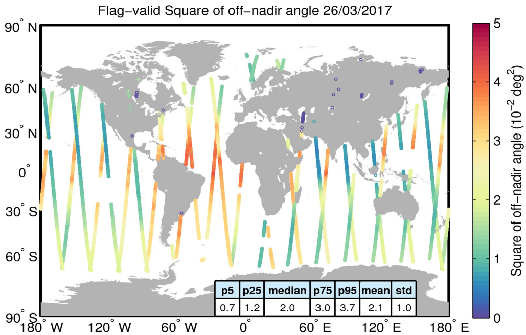
Figure 37. Geographical distribution of flag-valid mispointing data over oceans and lakes for 26/03/2017. The statistical values shown in the table refer to the mispointing in 10^{-2} deg 2 and are calculated over all measurements shown in the figure.
