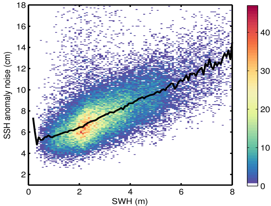
Figure 9. 2D histogram showing flag-valid SSH anomaly noise as a function of SWH for 26/03/2017. The black line denotes the median SSH anomaly noise as a function of SWH.
