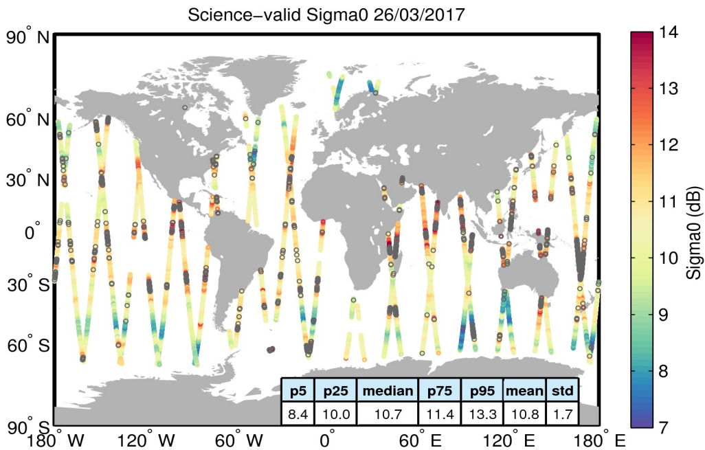
Figure 27. Geographical distribution of science-valid sigma0 data over oceans and lakes for 26/03/2017. The statistical values shown in the table refer to the sigma0 in dB and are calculated over all measurements shown in the figure. Gray circles denote records that have been rejected based on the editing criteria described in Table 4.
