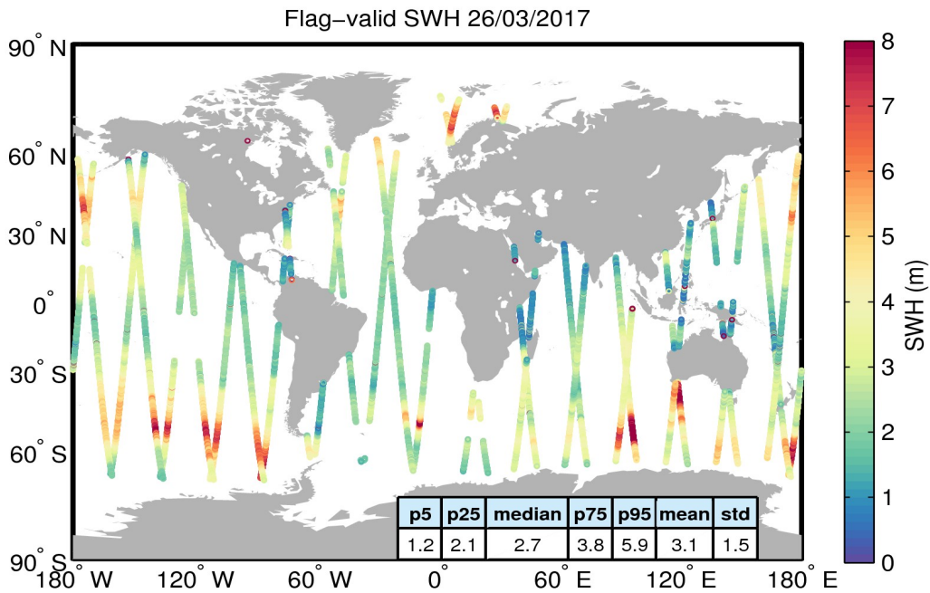
Figure 15. Geographical distribution of flag-valid SWH data over oceans and lakes for 26/03/2017. The statistical values shown in the table refer to the SWH in m and are calculated over all measurements shown in the figure.
