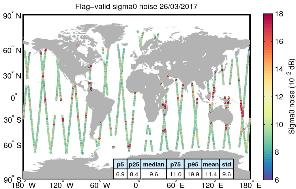
Figure 26. Geographical distribution of flag-valid 20-Hz sigma0 measurement noise over oceans and lakes for 26/03/2017. The statistical values shown in the table refer to the sigma0 noise and are calculated over all measurements shown in the figure.
