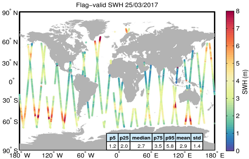
Figure 15. Geographical distribution of flag-valid SWH data over oceans and lakes for 25/03/2017. The statistical values shown in the table refer to the SWH in m and are calculated over all measurements shown in the figure.
