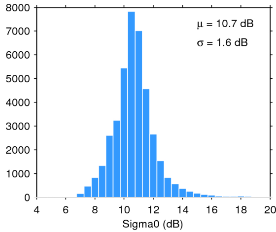
Figure 28. Histogram of science-valid sigma0 over oceans and lakes for 25/03/2017. The mean ( \mu ) and standard deviation ( \sigma ) are also shown. Note that values outside [4 20] dB are excluded from the histogram for the sake of readability but not from the computation of \mu and \sigma .
