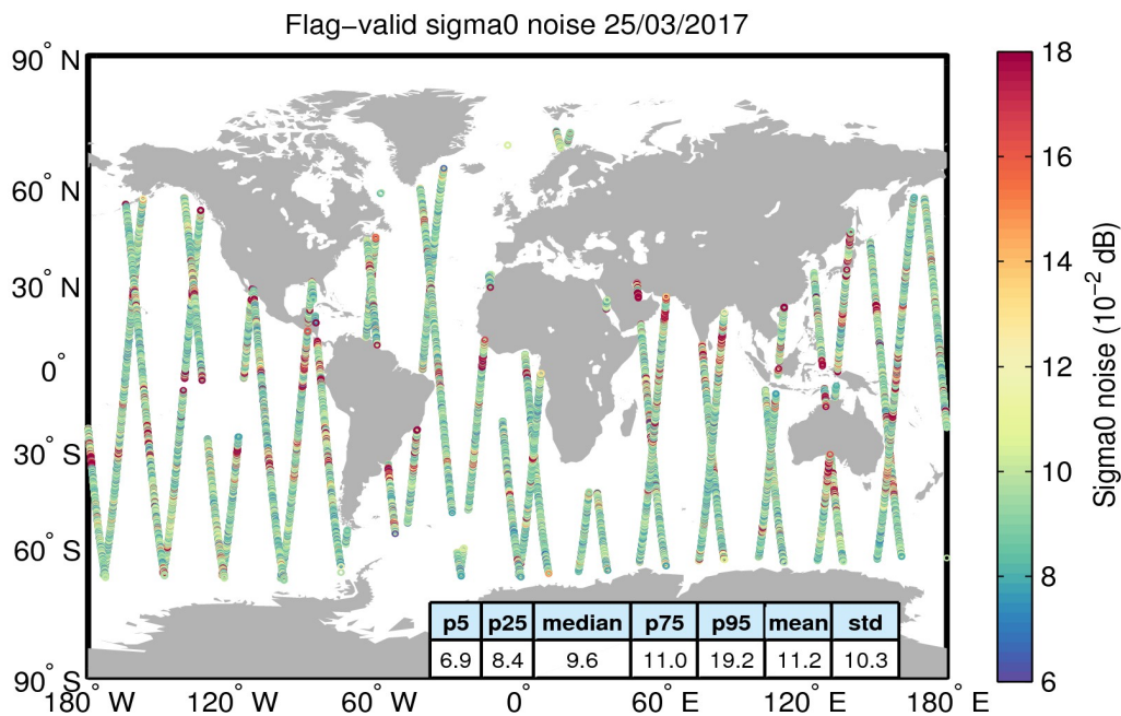
Figure 26. Geographical distribution of flag-valid 20-Hz sigma0 measurement noise over oceans and lakes for 25/03/2017. The statistical values shown in the table refer to the sigma0 noise and are calculated over all measurements shown in the figure.
