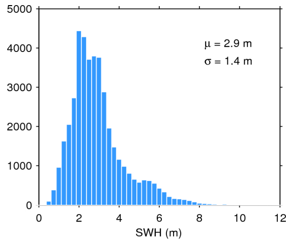
Figure 17. Histogram of flag-valid SWH over oceans and lakes for 25/03/2017. The mean ( \mu ) and standard deviation ( \sigma ) are also shown. Note that values larger than 12 m are excluded from the histogram for the sake of readability but not from the computation of \mu and \sigma .
