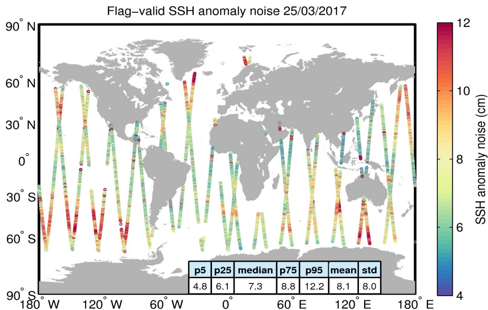
Figure 8. Geographical distribution of flag-valid 20-Hz SSH anomaly measurement noise over oceans and lakes for 25/03/2017. The statistical values shown in the table refer to the SSH anomaly noise and are calculated over all measurements shown in the figure.
