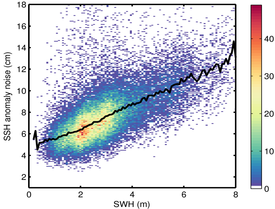
Figure 9. 2D histogram showing flag-valid SSH anomaly noise as a function of SWH for 25/03/2017. The black line denotes the median SSH anomaly noise as a function of SWH.
