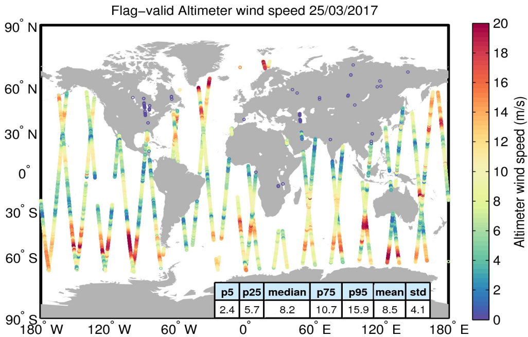
Figure 31. Geographical distribution of flag-valid wind data over oceans and lakes for 25/03/2017. The statistical values shown in the table refer to the wind in m/s and are calculated over all measurements shown in the figure.
