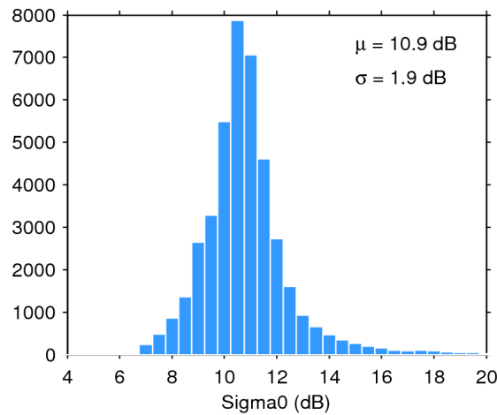
Figure 25. Histogram of flag-valid sigma0 over oceans and lakes for 25/03/2017. The mean ( \mu ) and standard deviation ( \sigma ) are also shown. Note that values outside [4 20] dB are excluded from the histogram for the sake of readability but not from the computation of \mu and \sigma .
