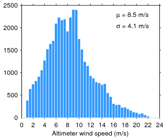
Figure 35. Histogram of science-valid wind over oceans and lakes for 25/03/2017. The mean ( \mu ) and standard deviation ( \sigma ) are also shown. Note that values larger than 24 m/s are excluded from the histogram for the sake of readability but not from the computation of \mu and \sigma .
