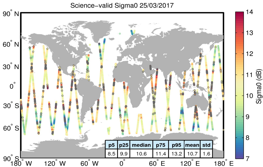
Figure 27. Geographical distribution of science-valid sigma0 data over oceans and lakes for 25/03/2017. The statistical values shown in the table refer to the sigma0 in dB and are calculated over all measurements shown in the figure. Gray circles denote records that have been rejected based on the editing criteria described in Table 4.
