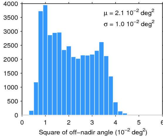
Figure 39. Histogram of flag-valid mispointing over oceans and lakes for 25/03/2017. The mean ( \mu ) and standard deviation ( \sigma ) are also shown. Note that values larger than 6 \cdot 10^{-2} \text{ deg}^2 are excluded from the histogram for the sake of readability but not from the computation of \mu and \sigma .
