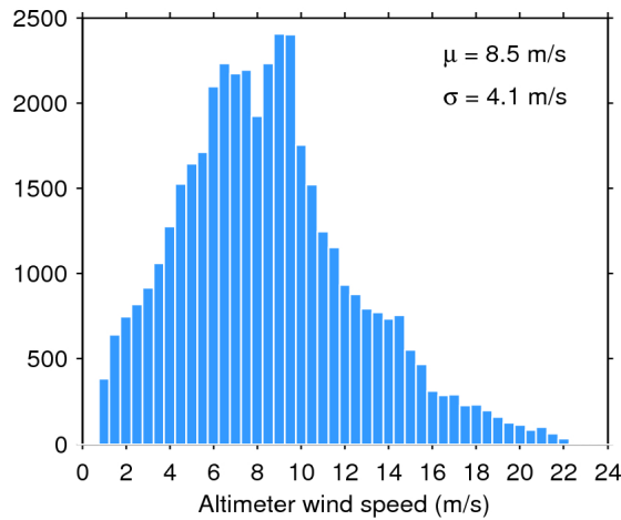
Figure 33. Histogram of flag-valid wind over oceans and lakes for 25/03/2017. The mean ( \mu ) and standard deviation ( \sigma ) are also shown. Note that values larger than 24 m/s are excluded from the histogram for the sake of readability but not from the computation of \mu and \sigma .
