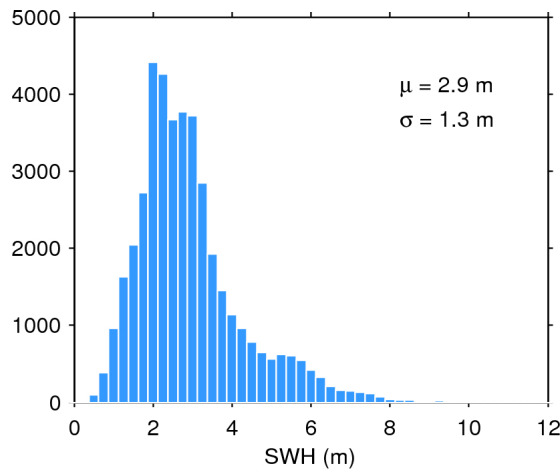
Figure 20. Histogram of science-valid SWH over oceans and lakes for 25/03/2017. The mean ( \mu ) and standard deviation ( \sigma ) are also shown. Note that values larger than 12 m are excluded from the histogram for the sake of readability but not from the computation of \mu and \sigma .
