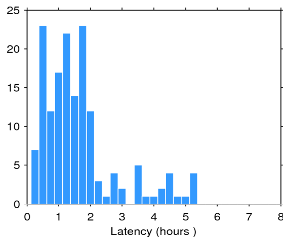
Figure 2. Histogram of the data latency for 25/03/2017. The y-axis denotes the number of files that are made available with a delay of x-hours with respect to the mean time of the records stored in the file.
