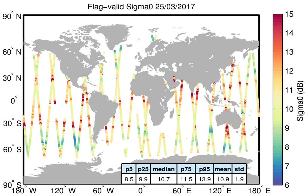
Figure 23. Geographical distribution of flag-valid sigma0 data over oceans and lakes for 25/03/2017. The statistical values shown in the table refer to the sigma0 in dB and are calculated over all measurements shown in the figure.
