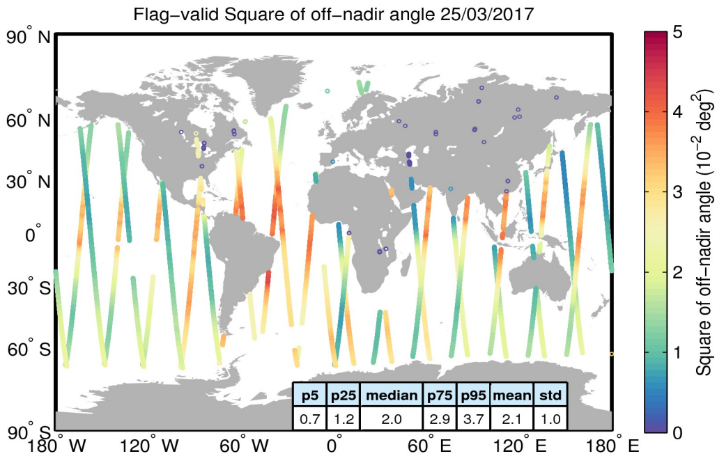
Figure 37. Geographical distribution of flag-valid mispointing data over oceans and lakes for 25/03/2017. The statistical values shown in the table refer to the mispointing in 10^{-2} deg 2 and are calculated over all measurements shown in the figure.
