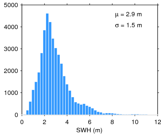
Figure 17. Histogram of flag-valid SWH over oceans and lakes for 24/03/2017. The mean ( \mu ) and standard deviation ( \sigma ) are also shown. Note that values larger than 12 m are excluded from the histogram for the sake of readability but not from the computation of \mu and \sigma .
