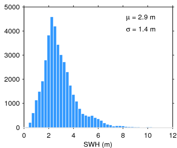
Figure 20. Histogram of science-valid SWH over oceans and lakes for 24/03/2017. The mean ( \mu ) and standard deviation ( \sigma ) are also shown. Note that values larger than 12 m are excluded from the histogram for the sake of readability but not from the computation of \mu and \sigma .
