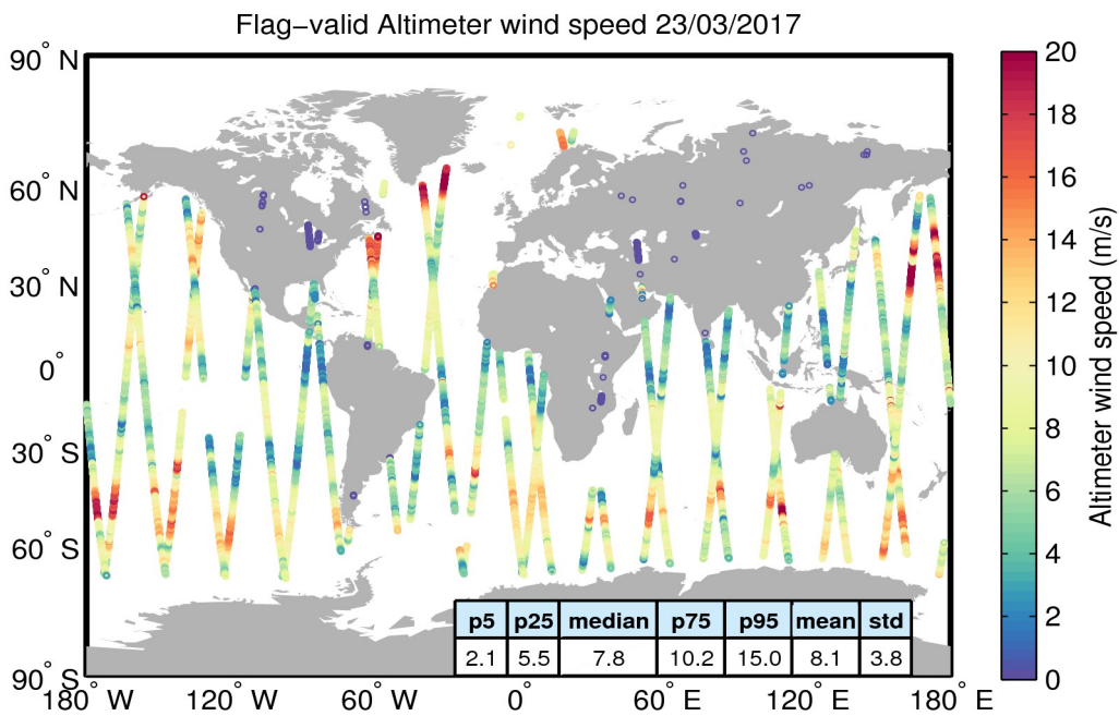
Figure 31. Geographical distribution of flag-valid wind data over oceans and lakes for 23/03/2017. The statistical values shown in the table refer to the wind in m/s and are calculated over all measurements shown in the figure.
