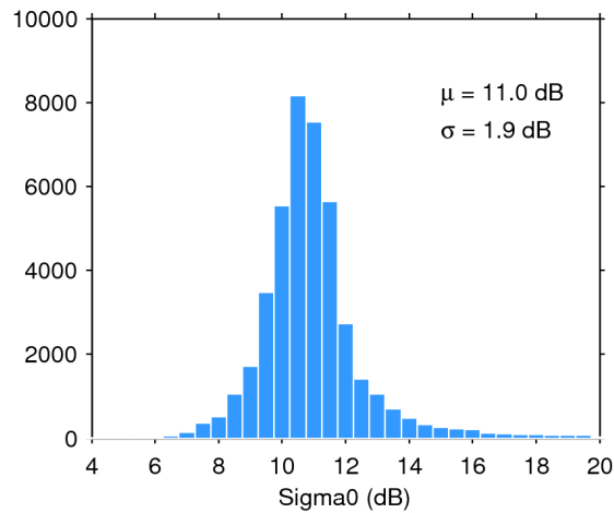
Figure 25. Histogram of flag-valid sigma0 over oceans and lakes for 23/03/2017. The mean ( \mu ) and standard deviation ( \sigma ) are also shown. Note that values outside [4 20] dB are excluded from the histogram for the sake of readability but not from the computation of \mu and \sigma .
