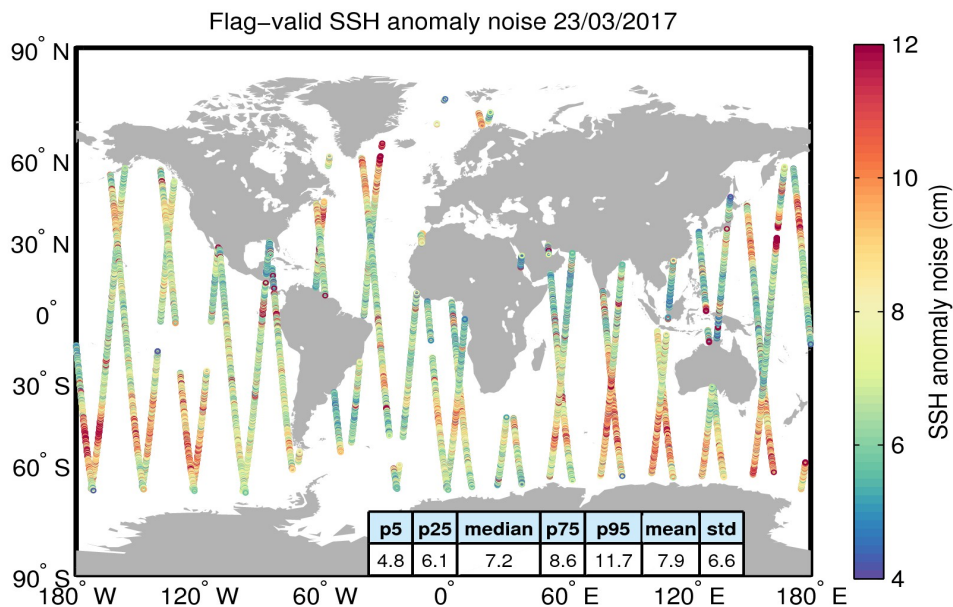
Figure 8. Geographical distribution of flag-valid 20-Hz SSH anomaly measurement noise over oceans and lakes for 23/03/2017. The statistical values shown in the table refer to the SSH anomaly noise and are calculated over all measurements shown in the figure.
