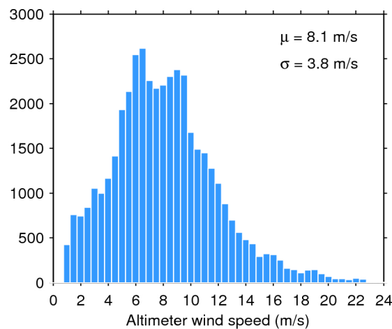
Figure 35. Histogram of science-valid wind over oceans and lakes for 23/03/2017. The mean ( \mu ) and standard deviation ( \sigma ) are also shown. Note that values larger than 24 m/s are excluded from the histogram for the sake of readability but not from the computation of \mu and \sigma .
