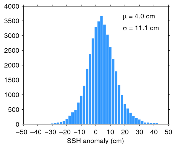
Figure 11. Histogram of science-valid SSH anomaly over oceans and lakes for 23/03/2017. The mean ( \mu ) and standard deviation ( \sigma ) are also shown. Note that values outside [-50 50] cm are excluded from the histogram for the sake of readability but not from the computation of \mu and \sigma .
