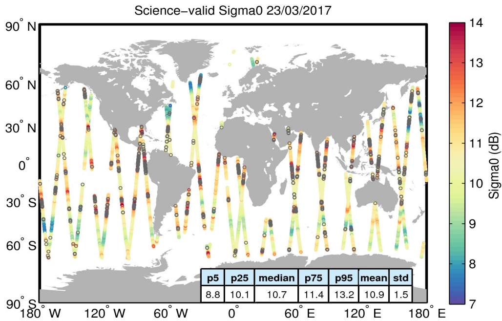
Figure 27. Geographical distribution of science-valid sigma0 data over oceans and lakes for 23/03/2017. The statistical values shown in the table refer to the sigma0 in dB and are calculated over all measurements shown in the figure. Gray circles denote records that have been rejected based on the editing criteria described in Table 4.
