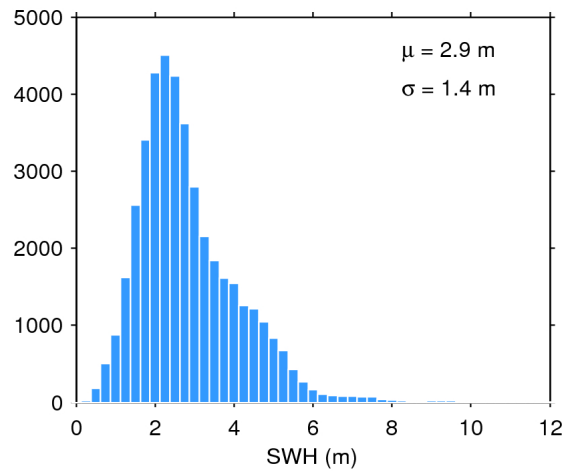
Figure 17. Histogram of flag-valid SWH over oceans and lakes for 23/03/2017. The mean ( \mu ) and standard deviation ( \sigma ) are also shown. Note that values larger than 12 m are excluded from the histogram for the sake of readability but not from the computation of \mu and \sigma .
