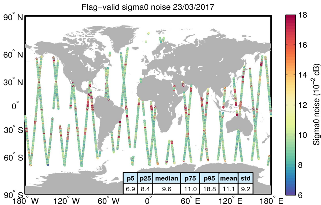
Figure 26. Geographical distribution of flag-valid 20-Hz sigma0 measurement noise over oceans and lakes for 23/03/2017. The statistical values shown in the table refer to the sigma0 noise and are calculated over all measurements shown in the figure.
