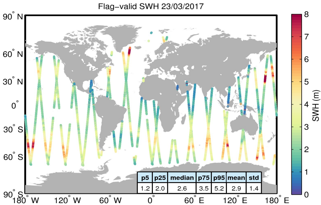
Figure 15. Geographical distribution of flag-valid SWH data over oceans and lakes for 23/03/2017. The statistical values shown in the table refer to the SWH in m and are calculated over all measurements shown in the figure.
