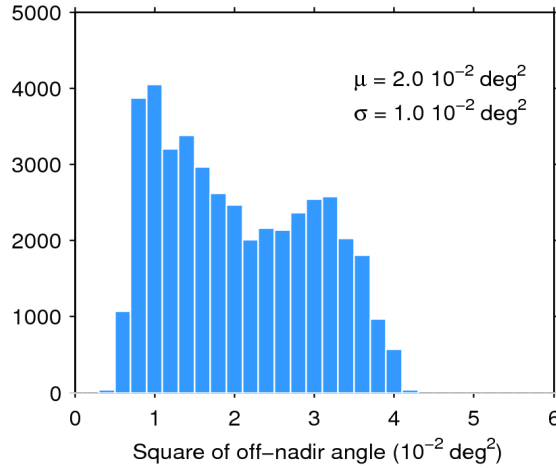
Figure 39. Histogram of flag-valid mispointing over oceans and lakes for 23/03/2017. The mean ( \mu ) and standard deviation ( \sigma ) are also shown. Note that values larger than 6 \cdot 10^{-2} \text{ deg}^2 are excluded from the histogram for the sake of readability but not from the computation of \mu and \sigma .
