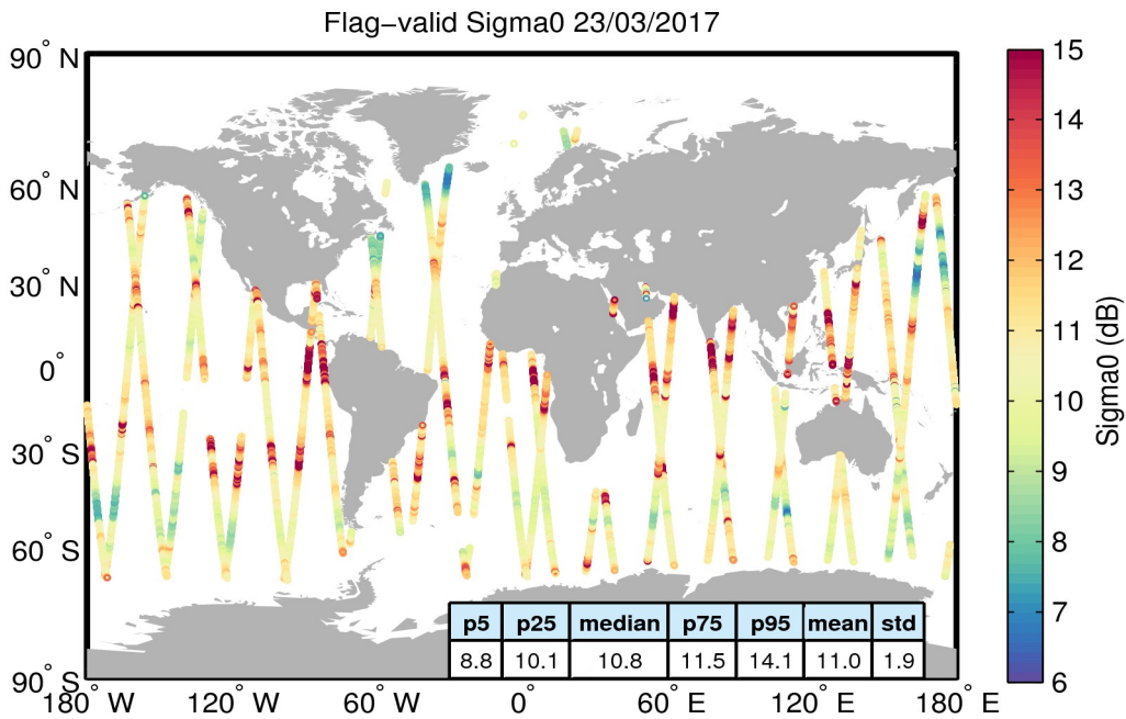
Figure 23. Geographical distribution of flag-valid sigma0 data over oceans and lakes for 23/03/2017. The statistical values shown in the table refer to the sigma0 in dB and are calculated over all measurements shown in the figure.
