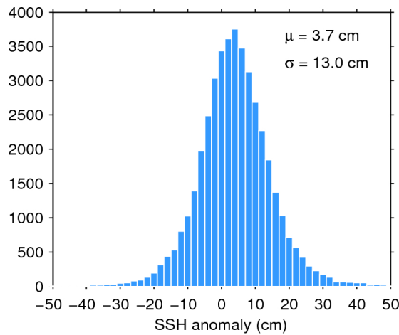
Figure 7. Histogram of flag-valid SSH anomaly over oceans and lakes for 23/03/2017. The mean ( \mu ) and standard deviation ( \sigma ) are also shown. Note that values outside [-50 50] cm are excluded from the histogram for the sake of readability but not from the computation of \mu and \sigma .
