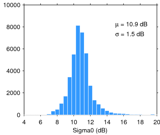
Figure 28. Histogram of science-valid sigma0 over oceans and lakes for 23/03/2017. The mean ( \mu ) and standard deviation ( \sigma ) are also shown. Note that values outside [4 20] dB are excluded from the histogram for the sake of readability but not from the computation of \mu and \sigma .
