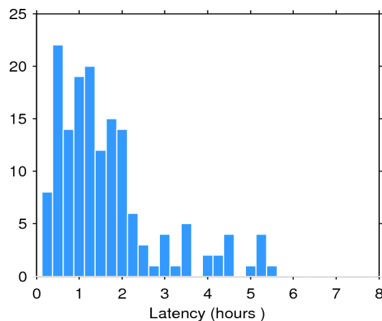
Figure 2. Histogram of the data latency for 23/03/2017. The y-axis denotes the number of files that are made available with a delay of x-hours with respect to the mean time of the records stored in the file.
