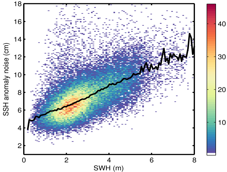
Figure 9. 2D histogram showing flag-valid SSH anomaly noise as a function of SWH for 23/03/2017. The black line denotes the median SSH anomaly noise as a function of SWH.
