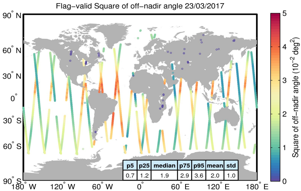
Figure 37. Geographical distribution of flag-valid mispointing data over oceans and lakes for 23/03/2017. The statistical values shown in the table refer to the mispointing in 10^{-2} deg 2 and are calculated over all measurements shown in the figure.
