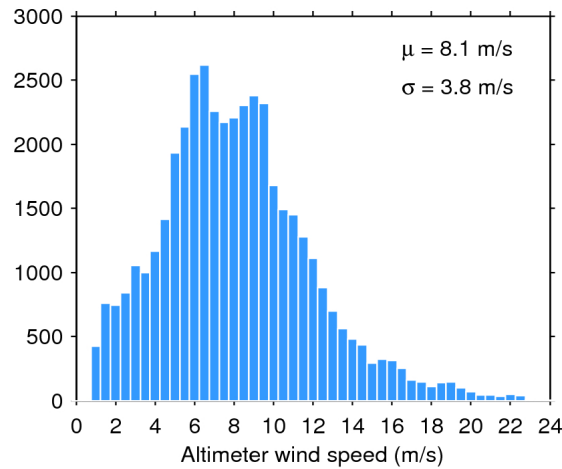
Figure 33. Histogram of flag-valid wind over oceans and lakes for 23/03/2017. The mean ( \mu ) and standard deviation ( \sigma ) are also shown. Note that values larger than 24 m/s are excluded from the histogram for the sake of readability but not from the computation of \mu and \sigma .
