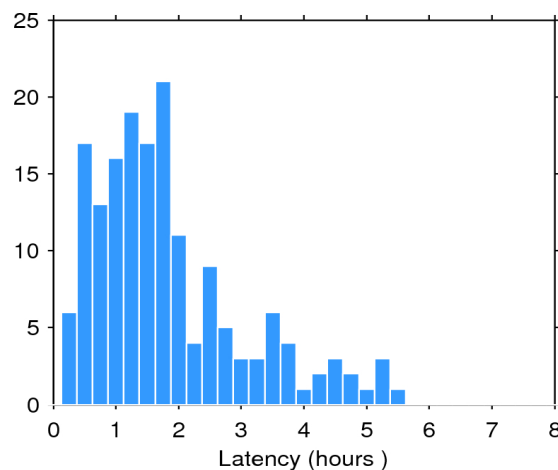
Figure 2. Histogram of the data latency for 22/03/2017. The y-axis denotes the number of files that are made available with a delay of x-hours with respect to the mean time of the records stored in the file.
