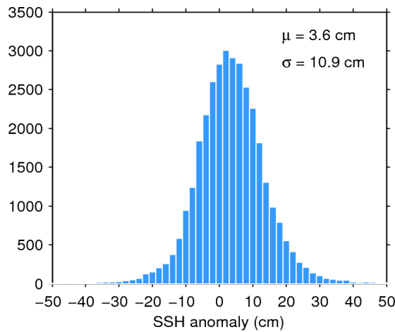
Figure 11. Histogram of science-valid SSH anomaly over oceans and lakes for 22/03/2017. The mean ( \mu ) and standard deviation ( \sigma ) are also shown. Note that values outside [-50 50] cm are excluded from the histogram for the sake of readability but not from the computation of \mu and \sigma .
