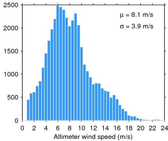
Figure 33. Histogram of flag-valid wind over oceans and lakes for 22/03/2017. The mean ( \mu ) and standard deviation ( \sigma ) are also shown. Note that values larger than 24 m/s are excluded from the histogram for the sake of readability but not from the computation of \mu and \sigma .
