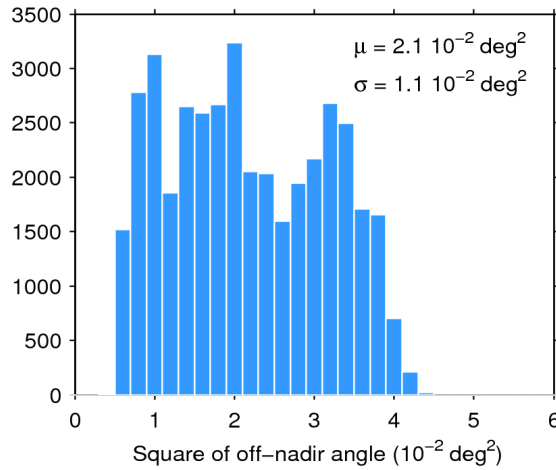
Figure 39. Histogram of flag-valid mispointing over oceans and lakes for 22/03/2017. The mean ( \mu ) and standard deviation ( \sigma ) are also shown. Note that values larger than 6 \cdot 10^{-2} \text{ deg}^2 are excluded from the histogram for the sake of readability but not from the computation of \mu and \sigma .
