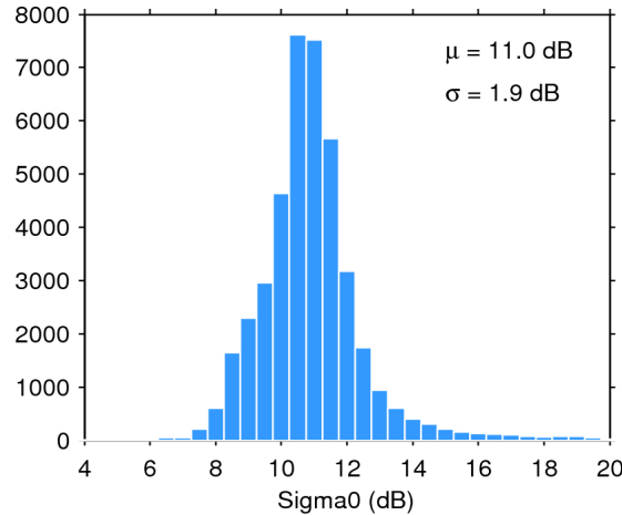
Figure 25. Histogram of flag-valid sigma0 over oceans and lakes for 22/03/2017. The mean ( \mu ) and standard deviation ( \sigma ) are also shown. Note that values outside [4 20] dB are excluded from the histogram for the sake of readability but not from the computation of \mu and \sigma .
