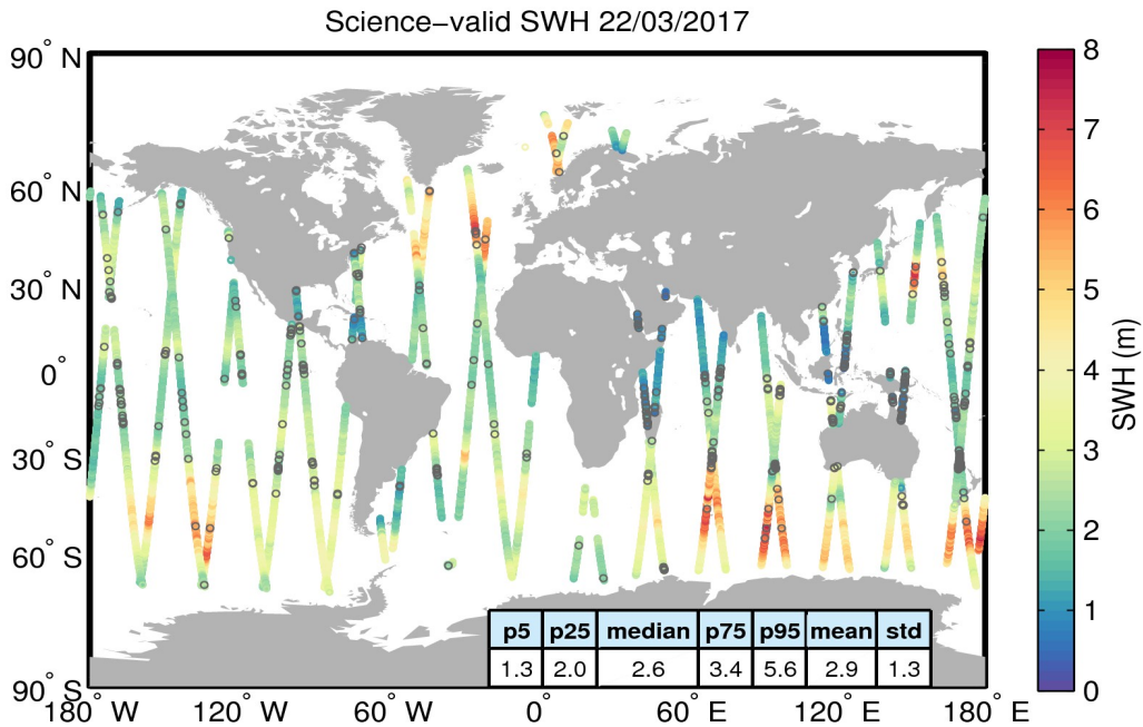
Figure 19. Geographical distribution of science-valid SWH data over oceans and lakes for 22/03/2017. The statistical values shown in the table refer to the SWH in m and are calculated over all measurements shown in the figure. Gray circles denote records that have been rejected based on the editing criteria described in Table 3.
