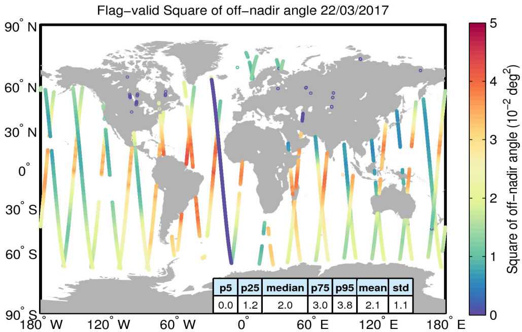
Figure 37. Geographical distribution of flag-valid mispointing data over oceans and lakes for 22/03/2017. The statistical values shown in the table refer to the mispointing in 10^{-2} deg 2 and are calculated over all measurements shown in the figure.
