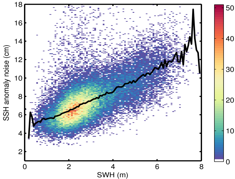
Figure 9. 2D histogram showing flag-valid SSH anomaly noise as a function of SWH for 22/03/2017. The black line denotes the median SSH anomaly noise as a function of SWH.
