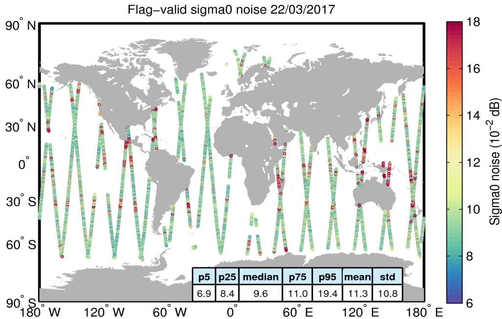
Figure 26. Geographical distribution of flag-valid 20-Hz sigma0 measurement noise over oceans and lakes for 22/03/2017. The statistical values shown in the table refer to the sigma0 noise and are calculated over all measurements shown in the figure.
