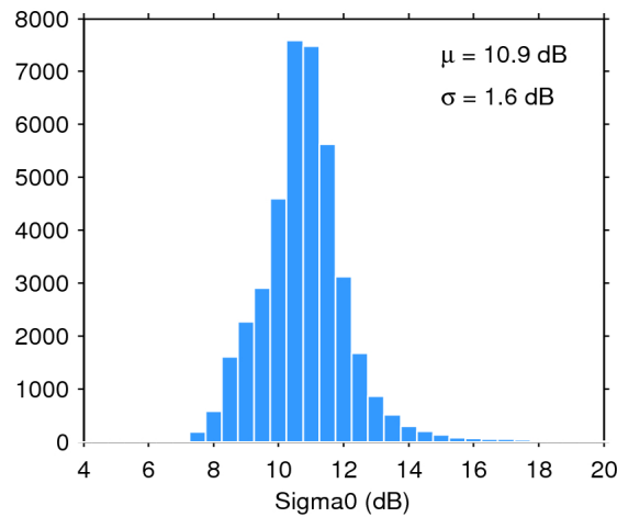
Figure 28. Histogram of science-valid sigma0 over oceans and lakes for 22/03/2017. The mean ( \mu ) and standard deviation ( \sigma ) are also shown. Note that values outside [4 20] dB are excluded from the histogram for the sake of readability but not from the computation of \mu and \sigma .
