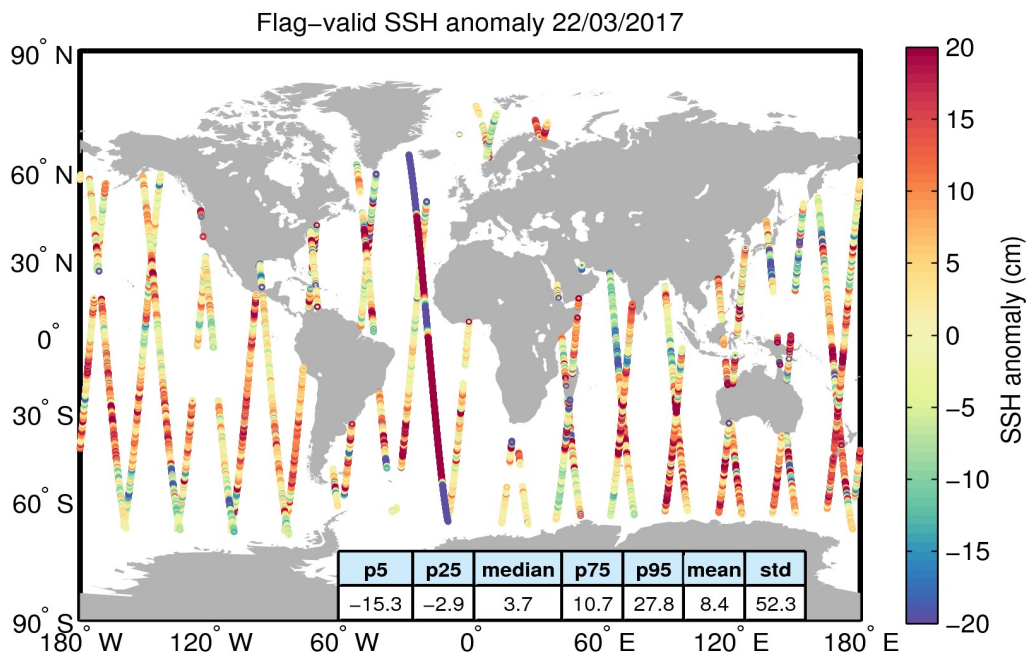
Figure 5. Geographical distribution of flag-valid 1-Hz SSH anomaly data over oceans and lakes for 22/03/2017. The statistical values shown in the table refer to the SSH anomaly in cm and are calculated over all measurements shown in the figure.
