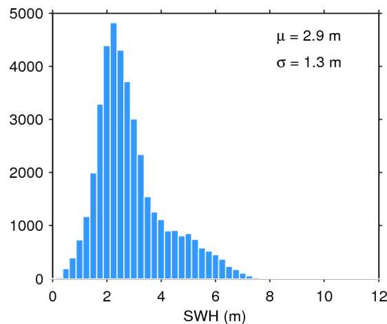
Figure 20. Histogram of science-valid SWH over oceans and lakes for 22/03/2017. The mean ( \mu ) and standard deviation ( \sigma ) are also shown. Note that values larger than 12 m are excluded from the histogram for the sake of readability but not from the computation of \mu and \sigma .
