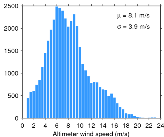
Figure 35. Histogram of science-valid wind over oceans and lakes for 22/03/2017. The mean ( \mu ) and standard deviation ( \sigma ) are also shown. Note that values larger than 24 m/s are excluded from the histogram for the sake of readability but not from the computation of \mu and \sigma .
