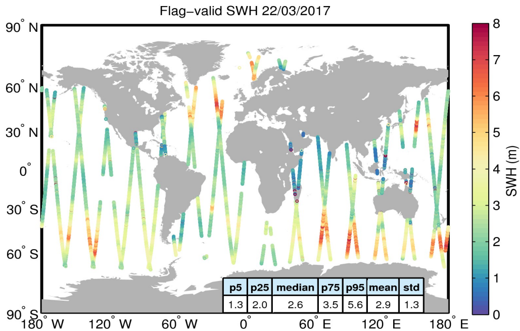
Figure 15. Geographical distribution of flag-valid SWH data over oceans and lakes for 22/03/2017. The statistical values shown in the table refer to the SWH in m and are calculated over all measurements shown in the figure.
