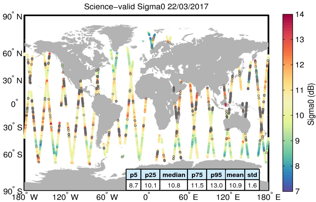
Figure 27. Geographical distribution of science-valid sigma0 data over oceans and lakes for 22/03/2017. The statistical values shown in the table refer to the sigma0 in dB and are calculated over all measurements shown in the figure. Gray circles denote records that have been rejected based on the editing criteria described in Table 4.
