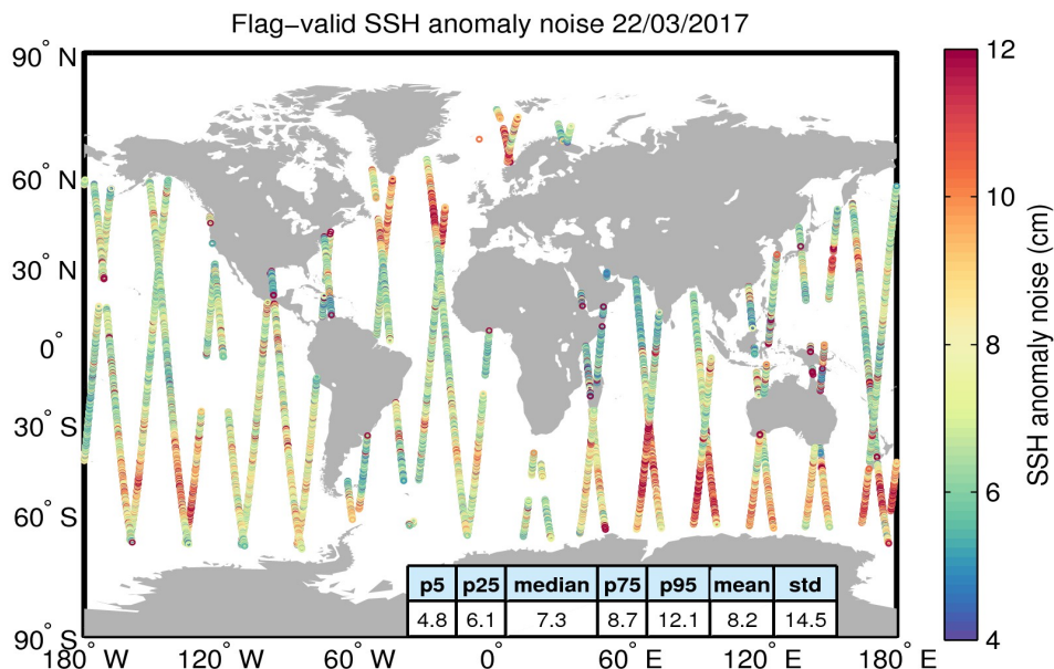
Figure 8. Geographical distribution of flag-valid 20-Hz SSH anomaly measurement noise over oceans and lakes for 22/03/2017. The statistical values shown in the table refer to the SSH anomaly noise and are calculated over all measurements shown in the figure.
