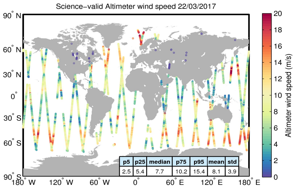
Figure 34. Geographical distribution of science-valid wind data over oceans and lakes for 22/03/2017. The statistical values shown in the table refer to the wind in m/s and are calculated over all measurements shown in the figure. Gray circles denote records that have been rejected based on the editing criteria described in Table 5.
