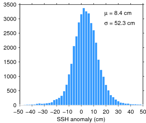
Figure 7. Histogram of flag-valid SSH anomaly over oceans and lakes for 22/03/2017. The mean ( \mu ) and standard deviation ( \sigma ) are also shown. Note that values outside [-50 50] cm are excluded from the histogram for the sake of readability but not from the computation of \mu and \sigma .
