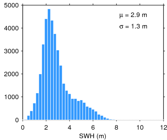
Figure 17. Histogram of flag-valid SWH over oceans and lakes for 22/03/2017. The mean ( \mu ) and standard deviation ( \sigma ) are also shown. Note that values larger than 12 m are excluded from the histogram for the sake of readability but not from the computation of \mu and \sigma .
