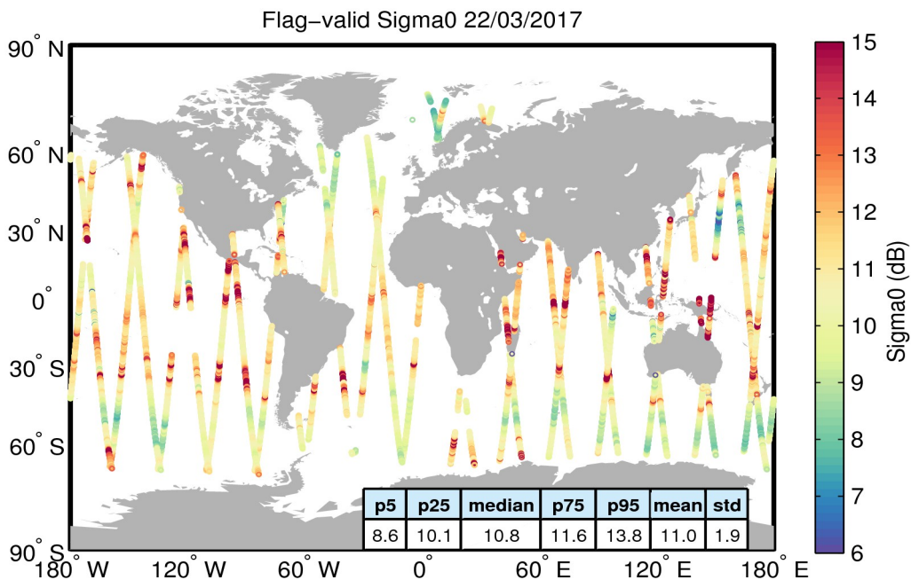
Figure 23. Geographical distribution of flag-valid sigma0 data over oceans and lakes for 22/03/2017. The statistical values shown in the table refer to the sigma0 in dB and are calculated over all measurements shown in the figure.
