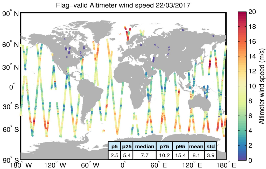
Figure 31. Geographical distribution of flag-valid wind data over oceans and lakes for 22/03/2017. The statistical values shown in the table refer to the wind in m/s and are calculated over all measurements shown in the figure.
