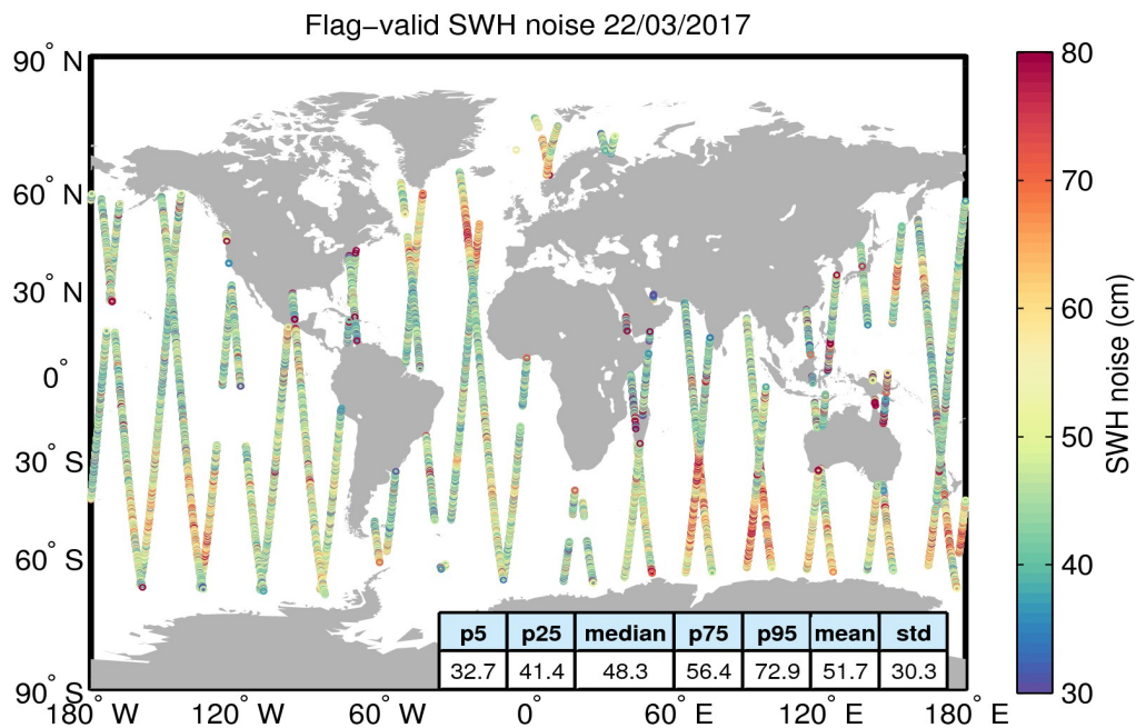
Figure 18. Geographical distribution of flag-valid 20-Hz SWH measurement noise over oceans and lakes for 22/03/2017. The statistical values shown in the table refer to the SWH noise and are calculated over all measurements shown in the figure.
