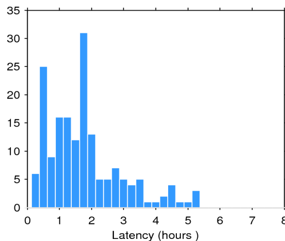
Figure 2. Histogram of the data latency for 21/03/2017. The y-axis denotes the number of files that are made available with a delay of x-hours with respect to the mean time of the records stored in the file.
