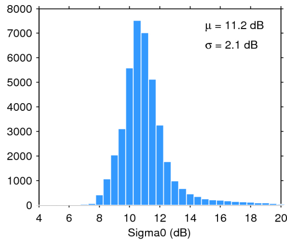
Figure 25. Histogram of flag-valid sigma0 over oceans and lakes for 21/03/2017. The mean ( \mu ) and standard deviation ( \sigma ) are also shown. Note that values outside [4 20] dB are excluded from the histogram for the sake of readability but not from the computation of \mu and \sigma .
