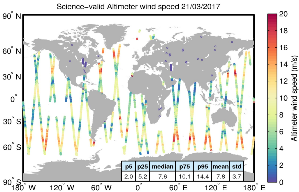
Figure 34. Geographical distribution of science-valid wind data over oceans and lakes for 21/03/2017. The statistical values shown in the table refer to the wind in m/s and are calculated over all measurements shown in the figure. Gray circles denote records that have been rejected based on the editing criteria described in Table 5.
