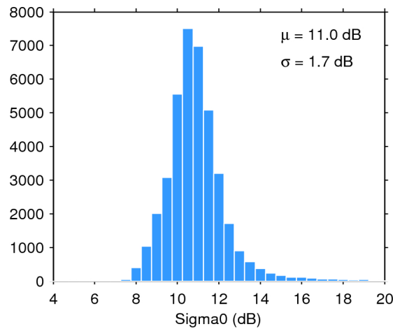
Figure 28. Histogram of science-valid sigma0 over oceans and lakes for 21/03/2017. The mean ( \mu ) and standard deviation ( \sigma ) are also shown. Note that values outside [4 20] dB are excluded from the histogram for the sake of readability but not from the computation of \mu and \sigma .
