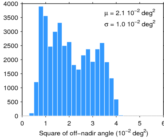
Figure 39. Histogram of flag-valid mispointing over oceans and lakes for 21/03/2017. The mean ( \mu ) and standard deviation ( \sigma ) are also shown. Note that values larger than 6 \cdot 10^{-2} \text{ deg}^2 are excluded from the histogram for the sake of readability but not from the computation of \mu and \sigma .
