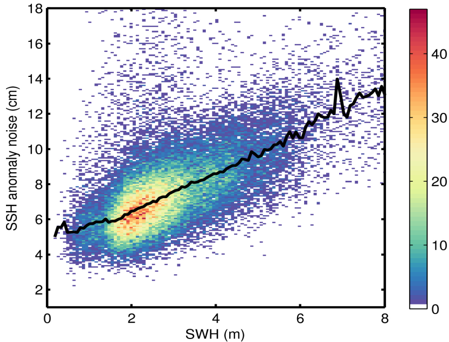
Figure 9. 2D histogram showing flag-valid SSH anomaly noise as a function of SWH for 21/03/2017. The black line denotes the median SSH anomaly noise as a function of SWH.
