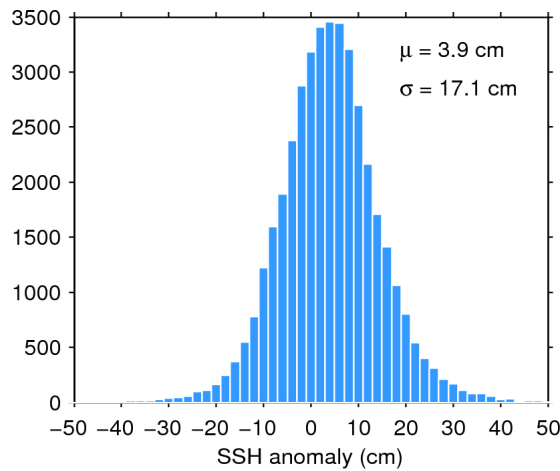
Figure 7. Histogram of flag-valid SSH anomaly over oceans and lakes for 21/03/2017. The mean ( \mu ) and standard deviation ( \sigma ) are also shown. Note that values outside [-50 50] cm are excluded from the histogram for the sake of readability but not from the computation of \mu and \sigma .
