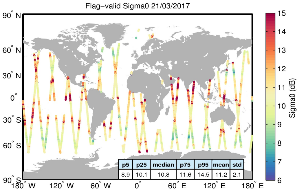
Figure 23. Geographical distribution of flag-valid sigma0 data over oceans and lakes for 21/03/2017. The statistical values shown in the table refer to the sigma0 in dB and are calculated over all measurements shown in the figure.
