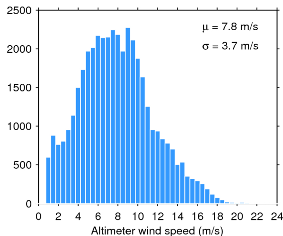
Figure 35. Histogram of science-valid wind over oceans and lakes for 21/03/2017. The mean ( \mu ) and standard deviation ( \sigma ) are also shown. Note that values larger than 24 m/s are excluded from the histogram for the sake of readability but not from the computation of \mu and \sigma .
