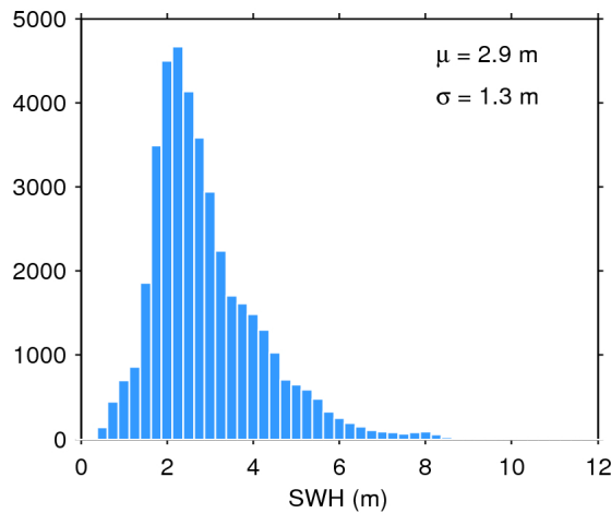
Figure 20. Histogram of science-valid SWH over oceans and lakes for 21/03/2017. The mean ( \mu ) and standard deviation ( \sigma ) are also shown. Note that values larger than 12 m are excluded from the histogram for the sake of readability but not from the computation of \mu and \sigma .
