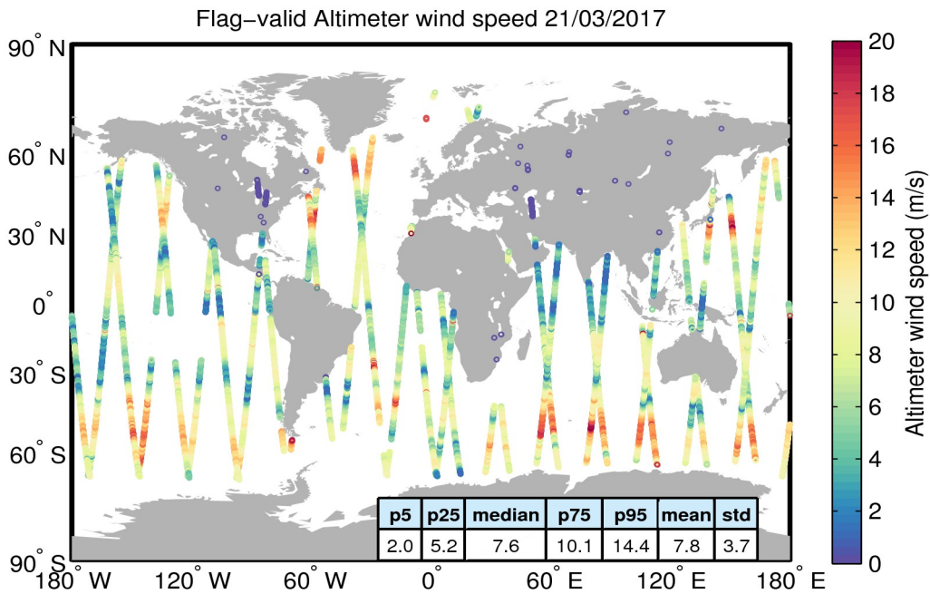
Figure 31. Geographical distribution of flag-valid wind data over oceans and lakes for 21/03/2017. The statistical values shown in the table refer to the wind in m/s and are calculated over all measurements shown in the figure.
