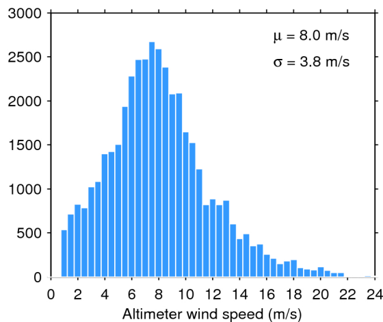
Figure 35. Histogram of science-valid wind over oceans and lakes for 19/03/2017. The mean ( \mu ) and standard deviation ( \sigma ) are also shown. Note that values larger than 24 m/s are excluded from the histogram for the sake of readability but not from the computation of \mu and \sigma .
