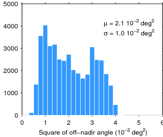
Figure 39. Histogram of flag-valid mispointing over oceans and lakes for 19/03/2017. The mean ( \mu ) and standard deviation ( \sigma ) are also shown. Note that values larger than 6 \cdot 10^{-2} \text{ deg}^2 are excluded from the histogram for the sake of readability but not from the computation of \mu and \sigma .
