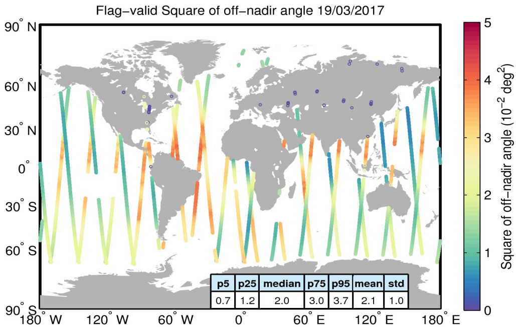
Figure 37. Geographical distribution of flag-valid mispointing data over oceans and lakes for 19/03/2017. The statistical values shown in the table refer to the mispointing in 10^{-2} deg 2 and are calculated over all measurements shown in the figure.
