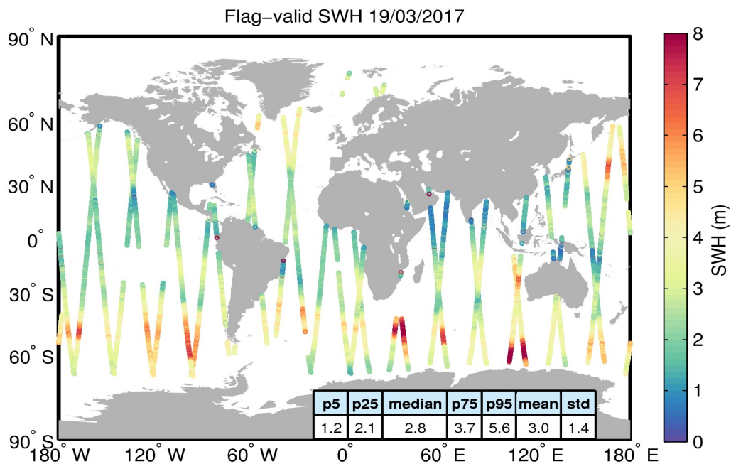
Figure 15. Geographical distribution of flag-valid SWH data over oceans and lakes for 19/03/2017. The statistical values shown in the table refer to the SWH in m and are calculated over all measurements shown in the figure.
