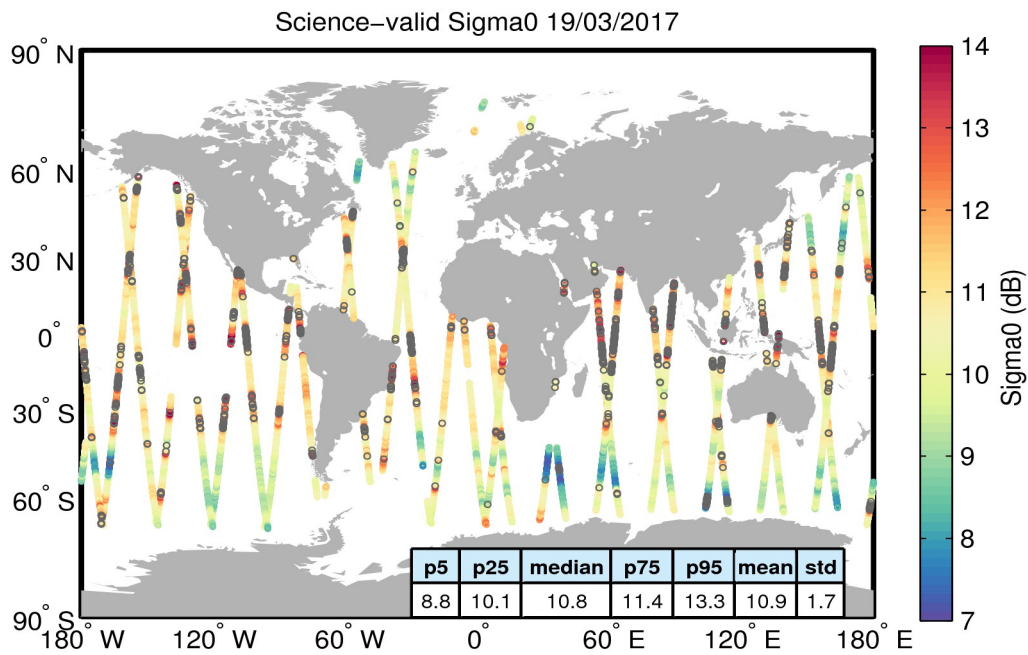
Figure 27. Geographical distribution of science-valid sigma0 data over oceans and lakes for 19/03/2017. The statistical values shown in the table refer to the sigma0 in dB and are calculated over all measurements shown in the figure. Gray circles denote records that have been rejected based on the editing criteria described in Table 4.
