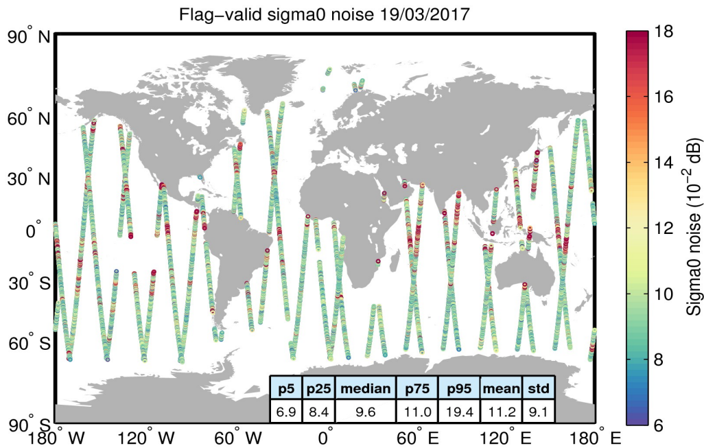
Figure 26. Geographical distribution of flag-valid 20-Hz sigma0 measurement noise over oceans and lakes for 19/03/2017. The statistical values shown in the table refer to the sigma0 noise and are calculated over all measurements shown in the figure.
