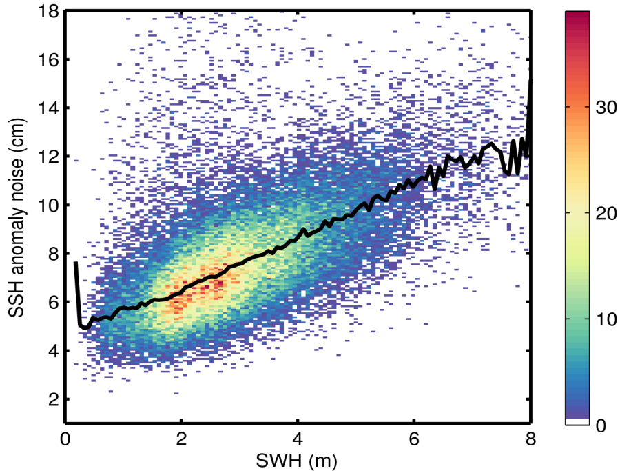
Figure 9. 2D histogram showing flag-valid SSH anomaly noise as a function of SWH for 19/03/2017. The black line denotes the median SSH anomaly noise as a function of SWH.
