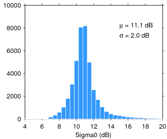
Figure 25. Histogram of flag-valid sigma0 over oceans and lakes for 19/03/2017. The mean ( \mu ) and standard deviation ( \sigma ) are also shown. Note that values outside [4 20] dB are excluded from the histogram for the sake of readability but not from the computation of \mu and \sigma .
