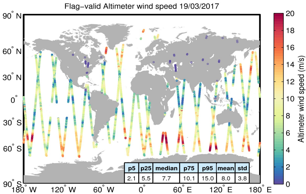
Figure 31. Geographical distribution of flag-valid wind data over oceans and lakes for 19/03/2017. The statistical values shown in the table refer to the wind in m/s and are calculated over all measurements shown in the figure.
