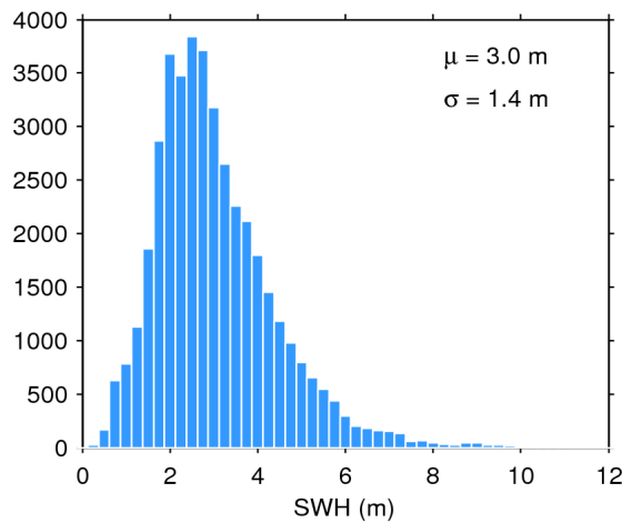
Figure 17. Histogram of flag-valid SWH over oceans and lakes for 19/03/2017. The mean ( \mu ) and standard deviation ( \sigma ) are also shown. Note that values larger than 12 m are excluded from the histogram for the sake of readability but not from the computation of \mu and \sigma .
