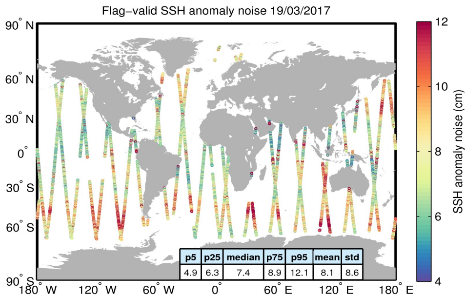
Figure 8. Geographical distribution of flag-valid 20-Hz SSH anomaly measurement noise over oceans and lakes for 19/03/2017. The statistical values shown in the table refer to the SSH anomaly noise and are calculated over all measurements shown in the figure.
