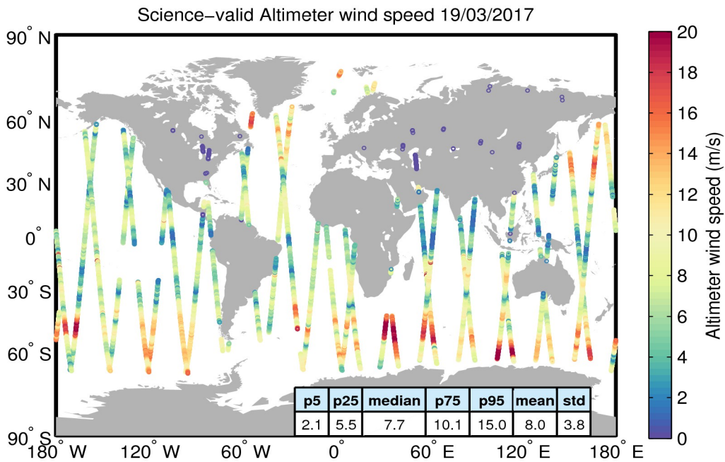
Figure 34. Geographical distribution of science-valid wind data over oceans and lakes for 19/03/2017. The statistical values shown in the table refer to the wind in m/s and are calculated over all measurements shown in the figure. Gray circles denote records that have been rejected based on the editing criteria described in Table 5.
