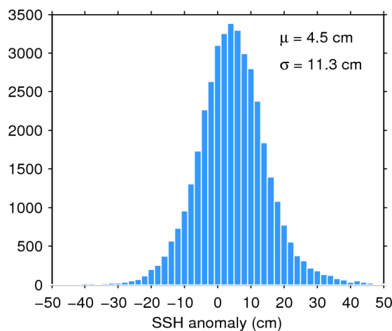
Figure 11. Histogram of science-valid SSH anomaly over oceans and lakes for 19/03/2017. The mean ( \mu ) and standard deviation ( \sigma ) are also shown. Note that values outside [-50 50] cm are excluded from the histogram for the sake of readability but not from the computation of \mu and \sigma .
