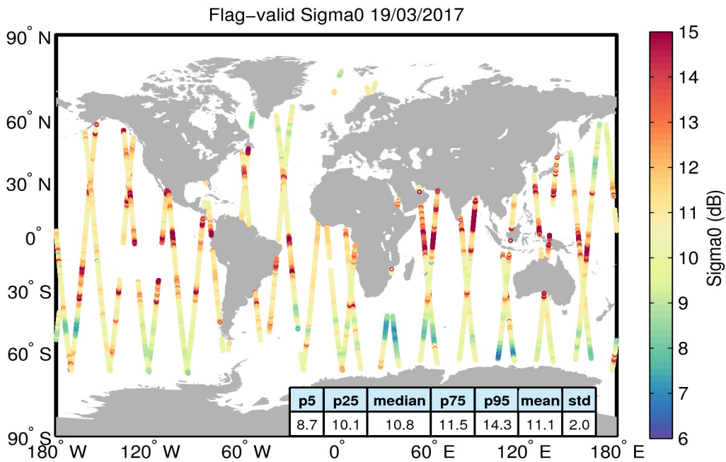
Figure 23. Geographical distribution of flag-valid sigma0 data over oceans and lakes for 19/03/2017. The statistical values shown in the table refer to the sigma0 in dB and are calculated over all measurements shown in the figure.
