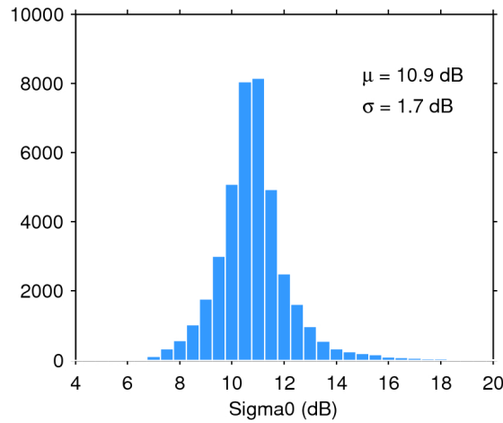
Figure 28. Histogram of science-valid sigma0 over oceans and lakes for 19/03/2017. The mean ( \mu ) and standard deviation ( \sigma ) are also shown. Note that values outside [4 20] dB are excluded from the histogram for the sake of readability but not from the computation of \mu and \sigma .
