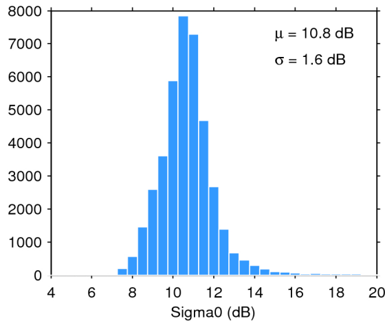
Figure 28. Histogram of science-valid sigma0 over oceans and lakes for 17/03/2017. The mean ( \mu ) and standard deviation ( \sigma ) are also shown. Note that values outside [4 20] dB are excluded from the histogram for the sake of readability but not from the computation of \mu and \sigma .
