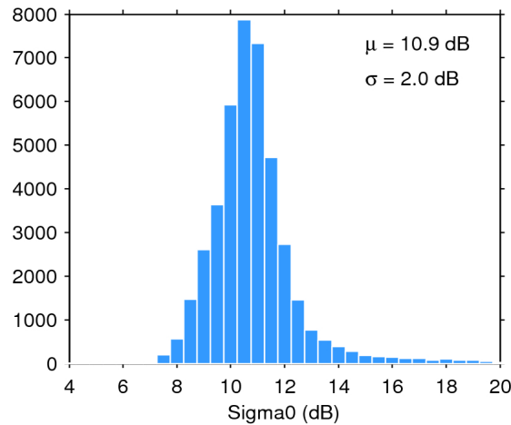
Figure 25. Histogram of flag-valid sigma0 over oceans and lakes for 17/03/2017. The mean ( \mu ) and standard deviation ( \sigma ) are also shown. Note that values outside [4 20] dB are excluded from the histogram for the sake of readability but not from the computation of \mu and \sigma .
