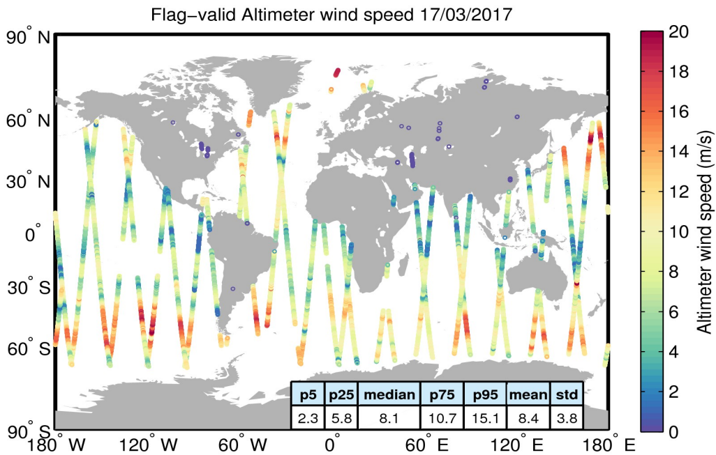
Figure 31. Geographical distribution of flag-valid wind data over oceans and lakes for 17/03/2017. The statistical values shown in the table refer to the wind in m/s and are calculated over all measurements shown in the figure.
