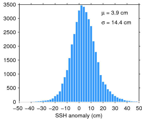
Figure 7. Histogram of flag-valid SSH anomaly over oceans and lakes for 17/03/2017. The mean ( \mu ) and standard deviation ( \sigma ) are also shown. Note that values outside [-50 50] cm are excluded from the histogram for the sake of readability but not from the computation of \mu and \sigma .
