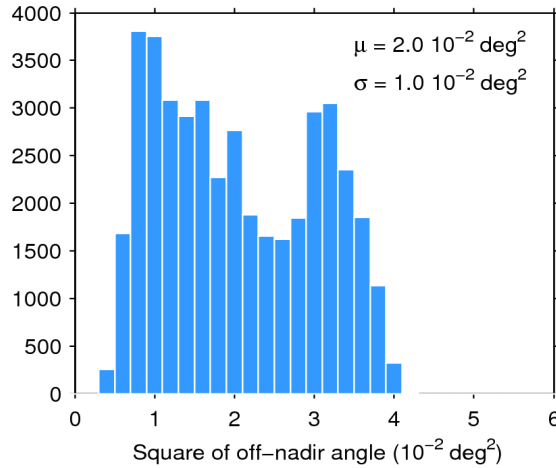
Figure 39. Histogram of flag-valid mispointing over oceans and lakes for 17/03/2017. The mean ( \mu ) and standard deviation ( \sigma ) are also shown. Note that values larger than 6 \cdot 10^{-2} \text{ deg}^2 are excluded from the histogram for the sake of readability but not from the computation of \mu and \sigma .
