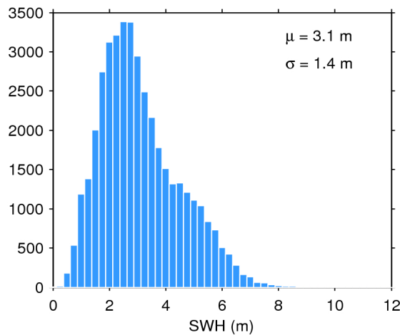
Figure 20. Histogram of science-valid SWH over oceans and lakes for 17/03/2017. The mean ( \mu ) and standard deviation ( \sigma ) are also shown. Note that values larger than 12 m are excluded from the histogram for the sake of readability but not from the computation of \mu and \sigma .
