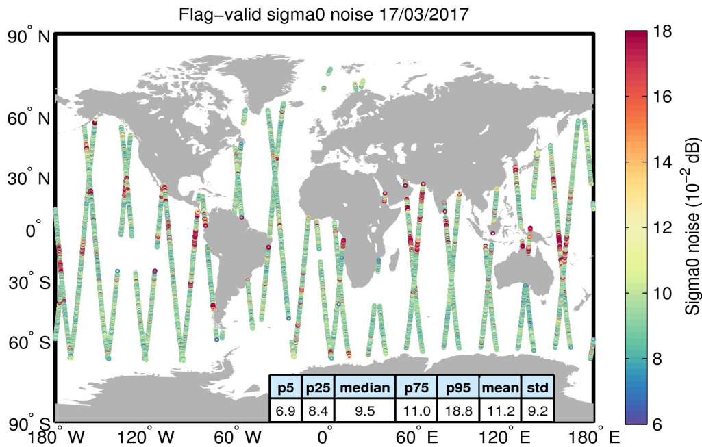
Figure 26. Geographical distribution of flag-valid 20-Hz sigma0 measurement noise over oceans and lakes for 17/03/2017. The statistical values shown in the table refer to the sigma0 noise and are calculated over all measurements shown in the figure.
