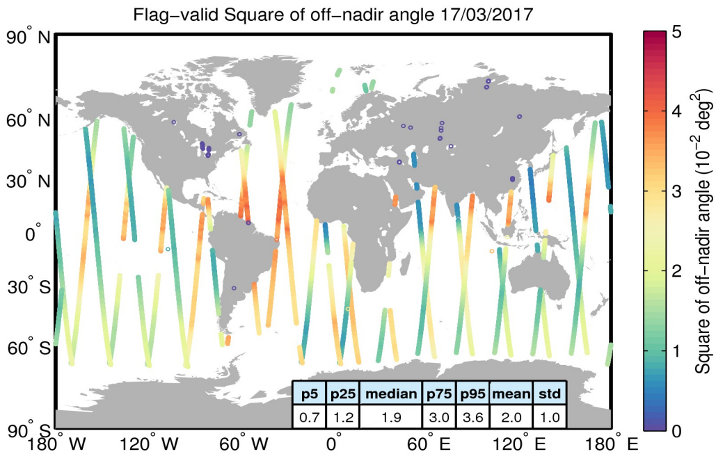
Figure 37. Geographical distribution of flag-valid mispointing data over oceans and lakes for 17/03/2017. The statistical values shown in the table refer to the mispointing in 10^{-2} deg 2 and are calculated over all measurements shown in the figure.
