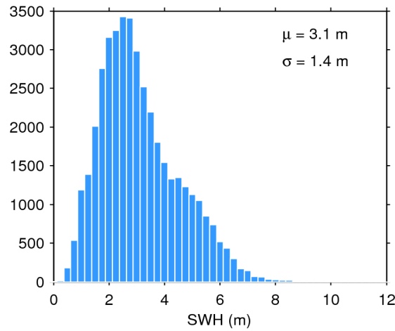
Figure 17. Histogram of flag-valid SWH over oceans and lakes for 17/03/2017. The mean ( \mu ) and standard deviation ( \sigma ) are also shown. Note that values larger than 12 m are excluded from the histogram for the sake of readability but not from the computation of \mu and \sigma .
