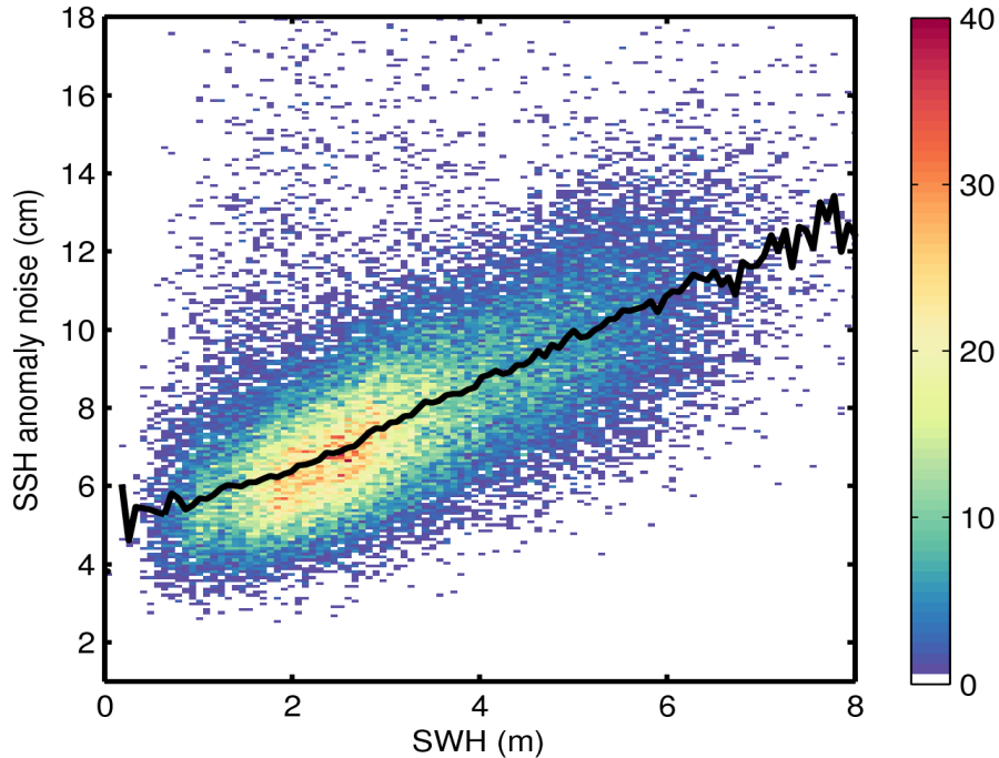
Figure 9. 2D histogram showing flag-valid SSH anomaly noise as a function of SWH for 17/03/2017. The black line denotes the median SSH anomaly noise as a function of SWH.
