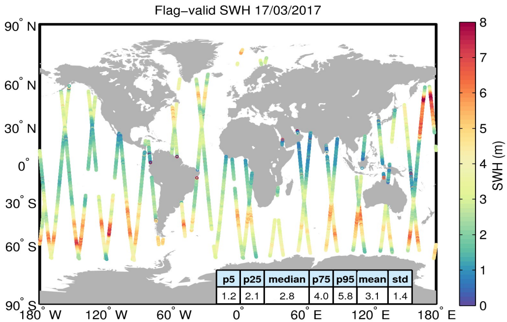
Figure 15. Geographical distribution of flag-valid SWH data over oceans and lakes for 17/03/2017. The statistical values shown in the table refer to the SWH in m and are calculated over all measurements shown in the figure.
