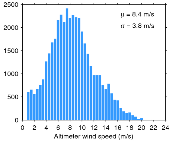
Figure 33. Histogram of flag-valid wind over oceans and lakes for 17/03/2017. The mean ( \mu ) and standard deviation ( \sigma ) are also shown. Note that values larger than 24 m/s are excluded from the histogram for the sake of readability but not from the computation of \mu and \sigma .
