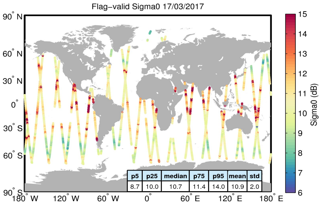
Figure 23. Geographical distribution of flag-valid sigma0 data over oceans and lakes for 17/03/2017. The statistical values shown in the table refer to the sigma0 in dB and are calculated over all measurements shown in the figure.
