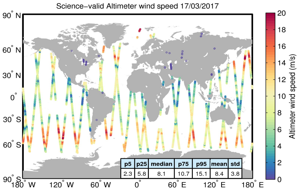
Figure 34. Geographical distribution of science-valid wind data over oceans and lakes for 17/03/2017. The statistical values shown in the table refer to the wind in m/s and are calculated over all measurements shown in the figure. Gray circles denote records that have been rejected based on the editing criteria described in Table 5.
