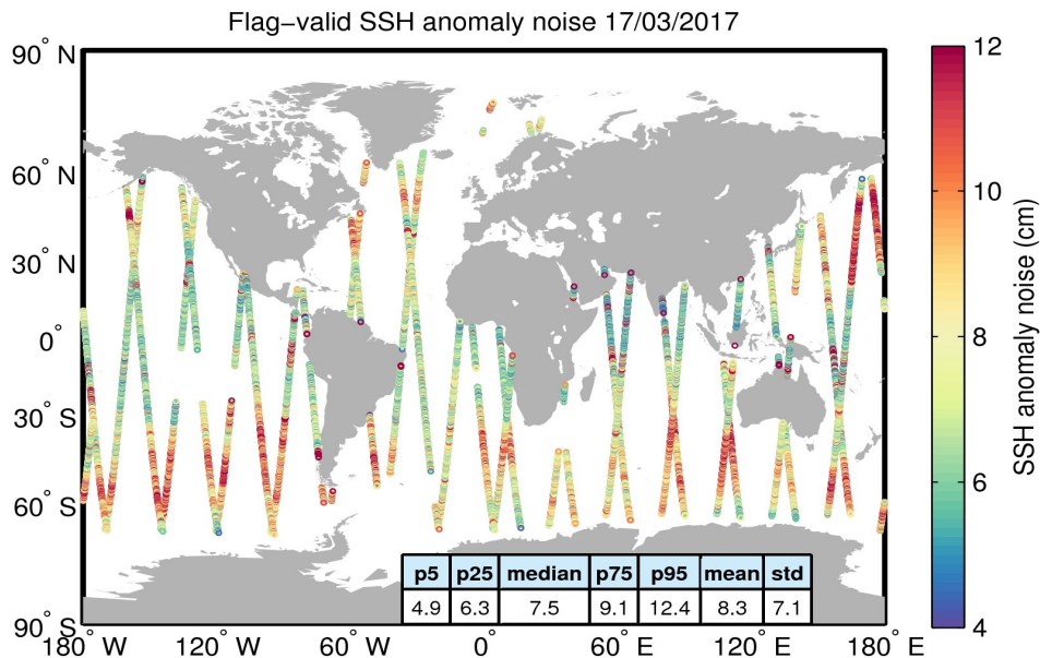
Figure 8. Geographical distribution of flag-valid 20-Hz SSH anomaly measurement noise over oceans and lakes for 17/03/2017. The statistical values shown in the table refer to the SSH anomaly noise and are calculated over all measurements shown in the figure.
