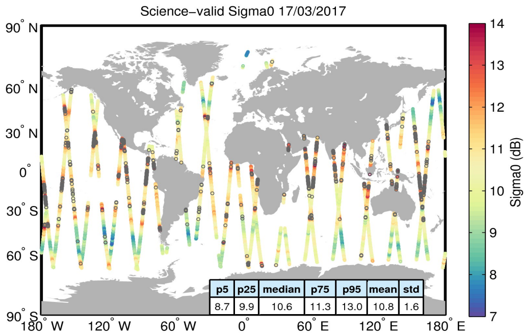
Figure 27. Geographical distribution of science-valid sigma0 data over oceans and lakes for 17/03/2017. The statistical values shown in the table refer to the sigma0 in dB and are calculated over all measurements shown in the figure. Gray circles denote records that have been rejected based on the editing criteria described in Table 4.
