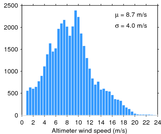
Figure 35. Histogram of science-valid wind over oceans and lakes for 15/03/2017. The mean ( \mu ) and standard deviation ( \sigma ) are also shown. Note that values larger than 24 m/s are excluded from the histogram for the sake of readability but not from the computation of \mu and \sigma .
