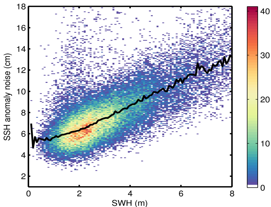
Figure 9. 2D histogram showing flag-valid SSH anomaly noise as a function of SWH for 15/03/2017. The black line denotes the median SSH anomaly noise as a function of SWH.
