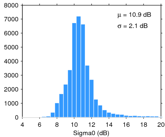
Figure 25. Histogram of flag-valid sigma0 over oceans and lakes for 15/03/2017. The mean ( \mu ) and standard deviation ( \sigma ) are also shown. Note that values outside [4 20] dB are excluded from the histogram for the sake of readability but not from the computation of \mu and \sigma .
