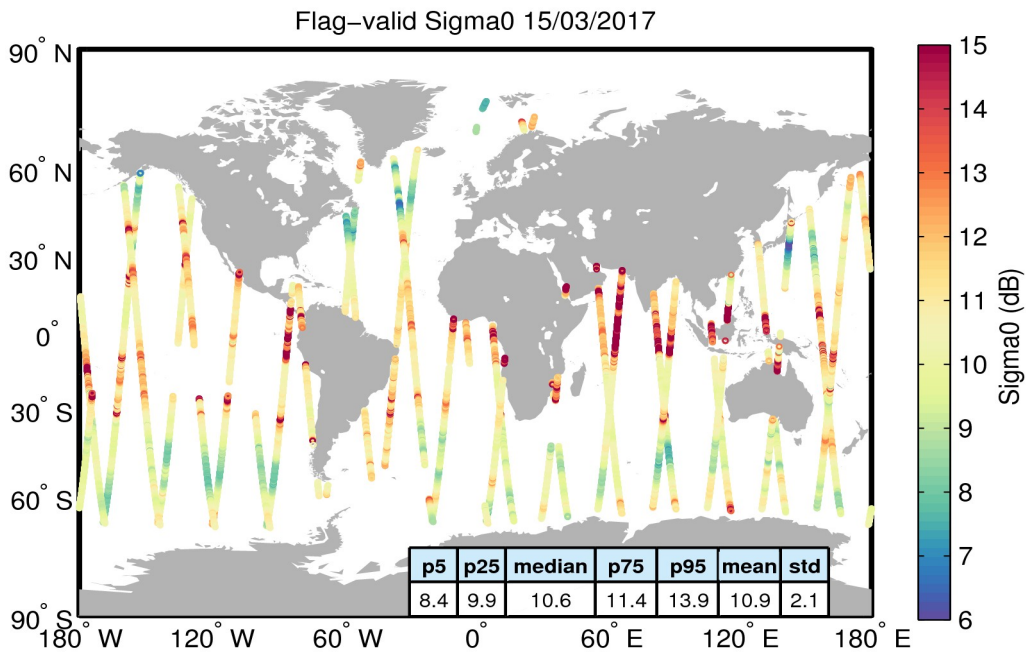
Figure 23. Geographical distribution of flag-valid sigma0 data over oceans and lakes for 15/03/2017. The statistical values shown in the table refer to the sigma0 in dB and are calculated over all measurements shown in the figure.
