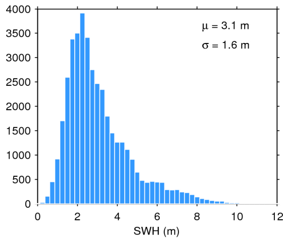
Figure 17. Histogram of flag-valid SWH over oceans and lakes for 15/03/2017. The mean ( \mu ) and standard deviation ( \sigma ) are also shown. Note that values larger than 12 m are excluded from the histogram for the sake of readability but not from the computation of \mu and \sigma .
