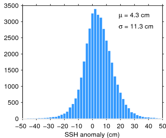
Figure 11. Histogram of science-valid SSH anomaly over oceans and lakes for 15/03/2017. The mean ( \mu ) and standard deviation ( \sigma ) are also shown. Note that values outside [-50 50] cm are excluded from the histogram for the sake of readability but not from the computation of \mu and \sigma .
