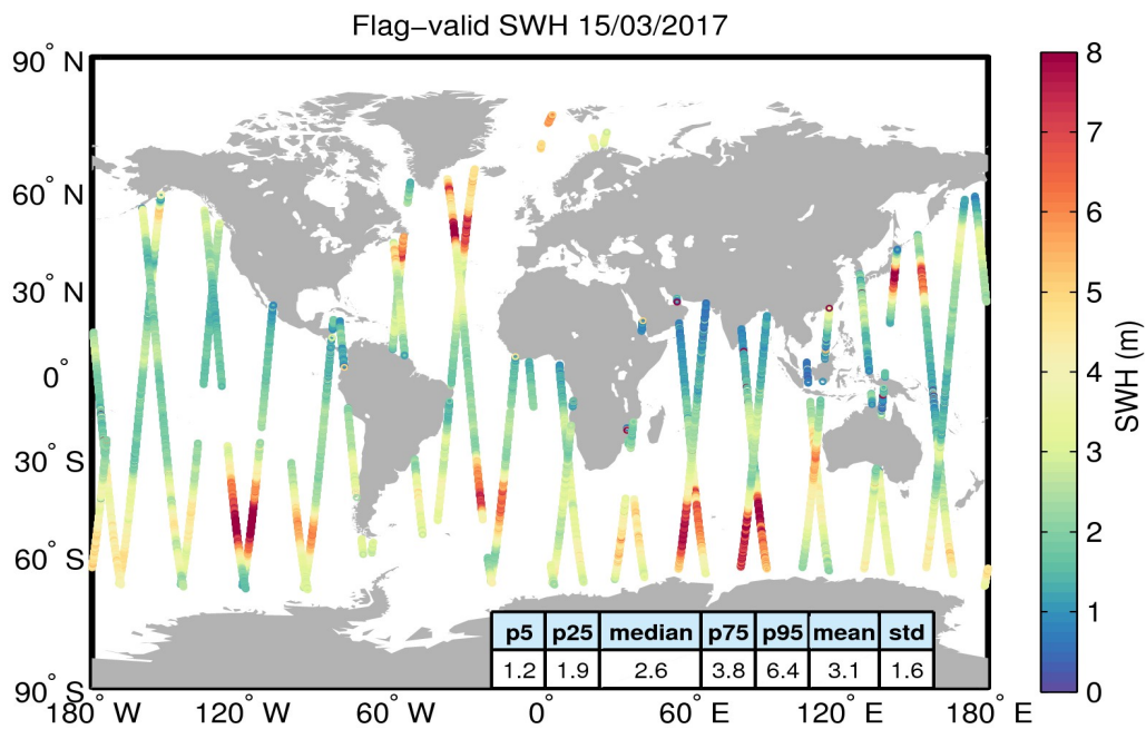
Figure 15. Geographical distribution of flag-valid SWH data over oceans and lakes for 15/03/2017. The statistical values shown in the table refer to the SWH in m and are calculated over all measurements shown in the figure.
