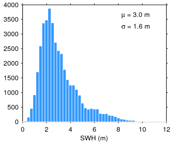
Figure 20. Histogram of science-valid SWH over oceans and lakes for 15/03/2017. The mean ( \mu ) and standard deviation ( \sigma ) are also shown. Note that values larger than 12 m are excluded from the histogram for the sake of readability but not from the computation of \mu and \sigma .
