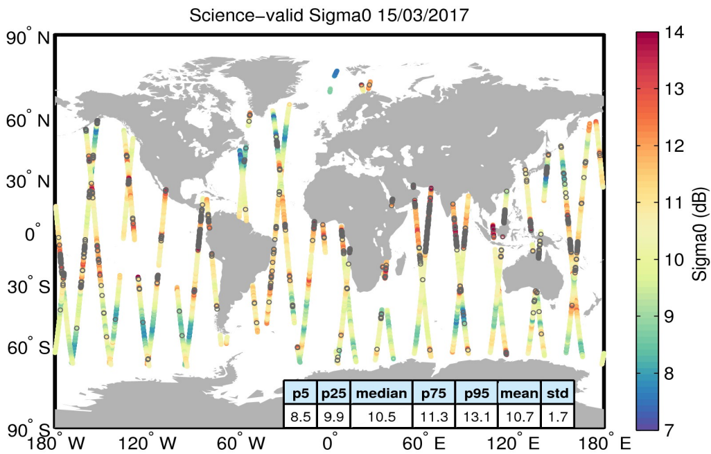
Figure 27. Geographical distribution of science-valid sigma0 data over oceans and lakes for 15/03/2017. The statistical values shown in the table refer to the sigma0 in dB and are calculated over all measurements shown in the figure. Gray circles denote records that have been rejected based on the editing criteria described in Table 4.
