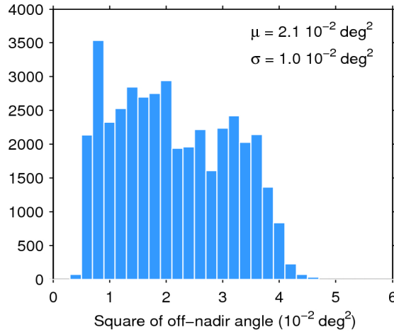
Figure 39. Histogram of flag-valid mispointing over oceans and lakes for 15/03/2017. The mean ( \mu ) and standard deviation ( \sigma ) are also shown. Note that values larger than 6 \cdot 10^{-2} \text{ deg}^2 are excluded from the histogram for the sake of readability but not from the computation of \mu and \sigma .
