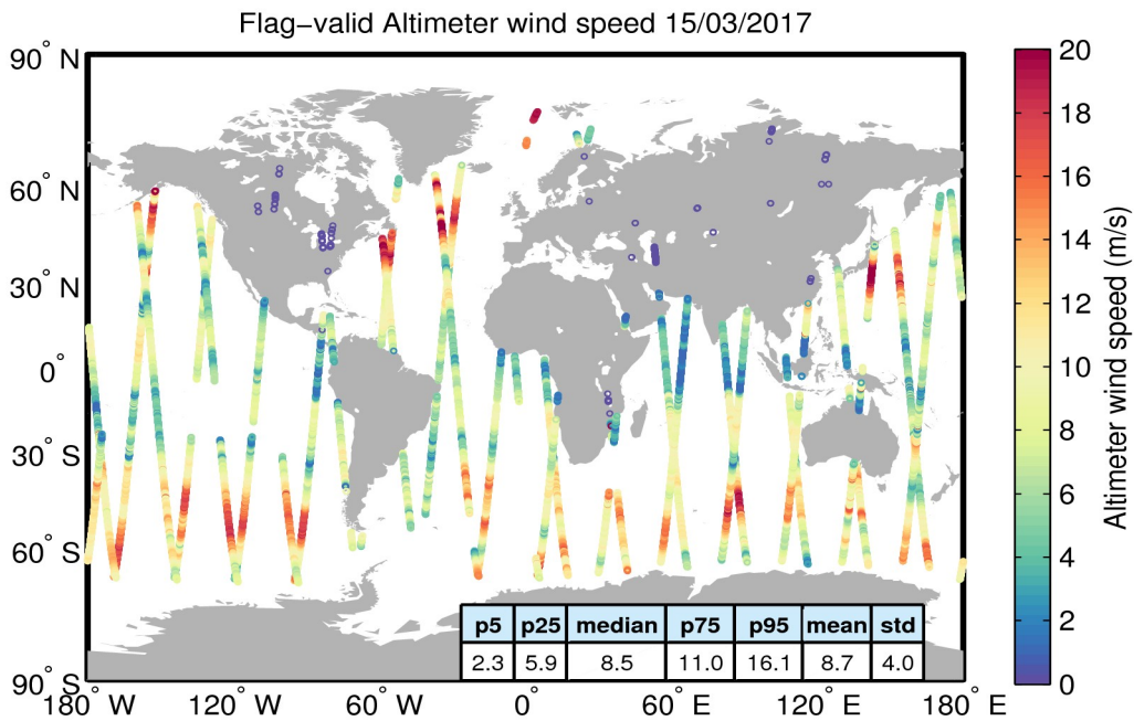
Figure 31. Geographical distribution of flag-valid wind data over oceans and lakes for 15/03/2017. The statistical values shown in the table refer to the wind in m/s and are calculated over all measurements shown in the figure.
