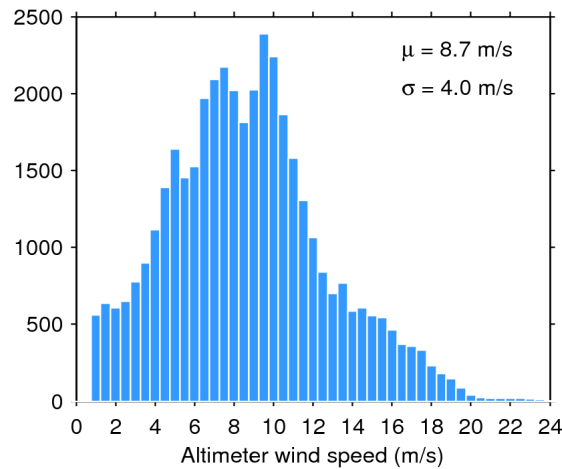
Figure 33. Histogram of flag-valid wind over oceans and lakes for 15/03/2017. The mean ( \mu ) and standard deviation ( \sigma ) are also shown. Note that values larger than 24 m/s are excluded from the histogram for the sake of readability but not from the computation of \mu and \sigma .
