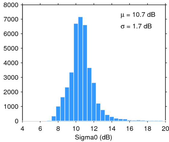
Figure 28. Histogram of science-valid sigma0 over oceans and lakes for 15/03/2017. The mean ( \mu ) and standard deviation ( \sigma ) are also shown. Note that values outside [4 20] dB are excluded from the histogram for the sake of readability but not from the computation of \mu and \sigma .
