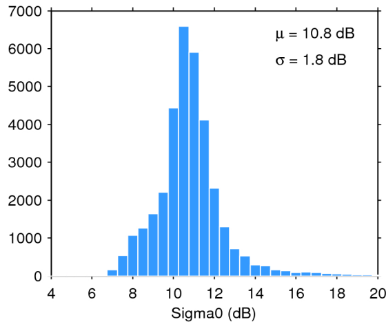
Figure 28. Histogram of science-valid sigma0 over oceans and lakes for 14/03/2017. The mean ( \mu ) and standard deviation ( \sigma ) are also shown. Note that values outside [4 20] dB are excluded from the histogram for the sake of readability but not from the computation of \mu and \sigma .
