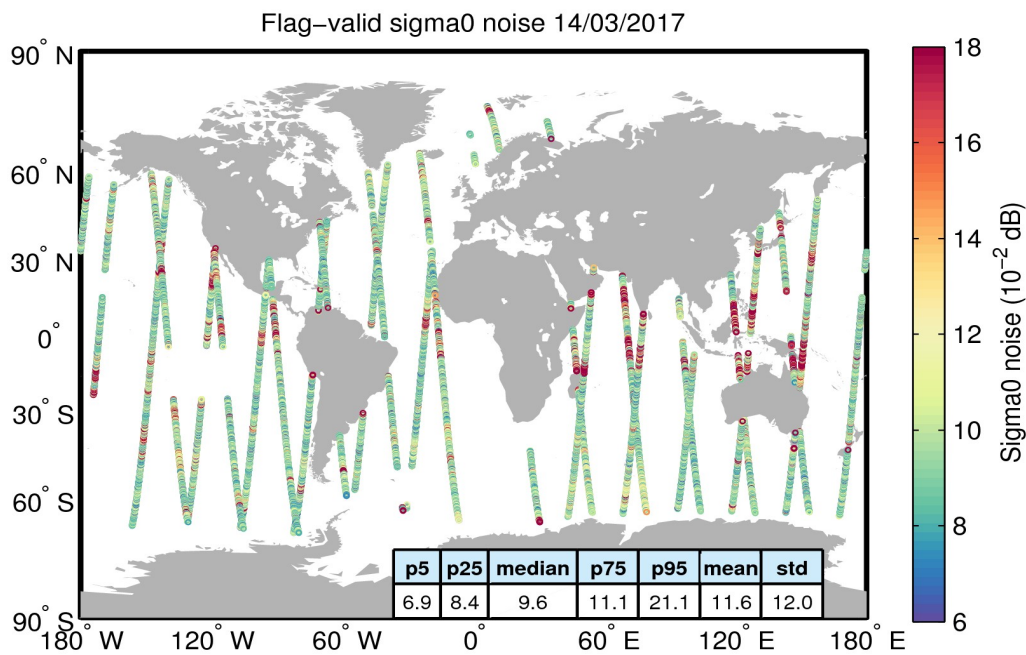
Figure 26. Geographical distribution of flag-valid 20-Hz sigma0 measurement noise over oceans and lakes for 14/03/2017. The statistical values shown in the table refer to the sigma0 noise and are calculated over all measurements shown in the figure.
