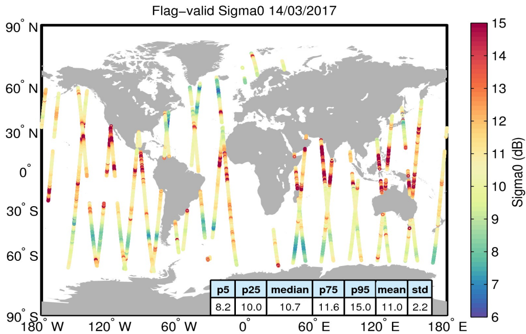
Figure 23. Geographical distribution of flag-valid sigma0 data over oceans and lakes for 14/03/2017. The statistical values shown in the table refer to the sigma0 in dB and are calculated over all measurements shown in the figure.
