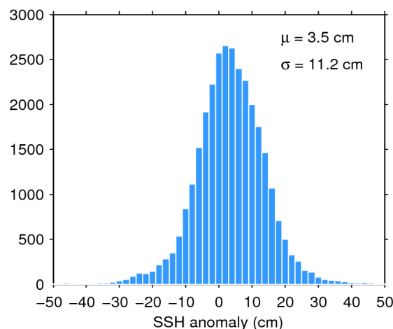
Figure 11. Histogram of science-valid SSH anomaly over oceans and lakes for 14/03/2017. The mean ( \mu ) and standard deviation ( \sigma ) are also shown. Note that values outside [-50 50] cm are excluded from the histogram for the sake of readability but not from the computation of \mu and \sigma .
