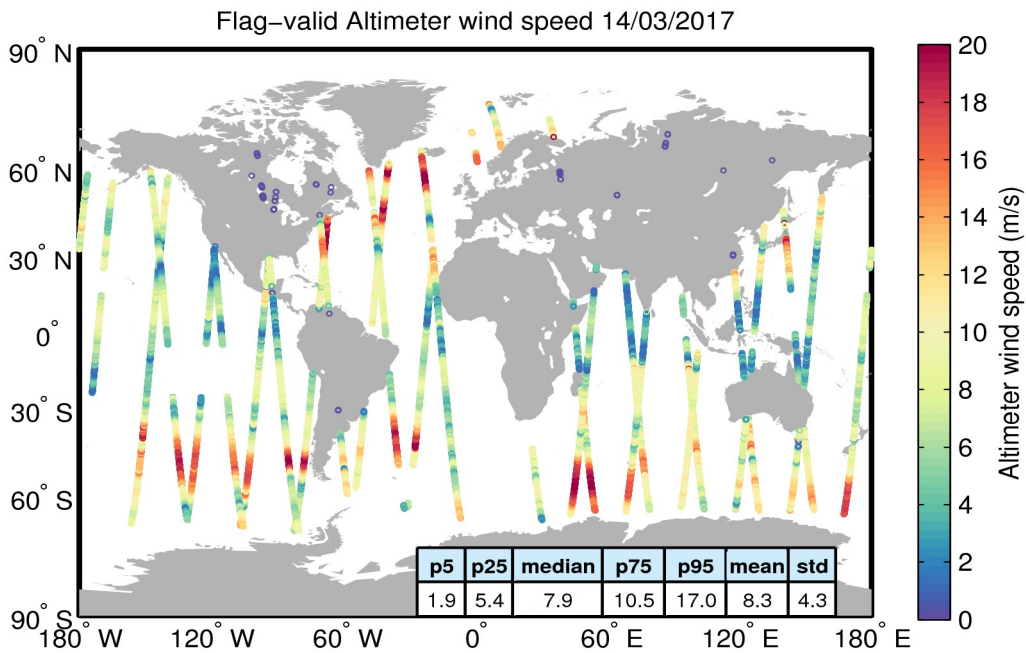
Figure 31. Geographical distribution of flag-valid wind data over oceans and lakes for 14/03/2017. The statistical values shown in the table refer to the wind in m/s and are calculated over all measurements shown in the figure.
