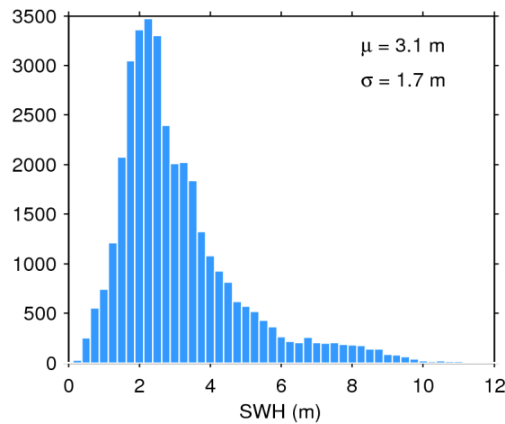
Figure 17. Histogram of flag-valid SWH over oceans and lakes for 14/03/2017. The mean ( \mu ) and standard deviation ( \sigma ) are also shown. Note that values larger than 12 m are excluded from the histogram for the sake of readability but not from the computation of \mu and \sigma .
