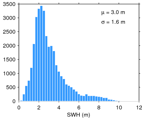
Figure 20. Histogram of science-valid SWH over oceans and lakes for 14/03/2017. The mean ( \mu ) and standard deviation ( \sigma ) are also shown. Note that values larger than 12 m are excluded from the histogram for the sake of readability but not from the computation of \mu and \sigma .
