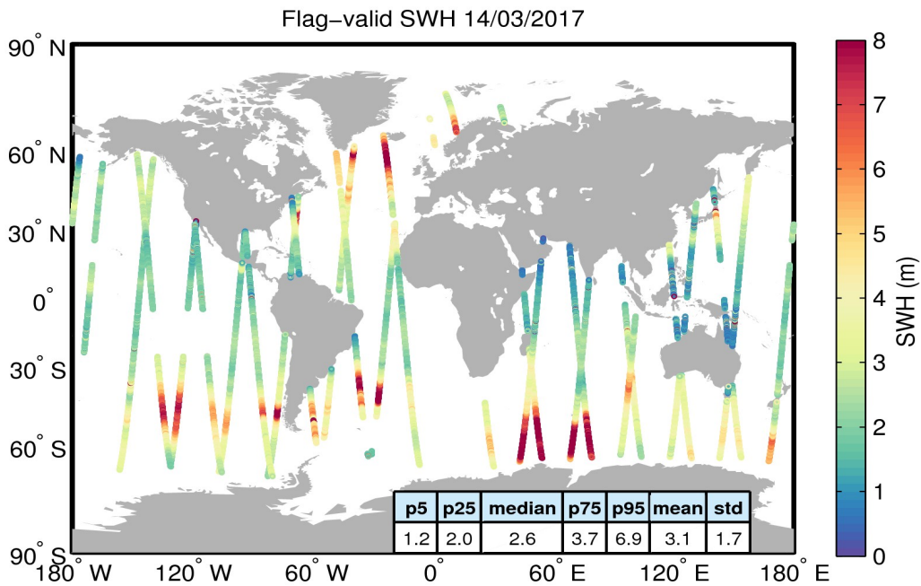
Figure 15. Geographical distribution of flag-valid SWH data over oceans and lakes for 14/03/2017. The statistical values shown in the table refer to the SWH in m and are calculated over all measurements shown in the figure.
