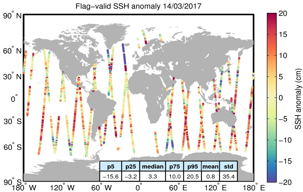
Figure 5. Geographical distribution of flag-valid 1-Hz SSH anomaly data over oceans and lakes for 14/03/2017. The statistical values shown in the table refer to the SSH anomaly in cm and are calculated over all measurements shown in the figure.
