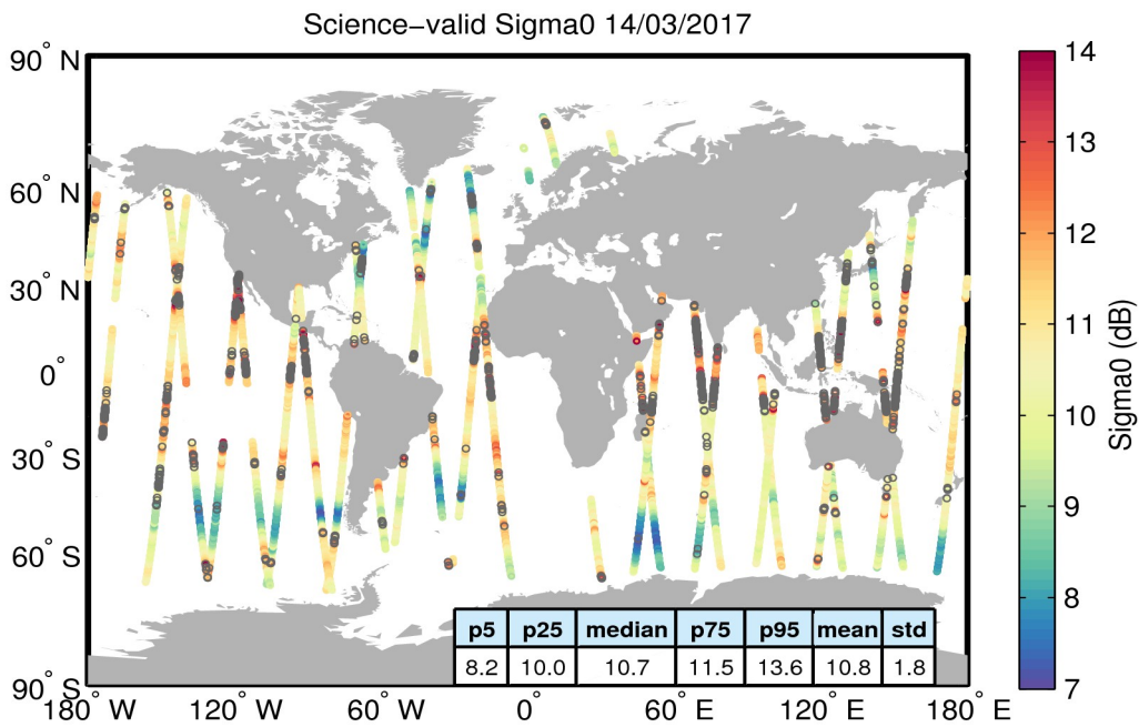
Figure 27. Geographical distribution of science-valid sigma0 data over oceans and lakes for 14/03/2017. The statistical values shown in the table refer to the sigma0 in dB and are calculated over all measurements shown in the figure. Gray circles denote records that have been rejected based on the editing criteria described in Table 4.
