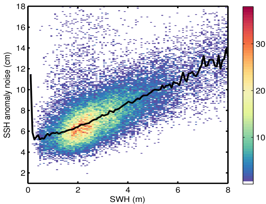
Figure 9. 2D histogram showing flag-valid SSH anomaly noise as a function of SWH for 14/03/2017. The black line denotes the median SSH anomaly noise as a function of SWH.
