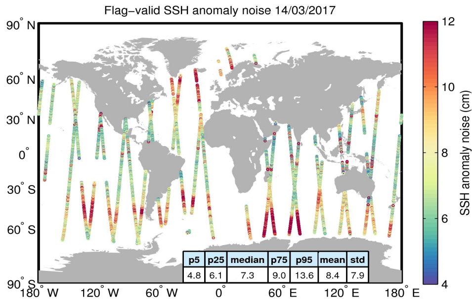
Figure 8. Geographical distribution of flag-valid 20-Hz SSH anomaly measurement noise over oceans and lakes for 14/03/2017. The statistical values shown in the table refer to the SSH anomaly noise and are calculated over all measurements shown in the figure.
