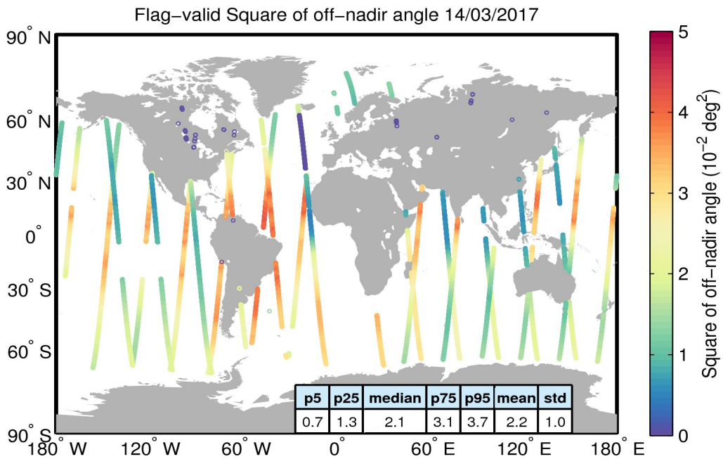
Figure 37. Geographical distribution of flag-valid mispointing data over oceans and lakes for 14/03/2017. The statistical values shown in the table refer to the mispointing in 10^{-2} deg 2 and are calculated over all measurements shown in the figure.
