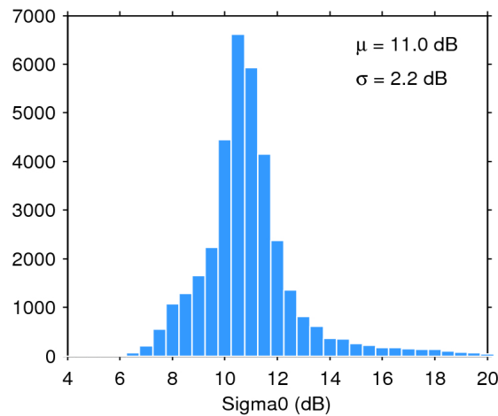
Figure 25. Histogram of flag-valid sigma0 over oceans and lakes for 14/03/2017. The mean ( \mu ) and standard deviation ( \sigma ) are also shown. Note that values outside [4 20] dB are excluded from the histogram for the sake of readability but not from the computation of \mu and \sigma .
