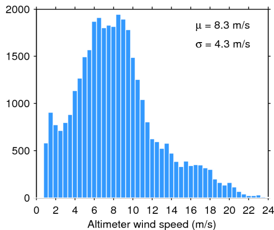
Figure 35. Histogram of science-valid wind over oceans and lakes for 14/03/2017. The mean ( \mu ) and standard deviation ( \sigma ) are also shown. Note that values larger than 24 m/s are excluded from the histogram for the sake of readability but not from the computation of \mu and \sigma .
