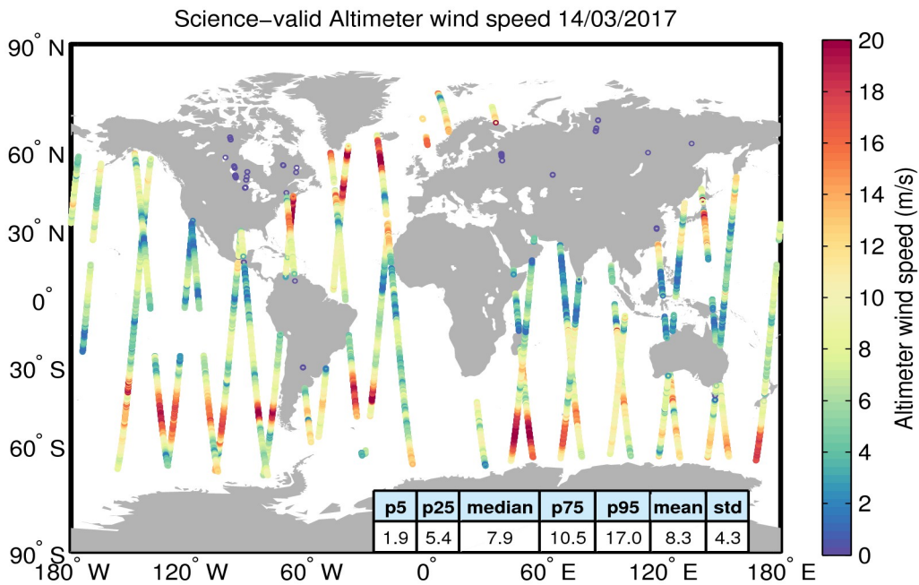
Figure 34. Geographical distribution of science-valid wind data over oceans and lakes for 14/03/2017. The statistical values shown in the table refer to the wind in m/s and are calculated over all measurements shown in the figure. Gray circles denote records that have been rejected based on the editing criteria described in Table 5.
