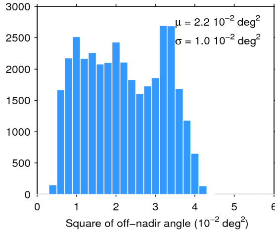
Figure 39. Histogram of flag-valid mispointing over oceans and lakes for 14/03/2017. The mean ( \mu ) and standard deviation ( \sigma ) are also shown. Note that values larger than 6 \cdot 10^{-2} \text{ deg}^2 are excluded from the histogram for the sake of readability but not from the computation of \mu and \sigma .
