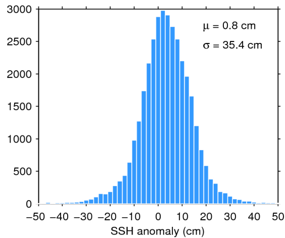
Figure 7. Histogram of flag-valid SSH anomaly over oceans and lakes for 14/03/2017. The mean ( \mu ) and standard deviation ( \sigma ) are also shown. Note that values outside [-50 50] cm are excluded from the histogram for the sake of readability but not from the computation of \mu and \sigma .
