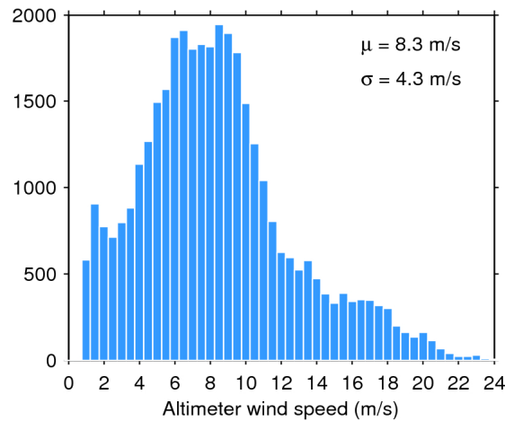
Figure 33. Histogram of flag-valid wind over oceans and lakes for 14/03/2017. The mean ( \mu ) and standard deviation ( \sigma ) are also shown. Note that values larger than 24 m/s are excluded from the histogram for the sake of readability but not from the computation of \mu and \sigma .
