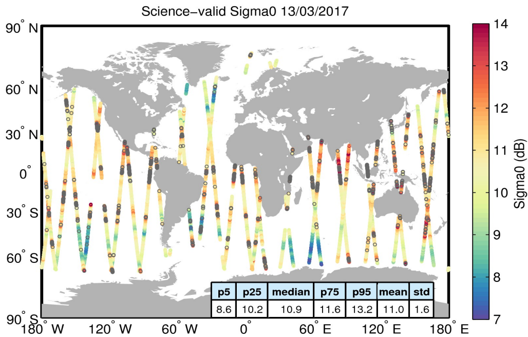
Figure 27. Geographical distribution of science-valid sigma0 data over oceans and lakes for 13/03/2017. The statistical values shown in the table refer to the sigma0 in dB and are calculated over all measurements shown in the figure. Gray circles denote records that have been rejected based on the editing criteria described in Table 4.
