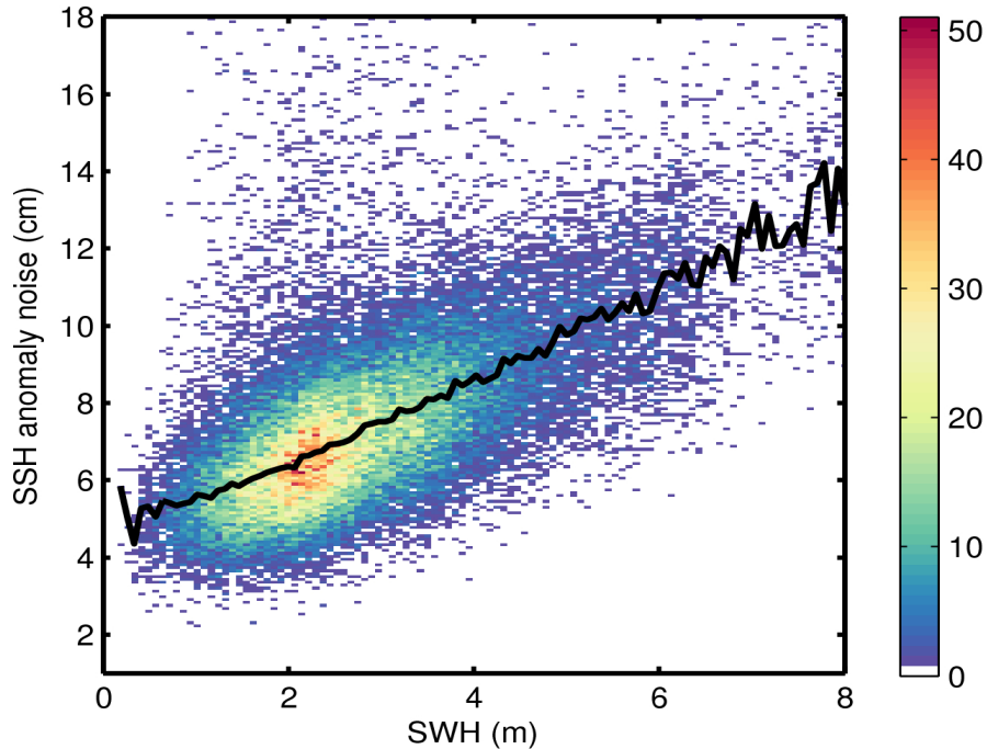
Figure 9. 2D histogram showing flag-valid SSH anomaly noise as a function of SWH for 13/03/2017. The black line denotes the median SSH anomaly noise as a function of SWH.
