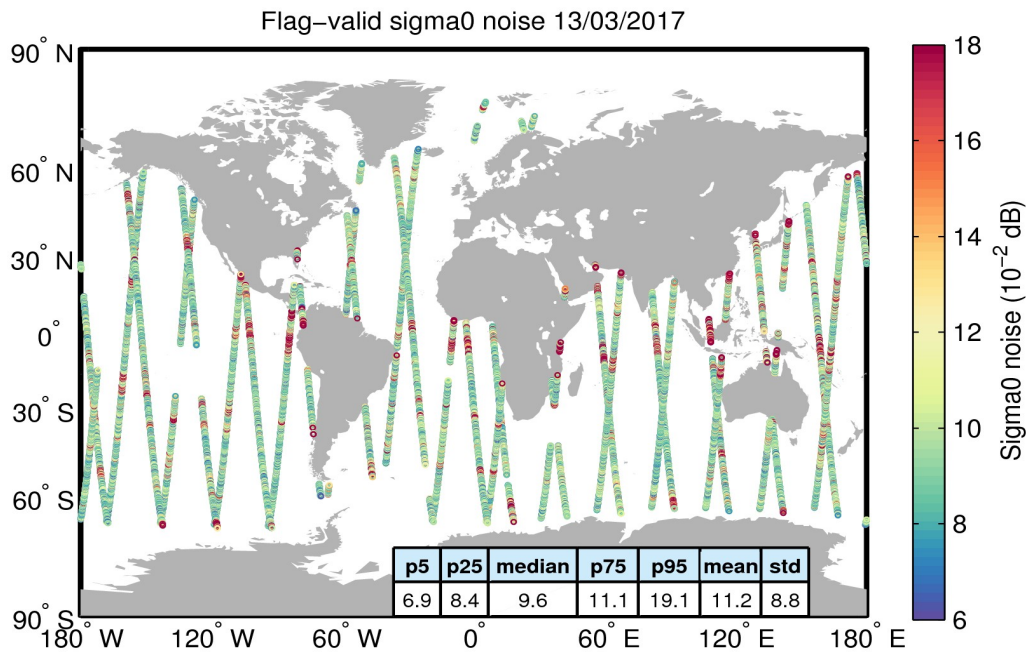
Figure 26. Geographical distribution of flag-valid 20-Hz sigma0 measurement noise over oceans and lakes for 13/03/2017. The statistical values shown in the table refer to the sigma0 noise and are calculated over all measurements shown in the figure.
