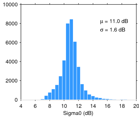
Figure 28. Histogram of science-valid sigma0 over oceans and lakes for 13/03/2017. The mean ( \mu ) and standard deviation ( \sigma ) are also shown. Note that values outside [4 20] dB are excluded from the histogram for the sake of readability but not from the computation of \mu and \sigma .
