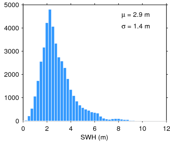
Figure 17. Histogram of flag-valid SWH over oceans and lakes for 13/03/2017. The mean ( \mu ) and standard deviation ( \sigma ) are also shown. Note that values larger than 12 m are excluded from the histogram for the sake of readability but not from the computation of \mu and \sigma .
