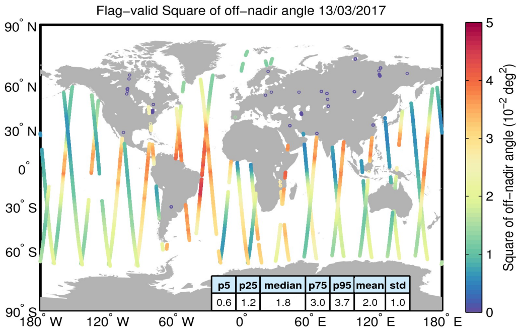
Figure 37. Geographical distribution of flag-valid mispointing data over oceans and lakes for 13/03/2017. The statistical values shown in the table refer to the mispointing in 10^{-2} deg 2 and are calculated over all measurements shown in the figure.
