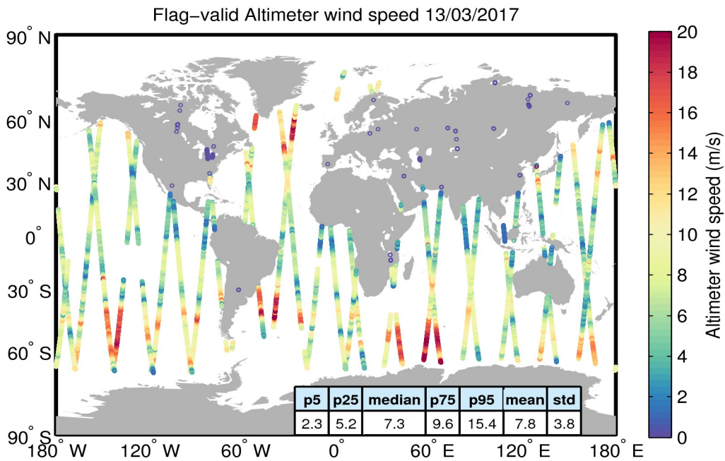
Figure 31. Geographical distribution of flag-valid wind data over oceans and lakes for 13/03/2017. The statistical values shown in the table refer to the wind in m/s and are calculated over all measurements shown in the figure.
