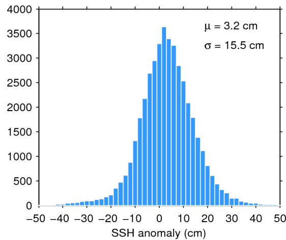
Figure 7. Histogram of flag-valid SSH anomaly over oceans and lakes for 13/03/2017. The mean ( \mu ) and standard deviation ( \sigma ) are also shown. Note that values outside [-50 50] cm are excluded from the histogram for the sake of readability but not from the computation of \mu and \sigma .
