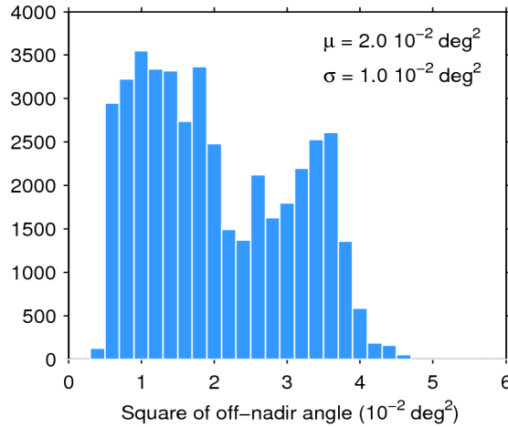
Figure 39. Histogram of flag-valid mispointing over oceans and lakes for 13/03/2017. The mean ( \mu ) and standard deviation ( \sigma ) are also shown. Note that values larger than 6 \cdot 10^{-2} \text{ deg}^2 are excluded from the histogram for the sake of readability but not from the computation of \mu and \sigma .
