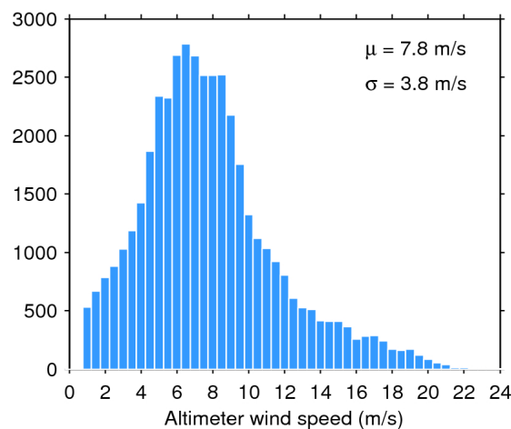
Figure 35. Histogram of science-valid wind over oceans and lakes for 13/03/2017. The mean ( \mu ) and standard deviation ( \sigma ) are also shown. Note that values larger than 24 m/s are excluded from the histogram for the sake of readability but not from the computation of \mu and \sigma .
