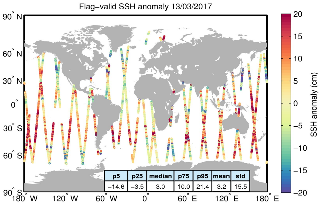
Figure 5. Geographical distribution of flag-valid 1-Hz SSH anomaly data over oceans and lakes for 13/03/2017. The statistical values shown in the table refer to the SSH anomaly in cm and are calculated over all measurements shown in the figure.
