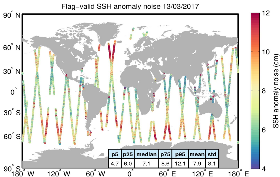
Figure 8. Geographical distribution of flag-valid 20-Hz SSH anomaly measurement noise over oceans and lakes for 13/03/2017. The statistical values shown in the table refer to the SSH anomaly noise and are calculated over all measurements shown in the figure.
