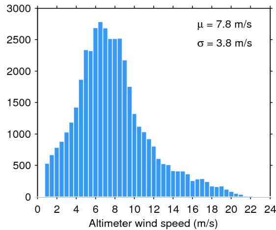
Figure 33. Histogram of flag-valid wind over oceans and lakes for 13/03/2017. The mean ( \mu ) and standard deviation ( \sigma ) are also shown. Note that values larger than 24 m/s are excluded from the histogram for the sake of readability but not from the computation of \mu and \sigma .
