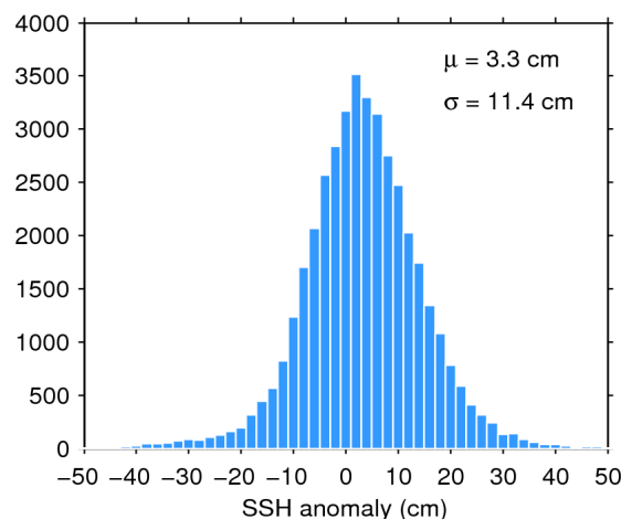
Figure 11. Histogram of science-valid SSH anomaly over oceans and lakes for 13/03/2017. The mean ( \mu ) and standard deviation ( \sigma ) are also shown. Note that values outside [-50 50] cm are excluded from the histogram for the sake of readability but not from the computation of \mu and \sigma .
