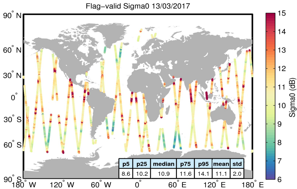
Figure 23. Geographical distribution of flag-valid sigma0 data over oceans and lakes for 13/03/2017. The statistical values shown in the table refer to the sigma0 in dB and are calculated over all measurements shown in the figure.
