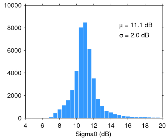
Figure 25. Histogram of flag-valid sigma0 over oceans and lakes for 13/03/2017. The mean ( \mu ) and standard deviation ( \sigma ) are also shown. Note that values outside [4 20] dB are excluded from the histogram for the sake of readability but not from the computation of \mu and \sigma .
