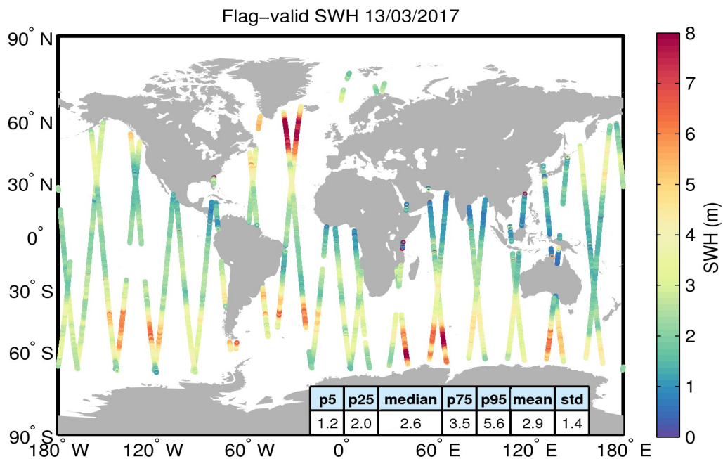
Figure 15. Geographical distribution of flag-valid SWH data over oceans and lakes for 13/03/2017. The statistical values shown in the table refer to the SWH in m and are calculated over all measurements shown in the figure.
