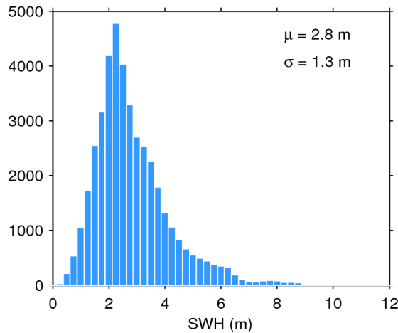
Figure 20. Histogram of science-valid SWH over oceans and lakes for 13/03/2017. The mean ( \mu ) and standard deviation ( \sigma ) are also shown. Note that values larger than 12 m are excluded from the histogram for the sake of readability but not from the computation of \mu and \sigma .
