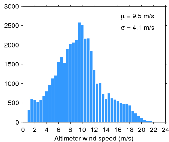
Figure 35. Histogram of science-valid wind over oceans and lakes for 12/03/2017. The mean ( \mu ) and standard deviation ( \sigma ) are also shown. Note that values larger than 24 m/s are excluded from the histogram for the sake of readability but not from the computation of \mu and \sigma .
