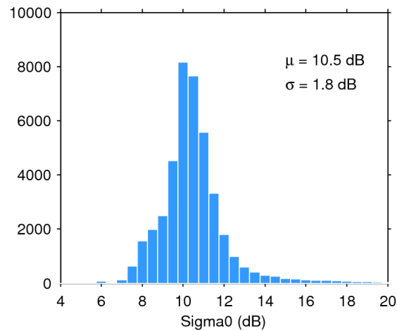
Figure 25. Histogram of flag-valid sigma0 over oceans and lakes for 12/03/2017. The mean ( \mu ) and standard deviation ( \sigma ) are also shown. Note that values outside [4 20] dB are excluded from the histogram for the sake of readability but not from the computation of \mu and \sigma .
