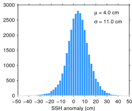
Figure 11. Histogram of science-valid SSH anomaly over oceans and lakes for 12/03/2017. The mean ( \mu ) and standard deviation ( \sigma ) are also shown. Note that values outside [-50 50] cm are excluded from the histogram for the sake of readability but not from the computation of \mu and \sigma .
