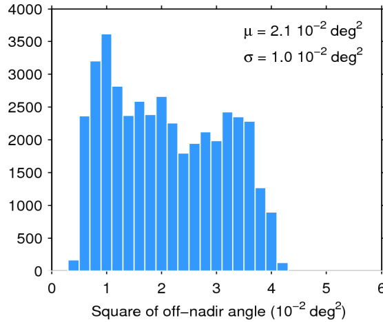
Figure 39. Histogram of flag-valid mispointing over oceans and lakes for 12/03/2017. The mean ( \mu ) and standard deviation ( \sigma ) are also shown. Note that values larger than 6 \cdot 10^{-2} \text{ deg}^2 are excluded from the histogram for the sake of readability but not from the computation of \mu and \sigma .
