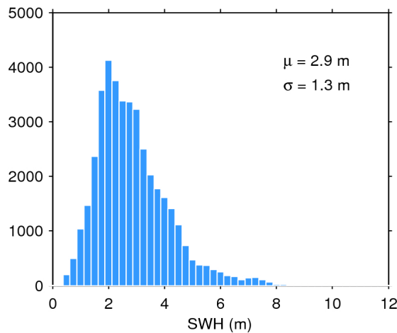
Figure 20. Histogram of science-valid SWH over oceans and lakes for 12/03/2017. The mean ( \mu ) and standard deviation ( \sigma ) are also shown. Note that values larger than 12 m are excluded from the histogram for the sake of readability but not from the computation of \mu and \sigma .
