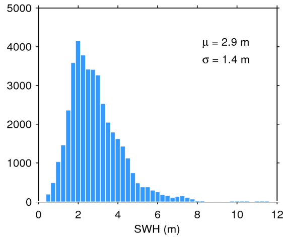
Figure 17. Histogram of flag-valid SWH over oceans and lakes for 12/03/2017. The mean ( \mu ) and standard deviation ( \sigma ) are also shown. Note that values larger than 12 m are excluded from the histogram for the sake of readability but not from the computation of \mu and \sigma .
