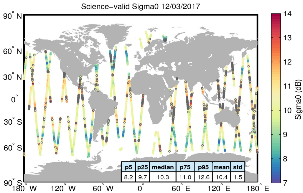
Figure 27. Geographical distribution of science-valid sigma0 data over oceans and lakes for 12/03/2017. The statistical values shown in the table refer to the sigma0 in dB and are calculated over all measurements shown in the figure. Gray circles denote records that have been rejected based on the editing criteria described in Table 4.
