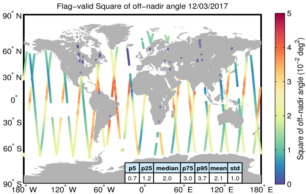
Figure 37. Geographical distribution of flag-valid mispointing data over oceans and lakes for 12/03/2017. The statistical values shown in the table refer to the mispointing in 10^{-2} deg 2 and are calculated over all measurements shown in the figure.
