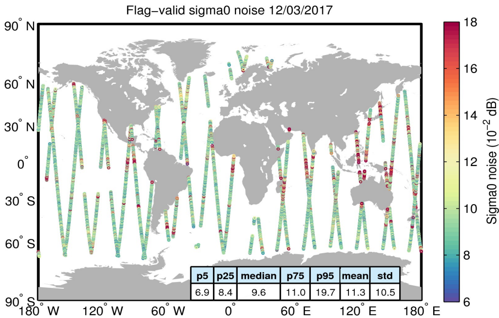
Figure 26. Geographical distribution of flag-valid 20-Hz sigma0 measurement noise over oceans and lakes for 12/03/2017. The statistical values shown in the table refer to the sigma0 noise and are calculated over all measurements shown in the figure.
