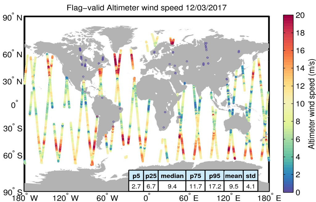
Figure 31. Geographical distribution of flag-valid wind data over oceans and lakes for 12/03/2017. The statistical values shown in the table refer to the wind in m/s and are calculated over all measurements shown in the figure.
