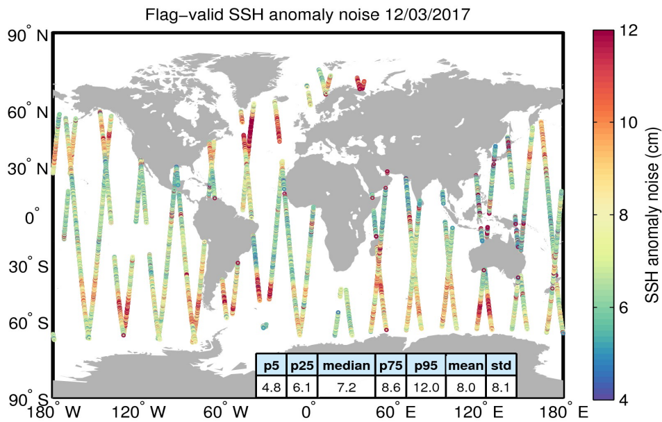
Figure 8. Geographical distribution of flag-valid 20-Hz SSH anomaly measurement noise over oceans and lakes for 12/03/2017. The statistical values shown in the table refer to the SSH anomaly noise and are calculated over all measurements shown in the figure.
