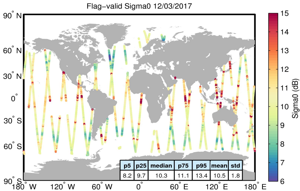
Figure 23. Geographical distribution of flag-valid sigma0 data over oceans and lakes for 12/03/2017. The statistical values shown in the table refer to the sigma0 in dB and are calculated over all measurements shown in the figure.
