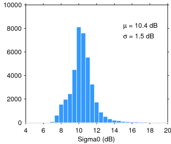
Figure 28. Histogram of science-valid sigma0 over oceans and lakes for 12/03/2017. The mean ( \mu ) and standard deviation ( \sigma ) are also shown. Note that values outside [4 20] dB are excluded from the histogram for the sake of readability but not from the computation of \mu and \sigma .
