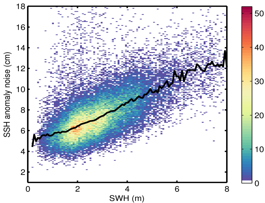
Figure 9. 2D histogram showing flag-valid SSH anomaly noise as a function of SWH for 12/03/2017. The black line denotes the median SSH anomaly noise as a function of SWH.
