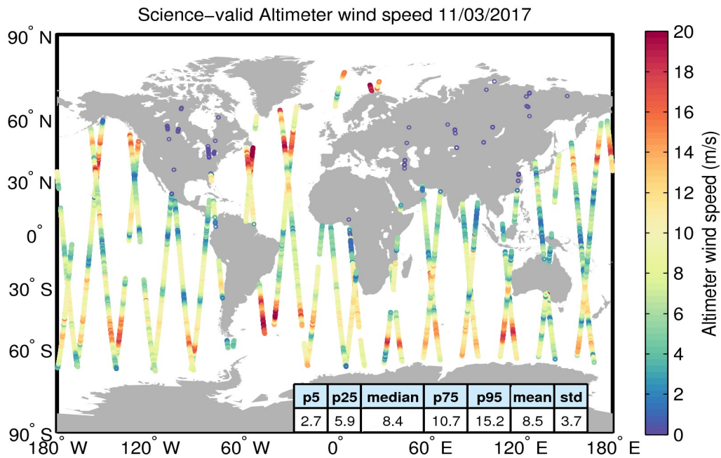
Figure 34. Geographical distribution of science-valid wind data over oceans and lakes for 11/03/2017. The statistical values shown in the table refer to the wind in m/s and are calculated over all measurements shown in the figure. Gray circles denote records that have been rejected based on the editing criteria described in Table 5.
