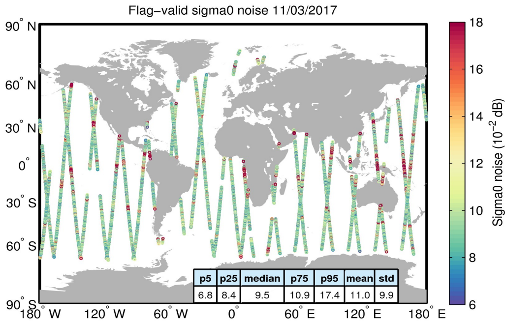
Figure 26. Geographical distribution of flag-valid 20-Hz sigma0 measurement noise over oceans and lakes for 11/03/2017. The statistical values shown in the table refer to the sigma0 noise and are calculated over all measurements shown in the figure.
