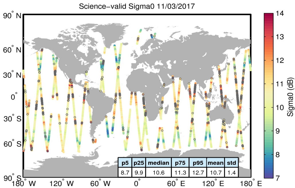
Figure 27. Geographical distribution of science-valid sigma0 data over oceans and lakes for 11/03/2017. The statistical values shown in the table refer to the sigma0 in dB and are calculated over all measurements shown in the figure. Gray circles denote records that have been rejected based on the editing criteria described in Table 4.
