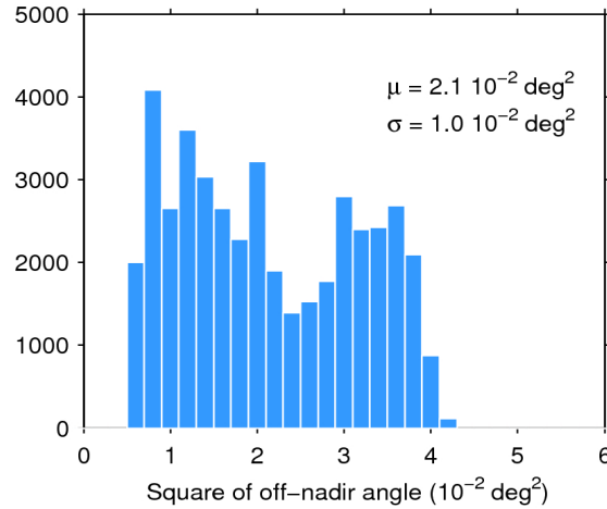
Figure 39. Histogram of flag-valid mispointing over oceans and lakes for 11/03/2017. The mean ( \mu ) and standard deviation ( \sigma ) are also shown. Note that values larger than 6 \cdot 10^{-2} \text{ deg}^2 are excluded from the histogram for the sake of readability but not from the computation of \mu and \sigma .
