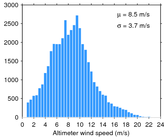
Figure 33. Histogram of flag-valid wind over oceans and lakes for 11/03/2017. The mean ( \mu ) and standard deviation ( \sigma ) are also shown. Note that values larger than 24 m/s are excluded from the histogram for the sake of readability but not from the computation of \mu and \sigma .
