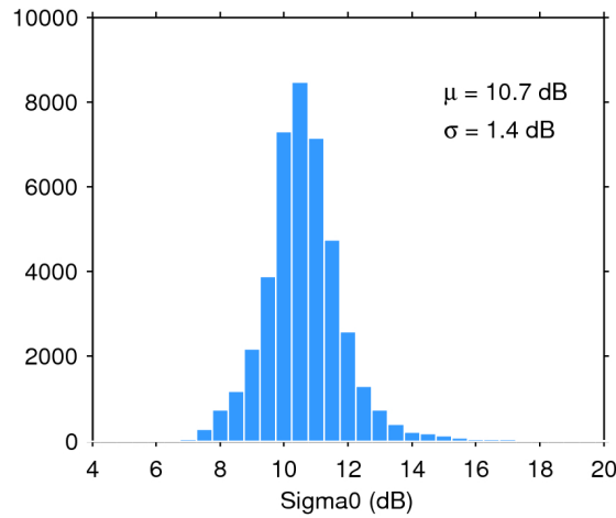
Figure 28. Histogram of science-valid sigma0 over oceans and lakes for 11/03/2017. The mean ( \mu ) and standard deviation ( \sigma ) are also shown. Note that values outside [4 20] dB are excluded from the histogram for the sake of readability but not from the computation of \mu and \sigma .
