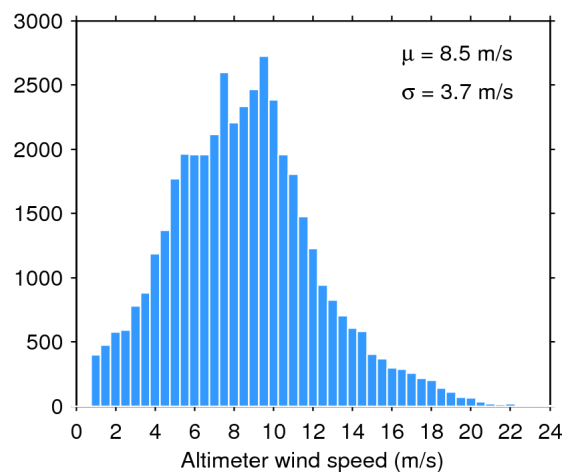
Figure 35. Histogram of science-valid wind over oceans and lakes for 11/03/2017. The mean ( \mu ) and standard deviation ( \sigma ) are also shown. Note that values larger than 24 m/s are excluded from the histogram for the sake of readability but not from the computation of \mu and \sigma .
