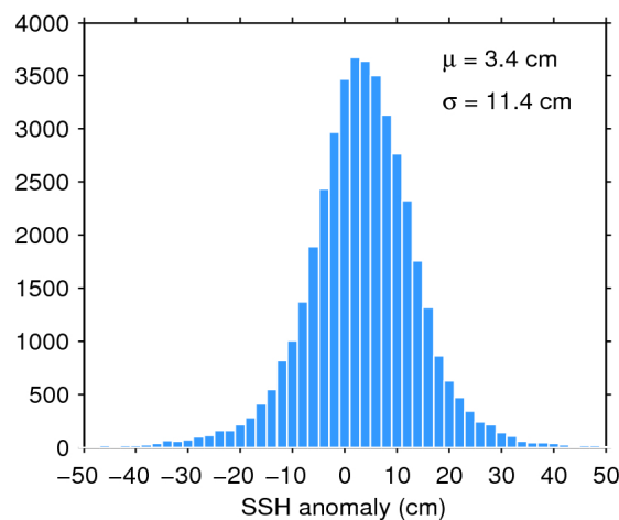
Figure 11. Histogram of science-valid SSH anomaly over oceans and lakes for 11/03/2017. The mean ( \mu ) and standard deviation ( \sigma ) are also shown. Note that values outside [-50 50] cm are excluded from the histogram for the sake of readability but not from the computation of \mu and \sigma .
