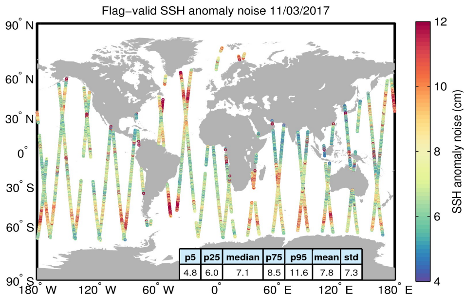
Figure 8. Geographical distribution of flag-valid 20-Hz SSH anomaly measurement noise over oceans and lakes for 11/03/2017. The statistical values shown in the table refer to the SSH anomaly noise and are calculated over all measurements shown in the figure.
