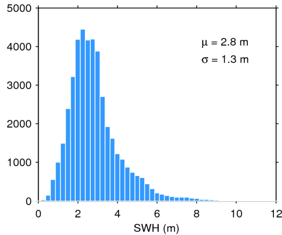
Figure 17. Histogram of flag-valid SWH over oceans and lakes for 11/03/2017. The mean ( \mu ) and standard deviation ( \sigma ) are also shown. Note that values larger than 12 m are excluded from the histogram for the sake of readability but not from the computation of \mu and \sigma .
