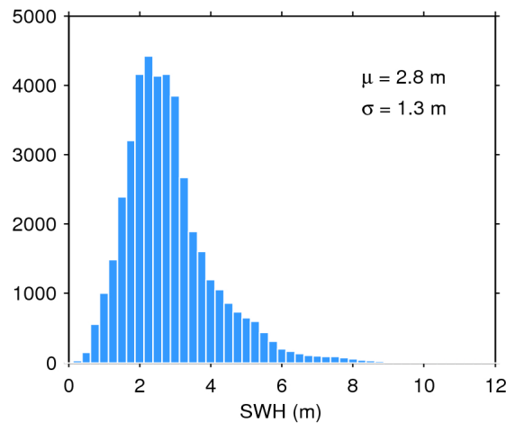
Figure 20. Histogram of science-valid SWH over oceans and lakes for 11/03/2017. The mean ( \mu ) and standard deviation ( \sigma ) are also shown. Note that values larger than 12 m are excluded from the histogram for the sake of readability but not from the computation of \mu and \sigma .
