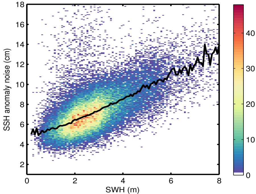
Figure 9. 2D histogram showing flag-valid SSH anomaly noise as a function of SWH for 11/03/2017. The black line denotes the median SSH anomaly noise as a function of SWH.
