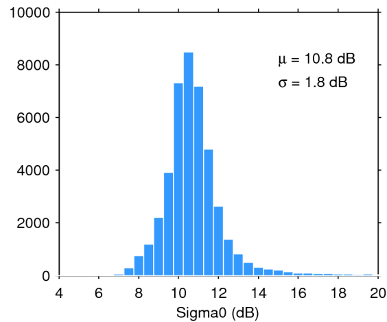
Figure 25. Histogram of flag-valid sigma0 over oceans and lakes for 11/03/2017. The mean ( \mu ) and standard deviation ( \sigma ) are also shown. Note that values outside [4 20] dB are excluded from the histogram for the sake of readability but not from the computation of \mu and \sigma .
