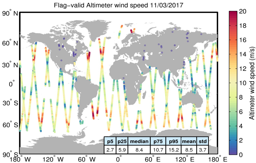
Figure 31. Geographical distribution of flag-valid wind data over oceans and lakes for 11/03/2017. The statistical values shown in the table refer to the wind in m/s and are calculated over all measurements shown in the figure.
