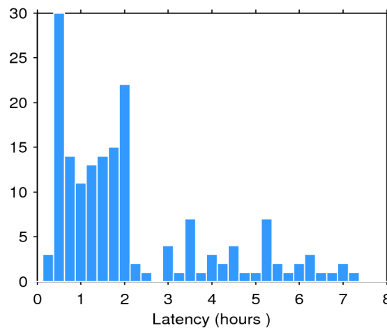
Figure 2. Histogram of the data latency for 10/03/2017. The y-axis denotes the number of files that are made available with a delay of x-hours with respect to the mean time of the records stored in the file.
