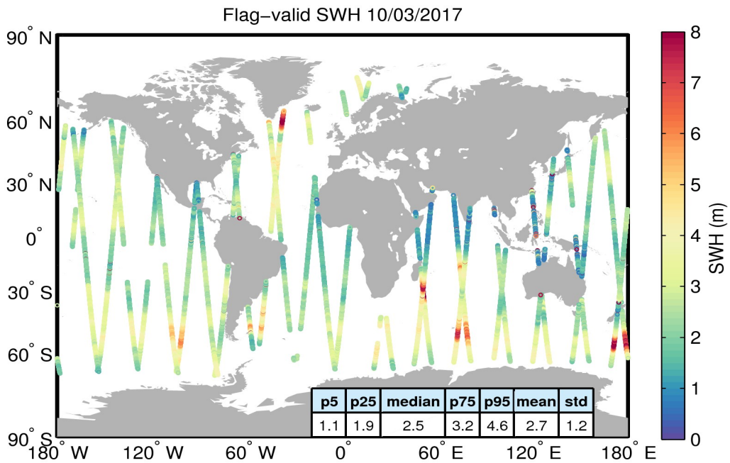
Figure 15. Geographical distribution of flag-valid SWH data over oceans and lakes for 10/03/2017. The statistical values shown in the table refer to the SWH in m and are calculated over all measurements shown in the figure.
