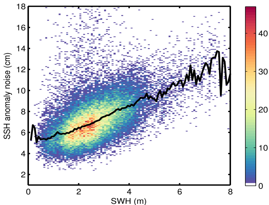
Figure 9. 2D histogram showing flag-valid SSH anomaly noise as a function of SWH for 10/03/2017. The black line denotes the median SSH anomaly noise as a function of SWH.
