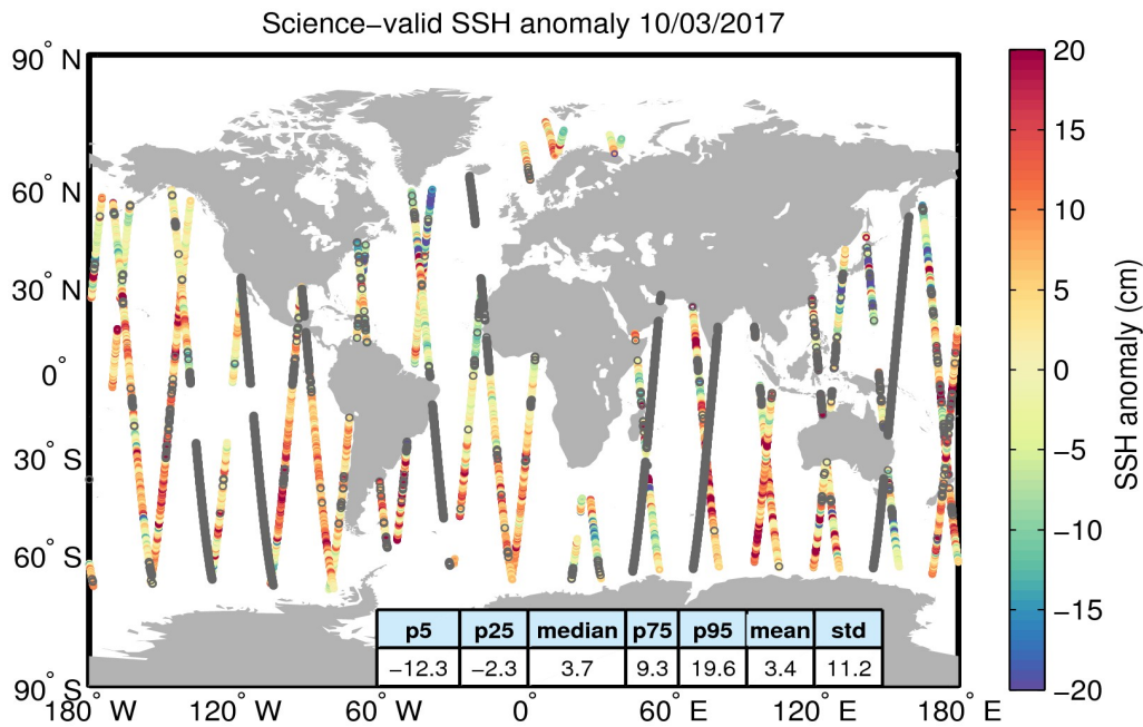
Figure 10. Geographical distribution of science-valid SSH anomaly data over oceans and lakes for 10/03/2017. The statistical values shown in the table refer to the SSH anomaly in cm and are calculated over all measurements shown in the figure. Gray circles denote records that have been rejected based on the editing criteria described in Table 2.
