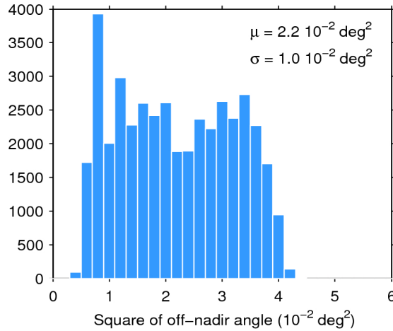
Figure 39. Histogram of flag-valid mispointing over oceans and lakes for 10/03/2017. The mean ( \mu ) and standard deviation ( \sigma ) are also shown. Note that values larger than 6 \cdot 10^{-2} \text{ deg}^2 are excluded from the histogram for the sake of readability but not from the computation of \mu and \sigma .
