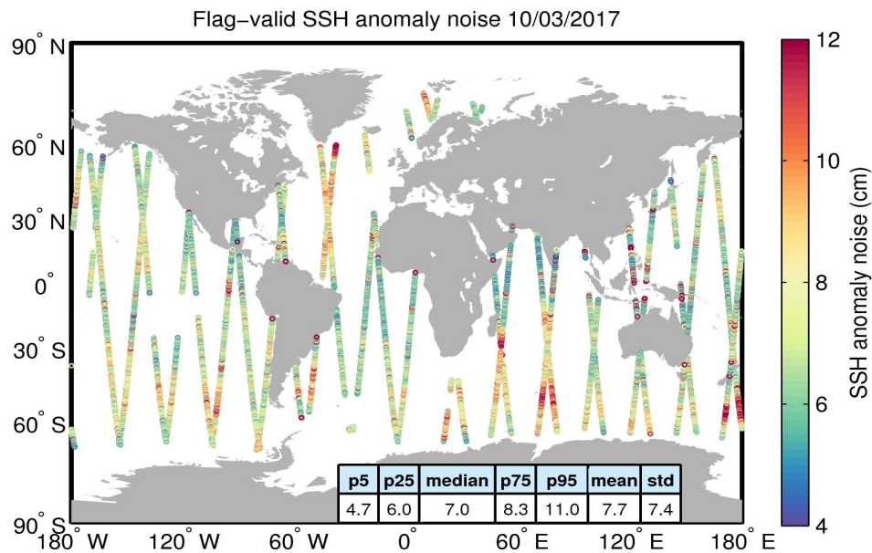
Figure 8. Geographical distribution of flag-valid 20-Hz SSH anomaly measurement noise over oceans and lakes for 10/03/2017. The statistical values shown in the table refer to the SSH anomaly noise and are calculated over all measurements shown in the figure.
