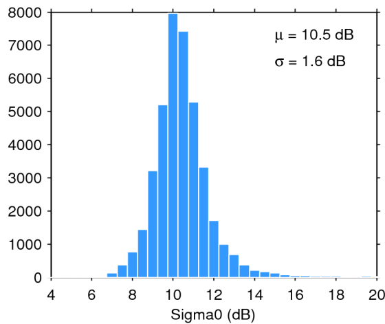
Figure 28. Histogram of science-valid sigma0 over oceans and lakes for 10/03/2017. The mean ( \mu ) and standard deviation ( \sigma ) are also shown. Note that values outside [4 20] dB are excluded from the histogram for the sake of readability but not from the computation of \mu and \sigma .
