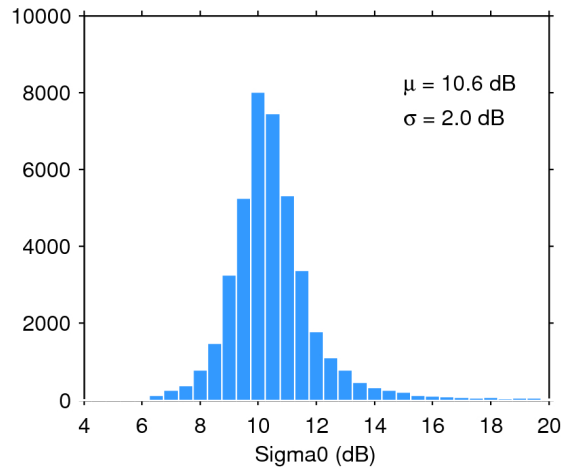
Figure 25. Histogram of flag-valid sigma0 over oceans and lakes for 10/03/2017. The mean ( \mu ) and standard deviation ( \sigma ) are also shown. Note that values outside [4 20] dB are excluded from the histogram for the sake of readability but not from the computation of \mu and \sigma .
