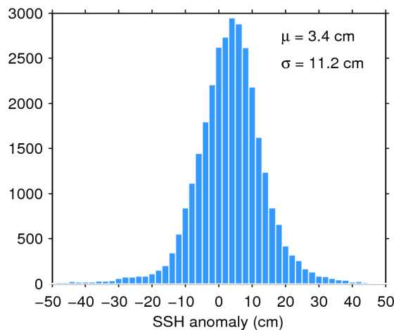
Figure 11. Histogram of science-valid SSH anomaly over oceans and lakes for 10/03/2017. The mean ( \mu ) and standard deviation ( \sigma ) are also shown. Note that values outside [-50 50] cm are excluded from the histogram for the sake of readability but not from the computation of \mu and \sigma .
