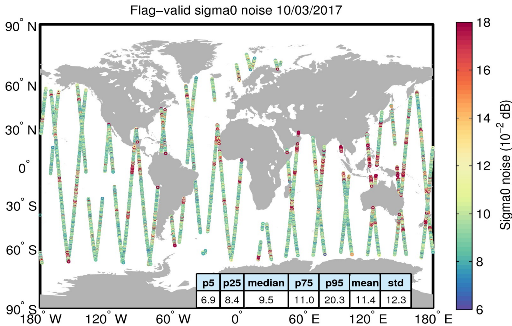
Figure 26. Geographical distribution of flag-valid 20-Hz sigma0 measurement noise over oceans and lakes for 10/03/2017. The statistical values shown in the table refer to the sigma0 noise and are calculated over all measurements shown in the figure.
