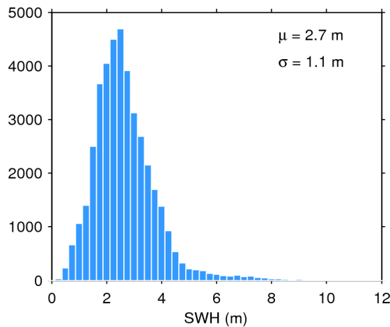
Figure 20. Histogram of science-valid SWH over oceans and lakes for 10/03/2017. The mean ( \mu ) and standard deviation ( \sigma ) are also shown. Note that values larger than 12 m are excluded from the histogram for the sake of readability but not from the computation of \mu and \sigma .
