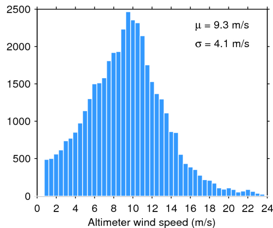
Figure 35. Histogram of science-valid wind over oceans and lakes for 10/03/2017. The mean ( \mu ) and standard deviation ( \sigma ) are also shown. Note that values larger than 24 m/s are excluded from the histogram for the sake of readability but not from the computation of \mu and \sigma .
