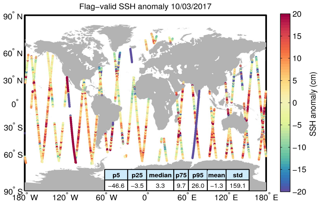
Figure 5. Geographical distribution of flag-valid 1-Hz SSH anomaly data over oceans and lakes for 10/03/2017. The statistical values shown in the table refer to the SSH anomaly in cm and are calculated over all measurements shown in the figure.
