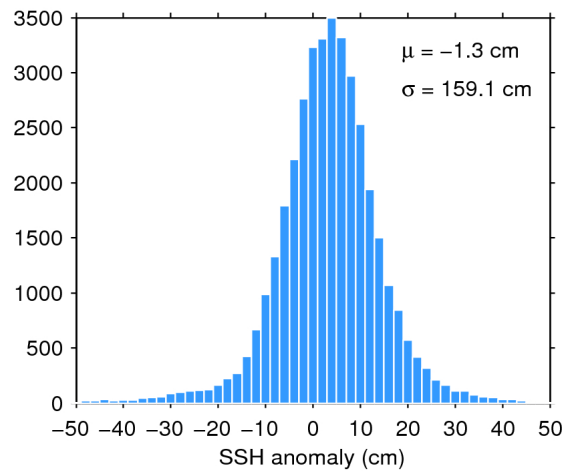
Figure 7. Histogram of flag-valid SSH anomaly over oceans and lakes for 10/03/2017. The mean ( \mu ) and standard deviation ( \sigma ) are also shown. Note that values outside [-50 50] cm are excluded from the histogram for the sake of readability but not from the computation of \mu and \sigma .
