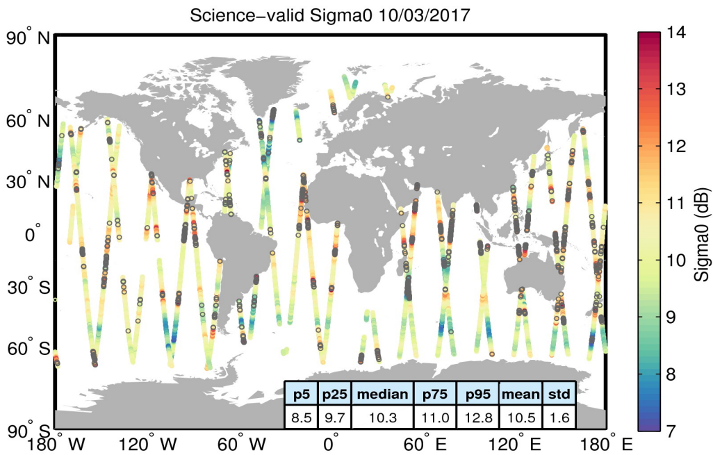
Figure 27. Geographical distribution of science-valid sigma0 data over oceans and lakes for 10/03/2017. The statistical values shown in the table refer to the sigma0 in dB and are calculated over all measurements shown in the figure. Gray circles denote records that have been rejected based on the editing criteria described in Table 4.
