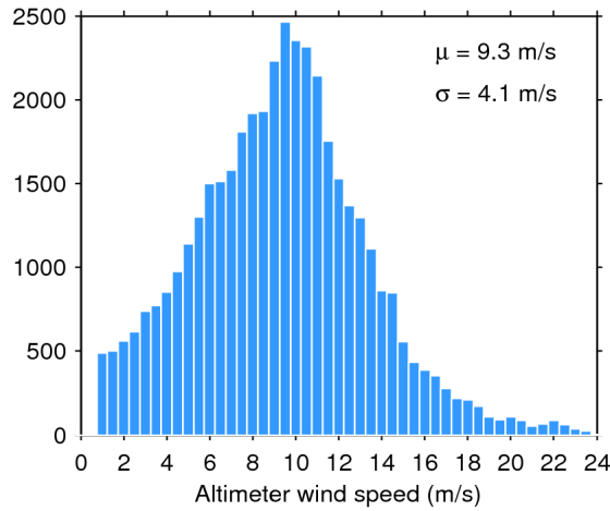
Figure 33. Histogram of flag-valid wind over oceans and lakes for 10/03/2017. The mean ( \mu ) and standard deviation ( \sigma ) are also shown. Note that values larger than 24 m/s are excluded from the histogram for the sake of readability but not from the computation of \mu and \sigma .
