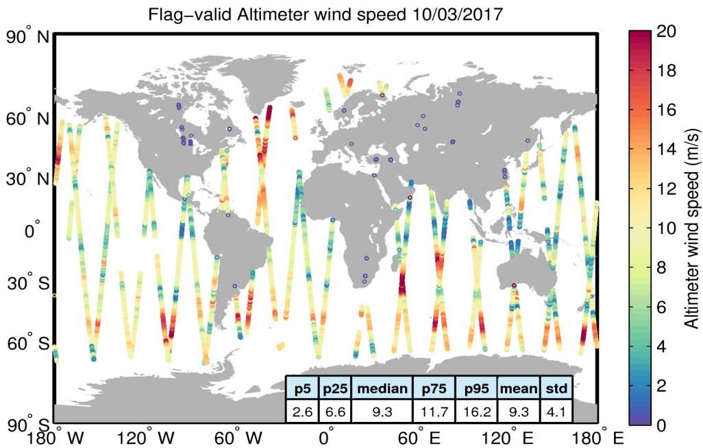
Figure 31. Geographical distribution of flag-valid wind data over oceans and lakes for 10/03/2017. The statistical values shown in the table refer to the wind in m/s and are calculated over all measurements shown in the figure.
