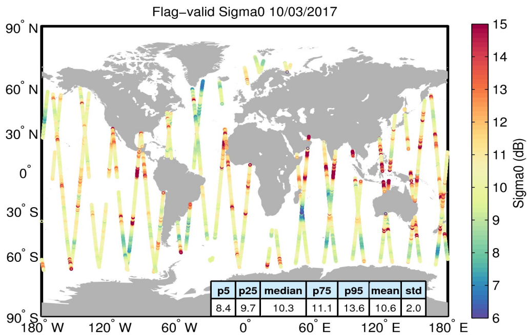
Figure 23. Geographical distribution of flag-valid sigma0 data over oceans and lakes for 10/03/2017. The statistical values shown in the table refer to the sigma0 in dB and are calculated over all measurements shown in the figure.
