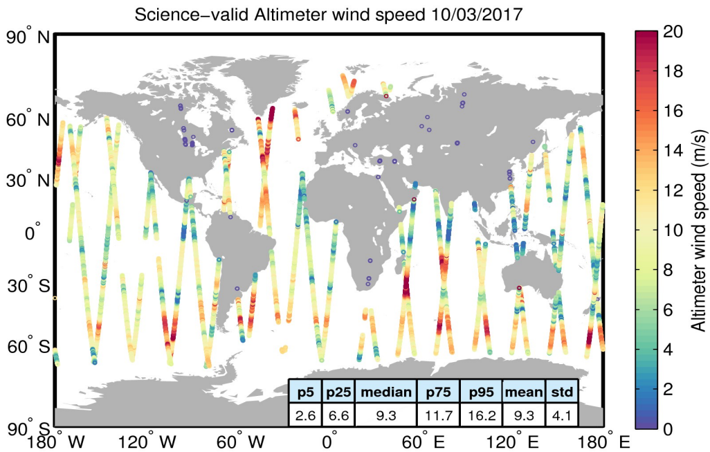
Figure 34. Geographical distribution of science-valid wind data over oceans and lakes for 10/03/2017. The statistical values shown in the table refer to the wind in m/s and are calculated over all measurements shown in the figure. Gray circles denote records that have been rejected based on the editing criteria described in Table 5.
