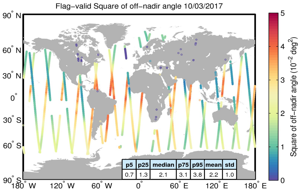
Figure 37. Geographical distribution of flag-valid mispointing data over oceans and lakes for 10/03/2017. The statistical values shown in the table refer to the mispointing in 10^{-2} deg 2 and are calculated over all measurements shown in the figure.
