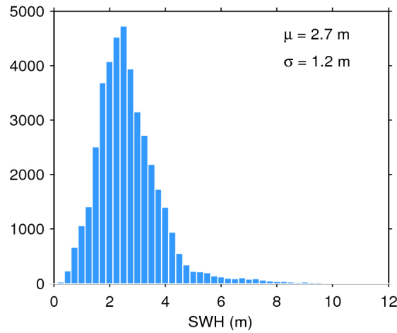
Figure 17. Histogram of flag-valid SWH over oceans and lakes for 10/03/2017. The mean ( \mu ) and standard deviation ( \sigma ) are also shown. Note that values larger than 12 m are excluded from the histogram for the sake of readability but not from the computation of \mu and \sigma .
