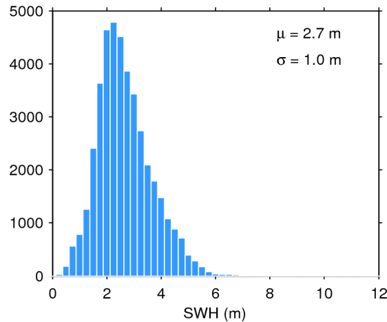
Figure 20. Histogram of science-valid SWH over oceans and lakes for 09/03/2017. The mean ( \mu ) and standard deviation ( \sigma ) are also shown. Note that values larger than 12 m are excluded from the histogram for the sake of readability but not from the computation of \mu and \sigma .
