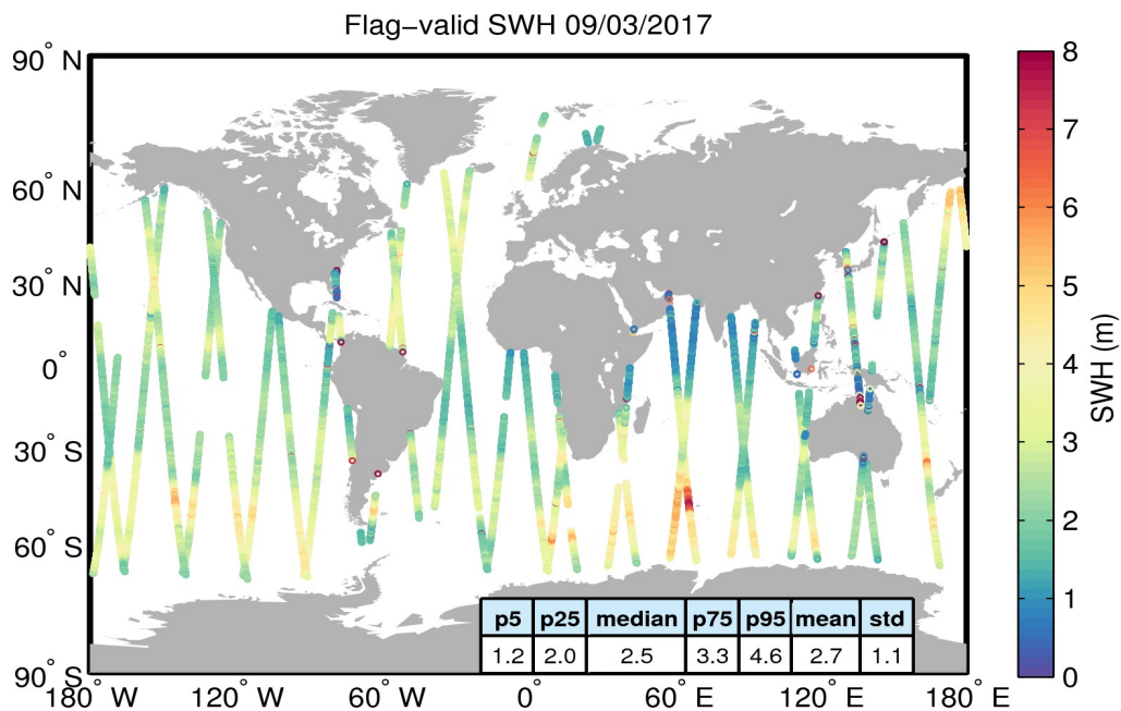
Figure 15. Geographical distribution of flag-valid SWH data over oceans and lakes for 09/03/2017. The statistical values shown in the table refer to the SWH in m and are calculated over all measurements shown in the figure.
