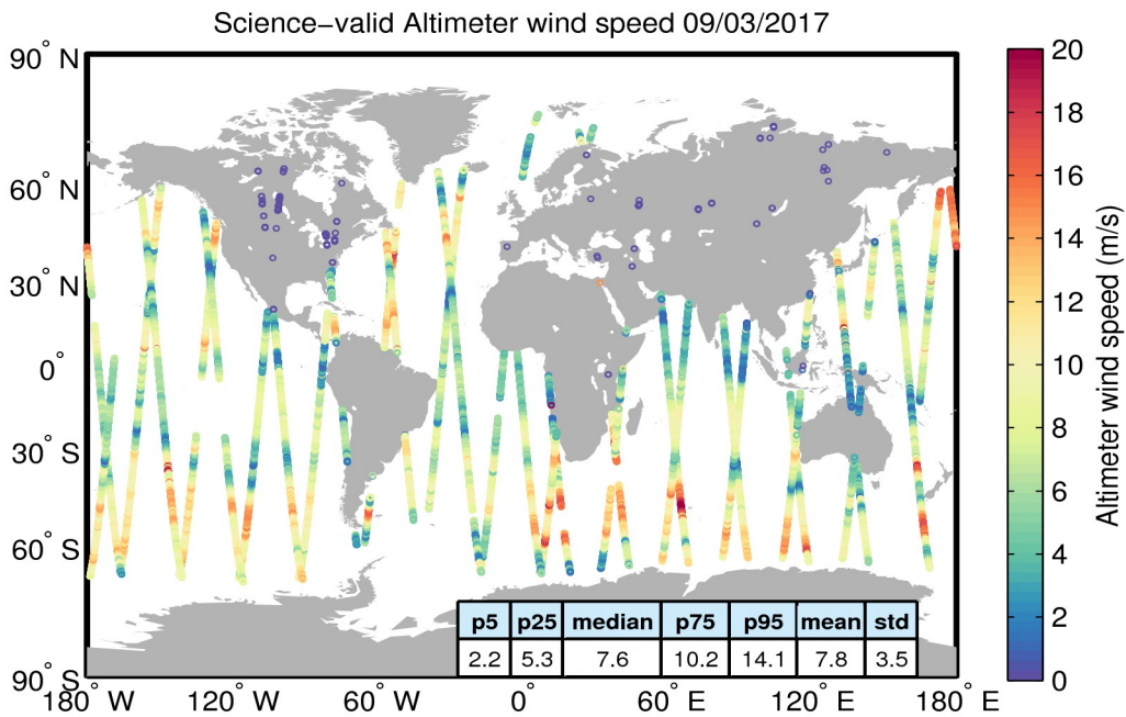
Figure 34. Geographical distribution of science-valid wind data over oceans and lakes for 09/03/2017. The statistical values shown in the table refer to the wind in m/s and are calculated over all measurements shown in the figure. Gray circles denote records that have been rejected based on the editing criteria described in Table 5.
