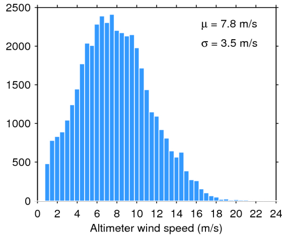
Figure 33. Histogram of flag-valid wind over oceans and lakes for 09/03/2017. The mean ( \mu ) and standard deviation ( \sigma ) are also shown. Note that values larger than 24 m/s are excluded from the histogram for the sake of readability but not from the computation of \mu and \sigma .
