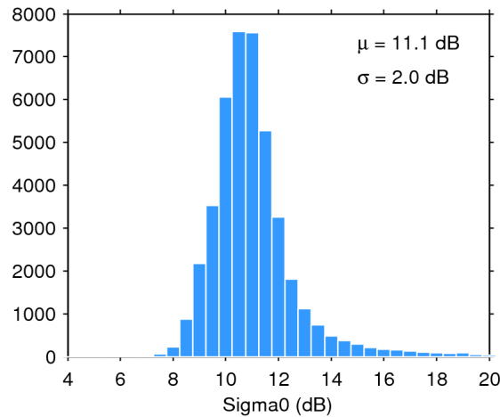
Figure 25. Histogram of flag-valid sigma0 over oceans and lakes for 09/03/2017. The mean ( \mu ) and standard deviation ( \sigma ) are also shown. Note that values outside [4 20] dB are excluded from the histogram for the sake of readability but not from the computation of \mu and \sigma .
