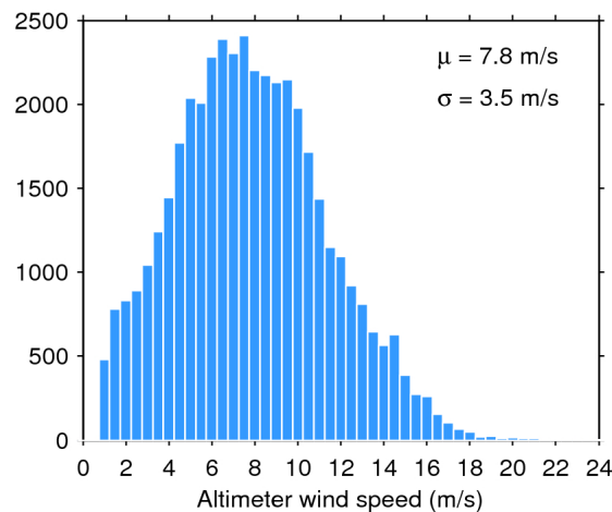
Figure 35. Histogram of science-valid wind over oceans and lakes for 09/03/2017. The mean ( \mu ) and standard deviation ( \sigma ) are also shown. Note that values larger than 24 m/s are excluded from the histogram for the sake of readability but not from the computation of \mu and \sigma .
