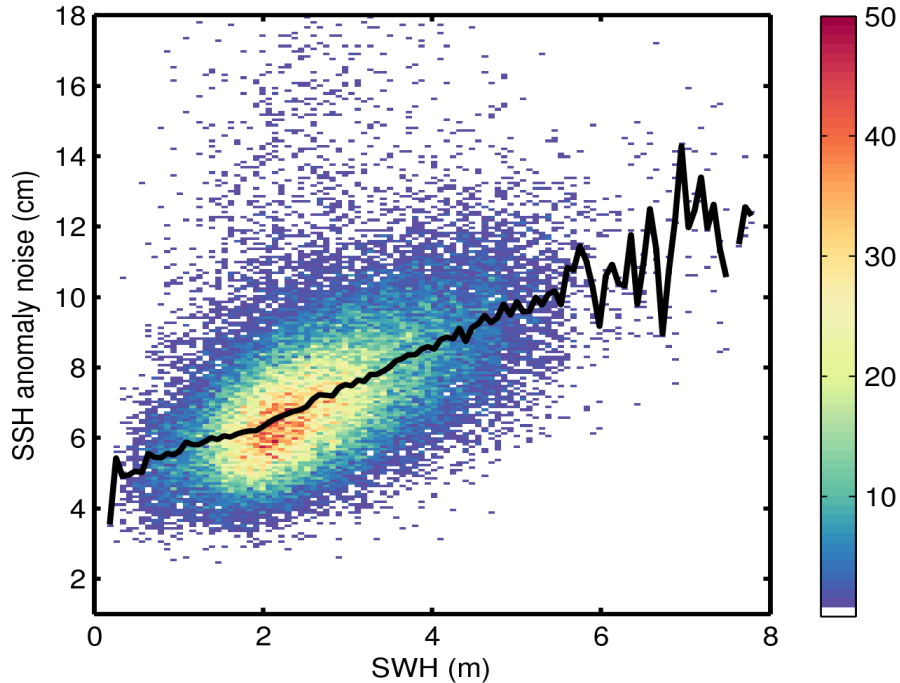
Figure 9. 2D histogram showing flag-valid SSH anomaly noise as a function of SWH for 09/03/2017. The black line denotes the median SSH anomaly noise as a function of SWH.
