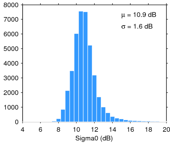
Figure 28. Histogram of science-valid sigma0 over oceans and lakes for 09/03/2017. The mean ( \mu ) and standard deviation ( \sigma ) are also shown. Note that values outside [4 20] dB are excluded from the histogram for the sake of readability but not from the computation of \mu and \sigma .
