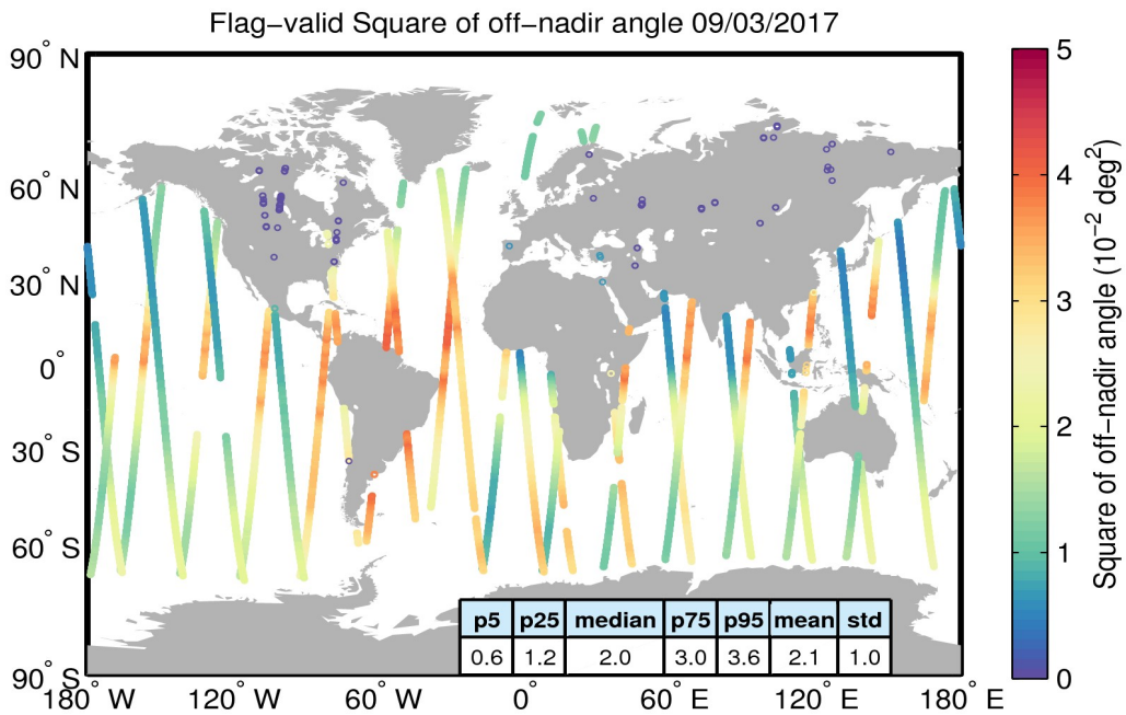
Figure 37. Geographical distribution of flag-valid mispointing data over oceans and lakes for 09/03/2017. The statistical values shown in the table refer to the mispointing in 10^{-2} deg 2 and are calculated over all measurements shown in the figure.
