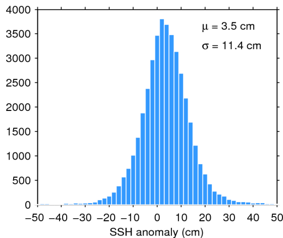
Figure 11. Histogram of science-valid SSH anomaly over oceans and lakes for 09/03/2017. The mean ( \mu ) and standard deviation ( \sigma ) are also shown. Note that values outside [-50 50] cm are excluded from the histogram for the sake of readability but not from the computation of \mu and \sigma .
