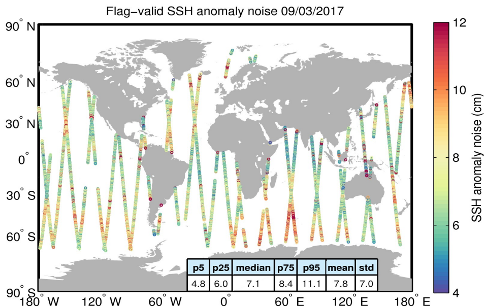
Figure 8. Geographical distribution of flag-valid 20-Hz SSH anomaly measurement noise over oceans and lakes for 09/03/2017. The statistical values shown in the table refer to the SSH anomaly noise and are calculated over all measurements shown in the figure.
