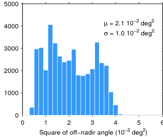
Figure 39. Histogram of flag-valid mispointing over oceans and lakes for 09/03/2017. The mean ( \mu ) and standard deviation ( \sigma ) are also shown. Note that values larger than 6 \cdot 10^{-2} \text{ deg}^2 are excluded from the histogram for the sake of readability but not from the computation of \mu and \sigma .
