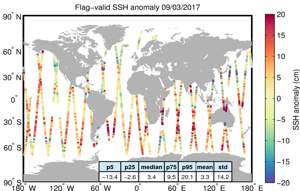
Figure 5. Geographical distribution of flag-valid 1-Hz SSH anomaly data over oceans and lakes for 09/03/2017. The statistical values shown in the table refer to the SSH anomaly in cm and are calculated over all measurements shown in the figure.
