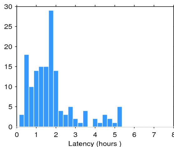
Figure 2. Histogram of the data latency for 09/03/2017. The y-axis denotes the number of files that are made available with a delay of x-hours with respect to the mean time of the records stored in the file.
