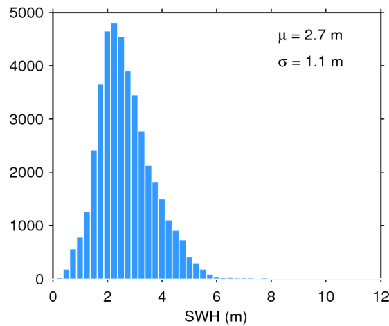
Figure 17. Histogram of flag-valid SWH over oceans and lakes for 09/03/2017. The mean ( \mu ) and standard deviation ( \sigma ) are also shown. Note that values larger than 12 m are excluded from the histogram for the sake of readability but not from the computation of \mu and \sigma .
