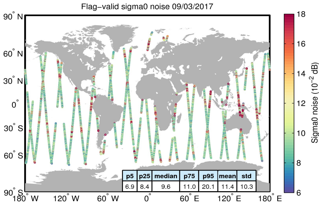
Figure 26. Geographical distribution of flag-valid 20-Hz sigma0 measurement noise over oceans and lakes for 09/03/2017. The statistical values shown in the table refer to the sigma0 noise and are calculated over all measurements shown in the figure.
