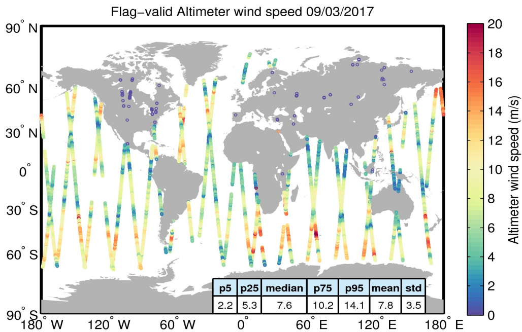
Figure 31. Geographical distribution of flag-valid wind data over oceans and lakes for 09/03/2017. The statistical values shown in the table refer to the wind in m/s and are calculated over all measurements shown in the figure.
