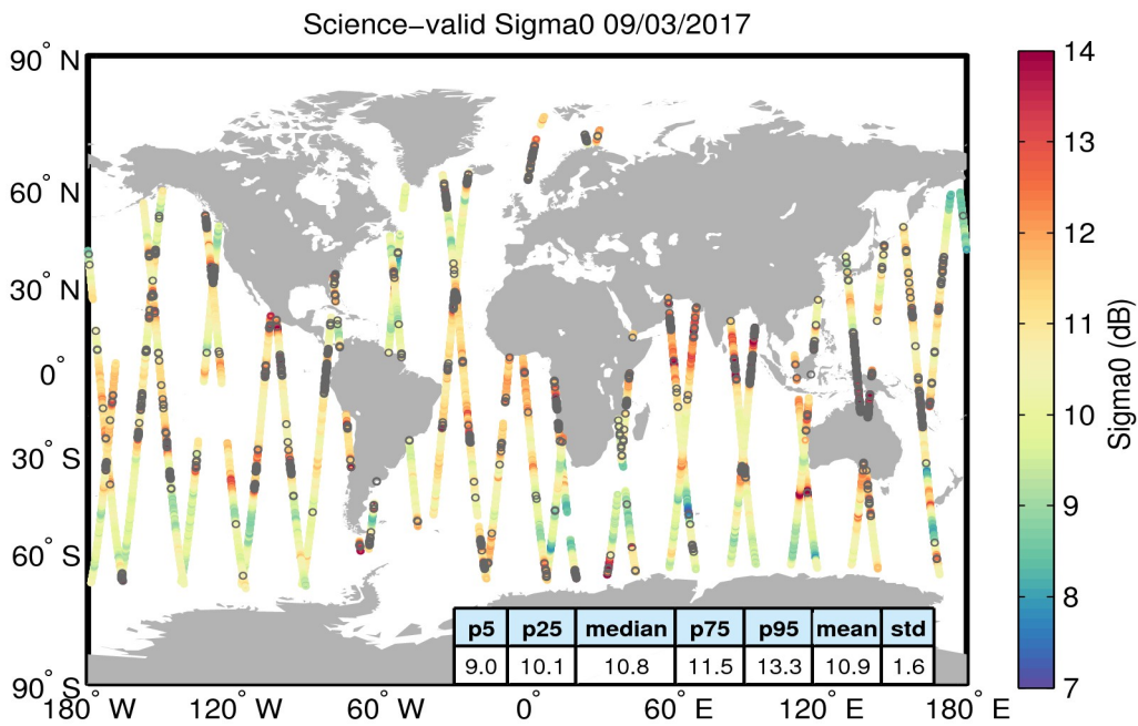
Figure 27. Geographical distribution of science-valid sigma0 data over oceans and lakes for 09/03/2017. The statistical values shown in the table refer to the sigma0 in dB and are calculated over all measurements shown in the figure. Gray circles denote records that have been rejected based on the editing criteria described in Table 4.
