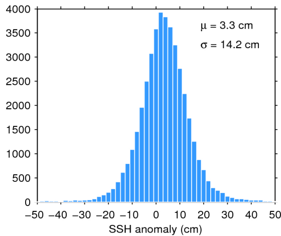
Figure 7. Histogram of flag-valid SSH anomaly over oceans and lakes for 09/03/2017. The mean ( \mu ) and standard deviation ( \sigma ) are also shown. Note that values outside [-50 50] cm are excluded from the histogram for the sake of readability but not from the computation of \mu and \sigma .
