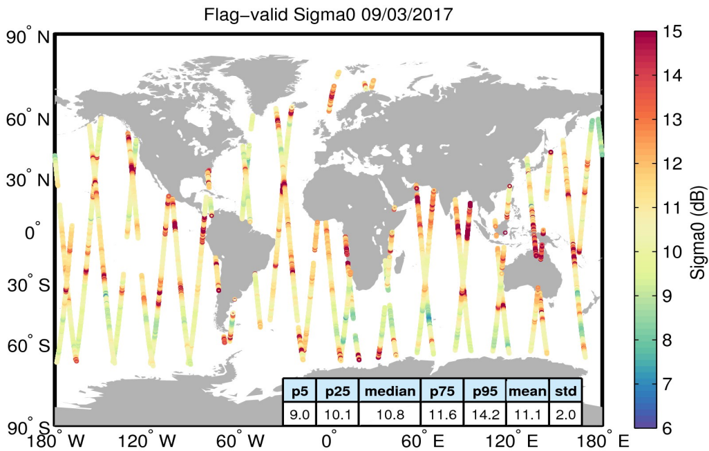
Figure 23. Geographical distribution of flag-valid sigma0 data over oceans and lakes for 09/03/2017. The statistical values shown in the table refer to the sigma0 in dB and are calculated over all measurements shown in the figure.
