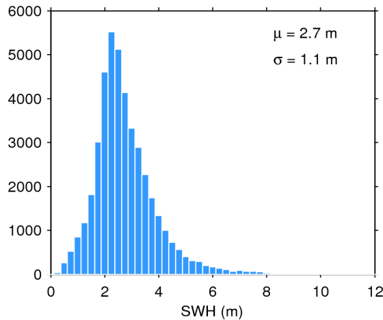
Figure 20. Histogram of science-valid SWH over oceans and lakes for 07/03/2017. The mean ( \mu ) and standard deviation ( \sigma ) are also shown. Note that values larger than 12 m are excluded from the histogram for the sake of readability but not from the computation of \mu and \sigma .
