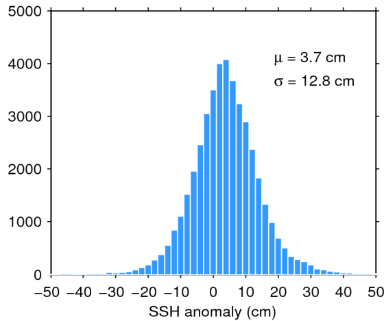
Figure 7. Histogram of flag-valid SSH anomaly over oceans and lakes for 07/03/2017. The mean ( \mu ) and standard deviation ( \sigma ) are also shown. Note that values outside [-50 50] cm are excluded from the histogram for the sake of readability but not from the computation of \mu and \sigma .
