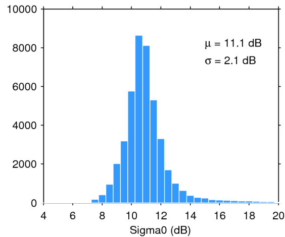
Figure 25. Histogram of flag-valid sigma0 over oceans and lakes for 07/03/2017. The mean ( \mu ) and standard deviation ( \sigma ) are also shown. Note that values outside [4 20] dB are excluded from the histogram for the sake of readability but not from the computation of \mu and \sigma .
