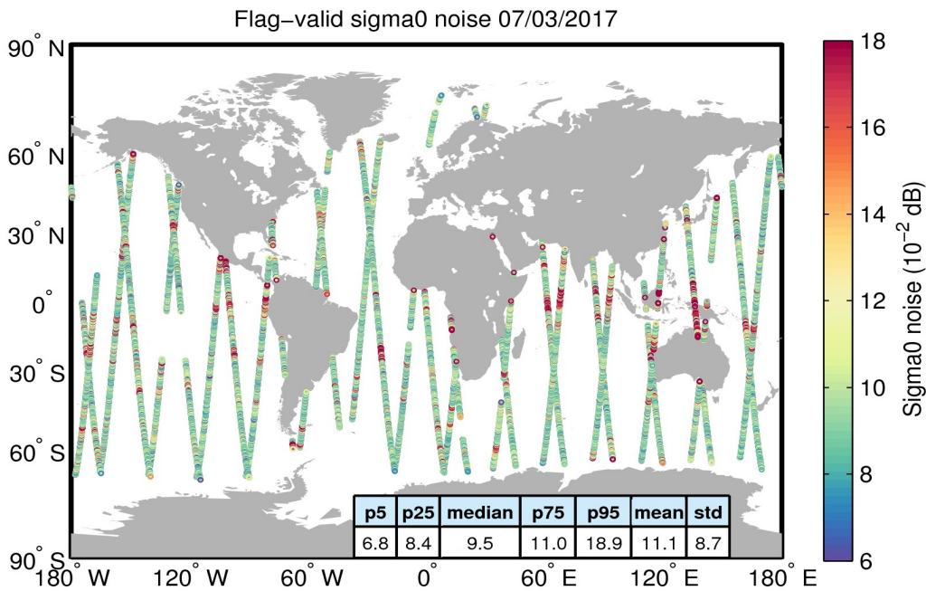
Figure 26. Geographical distribution of flag-valid 20-Hz sigma0 measurement noise over oceans and lakes for 07/03/2017. The statistical values shown in the table refer to the sigma0 noise and are calculated over all measurements shown in the figure.
