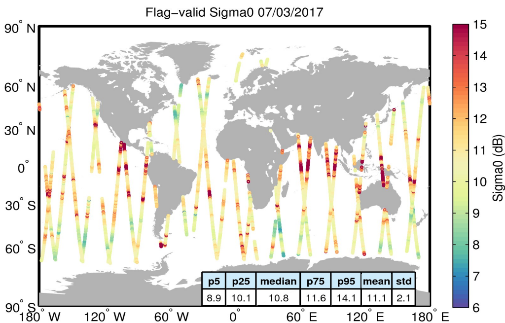
Figure 23. Geographical distribution of flag-valid sigma0 data over oceans and lakes for 07/03/2017. The statistical values shown in the table refer to the sigma0 in dB and are calculated over all measurements shown in the figure.
