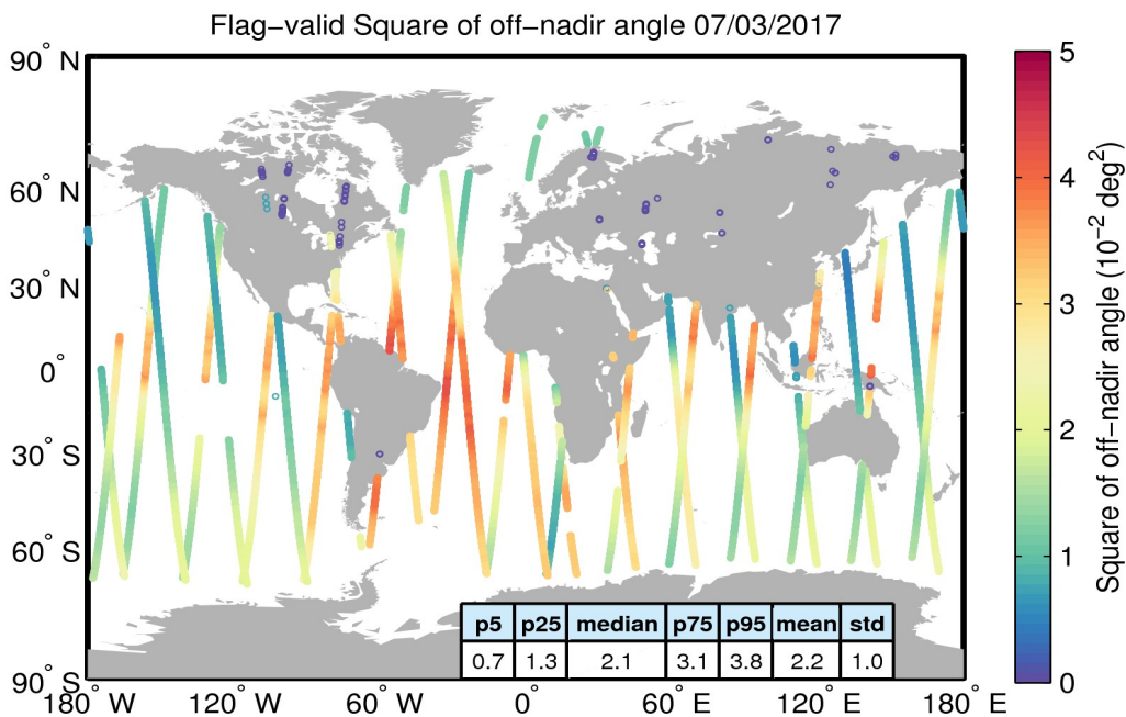
Figure 37. Geographical distribution of flag-valid mispointing data over oceans and lakes for 07/03/2017. The statistical values shown in the table refer to the mispointing in 10^{-2} deg 2 and are calculated over all measurements shown in the figure.
