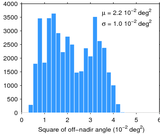
Figure 39. Histogram of flag-valid mispointing over oceans and lakes for 07/03/2017. The mean ( \mu ) and standard deviation ( \sigma ) are also shown. Note that values larger than 6 \cdot 10^{-2} \text{ deg}^2 are excluded from the histogram for the sake of readability but not from the computation of \mu and \sigma .
