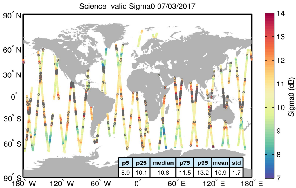
Figure 27. Geographical distribution of science-valid sigma0 data over oceans and lakes for 07/03/2017. The statistical values shown in the table refer to the sigma0 in dB and are calculated over all measurements shown in the figure. Gray circles denote records that have been rejected based on the editing criteria described in Table 4.
