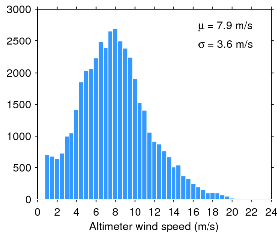
Figure 35. Histogram of science-valid wind over oceans and lakes for 07/03/2017. The mean ( \mu ) and standard deviation ( \sigma ) are also shown. Note that values larger than 24 m/s are excluded from the histogram for the sake of readability but not from the computation of \mu and \sigma .
