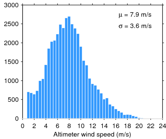
Figure 33. Histogram of flag-valid wind over oceans and lakes for 07/03/2017. The mean ( \mu ) and standard deviation ( \sigma ) are also shown. Note that values larger than 24 m/s are excluded from the histogram for the sake of readability but not from the computation of \mu and \sigma .
