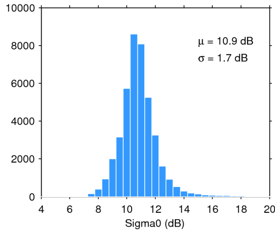
Figure 28. Histogram of science-valid sigma0 over oceans and lakes for 07/03/2017. The mean ( \mu ) and standard deviation ( \sigma ) are also shown. Note that values outside [4 20] dB are excluded from the histogram for the sake of readability but not from the computation of \mu and \sigma .
