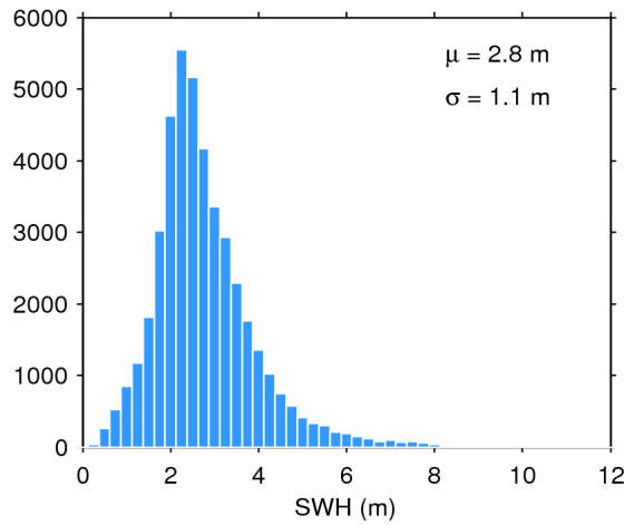
Figure 17. Histogram of flag-valid SWH over oceans and lakes for 07/03/2017. The mean ( \mu ) and standard deviation ( \sigma ) are also shown. Note that values larger than 12 m are excluded from the histogram for the sake of readability but not from the computation of \mu and \sigma .
