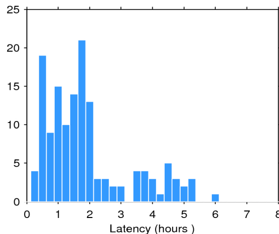
Figure 2. Histogram of the data latency for 07/03/2017. The y-axis denotes the number of files that are made available with a delay of x-hours with respect to the mean time of the records stored in the file.
