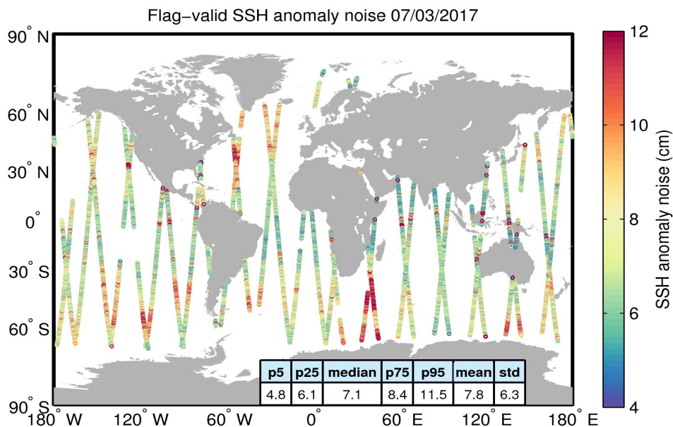
Figure 8. Geographical distribution of flag-valid 20-Hz SSH anomaly measurement noise over oceans and lakes for 07/03/2017. The statistical values shown in the table refer to the SSH anomaly noise and are calculated over all measurements shown in the figure.
