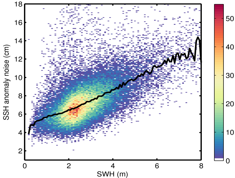
Figure 9. 2D histogram showing flag-valid SSH anomaly noise as a function of SWH for 07/03/2017. The black line denotes the median SSH anomaly noise as a function of SWH.
