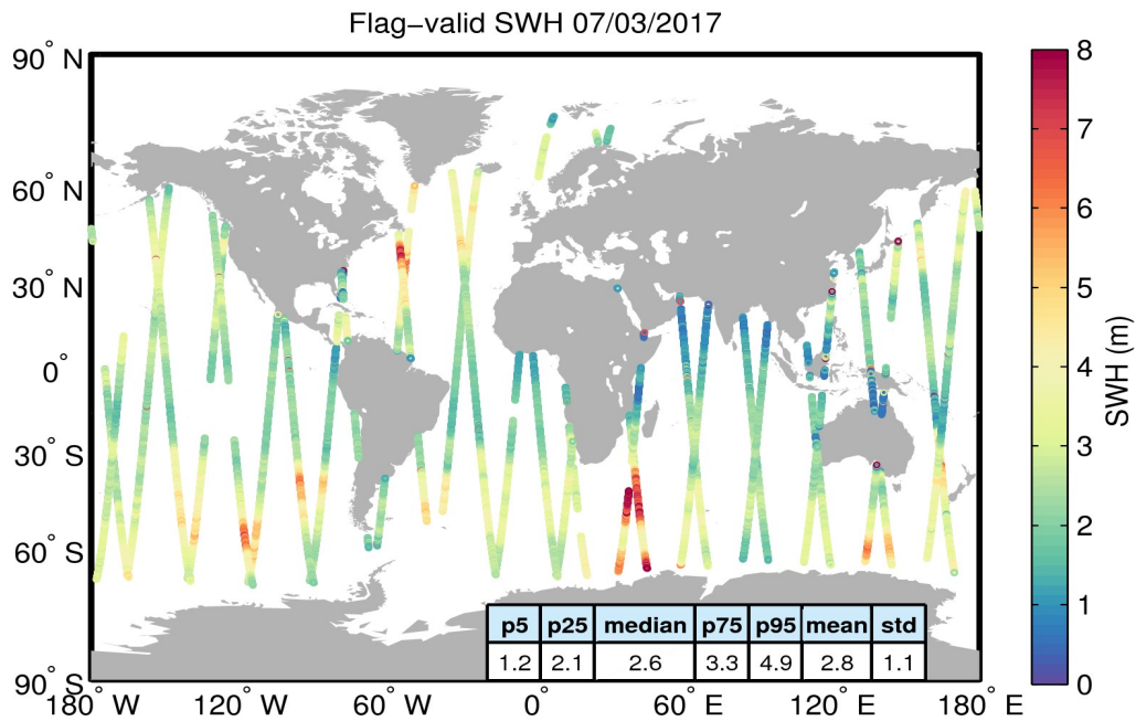
Figure 15. Geographical distribution of flag-valid SWH data over oceans and lakes for 07/03/2017. The statistical values shown in the table refer to the SWH in m and are calculated over all measurements shown in the figure.
