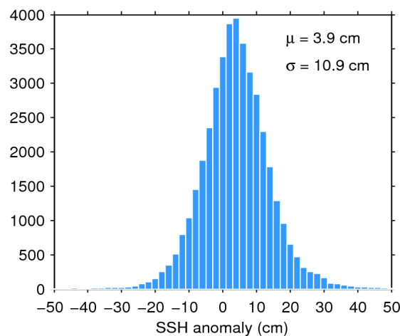
Figure 11. Histogram of science-valid SSH anomaly over oceans and lakes for 07/03/2017. The mean ( \mu ) and standard deviation ( \sigma ) are also shown. Note that values outside [-50 50] cm are excluded from the histogram for the sake of readability but not from the computation of \mu and \sigma .
