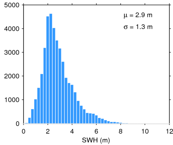
Figure 17. Histogram of flag-valid SWH over oceans and lakes for 05/03/2017. The mean ( \mu ) and standard deviation ( \sigma ) are also shown. Note that values larger than 12 m are excluded from the histogram for the sake of readability but not from the computation of \mu and \sigma .
