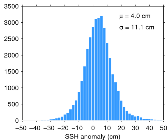
Figure 11. Histogram of science-valid SSH anomaly over oceans and lakes for 05/03/2017. The mean ( \mu ) and standard deviation ( \sigma ) are also shown. Note that values outside [-50 50] cm are excluded from the histogram for the sake of readability but not from the computation of \mu and \sigma .
