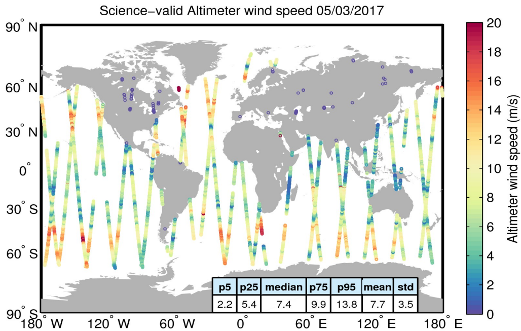
Figure 34. Geographical distribution of science-valid wind data over oceans and lakes for 05/03/2017. The statistical values shown in the table refer to the wind in m/s and are calculated over all measurements shown in the figure. Gray circles denote records that have been rejected based on the editing criteria described in Table 5.
