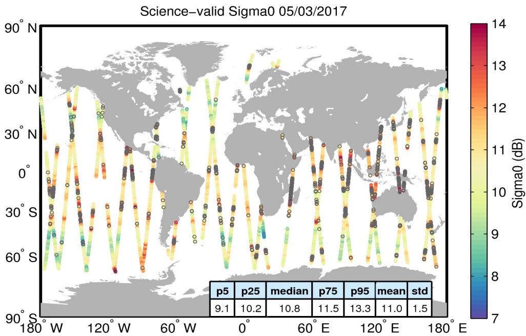
Figure 27. Geographical distribution of science-valid sigma0 data over oceans and lakes for 05/03/2017. The statistical values shown in the table refer to the sigma0 in dB and are calculated over all measurements shown in the figure. Gray circles denote records that have been rejected based on the editing criteria described in Table 4.
