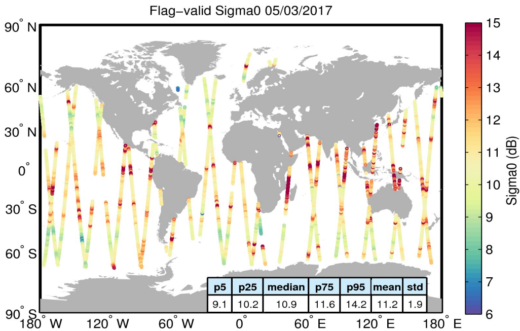
Figure 23. Geographical distribution of flag-valid sigma0 data over oceans and lakes for 05/03/2017. The statistical values shown in the table refer to the sigma0 in dB and are calculated over all measurements shown in the figure.
