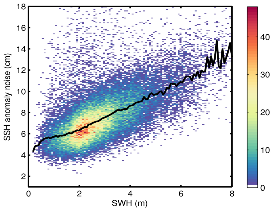
Figure 9. 2D histogram showing flag-valid SSH anomaly noise as a function of SWH for 05/03/2017. The black line denotes the median SSH anomaly noise as a function of SWH.
