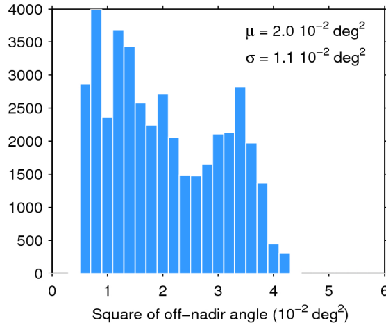
Figure 39. Histogram of flag-valid mispointing over oceans and lakes for 05/03/2017. The mean ( \mu ) and standard deviation ( \sigma ) are also shown. Note that values larger than 6 \cdot 10^{-2} \text{ deg}^2 are excluded from the histogram for the sake of readability but not from the computation of \mu and \sigma .
