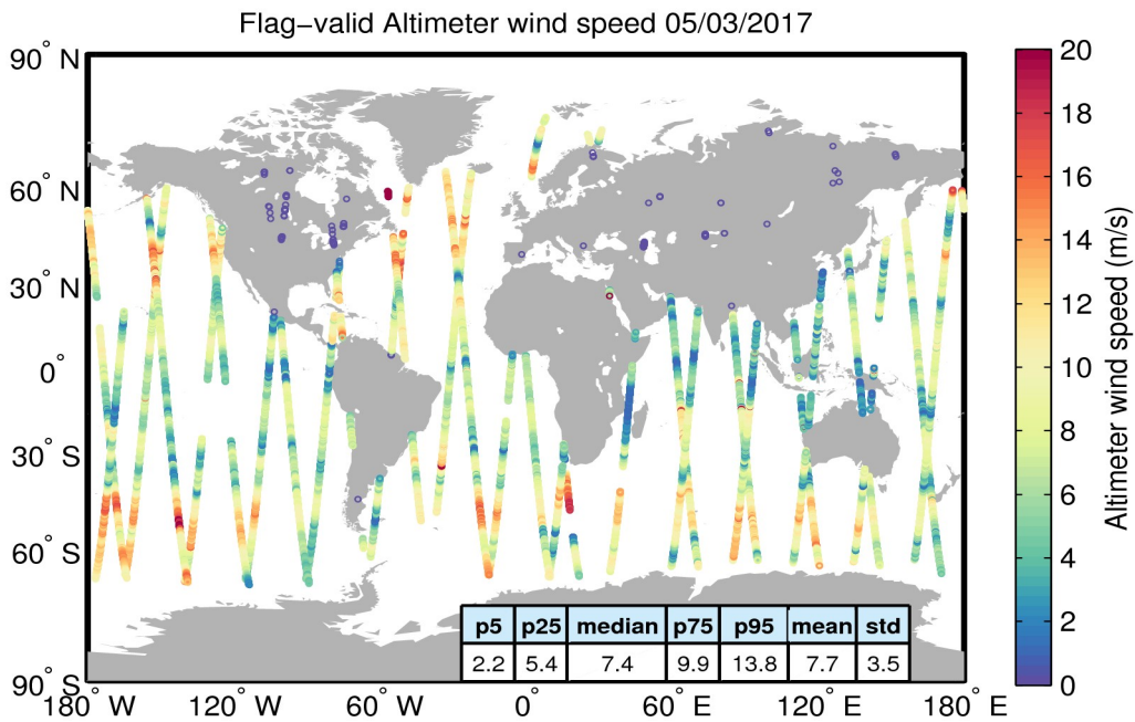
Figure 31. Geographical distribution of flag-valid wind data over oceans and lakes for 05/03/2017. The statistical values shown in the table refer to the wind in m/s and are calculated over all measurements shown in the figure.
