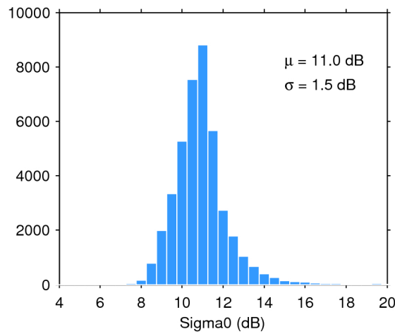
Figure 28. Histogram of science-valid sigma0 over oceans and lakes for 05/03/2017. The mean ( \mu ) and standard deviation ( \sigma ) are also shown. Note that values outside [4 20] dB are excluded from the histogram for the sake of readability but not from the computation of \mu and \sigma .
