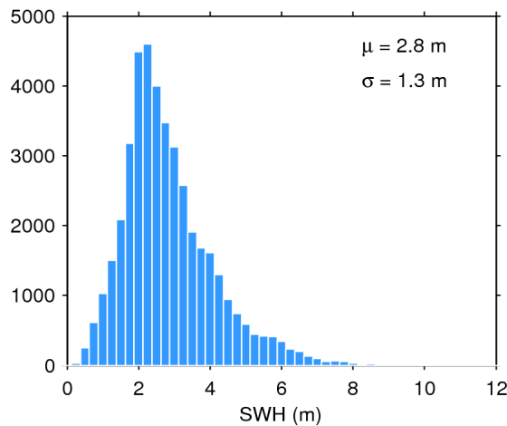
Figure 20. Histogram of science-valid SWH over oceans and lakes for 05/03/2017. The mean ( \mu ) and standard deviation ( \sigma ) are also shown. Note that values larger than 12 m are excluded from the histogram for the sake of readability but not from the computation of \mu and \sigma .
