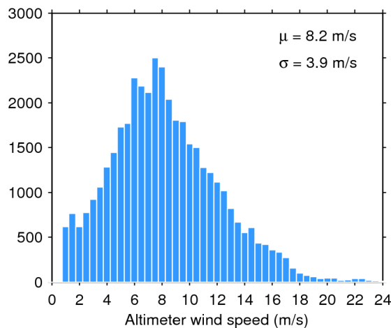
Figure 35. Histogram of science-valid wind over oceans and lakes for 04/03/2017. The mean ( \mu ) and standard deviation ( \sigma ) are also shown. Note that values larger than 24 m/s are excluded from the histogram for the sake of readability but not from the computation of \mu and \sigma .
