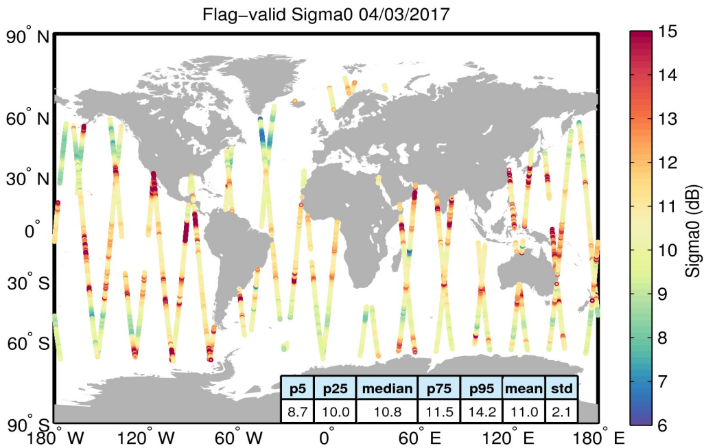
Figure 23. Geographical distribution of flag-valid sigma0 data over oceans and lakes for 04/03/2017. The statistical values shown in the table refer to the sigma0 in dB and are calculated over all measurements shown in the figure.
