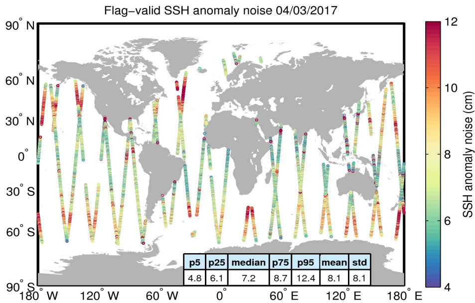
Figure 8. Geographical distribution of flag-valid 20-Hz SSH anomaly measurement noise over oceans and lakes for 04/03/2017. The statistical values shown in the table refer to the SSH anomaly noise and are calculated over all measurements shown in the figure.
