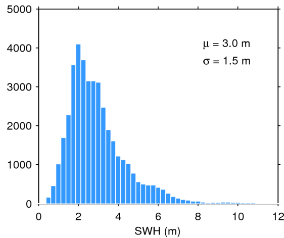
Figure 17. Histogram of flag-valid SWH over oceans and lakes for 04/03/2017. The mean ( \mu ) and standard deviation ( \sigma ) are also shown. Note that values larger than 12 m are excluded from the histogram for the sake of readability but not from the computation of \mu and \sigma .
