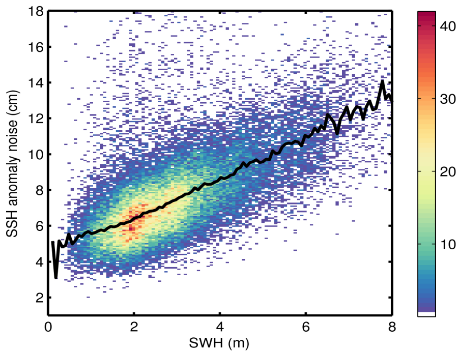
Figure 9. 2D histogram showing flag-valid SSH anomaly noise as a function of SWH for 04/03/2017. The black line denotes the median SSH anomaly noise as a function of SWH.
