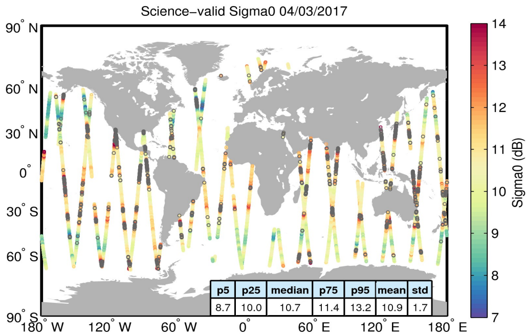
Figure 27. Geographical distribution of science-valid sigma0 data over oceans and lakes for 04/03/2017. The statistical values shown in the table refer to the sigma0 in dB and are calculated over all measurements shown in the figure. Gray circles denote records that have been rejected based on the editing criteria described in Table 4.
