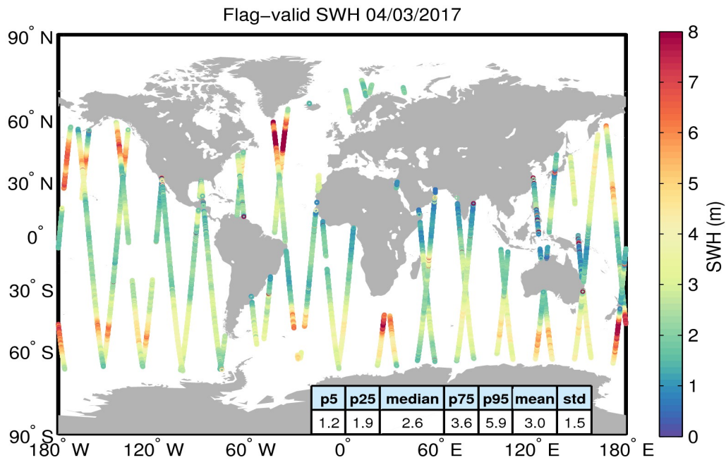
Figure 15. Geographical distribution of flag-valid SWH data over oceans and lakes for 04/03/2017. The statistical values shown in the table refer to the SWH in m and are calculated over all measurements shown in the figure.
