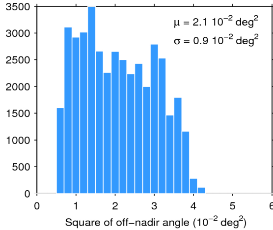
Figure 39. Histogram of flag-valid mispointing over oceans and lakes for 04/03/2017. The mean ( \mu ) and standard deviation ( \sigma ) are also shown. Note that values larger than 6 \cdot 10^{-2} \text{ deg}^2 are excluded from the histogram for the sake of readability but not from the computation of \mu and \sigma .
