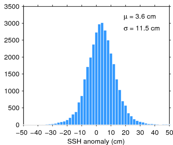
Figure 11. Histogram of science-valid SSH anomaly over oceans and lakes for 04/03/2017. The mean ( \mu ) and standard deviation ( \sigma ) are also shown. Note that values outside [-50 50] cm are excluded from the histogram for the sake of readability but not from the computation of \mu and \sigma .
