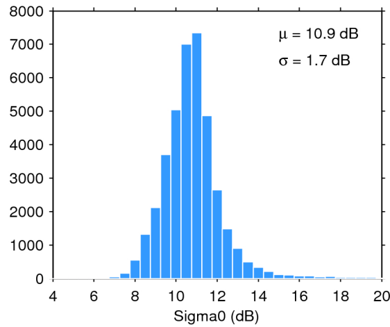
Figure 28. Histogram of science-valid sigma0 over oceans and lakes for 04/03/2017. The mean ( \mu ) and standard deviation ( \sigma ) are also shown. Note that values outside [4 20] dB are excluded from the histogram for the sake of readability but not from the computation of \mu and \sigma .
