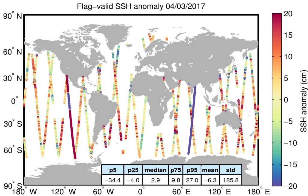
Figure 5. Geographical distribution of flag-valid 1-Hz SSH anomaly data over oceans and lakes for 04/03/2017. The statistical values shown in the table refer to the SSH anomaly in cm and are calculated over all measurements shown in the figure.
