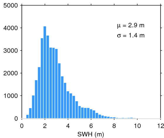
Figure 20. Histogram of science-valid SWH over oceans and lakes for 04/03/2017. The mean ( \mu ) and standard deviation ( \sigma ) are also shown. Note that values larger than 12 m are excluded from the histogram for the sake of readability but not from the computation of \mu and \sigma .
