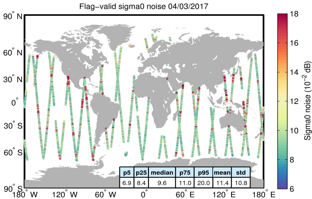
Figure 26. Geographical distribution of flag-valid 20-Hz sigma0 measurement noise over oceans and lakes for 04/03/2017. The statistical values shown in the table refer to the sigma0 noise and are calculated over all measurements shown in the figure.
