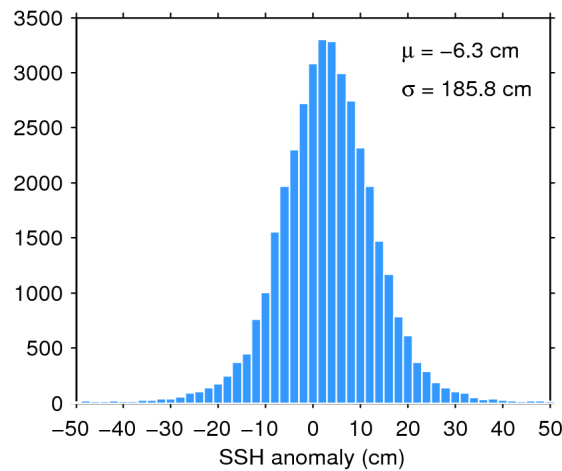
Figure 7. Histogram of flag-valid SSH anomaly over oceans and lakes for 04/03/2017. The mean ( \mu ) and standard deviation ( \sigma ) are also shown. Note that values outside [-50 50] cm are excluded from the histogram for the sake of readability but not from the computation of \mu and \sigma .
