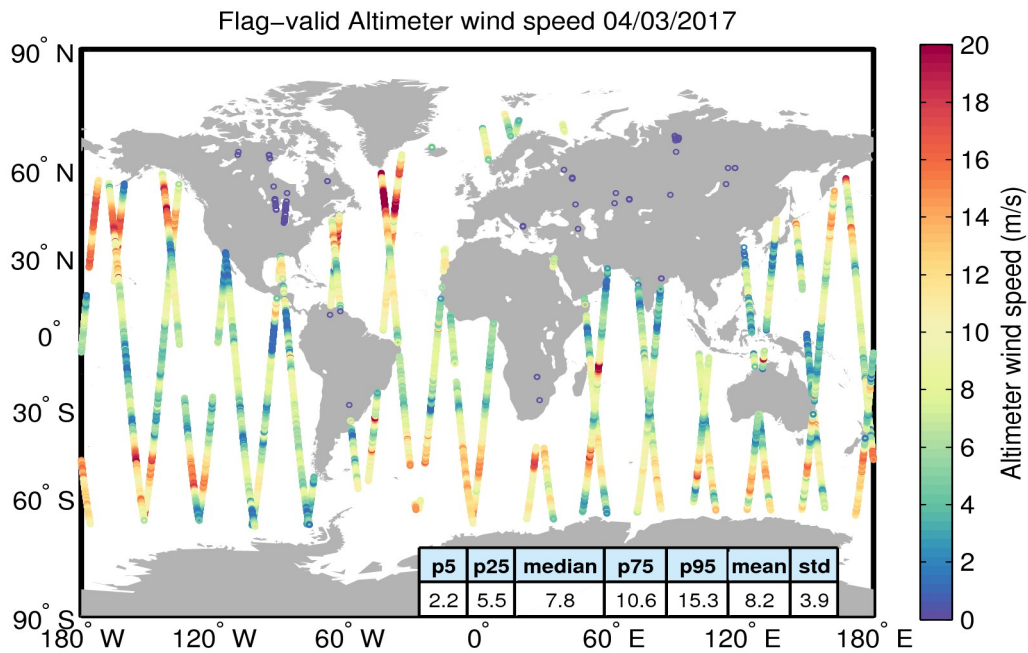
Figure 31. Geographical distribution of flag-valid wind data over oceans and lakes for 04/03/2017. The statistical values shown in the table refer to the wind in m/s and are calculated over all measurements shown in the figure.
