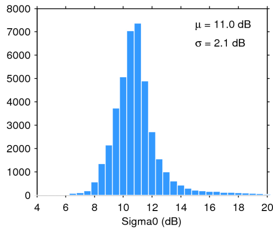
Figure 25. Histogram of flag-valid sigma0 over oceans and lakes for 04/03/2017. The mean ( \mu ) and standard deviation ( \sigma ) are also shown. Note that values outside [4 20] dB are excluded from the histogram for the sake of readability but not from the computation of \mu and \sigma .
