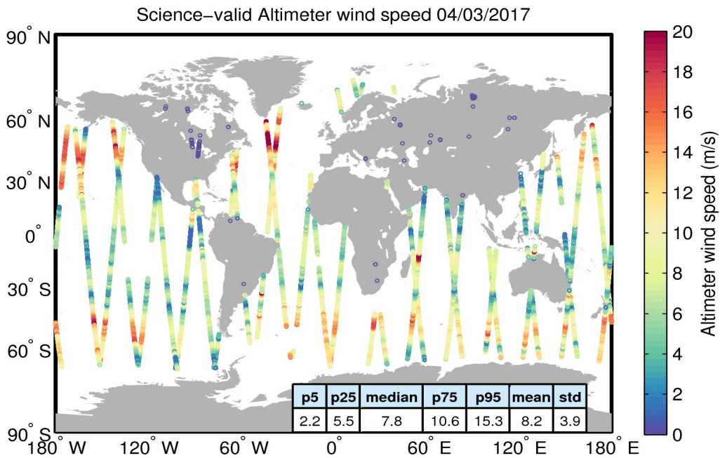
Figure 34. Geographical distribution of science-valid wind data over oceans and lakes for 04/03/2017. The statistical values shown in the table refer to the wind in m/s and are calculated over all measurements shown in the figure. Gray circles denote records that have been rejected based on the editing criteria described in Table 5.
