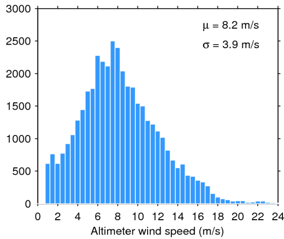
Figure 33. Histogram of flag-valid wind over oceans and lakes for 04/03/2017. The mean ( \mu ) and standard deviation ( \sigma ) are also shown. Note that values larger than 24 m/s are excluded from the histogram for the sake of readability but not from the computation of \mu and \sigma .
