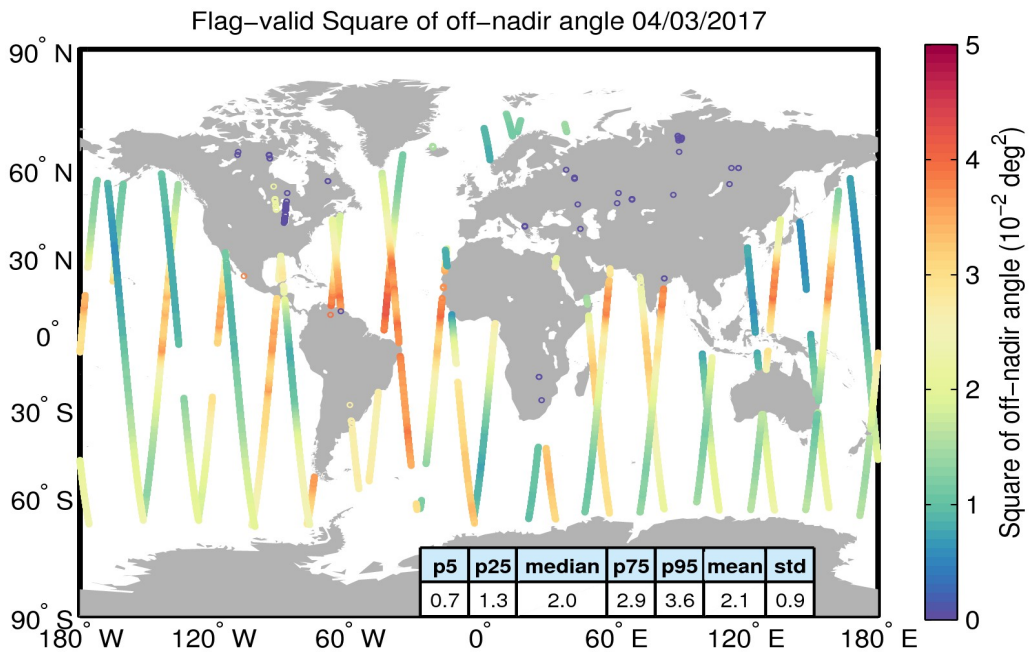
Figure 37. Geographical distribution of flag-valid mispointing data over oceans and lakes for 04/03/2017. The statistical values shown in the table refer to the mispointing in 10^{-2} deg 2 and are calculated over all measurements shown in the figure.
