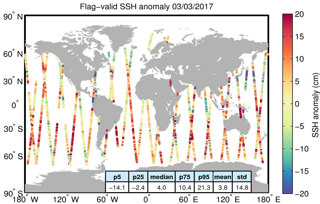
Figure 5. Geographical distribution of flag-valid 1-Hz SSH anomaly data over oceans and lakes for 03/03/2017. The statistical values shown in the table refer to the SSH anomaly in cm and are calculated over all measurements shown in the figure.
