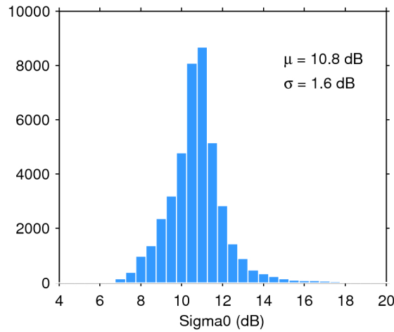
Figure 28. Histogram of science-valid sigma0 over oceans and lakes for 03/03/2017. The mean ( \mu ) and standard deviation ( \sigma ) are also shown. Note that values outside [4 20] dB are excluded from the histogram for the sake of readability but not from the computation of \mu and \sigma .
