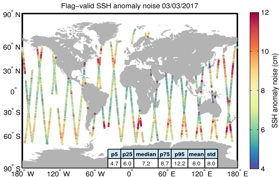
Figure 8. Geographical distribution of flag-valid 20-Hz SSH anomaly measurement noise over oceans and lakes for 03/03/2017. The statistical values shown in the table refer to the SSH anomaly noise and are calculated over all measurements shown in the figure.
