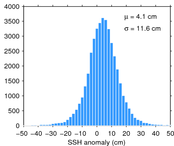
Figure 11. Histogram of science-valid SSH anomaly over oceans and lakes for 03/03/2017. The mean ( \mu ) and standard deviation ( \sigma ) are also shown. Note that values outside [-50 50] cm are excluded from the histogram for the sake of readability but not from the computation of \mu and \sigma .
