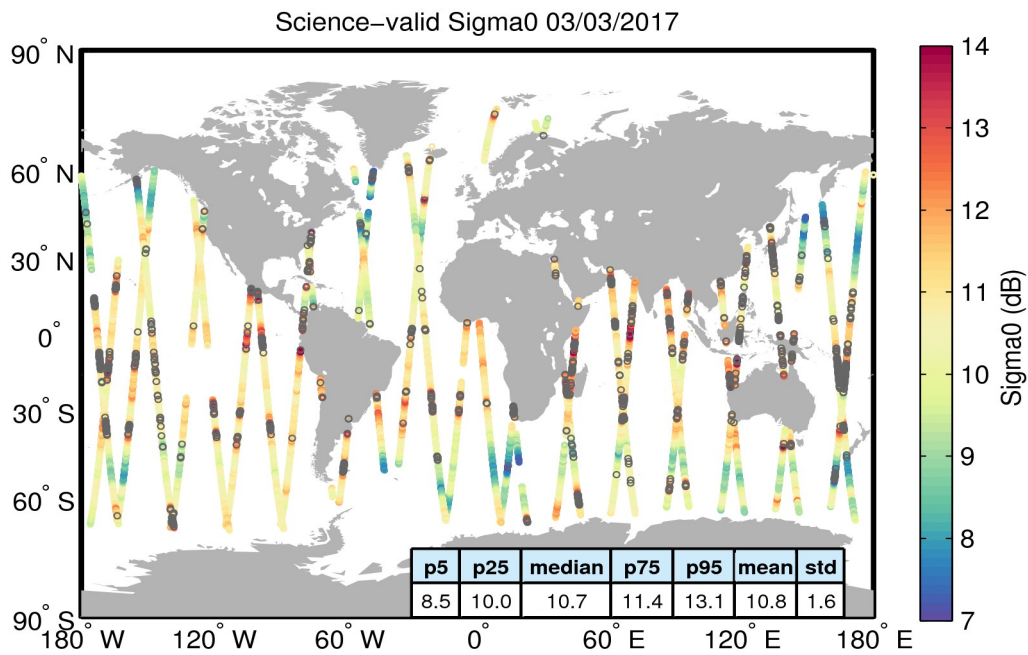
Figure 27. Geographical distribution of science-valid sigma0 data over oceans and lakes for 03/03/2017. The statistical values shown in the table refer to the sigma0 in dB and are calculated over all measurements shown in the figure. Gray circles denote records that have been rejected based on the editing criteria described in Table 4.
