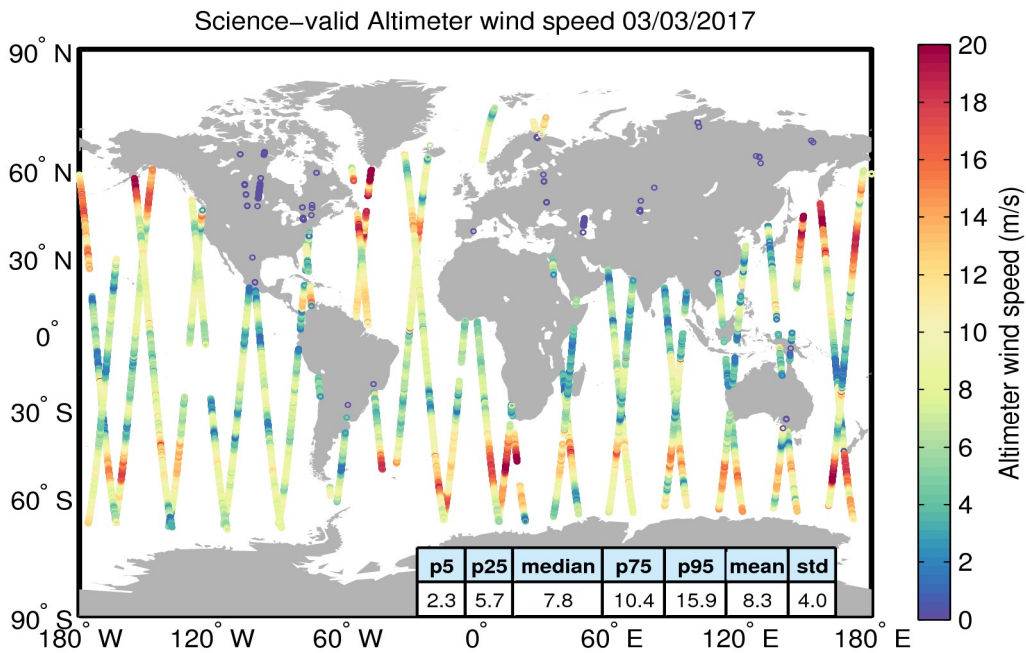
Figure 34. Geographical distribution of science-valid wind data over oceans and lakes for 03/03/2017. The statistical values shown in the table refer to the wind in m/s and are calculated over all measurements shown in the figure. Gray circles denote records that have been rejected based on the editing criteria described in Table 5.
