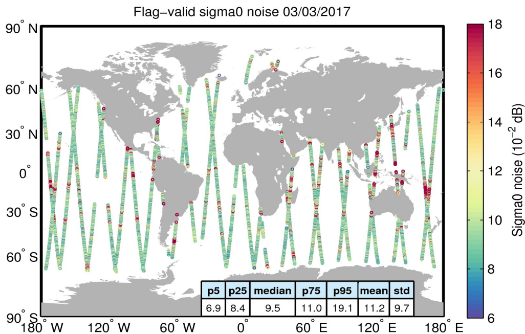
Figure 26. Geographical distribution of flag-valid 20-Hz sigma0 measurement noise over oceans and lakes for 03/03/2017. The statistical values shown in the table refer to the sigma0 noise and are calculated over all measurements shown in the figure.
