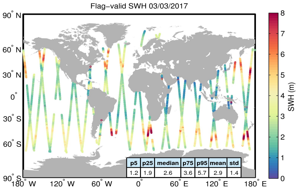
Figure 15. Geographical distribution of flag-valid SWH data over oceans and lakes for 03/03/2017. The statistical values shown in the table refer to the SWH in m and are calculated over all measurements shown in the figure.
