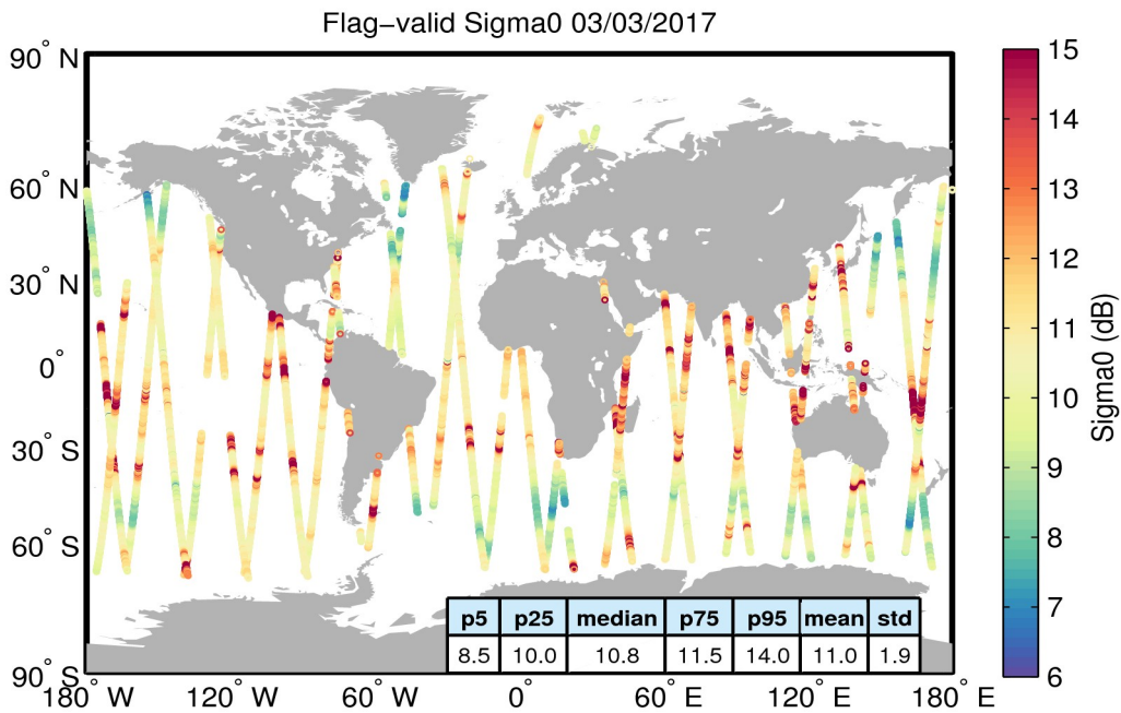
Figure 23. Geographical distribution of flag-valid sigma0 data over oceans and lakes for 03/03/2017. The statistical values shown in the table refer to the sigma0 in dB and are calculated over all measurements shown in the figure.
