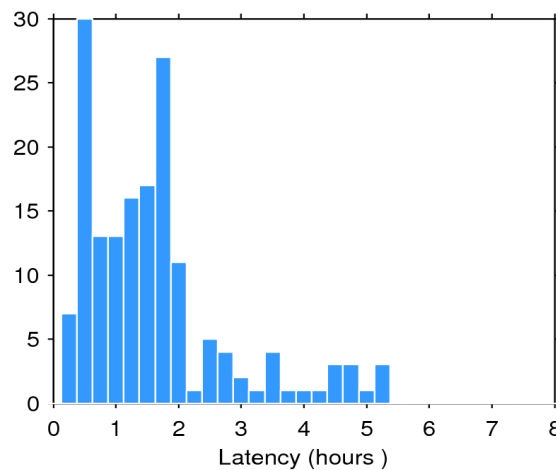
Figure 2. Histogram of the data latency for 03/03/2017. The y-axis denotes the number of files that are made available with a delay of x-hours with respect to the mean time of the records stored in the file.
