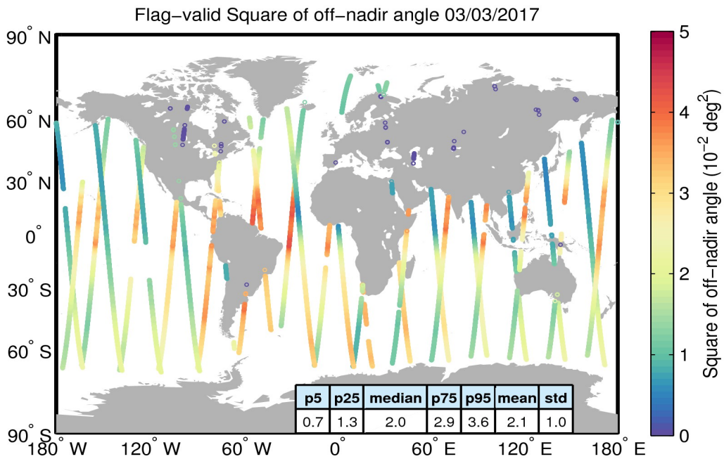
Figure 37. Geographical distribution of flag-valid mispointing data over oceans and lakes for 03/03/2017. The statistical values shown in the table refer to the mispointing in 10^{-2} deg 2 and are calculated over all measurements shown in the figure.
