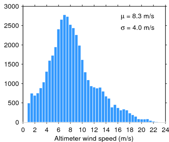
Figure 35. Histogram of science-valid wind over oceans and lakes for 03/03/2017. The mean ( \mu ) and standard deviation ( \sigma ) are also shown. Note that values larger than 24 m/s are excluded from the histogram for the sake of readability but not from the computation of \mu and \sigma .
