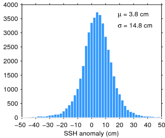
Figure 7. Histogram of flag-valid SSH anomaly over oceans and lakes for 03/03/2017. The mean ( \mu ) and standard deviation ( \sigma ) are also shown. Note that values outside [-50 50] cm are excluded from the histogram for the sake of readability but not from the computation of \mu and \sigma .
