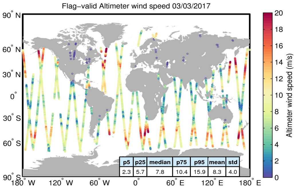
Figure 31. Geographical distribution of flag-valid wind data over oceans and lakes for 03/03/2017. The statistical values shown in the table refer to the wind in m/s and are calculated over all measurements shown in the figure.
