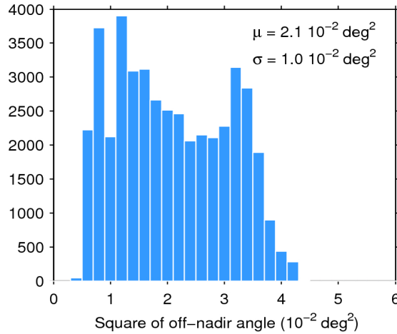
Figure 39. Histogram of flag-valid mispointing over oceans and lakes for 03/03/2017. The mean ( \mu ) and standard deviation ( \sigma ) are also shown. Note that values larger than 6 \cdot 10^{-2} \text{ deg}^2 are excluded from the histogram for the sake of readability but not from the computation of \mu and \sigma .
