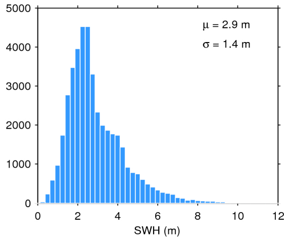
Figure 20. Histogram of science-valid SWH over oceans and lakes for 03/03/2017. The mean ( \mu ) and standard deviation ( \sigma ) are also shown. Note that values larger than 12 m are excluded from the histogram for the sake of readability but not from the computation of \mu and \sigma .
