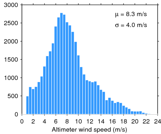
Figure 33. Histogram of flag-valid wind over oceans and lakes for 03/03/2017. The mean ( \mu ) and standard deviation ( \sigma ) are also shown. Note that values larger than 24 m/s are excluded from the histogram for the sake of readability but not from the computation of \mu and \sigma .
