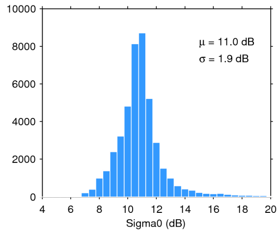
Figure 25. Histogram of flag-valid sigma0 over oceans and lakes for 03/03/2017. The mean ( \mu ) and standard deviation ( \sigma ) are also shown. Note that values outside [4 20] dB are excluded from the histogram for the sake of readability but not from the computation of \mu and \sigma .
