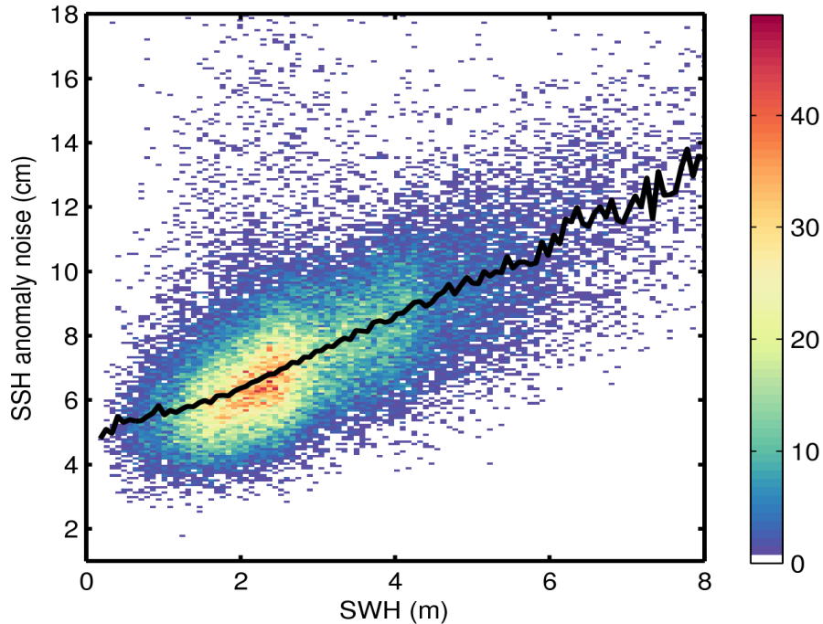
Figure 9. 2D histogram showing flag-valid SSH anomaly noise as a function of SWH for 03/03/2017. The black line denotes the median SSH anomaly noise as a function of SWH.
