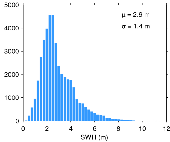
Figure 17. Histogram of flag-valid SWH over oceans and lakes for 03/03/2017. The mean ( \mu ) and standard deviation ( \sigma ) are also shown. Note that values larger than 12 m are excluded from the histogram for the sake of readability but not from the computation of \mu and \sigma .
