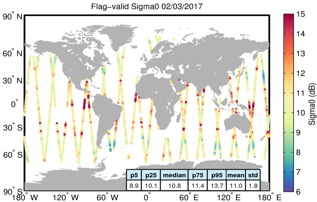
Figure 23. Geographical distribution of flag-valid sigma0 data over oceans and lakes for 02/03/2017. The statistical values shown in the table refer to the sigma0 in dB and are calculated over all measurements shown in the figure.
