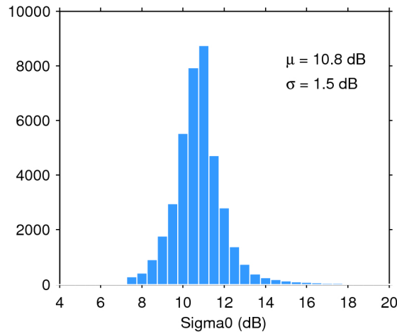
Figure 28. Histogram of science-valid sigma0 over oceans and lakes for 02/03/2017. The mean ( \mu ) and standard deviation ( \sigma ) are also shown. Note that values outside [4 20] dB are excluded from the histogram for the sake of readability but not from the computation of \mu and \sigma .
