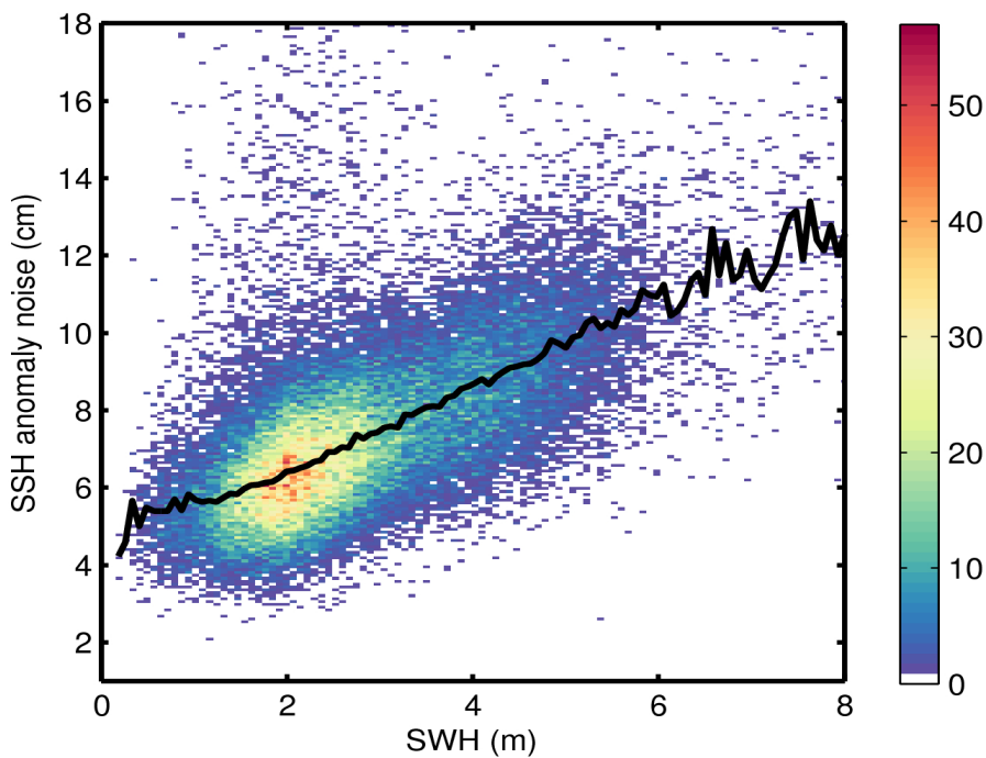
Figure 9. 2D histogram showing flag-valid SSH anomaly noise as a function of SWH for 02/03/2017. The black line denotes the median SSH anomaly noise as a function of SWH.
