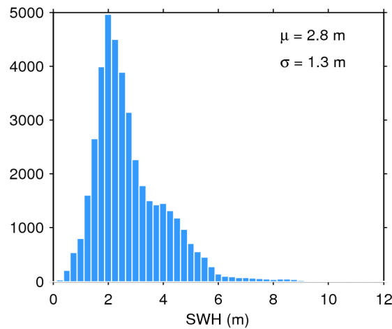
Figure 17. Histogram of flag-valid SWH over oceans and lakes for 02/03/2017. The mean ( \mu ) and standard deviation ( \sigma ) are also shown. Note that values larger than 12 m are excluded from the histogram for the sake of readability but not from the computation of \mu and \sigma .
