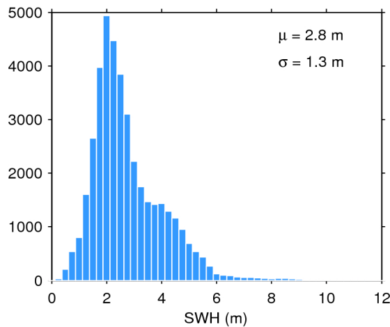
Figure 20. Histogram of science-valid SWH over oceans and lakes for 02/03/2017. The mean ( \mu ) and standard deviation ( \sigma ) are also shown. Note that values larger than 12 m are excluded from the histogram for the sake of readability but not from the computation of \mu and \sigma .
