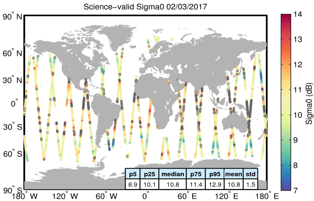
Figure 27. Geographical distribution of science-valid sigma0 data over oceans and lakes for 02/03/2017. The statistical values shown in the table refer to the sigma0 in dB and are calculated over all measurements shown in the figure. Gray circles denote records that have been rejected based on the editing criteria described in Table 4.
