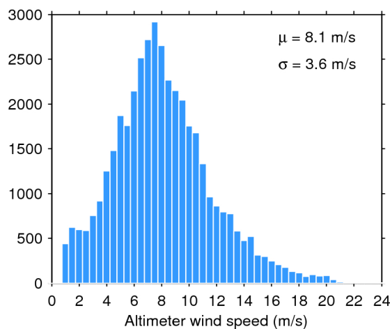
Figure 35. Histogram of science-valid wind over oceans and lakes for 02/03/2017. The mean ( \mu ) and standard deviation ( \sigma ) are also shown. Note that values larger than 24 m/s are excluded from the histogram for the sake of readability but not from the computation of \mu and \sigma .
