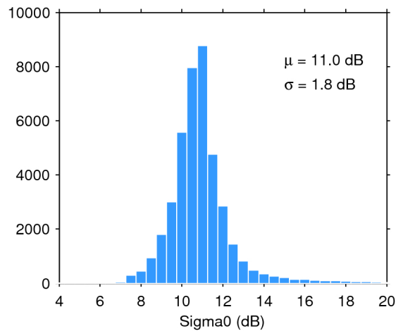
Figure 25. Histogram of flag-valid sigma0 over oceans and lakes for 02/03/2017. The mean ( \mu ) and standard deviation ( \sigma ) are also shown. Note that values outside [4 20] dB are excluded from the histogram for the sake of readability but not from the computation of \mu and \sigma .
