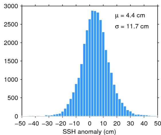
Figure 11. Histogram of science-valid SSH anomaly over oceans and lakes for 02/03/2017. The mean ( \mu ) and standard deviation ( \sigma ) are also shown. Note that values outside [-50 50] cm are excluded from the histogram for the sake of readability but not from the computation of \mu and \sigma .
