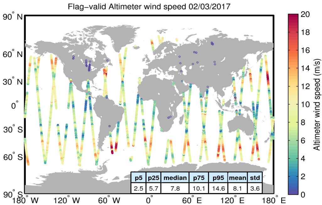
Figure 31. Geographical distribution of flag-valid wind data over oceans and lakes for 02/03/2017. The statistical values shown in the table refer to the wind in m/s and are calculated over all measurements shown in the figure.
