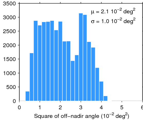
Figure 39. Histogram of flag-valid mispointing over oceans and lakes for 02/03/2017. The mean ( \mu ) and standard deviation ( \sigma ) are also shown. Note that values larger than 6 \cdot 10^{-2} \text{ deg}^2 are excluded from the histogram for the sake of readability but not from the computation of \mu and \sigma .
