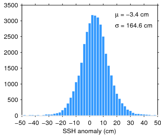
Figure 7. Histogram of flag-valid SSH anomaly over oceans and lakes for 02/03/2017. The mean ( \mu ) and standard deviation ( \sigma ) are also shown. Note that values outside [-50 50] cm are excluded from the histogram for the sake of readability but not from the computation of \mu and \sigma .
