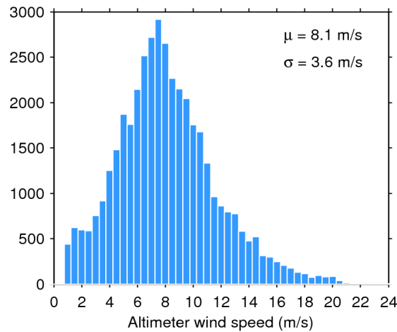
Figure 33. Histogram of flag-valid wind over oceans and lakes for 02/03/2017. The mean ( \mu ) and standard deviation ( \sigma ) are also shown. Note that values larger than 24 m/s are excluded from the histogram for the sake of readability but not from the computation of \mu and \sigma .
