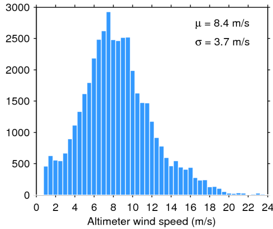
Figure 33. Histogram of flag-valid wind over oceans and lakes for 01/03/2017. The mean ( \mu ) and standard deviation ( \sigma ) are also shown. Note that values larger than 24 m/s are excluded from the histogram for the sake of readability but not from the computation of \mu and \sigma .
