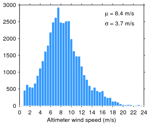
Figure 35. Histogram of science-valid wind over oceans and lakes for 01/03/2017. The mean ( \mu ) and standard deviation ( \sigma ) are also shown. Note that values larger than 24 m/s are excluded from the histogram for the sake of readability but not from the computation of \mu and \sigma .
