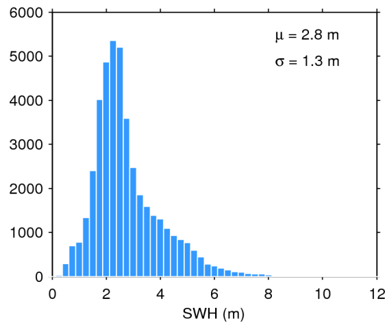
Figure 17. Histogram of flag-valid SWH over oceans and lakes for 01/03/2017. The mean ( \mu ) and standard deviation ( \sigma ) are also shown. Note that values larger than 12 m are excluded from the histogram for the sake of readability but not from the computation of \mu and \sigma .
