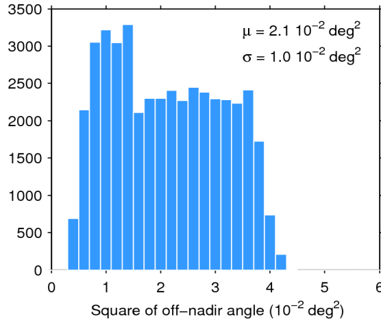
Figure 39. Histogram of flag-valid mispointing over oceans and lakes for 01/03/2017. The mean ( \mu ) and standard deviation ( \sigma ) are also shown. Note that values larger than 6 \cdot 10^{-2} \text{ deg}^2 are excluded from the histogram for the sake of readability but not from the computation of \mu and \sigma .
