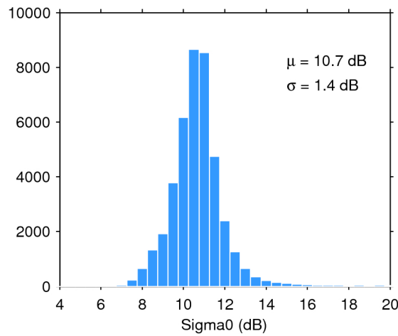
Figure 28. Histogram of science-valid sigma0 over oceans and lakes for 01/03/2017. The mean ( \mu ) and standard deviation ( \sigma ) are also shown. Note that values outside [4 20] dB are excluded from the histogram for the sake of readability but not from the computation of \mu and \sigma .
