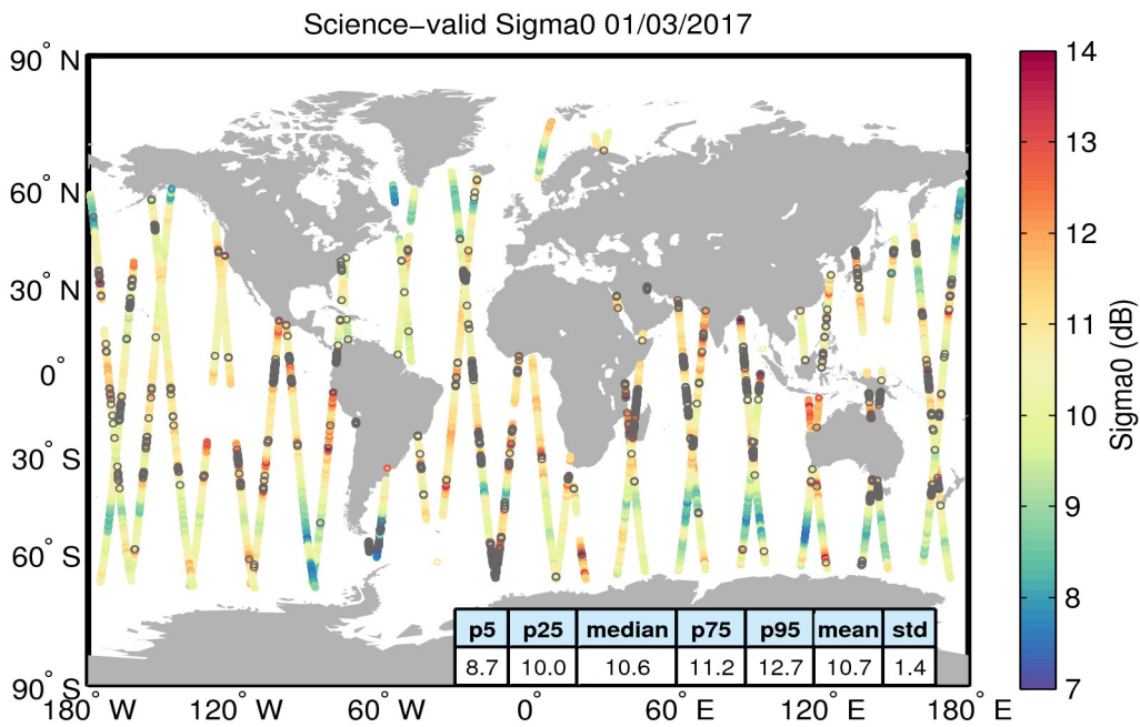
Figure 27. Geographical distribution of science-valid sigma0 data over oceans and lakes for 01/03/2017. The statistical values shown in the table refer to the sigma0 in dB and are calculated over all measurements shown in the figure. Gray circles denote records that have been rejected based on the editing criteria described in Table 4.
