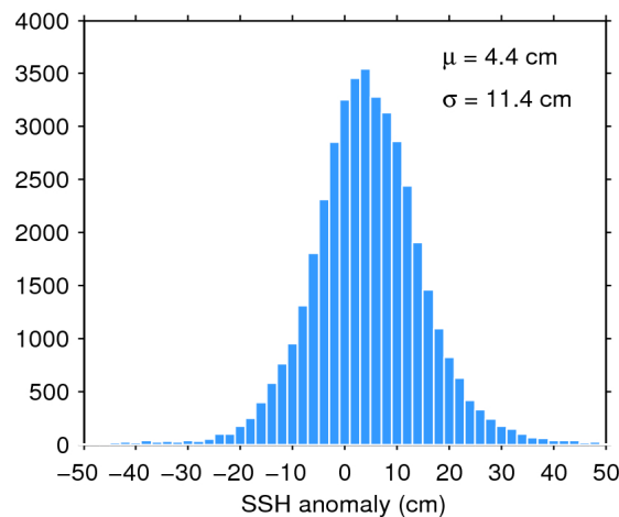
Figure 11. Histogram of science-valid SSH anomaly over oceans and lakes for 01/03/2017. The mean ( \mu ) and standard deviation ( \sigma ) are also shown. Note that values outside [-50 50] cm are excluded from the histogram for the sake of readability but not from the computation of \mu and \sigma .
