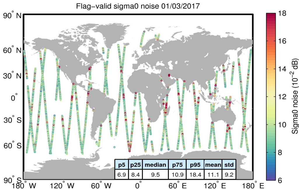
Figure 26. Geographical distribution of flag-valid 20-Hz sigma0 measurement noise over oceans and lakes for 01/03/2017. The statistical values shown in the table refer to the sigma0 noise and are calculated over all measurements shown in the figure.
