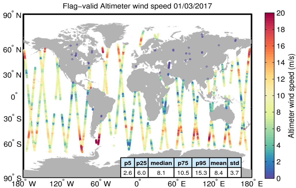
Figure 31. Geographical distribution of flag-valid wind data over oceans and lakes for 01/03/2017. The statistical values shown in the table refer to the wind in m/s and are calculated over all measurements shown in the figure.
