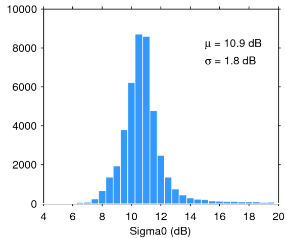
Figure 25. Histogram of flag-valid sigma0 over oceans and lakes for 01/03/2017. The mean ( \mu ) and standard deviation ( \sigma ) are also shown. Note that values outside [4 20] dB are excluded from the histogram for the sake of readability but not from the computation of \mu and \sigma .
