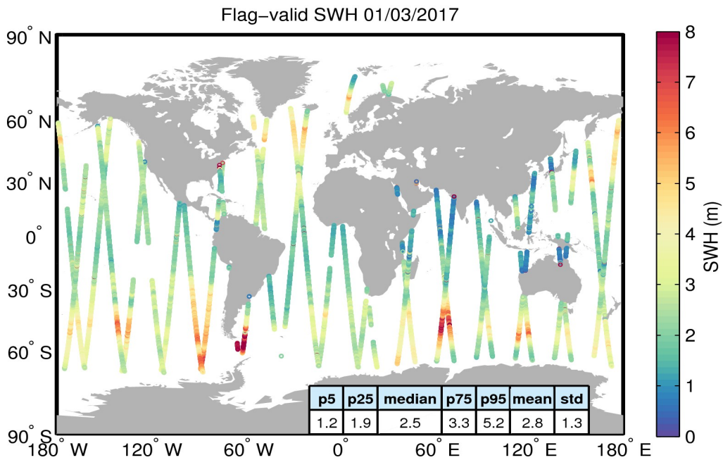
Figure 15. Geographical distribution of flag-valid SWH data over oceans and lakes for 01/03/2017. The statistical values shown in the table refer to the SWH in m and are calculated over all measurements shown in the figure.
