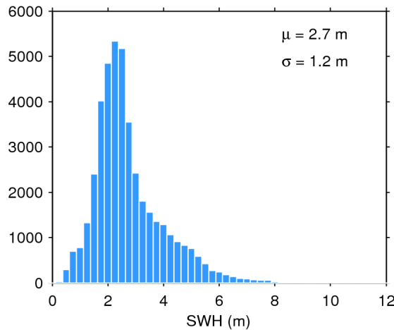
Figure 20. Histogram of science-valid SWH over oceans and lakes for 01/03/2017. The mean ( \mu ) and standard deviation ( \sigma ) are also shown. Note that values larger than 12 m are excluded from the histogram for the sake of readability but not from the computation of \mu and \sigma .
