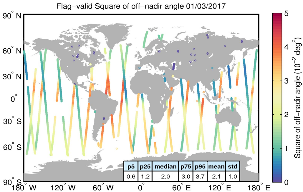
Figure 37. Geographical distribution of flag-valid mispointing data over oceans and lakes for 01/03/2017. The statistical values shown in the table refer to the mispointing in 10^{-2} deg 2 and are calculated over all measurements shown in the figure.
