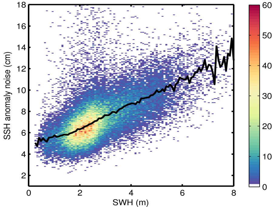
Figure 9. 2D histogram showing flag-valid SSH anomaly noise as a function of SWH for 01/03/2017. The black line denotes the median SSH anomaly noise as a function of SWH.
