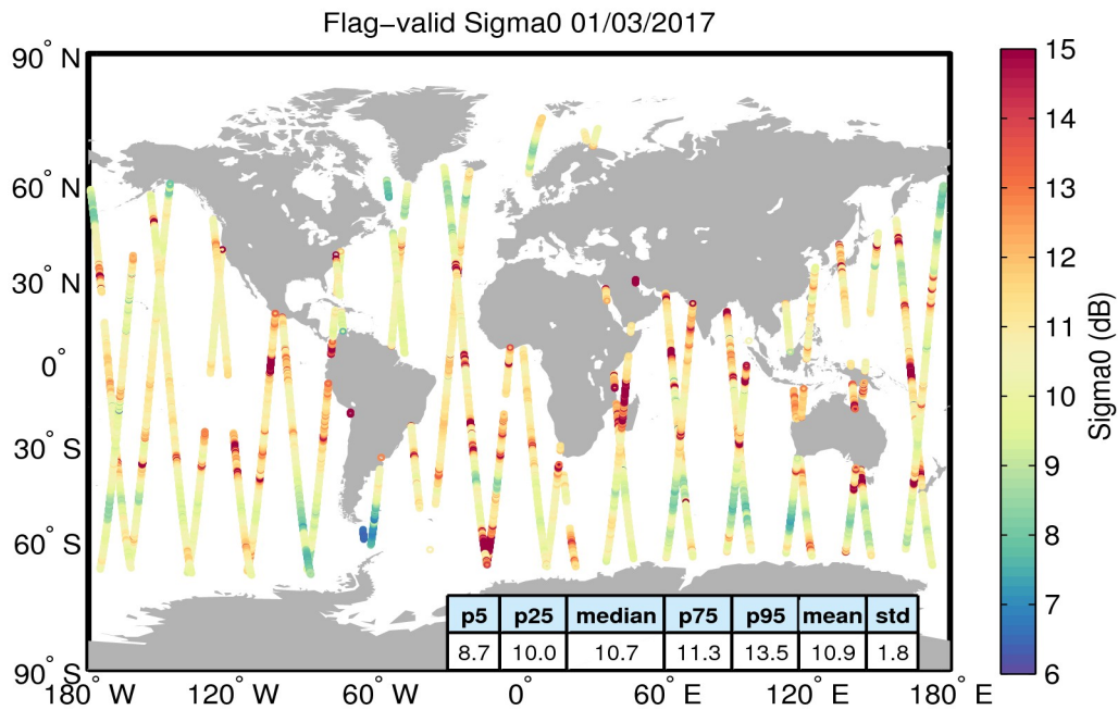
Figure 23. Geographical distribution of flag-valid sigma0 data over oceans and lakes for 01/03/2017. The statistical values shown in the table refer to the sigma0 in dB and are calculated over all measurements shown in the figure.
