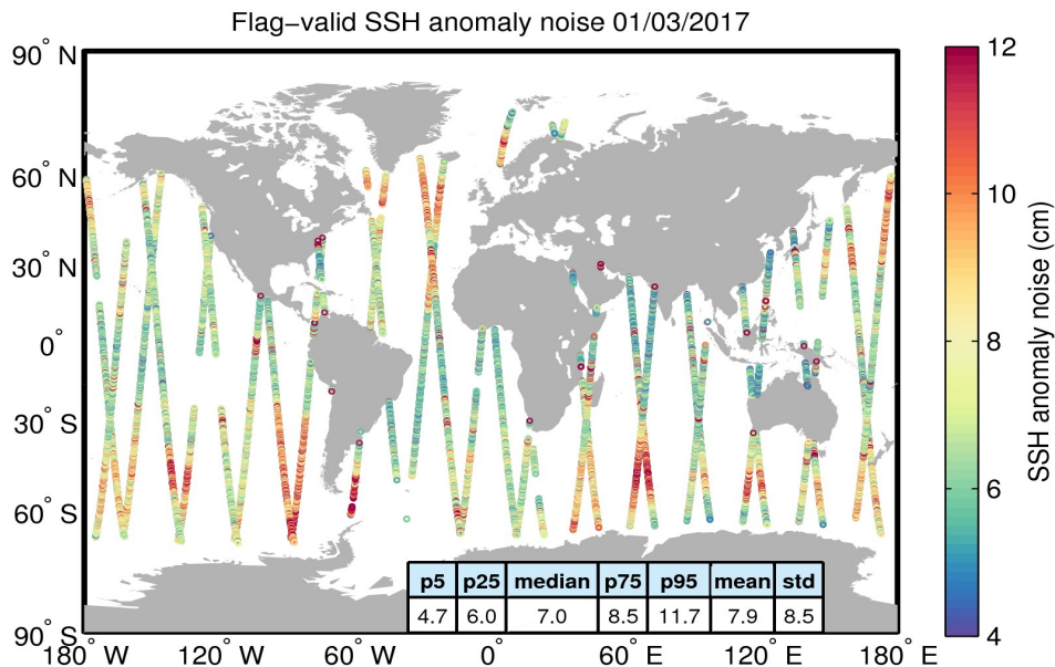
Figure 8. Geographical distribution of flag-valid 20-Hz SSH anomaly measurement noise over oceans and lakes for 01/03/2017. The statistical values shown in the table refer to the SSH anomaly noise and are calculated over all measurements shown in the figure.
