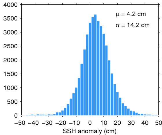
Figure 7. Histogram of flag-valid SSH anomaly over oceans and lakes for 01/03/2017. The mean ( \mu ) and standard deviation ( \sigma ) are also shown. Note that values outside [-50 50] cm are excluded from the histogram for the sake of readability but not from the computation of \mu and \sigma .
