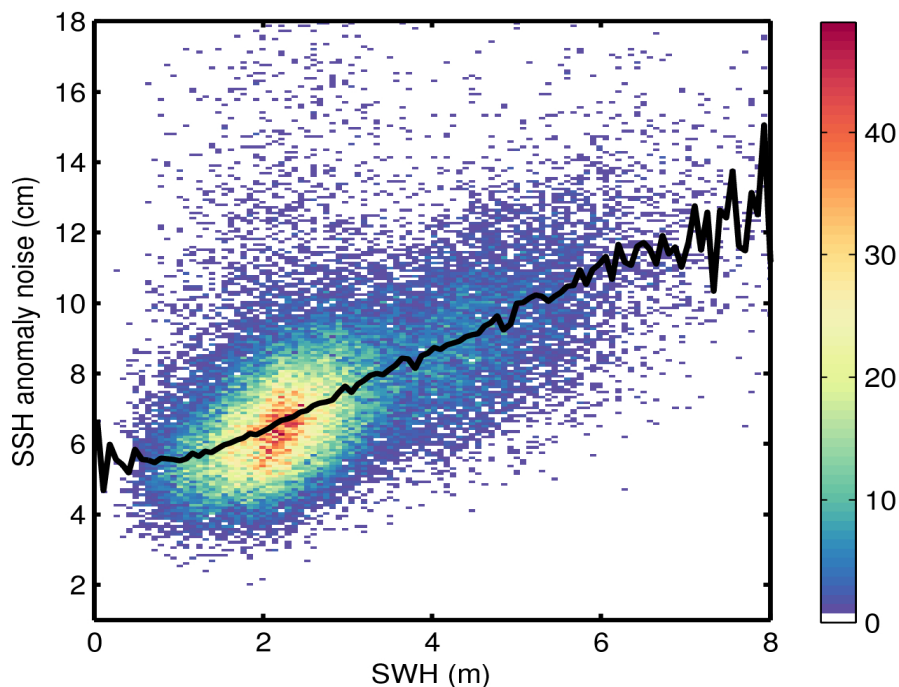
Figure 9. 2D histogram showing flag-valid SSH anomaly noise as a function of SWH for 28/02/2017. The black line denotes the median SSH anomaly noise as a function of SWH.
