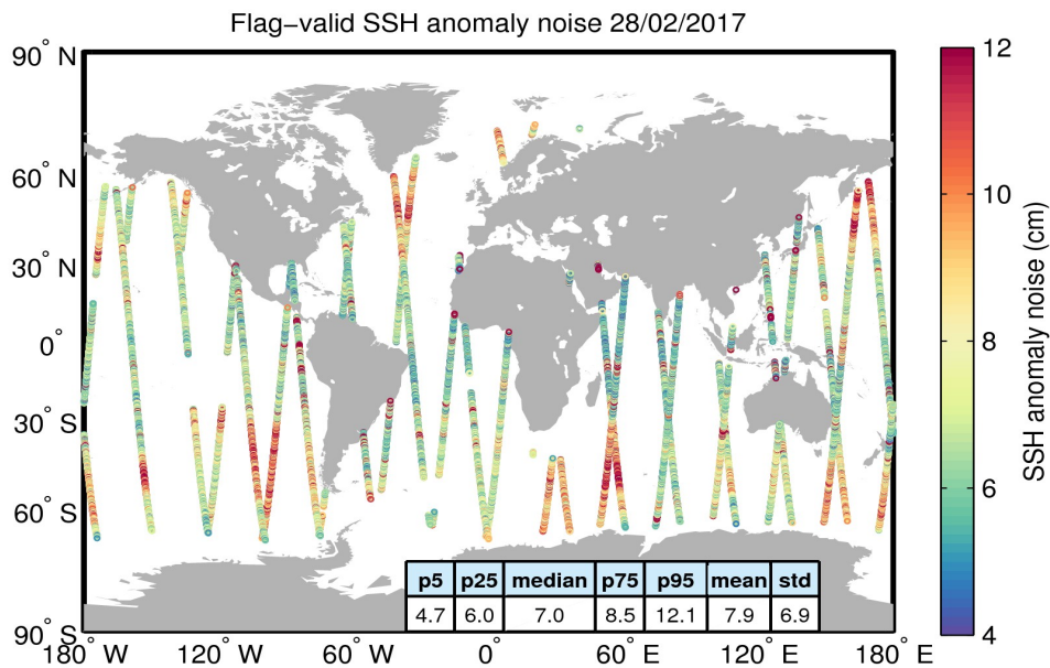
Figure 8. Geographical distribution of flag-valid 20-Hz SSH anomaly measurement noise over oceans and lakes for 28/02/2017. The statistical values shown in the table refer to the SSH anomaly noise and are calculated over all measurements shown in the figure.
