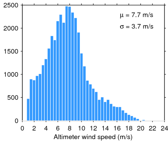
Figure 33. Histogram of flag-valid wind over oceans and lakes for 28/02/2017. The mean ( \mu ) and standard deviation ( \sigma ) are also shown. Note that values larger than 24 m/s are excluded from the histogram for the sake of readability but not from the computation of \mu and \sigma .
