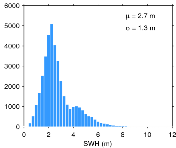
Figure 17. Histogram of flag-valid SWH over oceans and lakes for 28/02/2017. The mean ( \mu ) and standard deviation ( \sigma ) are also shown. Note that values larger than 12 m are excluded from the histogram for the sake of readability but not from the computation of \mu and \sigma .
