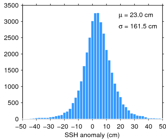
Figure 7. Histogram of flag-valid SSH anomaly over oceans and lakes for 28/02/2017. The mean ( \mu ) and standard deviation ( \sigma ) are also shown. Note that values outside [-50 50] cm are excluded from the histogram for the sake of readability but not from the computation of \mu and \sigma .
