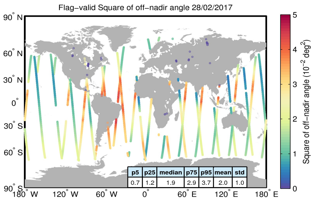
Figure 37. Geographical distribution of flag-valid mispointing data over oceans and lakes for 28/02/2017. The statistical values shown in the table refer to the mispointing in 10^{-2} \text{ deg}^2 and are calculated over all measurements shown in the figure.
