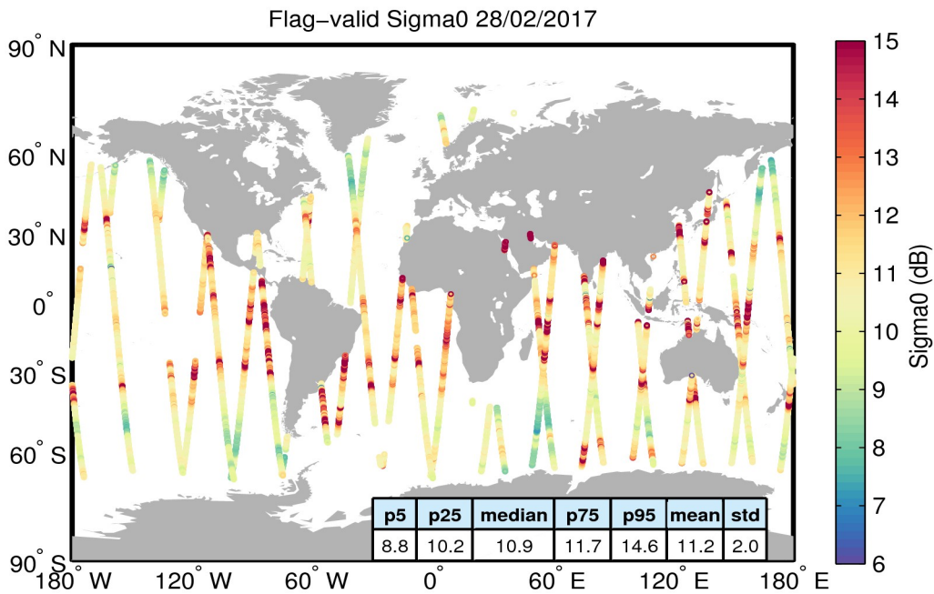
Figure 23. Geographical distribution of flag-valid sigma0 data over oceans and lakes for 28/02/2017. The statistical values shown in the table refer to the sigma0 in dB and are calculated over all measurements shown in the figure.
