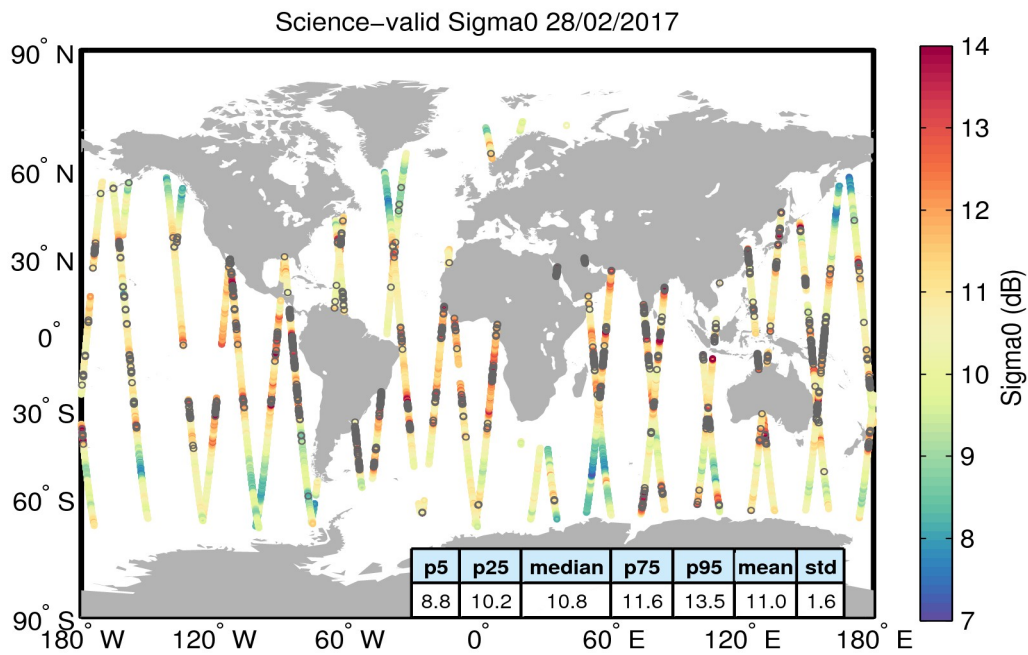
Figure 27. Geographical distribution of science-valid sigma0 data over oceans and lakes for 28/02/2017. The statistical values shown in the table refer to the sigma0 in dB and are calculated over all measurements shown in the figure. Gray circles denote records that have been rejected based on the editing criteria described in Table 4.
