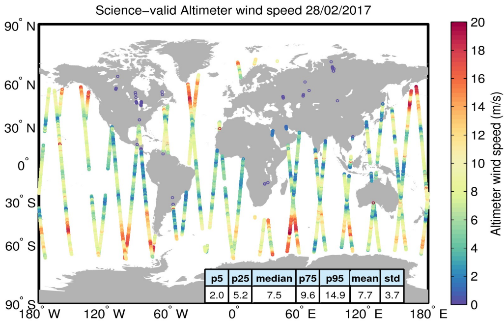
Figure 34. Geographical distribution of science-valid wind data over oceans and lakes for 28/02/2017. The statistical values shown in the table refer to the wind in m/s and are calculated over all measurements shown in the figure. Gray circles denote records that have been rejected based on the editing criteria described in Table 5.
