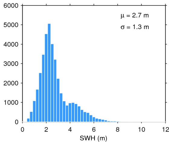
Figure 20. Histogram of science-valid SWH over oceans and lakes for 28/02/2017. The mean ( \mu ) and standard deviation ( \sigma ) are also shown. Note that values larger than 12 m are excluded from the histogram for the sake of readability but not from the computation of \mu and \sigma .
