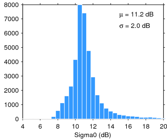
Figure 25. Histogram of flag-valid sigma0 over oceans and lakes for 28/02/2017. The mean ( \mu ) and standard deviation ( \sigma ) are also shown. Note that values outside [4 20] dB are excluded from the histogram for the sake of readability but not from the computation of \mu and \sigma .
