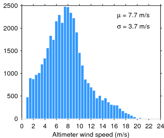
Figure 35. Histogram of science-valid wind over oceans and lakes for 28/02/2017. The mean ( \mu ) and standard deviation ( \sigma ) are also shown. Note that values larger than 24 m/s are excluded from the histogram for the sake of readability but not from the computation of \mu and \sigma .
