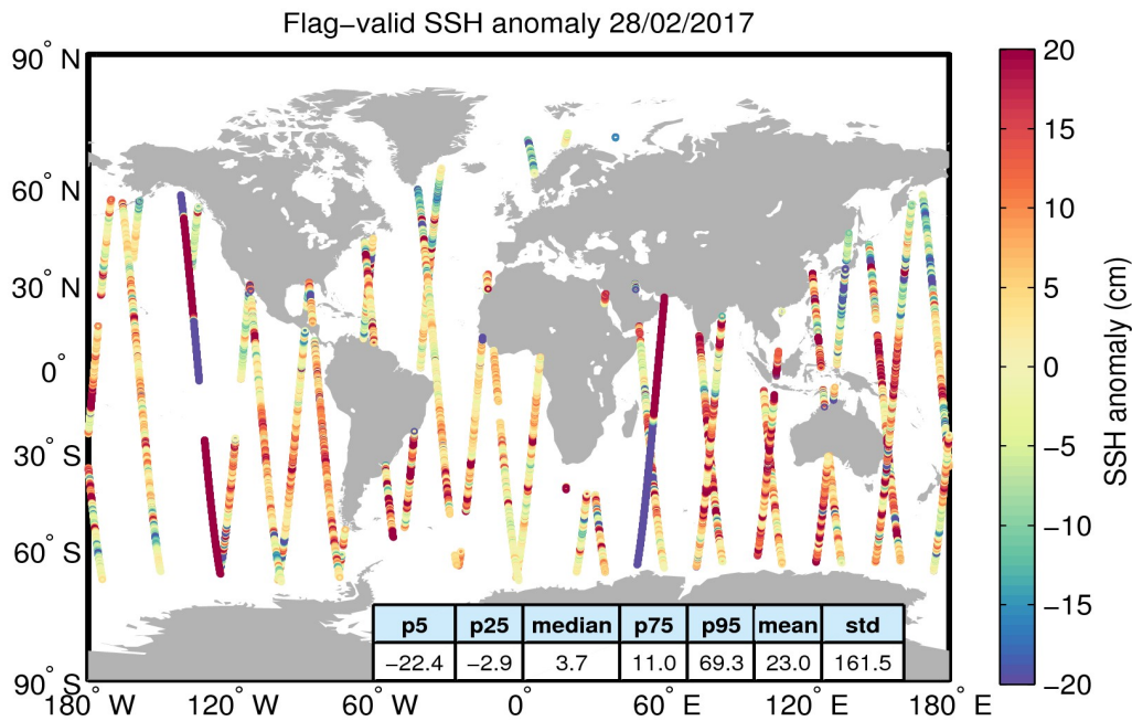
Figure 5. Geographical distribution of flag-valid 1-Hz SSH anomaly data over oceans and lakes for 28/02/2017. The statistical values shown in the table refer to the SSH anomaly in cm and are calculated over all measurements shown in the figure.
