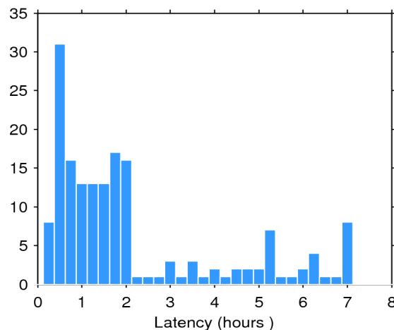
Figure 2. Histogram of the data latency for 28/02/2017. The y-axis denotes the number of files that are made available with a delay of x-hours with respect to the mean time of the records stored in the file.
