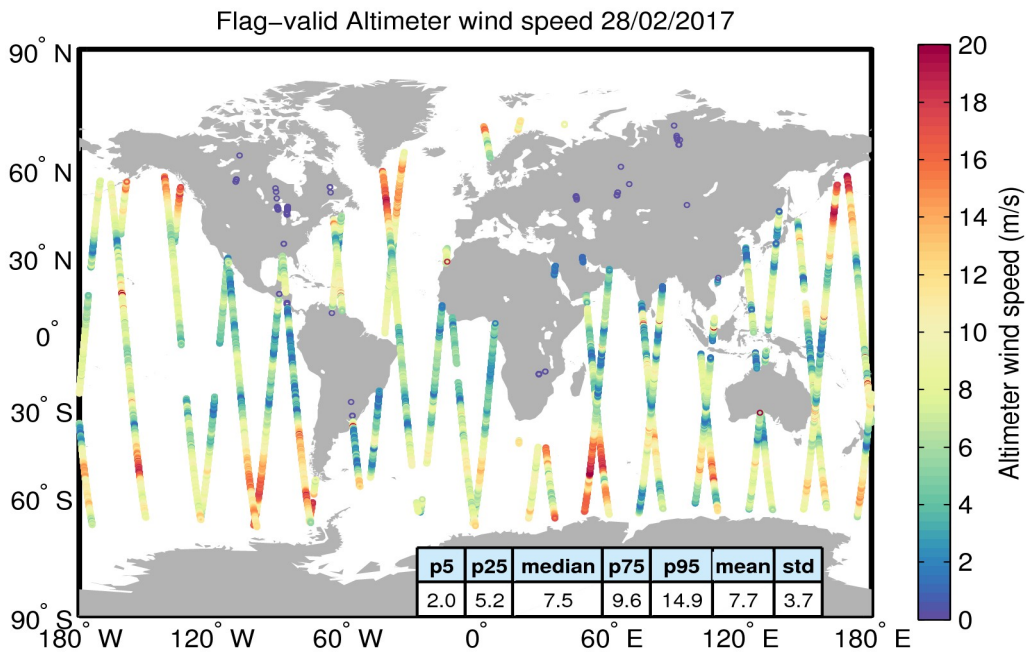
Figure 31. Geographical distribution of flag-valid wind data over oceans and lakes for 28/02/2017. The statistical values shown in the table refer to the wind in m/s and are calculated over all measurements shown in the figure.
