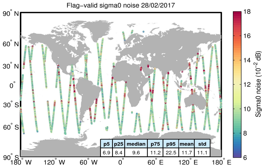
Figure 26. Geographical distribution of flag-valid 20-Hz sigma0 measurement noise over oceans and lakes for 28/02/2017. The statistical values shown in the table refer to the sigma0 noise and are calculated over all measurements shown in the figure.
