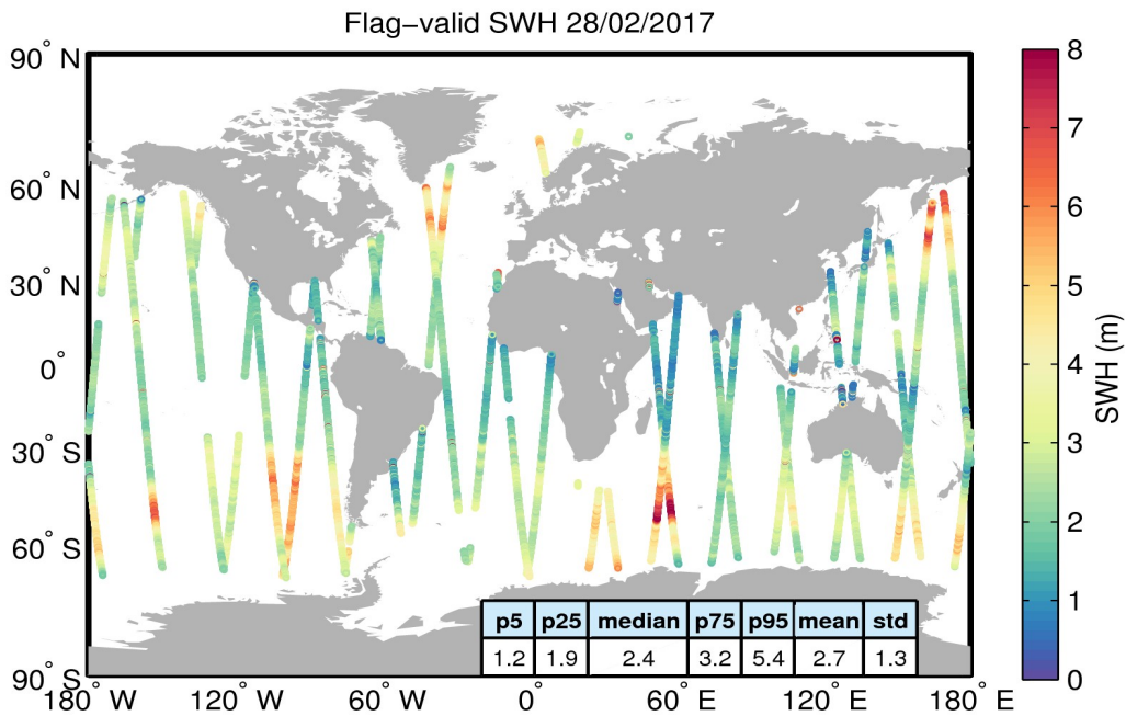
Figure 15. Geographical distribution of flag-valid SWH data over oceans and lakes for 28/02/2017. The statistical values shown in the table refer to the SWH in m and are calculated over all measurements shown in the figure.
