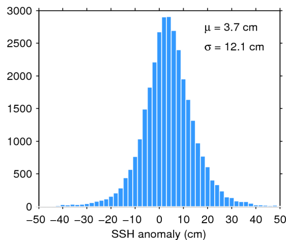
Figure 11. Histogram of science-valid SSH anomaly over oceans and lakes for 28/02/2017. The mean ( \mu ) and standard deviation ( \sigma ) are also shown. Note that values outside [-50 50] cm are excluded from the histogram for the sake of readability but not from the computation of \mu and \sigma .
