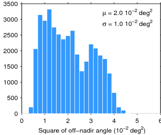
Figure 39. Histogram of flag-valid mispointing over oceans and lakes for 28/02/2017. The mean ( \mu ) and standard deviation ( \sigma ) are also shown. Note that values larger than 6 \cdot 10^{-2} \text{ deg}^2 are excluded from the histogram for the sake of readability but not from the computation of \mu and \sigma .
