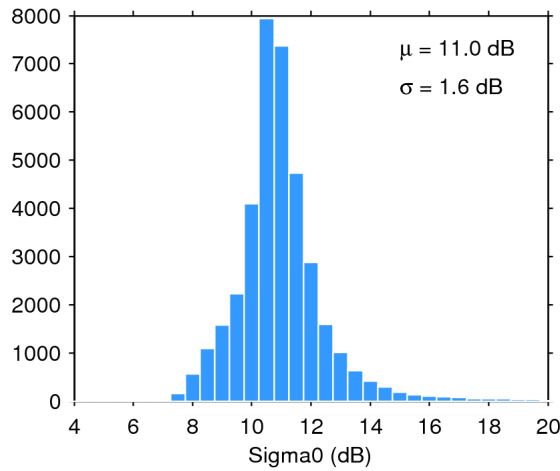
Figure 28. Histogram of science-valid sigma0 over oceans and lakes for 28/02/2017. The mean ( \mu ) and standard deviation ( \sigma ) are also shown. Note that values outside [4 20] dB are excluded from the histogram for the sake of readability but not from the computation of \mu and \sigma .
