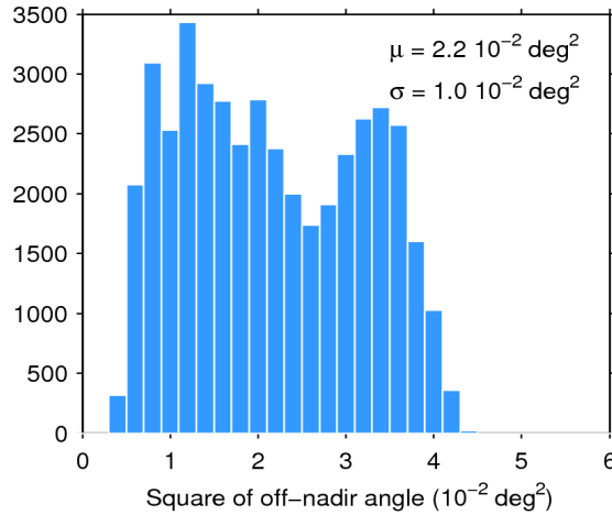
Figure 39. Histogram of flag-valid mispointing over oceans and lakes for 27/02/2017. The mean ( \mu ) and standard deviation ( \sigma ) are also shown. Note that values larger than 6 \cdot 10^{-2} \text{ deg}^2 are excluded from the histogram for the sake of readability but not from the computation of \mu and \sigma .
