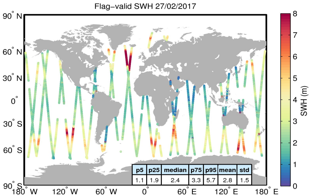
Figure 15. Geographical distribution of flag-valid SWH data over oceans and lakes for 27/02/2017. The statistical values shown in the table refer to the SWH in m and are calculated over all measurements shown in the figure.
