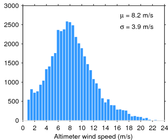
Figure 35. Histogram of science-valid wind over oceans and lakes for 27/02/2017. The mean ( \mu ) and standard deviation ( \sigma ) are also shown. Note that values larger than 24 m/s are excluded from the histogram for the sake of readability but not from the computation of \mu and \sigma .
