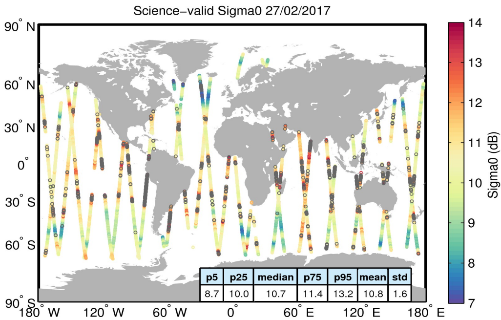
Figure 27. Geographical distribution of science-valid sigma0 data over oceans and lakes for 27/02/2017. The statistical values shown in the table refer to the sigma0 in dB and are calculated over all measurements shown in the figure. Gray circles denote records that have been rejected based on the editing criteria described in Table 4.
