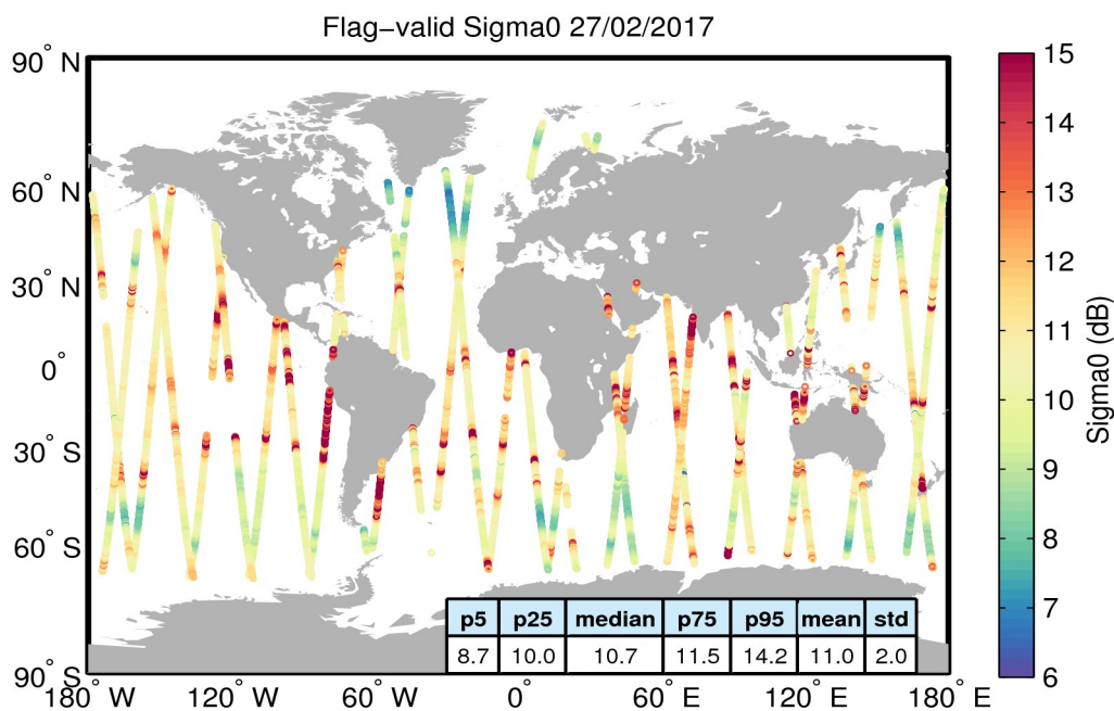
Figure 23. Geographical distribution of flag-valid sigma0 data over oceans and lakes for 27/02/2017. The statistical values shown in the table refer to the sigma0 in dB and are calculated over all measurements shown in the figure.
