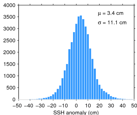
Figure 11. Histogram of science-valid SSH anomaly over oceans and lakes for 27/02/2017. The mean ( \mu ) and standard deviation ( \sigma ) are also shown. Note that values outside [-50 50] cm are excluded from the histogram for the sake of readability but not from the computation of \mu and \sigma .
