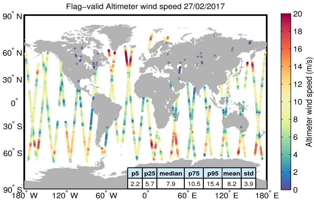
Figure 31. Geographical distribution of flag-valid wind data over oceans and lakes for 27/02/2017. The statistical values shown in the table refer to the wind in m/s and are calculated over all measurements shown in the figure.
