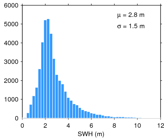
Figure 17. Histogram of flag-valid SWH over oceans and lakes for 27/02/2017. The mean ( \mu ) and standard deviation ( \sigma ) are also shown. Note that values larger than 12 m are excluded from the histogram for the sake of readability but not from the computation of \mu and \sigma .
