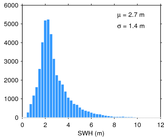
Figure 20. Histogram of science-valid SWH over oceans and lakes for 27/02/2017. The mean ( \mu ) and standard deviation ( \sigma ) are also shown. Note that values larger than 12 m are excluded from the histogram for the sake of readability but not from the computation of \mu and \sigma .
