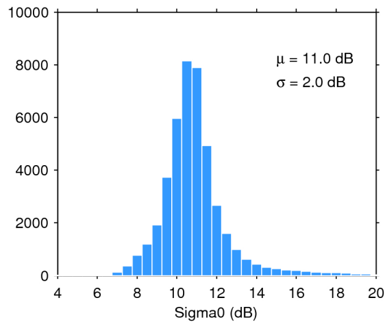
Figure 25. Histogram of flag-valid sigma0 over oceans and lakes for 27/02/2017. The mean ( \mu ) and standard deviation ( \sigma ) are also shown. Note that values outside [4 20] dB are excluded from the histogram for the sake of readability but not from the computation of \mu and \sigma .
