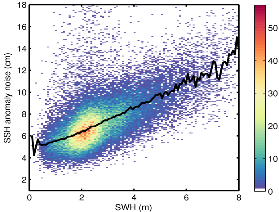
Figure 9. 2D histogram showing flag-valid SSH anomaly noise as a function of SWH for 27/02/2017. The black line denotes the median SSH anomaly noise as a function of SWH.
