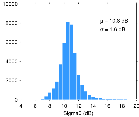
Figure 28. Histogram of science-valid sigma0 over oceans and lakes for 27/02/2017. The mean ( \mu ) and standard deviation ( \sigma ) are also shown. Note that values outside [4 20] dB are excluded from the histogram for the sake of readability but not from the computation of \mu and \sigma .
